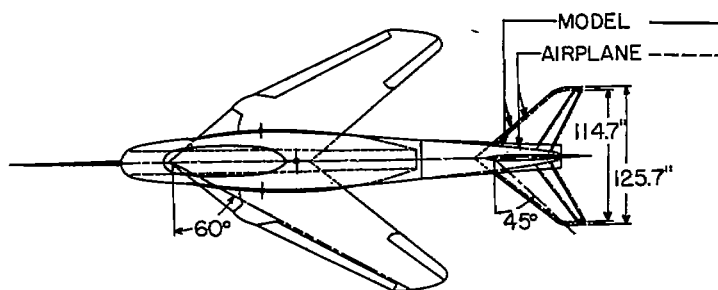
Figure 1.- Plan form of airplane A.
