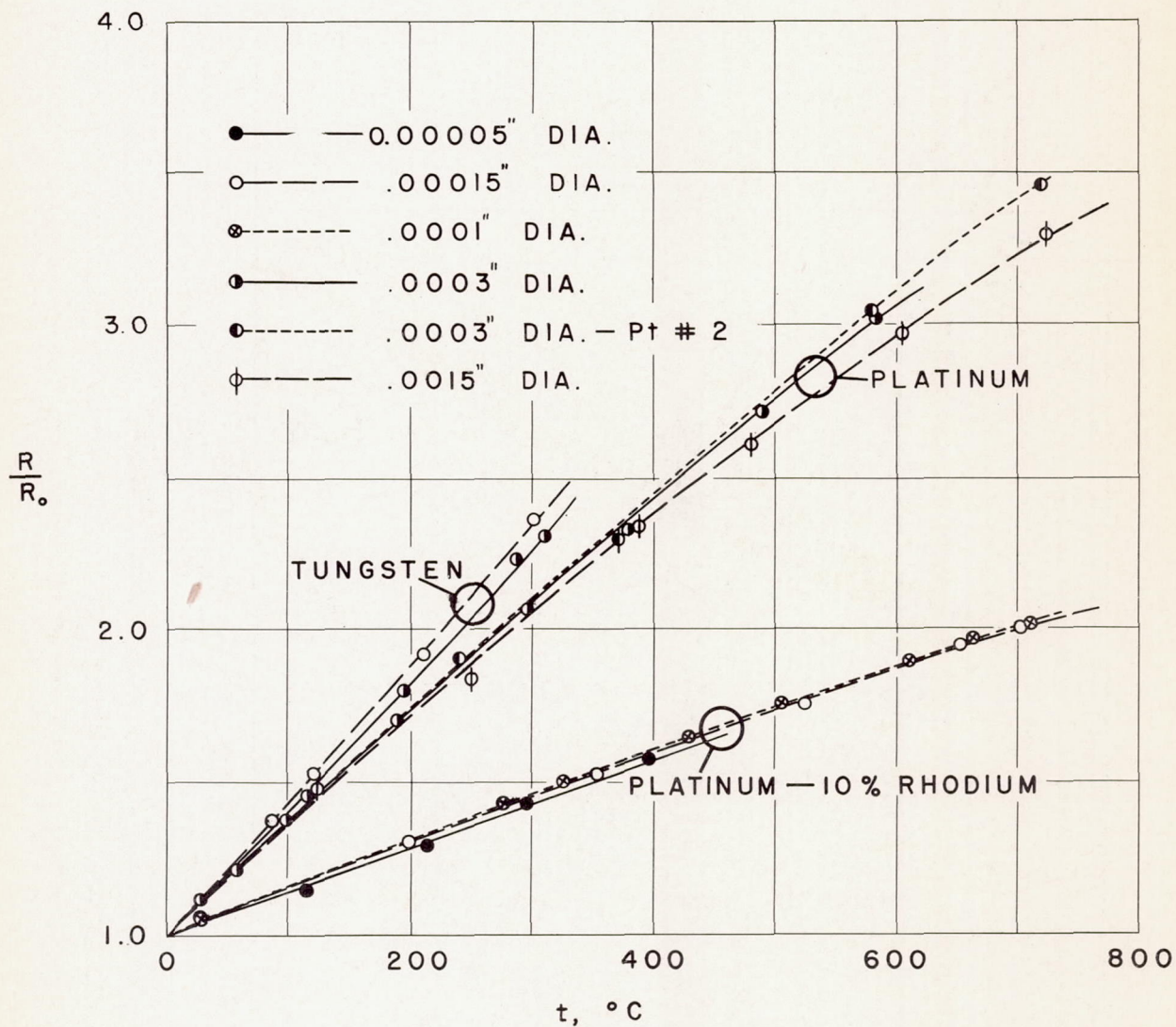
Figure 8.- Temperature-resistance relationship for various wires.
