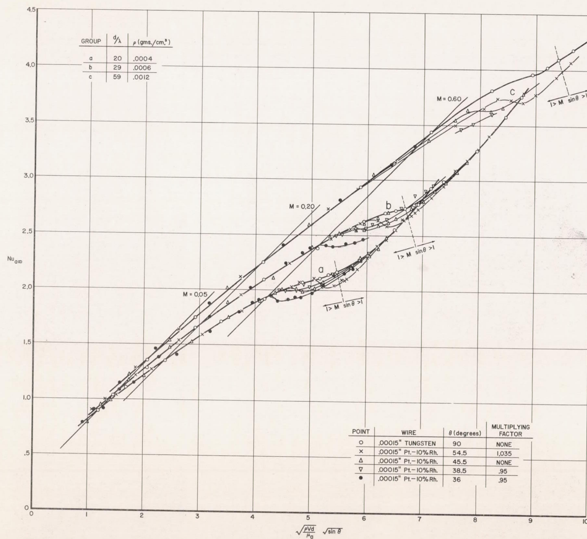
Figure 27.- Comparison of Nusselt numbers of several swept wires with Nusselt number of a normal wire at selected Mach numbers and densities.
