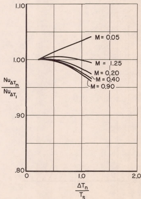
(l) 0.0015-inch-diameter platinum wire; \rho = 0.0012 gram per cubic centimeter; d/\lambda = 590 .
