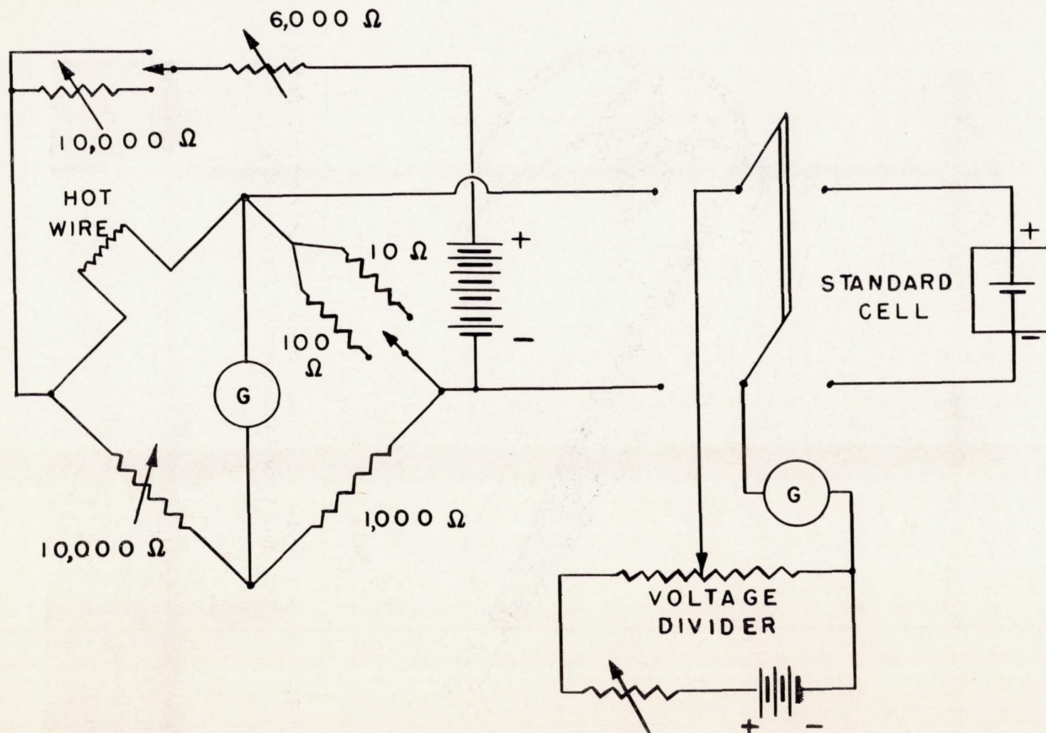
Figure 6.- Electrical circuit.
