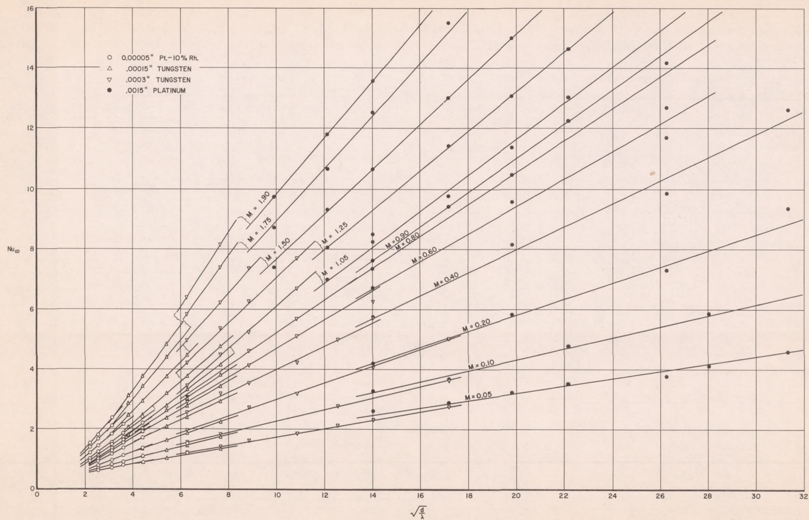
Figure 16.- Variation of Nusselt number with \sqrt{d/\lambda} for infinitely long wires.
