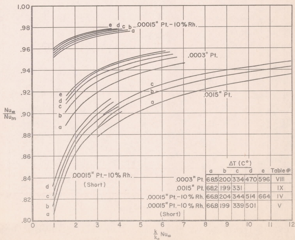
Figure 12.- End-loss correction factors.
