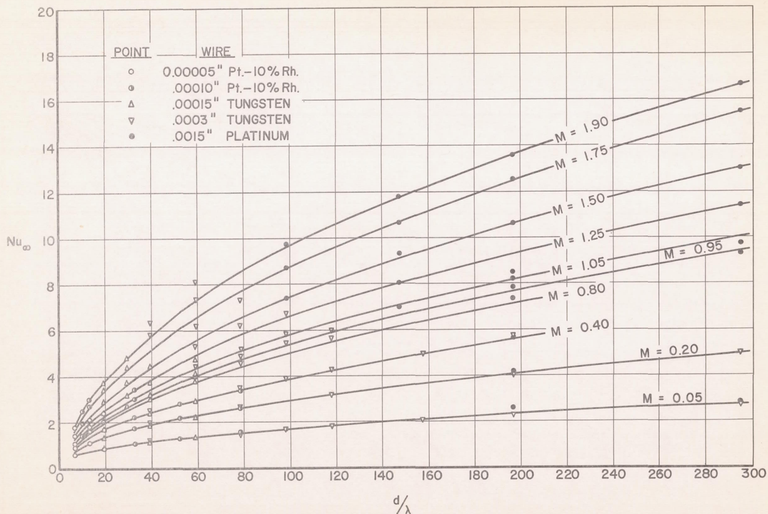
Figure 15.- Variation of Nusselt number with d/\lambda for infinitely long wires.
