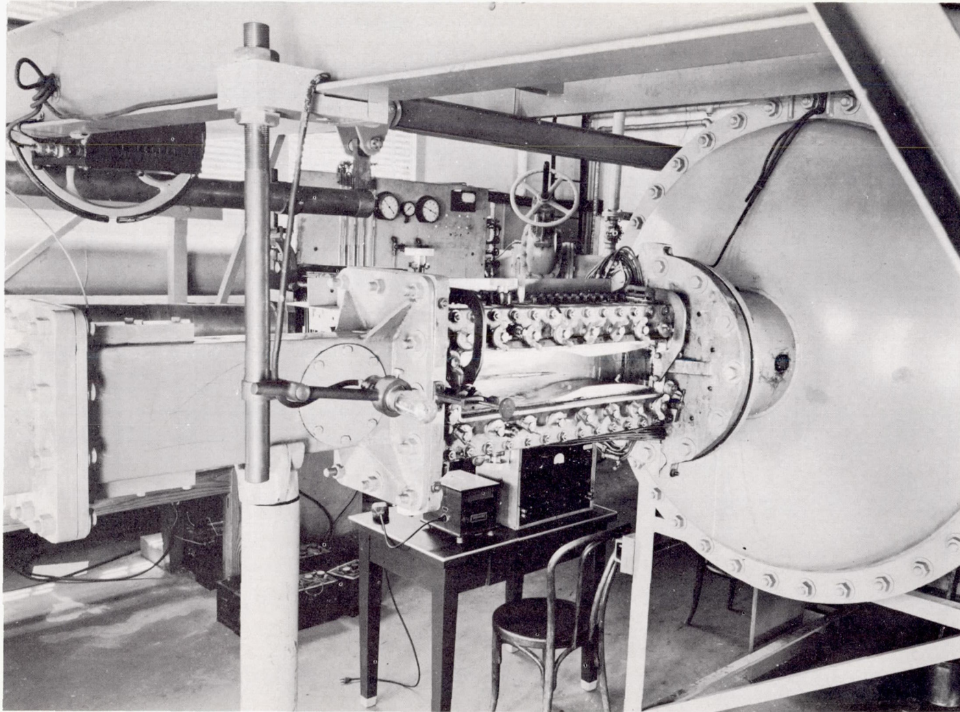
Figure 2.- Test section with supersonic blocks. L-87568
