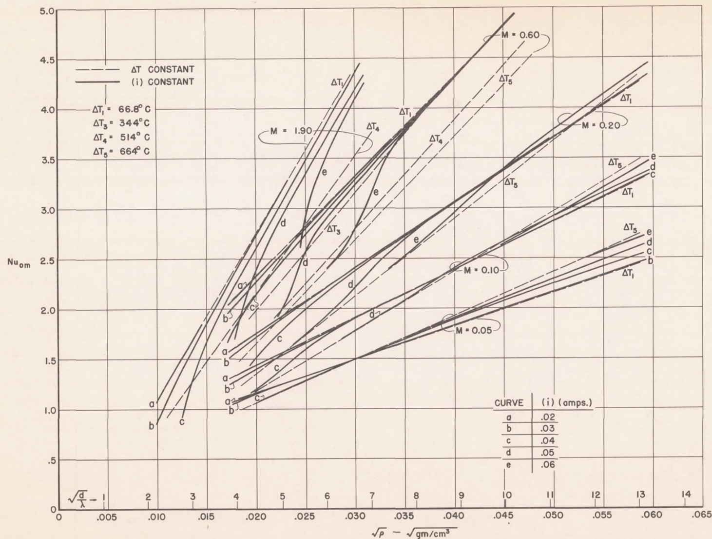
Figure 23.- Comparison of hot-wire calibrations with density variable under constant-temperature and constant-current operation. 0.00015-inch-diameter platinum wire containing 10 percent rhodium.
