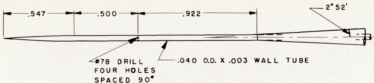
Figure 3.- Static-pressure probe. Dimensions are in inches.
