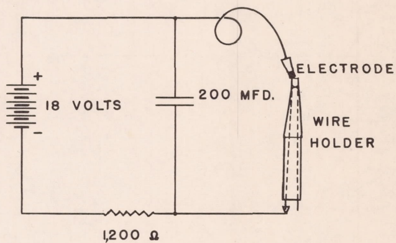
Figure 10.- Electric-arc welding circuit.
