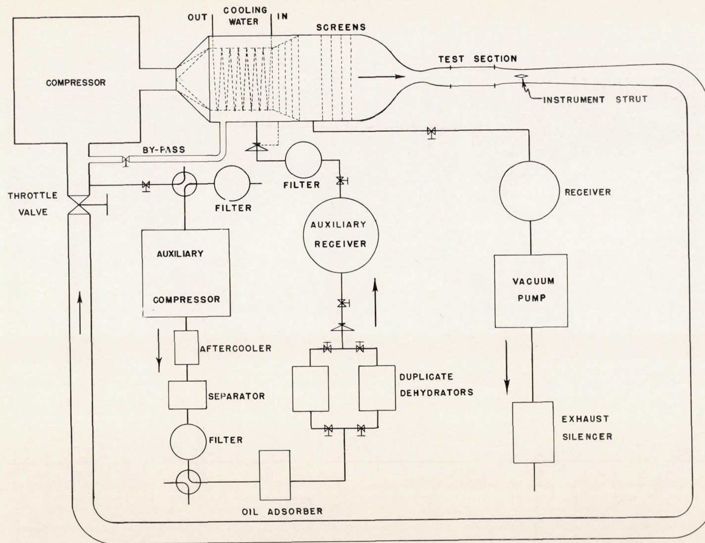
Figure 1.- Diagrammatic sketch of supersonic wind tunnel.
