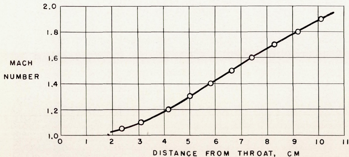
Figure 4.- Calibration curve for supersonic nozzle. \rho = 0.0006 gram per cubic centimeter.
