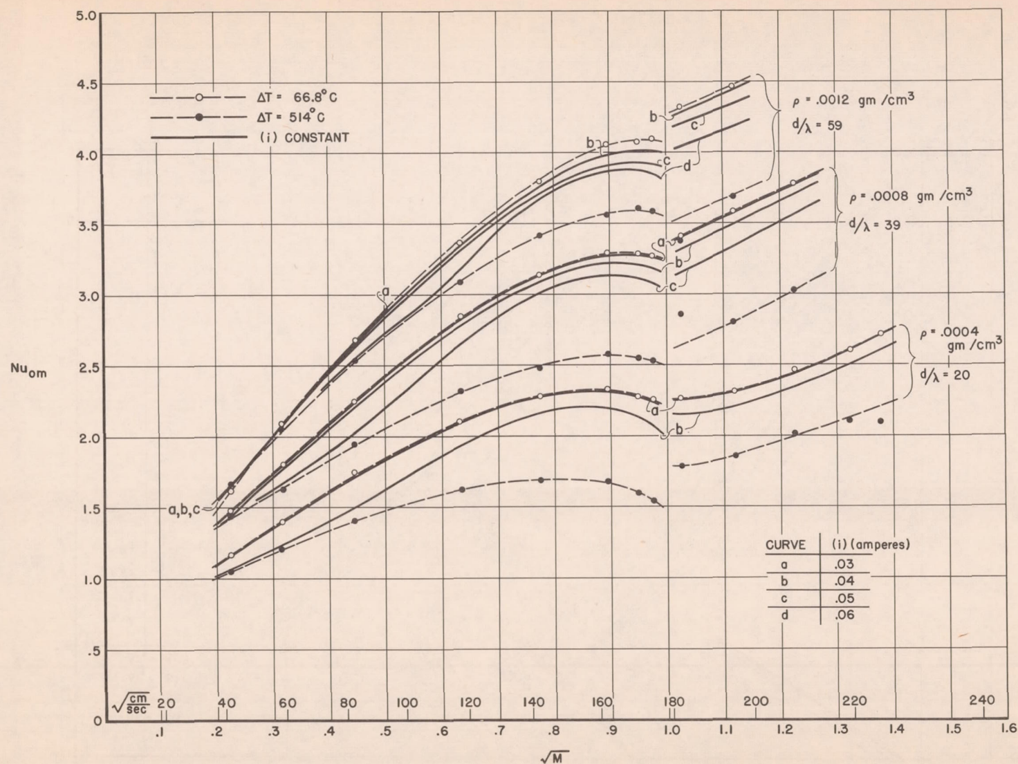
Figure 24.- Comparison of hot-wire calibrations with Mach number variable under constant-temperature and constant-current operation. 0.00015-inch-diameter platinum wire containing 10 percent rhodium.
