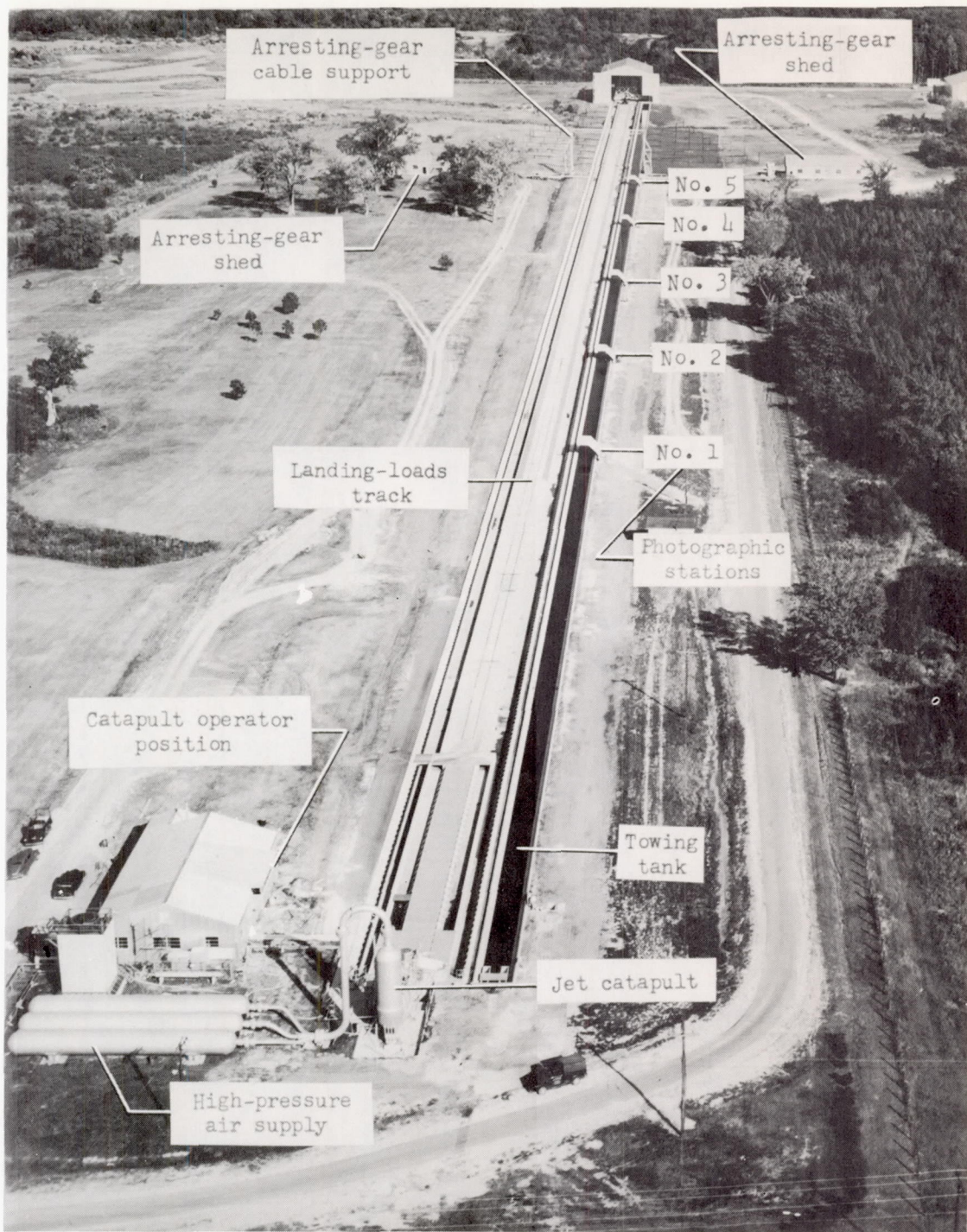
Figure 3.- Aerial view of the Langley high-speed hydrodynamics facility. L-95913
