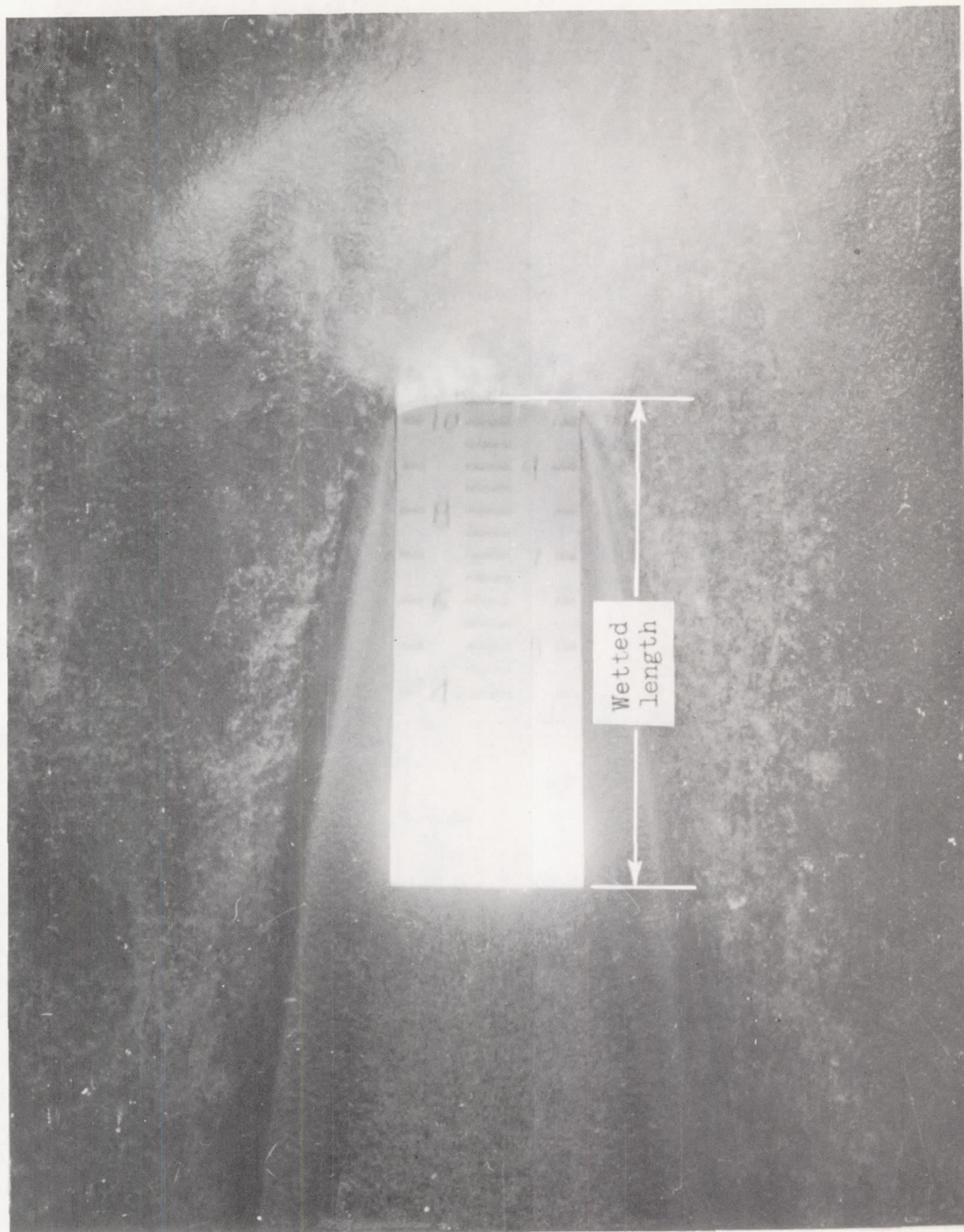
Figure 7.- Typical underwater photograph. \tau = 18^\circ ; V = 98.9 fps. L-95914
