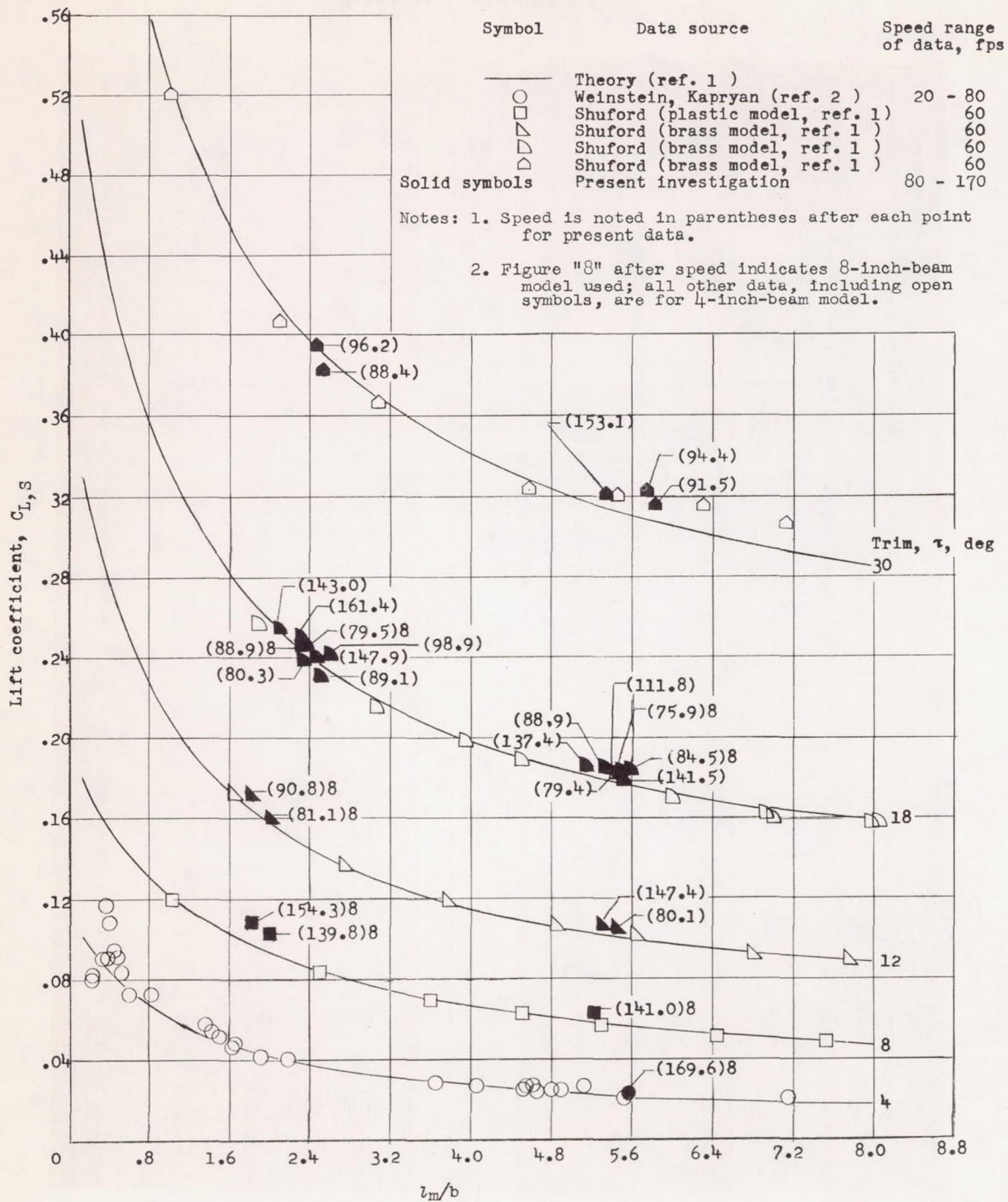
Figure 8.- Comparison of data from the high-speed hydrodynamics facility with theory and with data from lower speed towing tanks.
