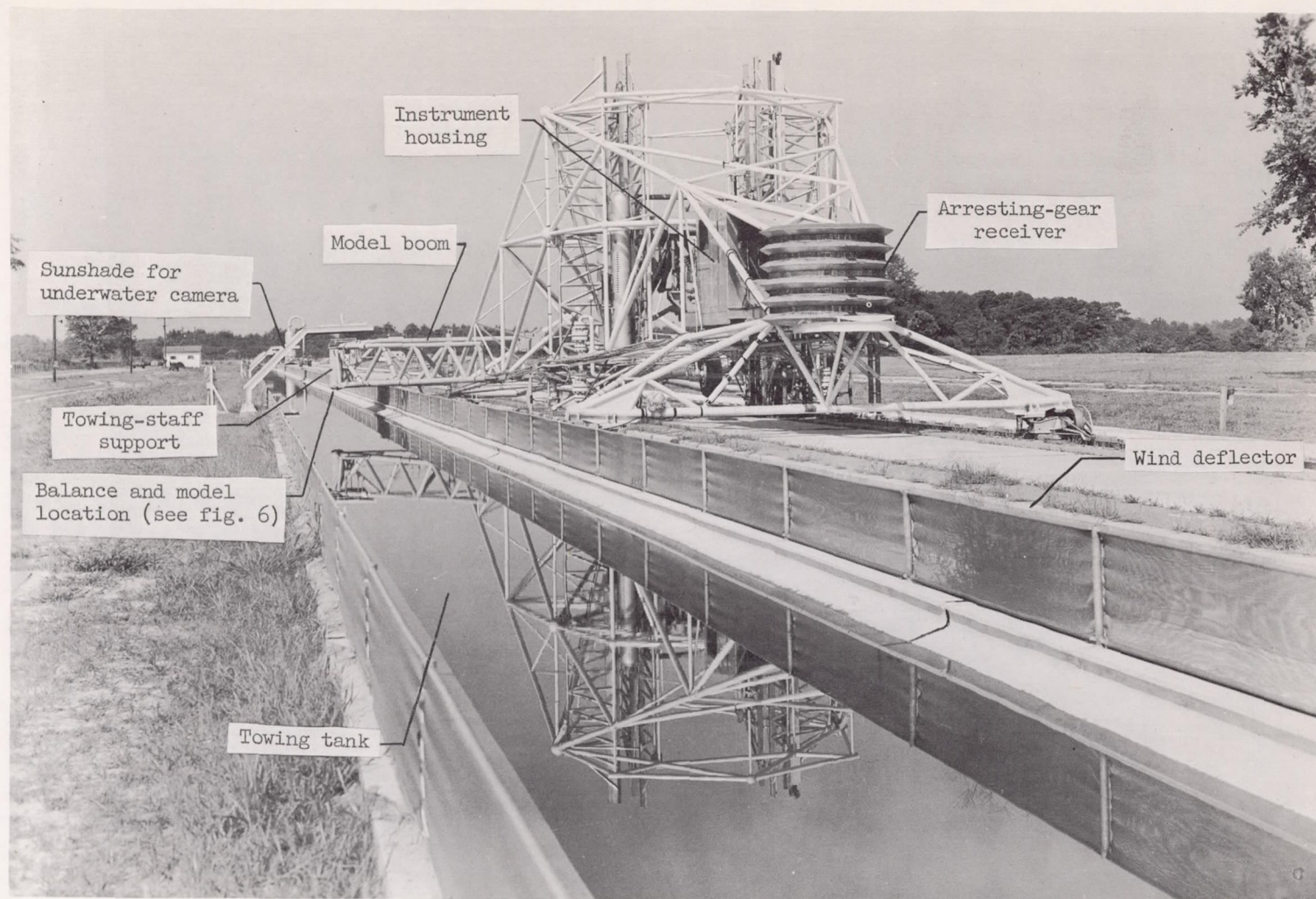
Figure 4.- Photograph of landing-loads carriage with temporary boom installed.
