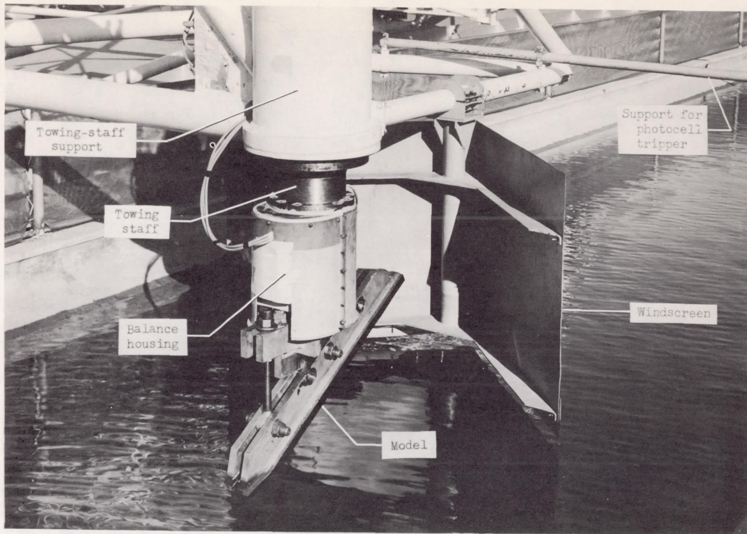
L-96656.1 Figure 6.- Photograph of test setup with 4-inch-beam model installed.
