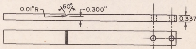
(c) Rectangular, notched specimen
