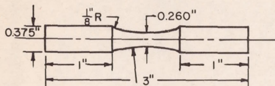
(a) Unnotched specimen
