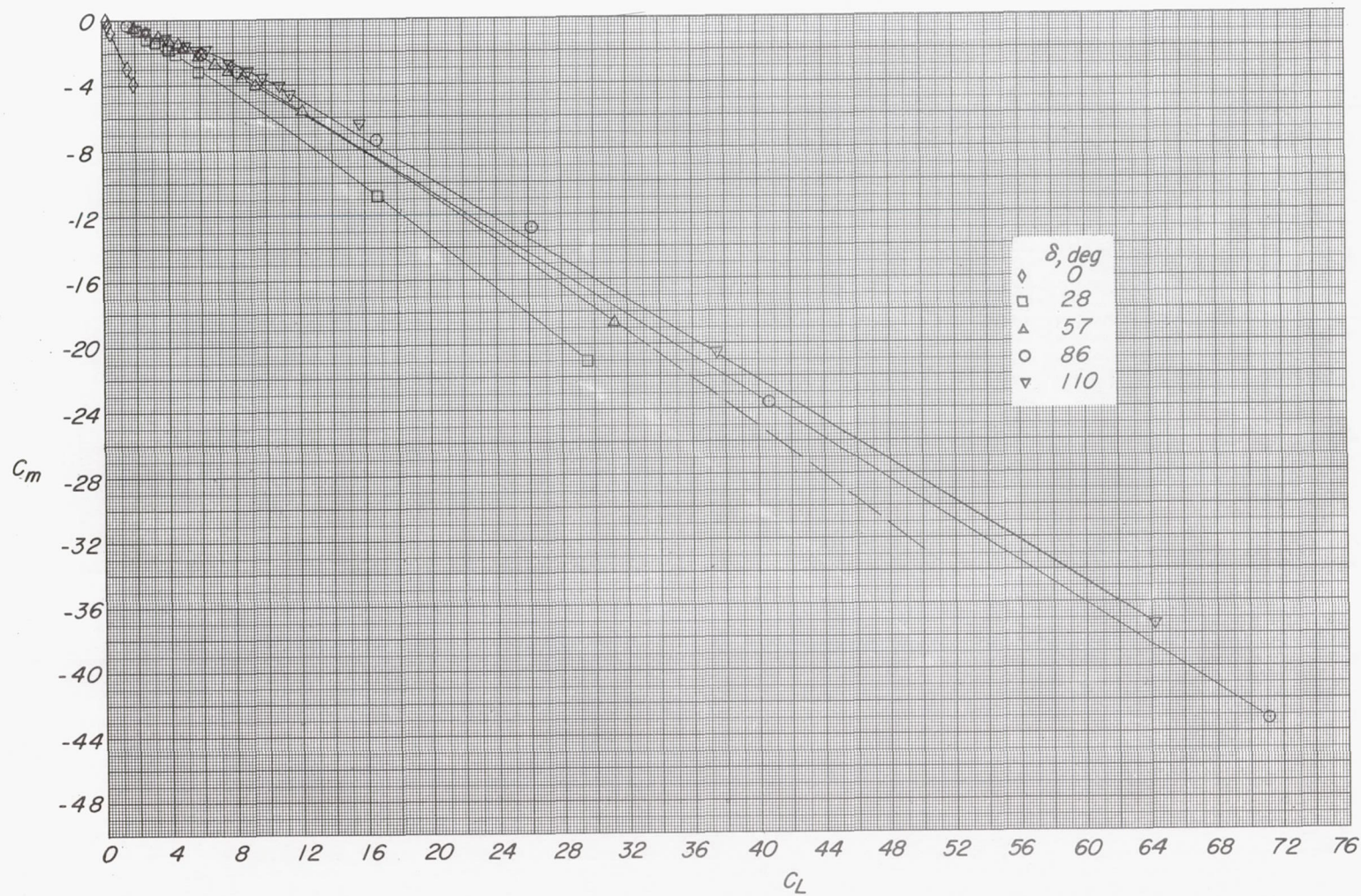
(c) C_m against C_L .
