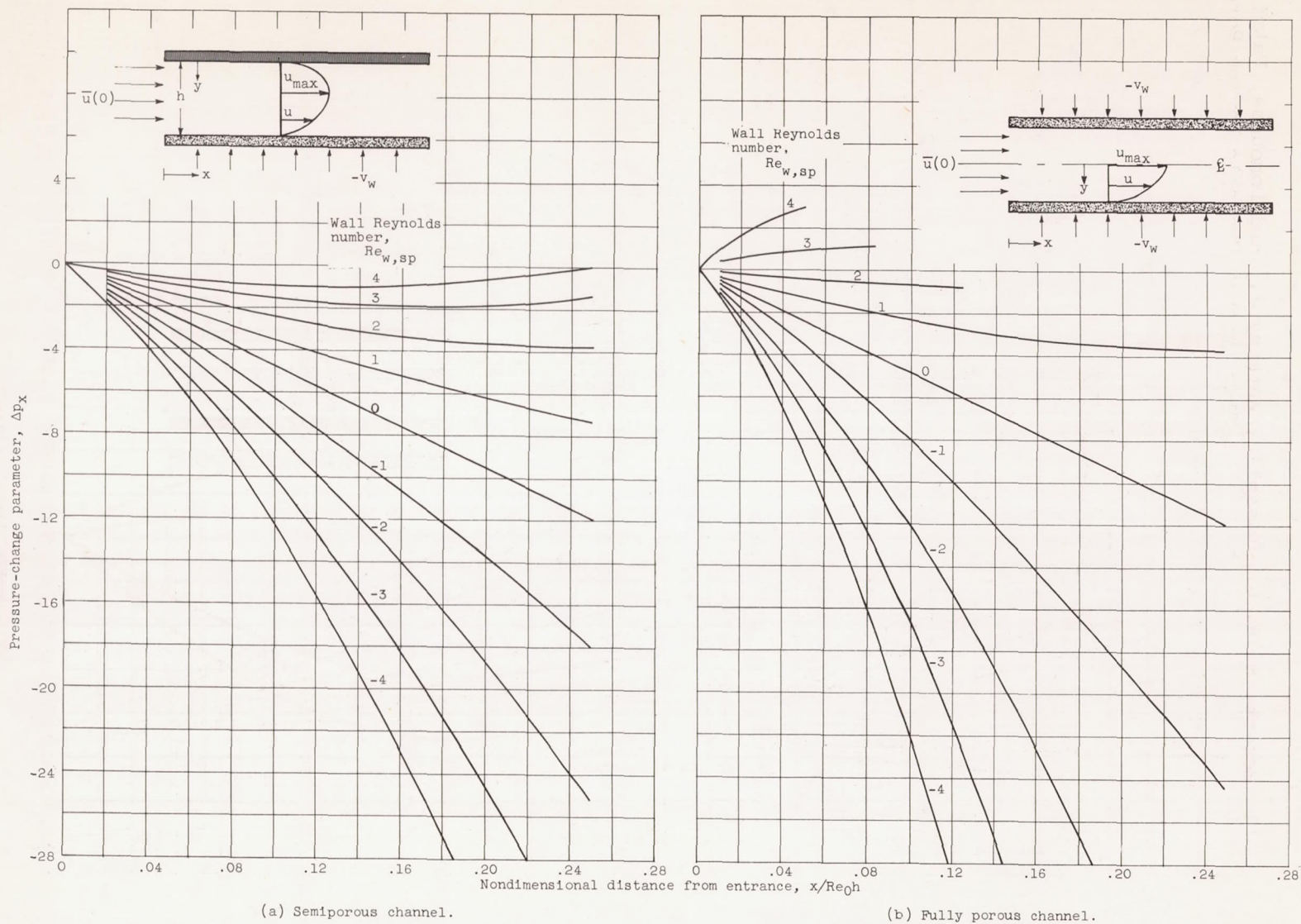
Figure 4. - Pressure change in porous channels; 0 \leq \frac{x}{Re_0h} \leq 0.25 .
