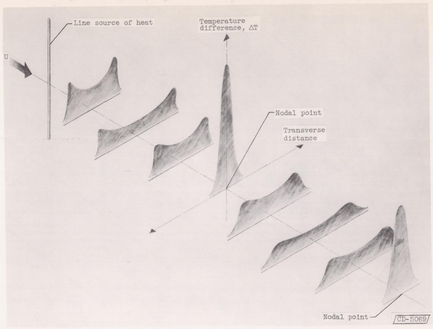
Figure 5. - Typical time-mean temperature profiles in mixing region for small deformation of the molecular-diffusion wake.
