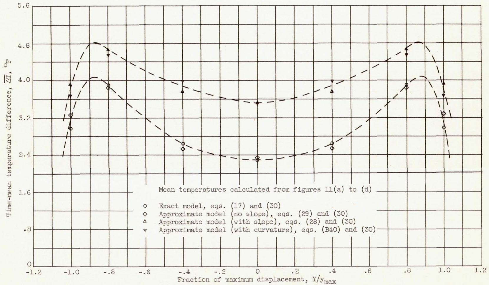
Figure 12. - Comparison of exact and approximate solutions for mean temperature. Dimensionless axial position, 7.5; coefficient of thermal diffusivity, 2.37 \times 10^{-4} square feet per second; stream-velocity - frequency ratio, 0.0338 foot; ratio of root-mean-square velocity fluctuation to stream velocity, 0.947; rate of heat release from line source per unit length, 0.0308 Btu per second per foot.
