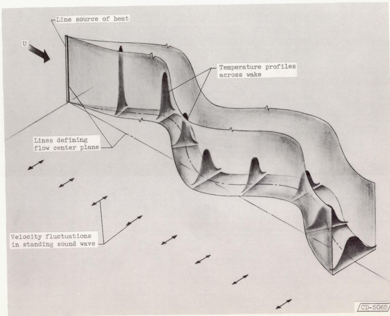
(a) Typical temperature profiles in molecular-diffusion wake at an instant.
