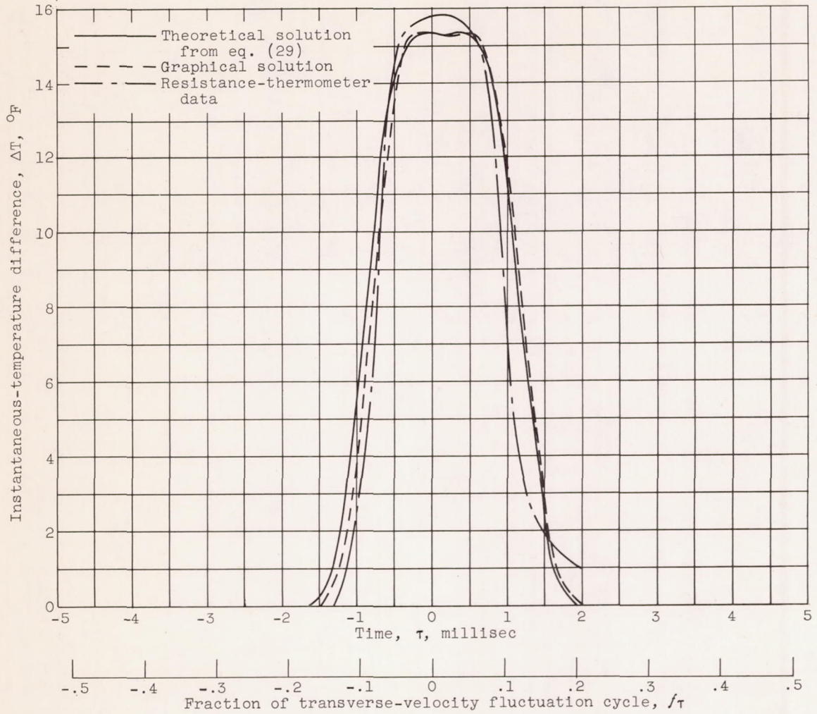
Figure 9. - Concluded. Instantaneous temperature-time variation at various lateral positions. X = 2.98 inches or fX/U = 1.47 .
