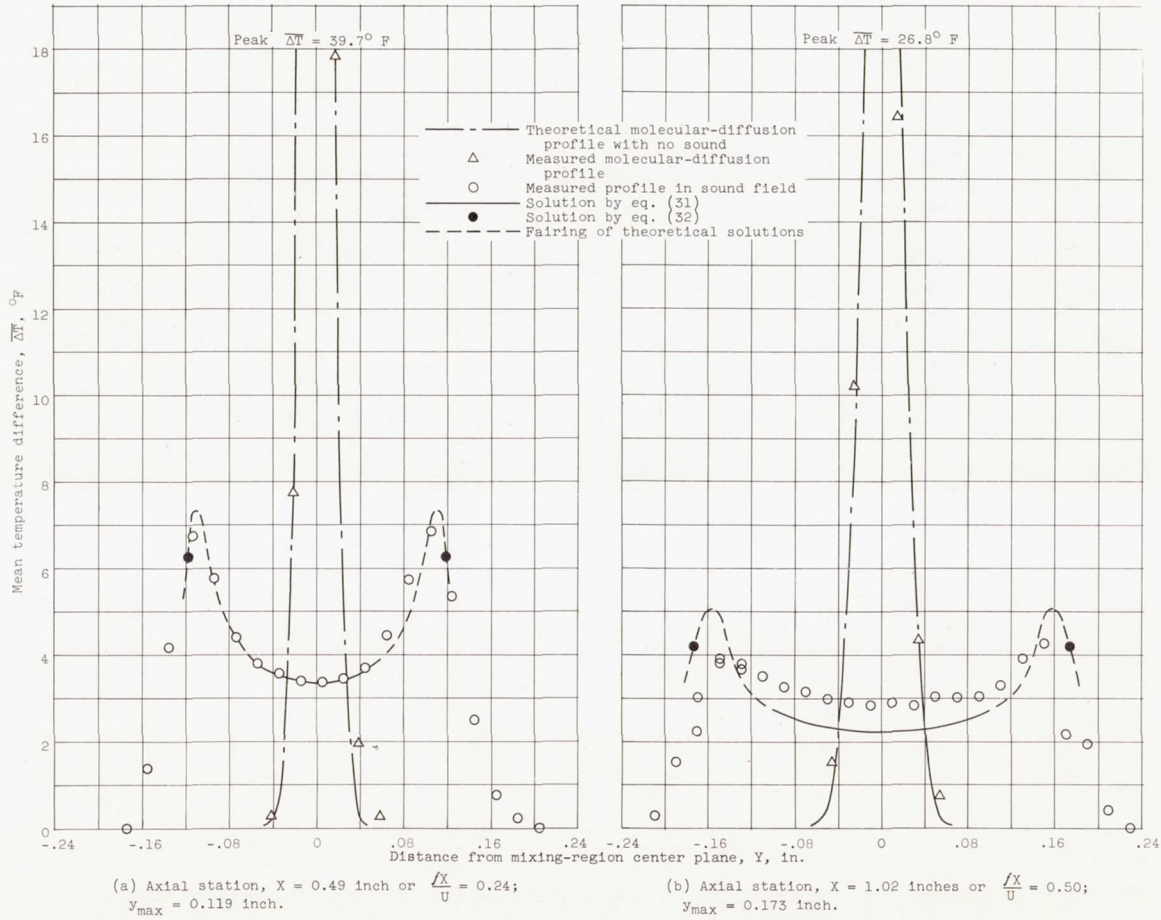
Figure 10. - Comparison of theoretical and experimental time-mean temperature-difference profiles at various axial stations.
