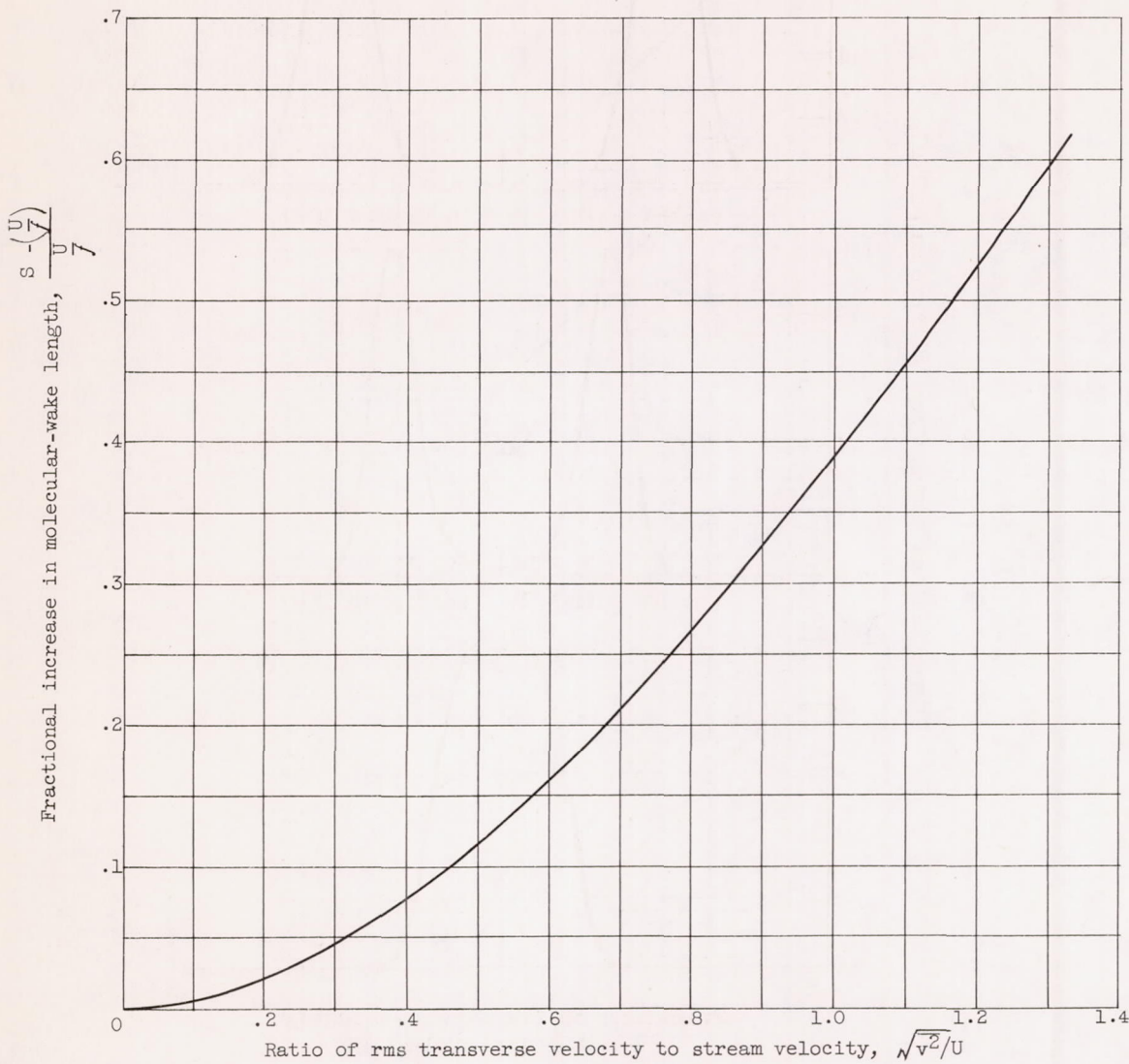
(a) Stretching of molecular-diffusion wake.
