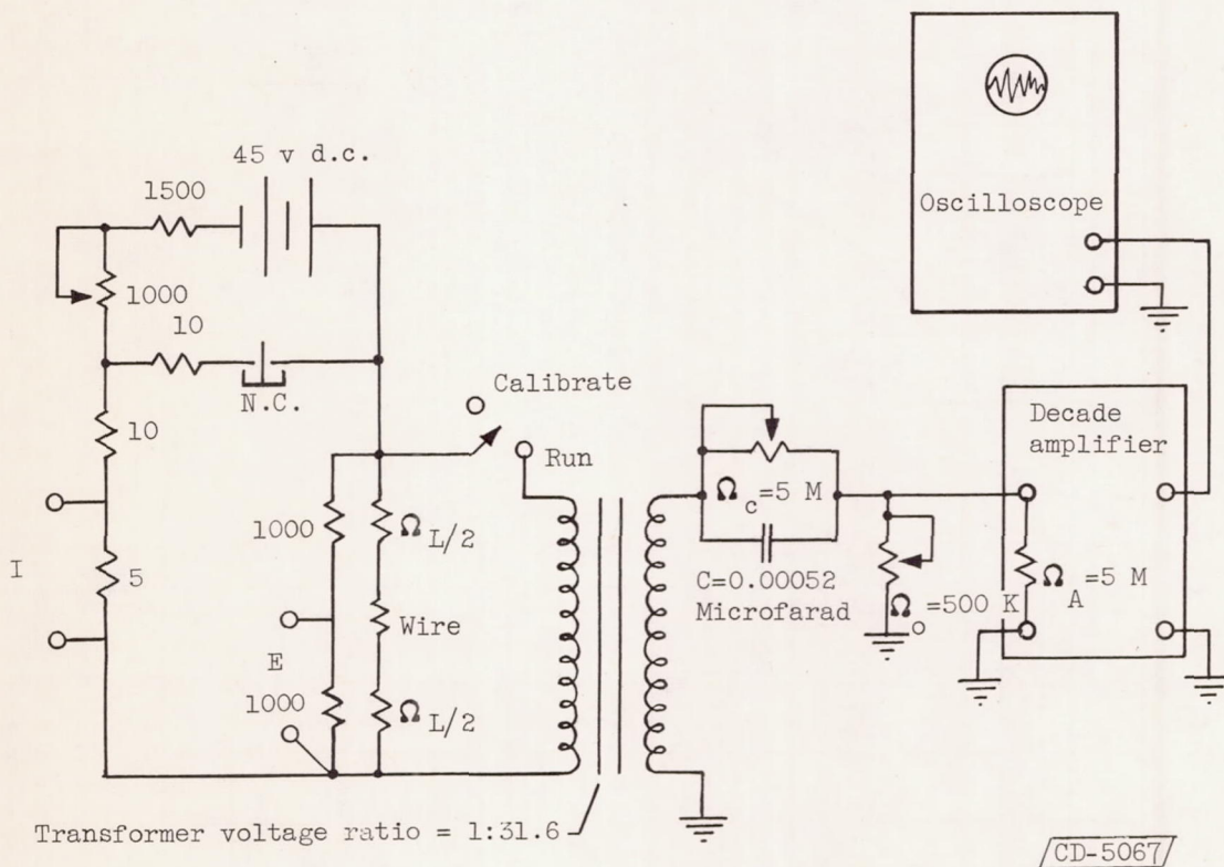
(b) Resistance-thermometer circuit.
