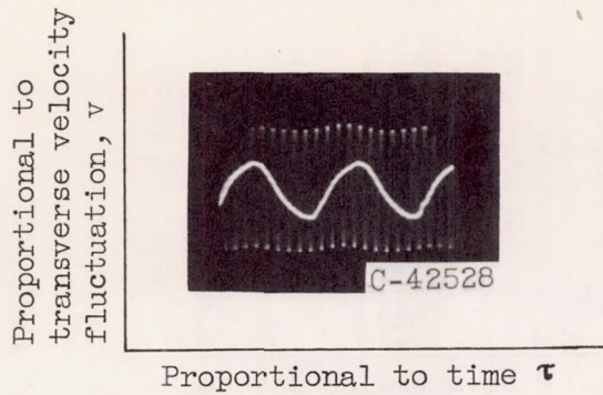
(a) Typical oscillogram of transverse velocity fluctuation.
