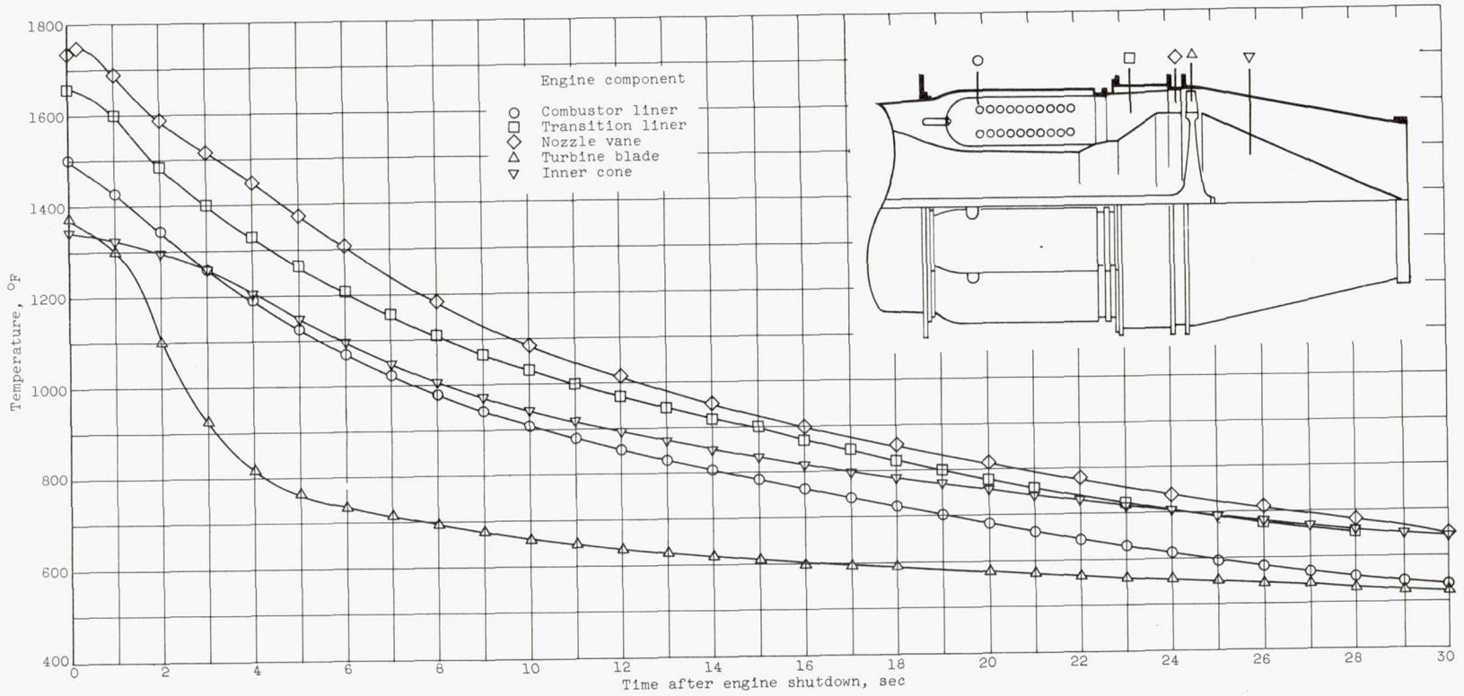
Figure 29. - History of maximum temperatures on engine components in main gas stream.
