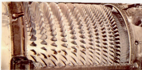
Figure 26. - Fuel-dye stains on J35-engine compressor following F-84 crash.
