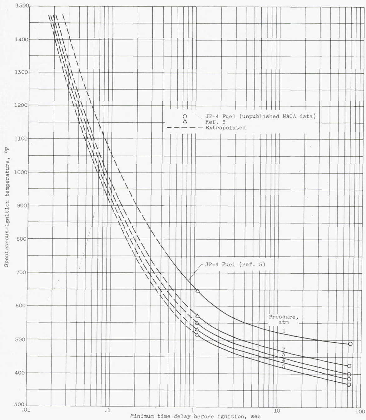
Figure 8. - Ignition characteristics of aviation fuels.
