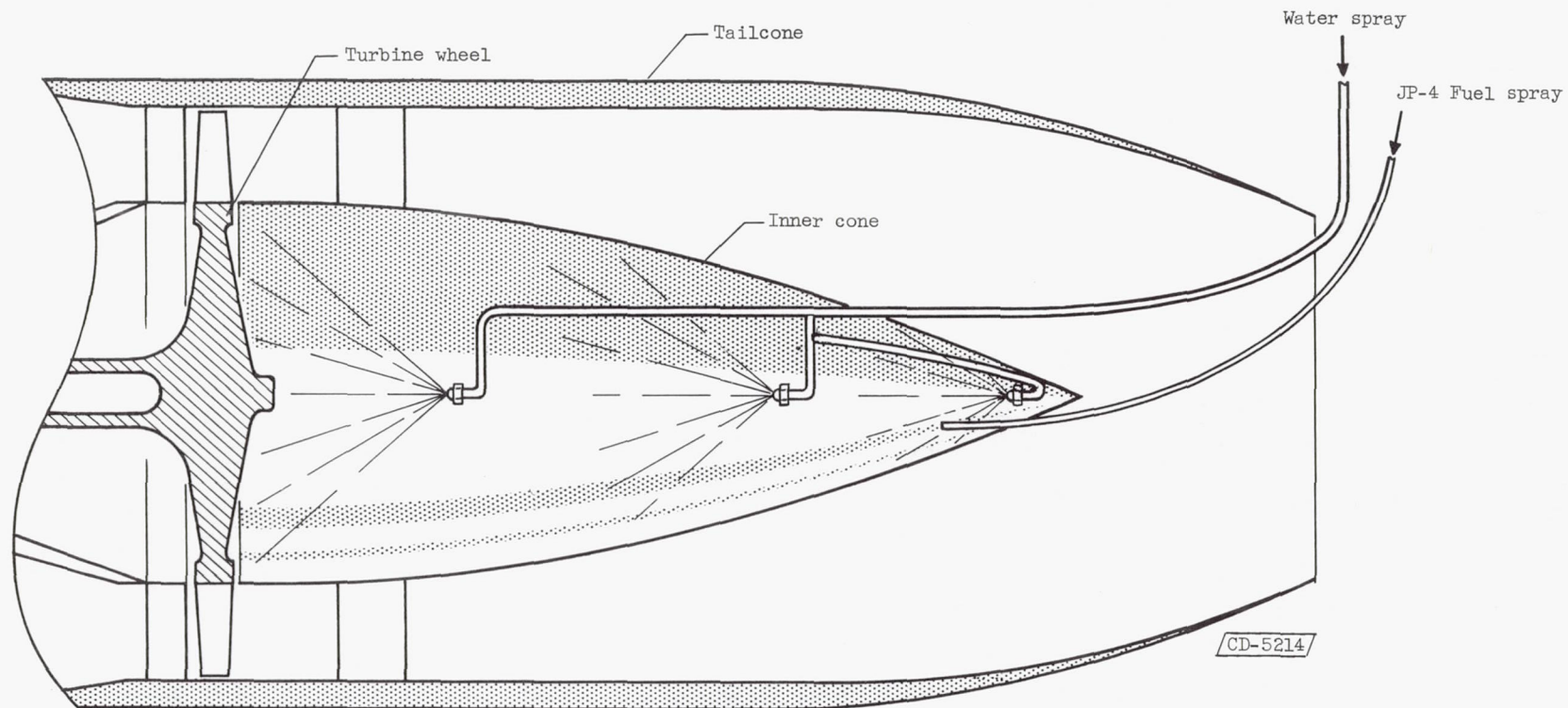
Figure 34. - Sketch of typical equipment used to study ignition hazard (J30 inner tailcone).
