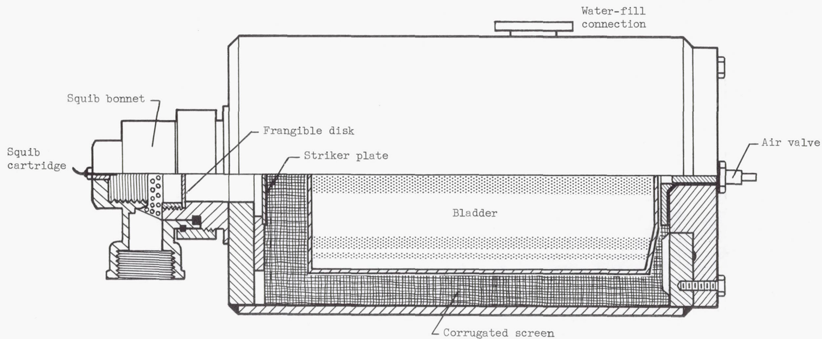
Figure 23. - Bladder-type water reservoir.
