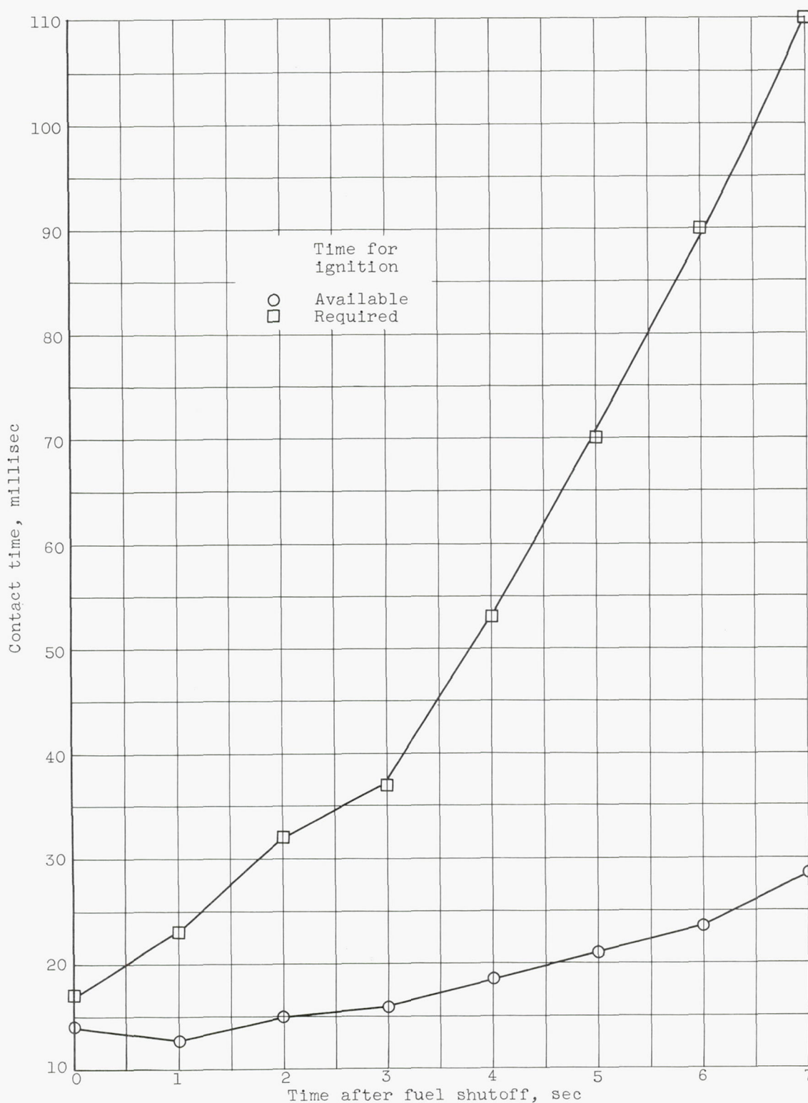
Figure 10. - Analysis of ignition probability for J35 combustor.
