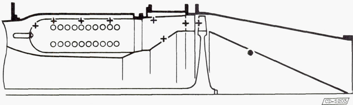
Figure 7. - Maximum temperatures of metal components in main gas streams of J47 and J35 engines.
