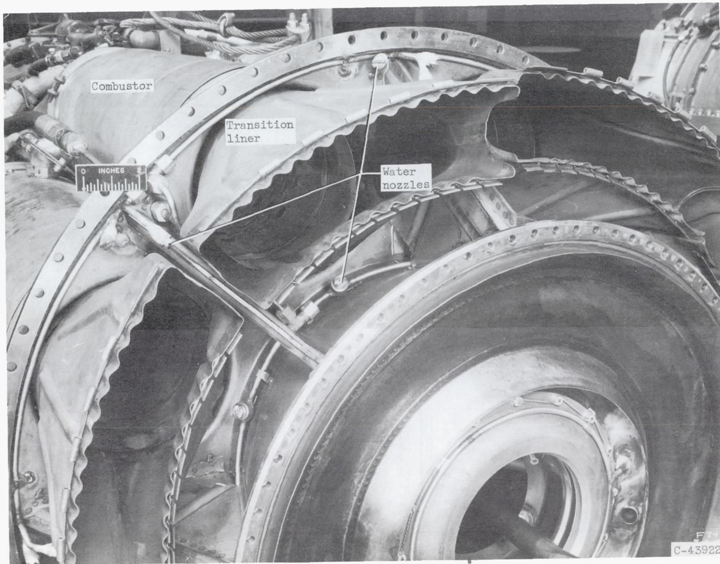
Figure 16. - Transition-liner water spray system (J35 and J47 engines).
