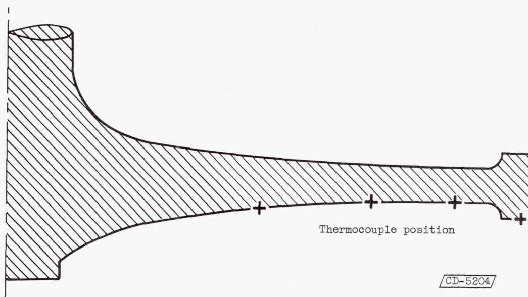
Figure 28. - Maximum temperatures recorded on J47-engine turbine wheel.
