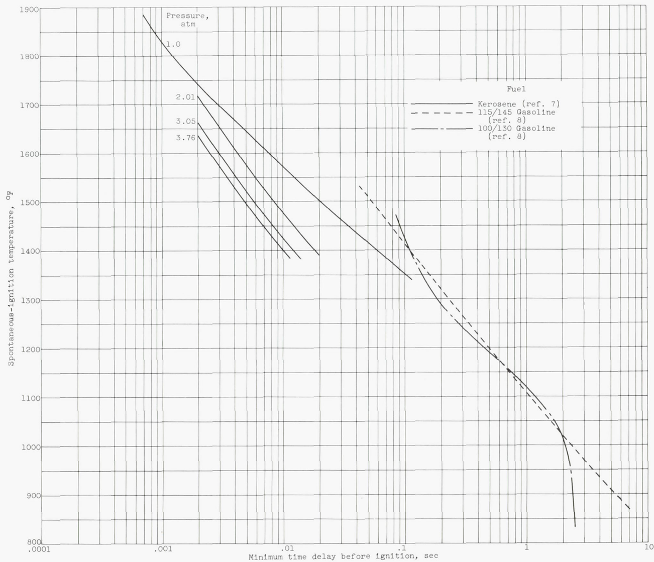
Figure 8. - Concluded. Ignition characteristics of aviation fuels.
