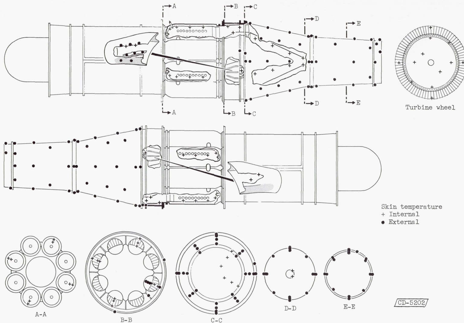
Figure 6. - Thermocouple locations on J47 engine.
