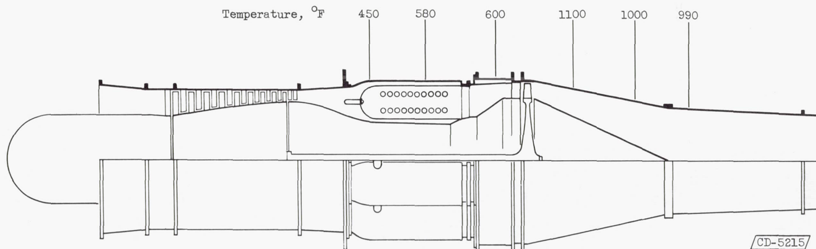
Figure 32. - Maximum external skin temperatures on J47 engine.
