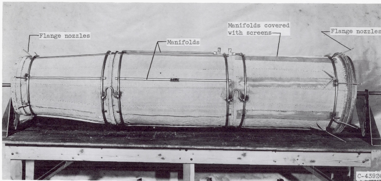
Figure 19. - Typical water distribution system for F-84 tailpipe or tailcone.
