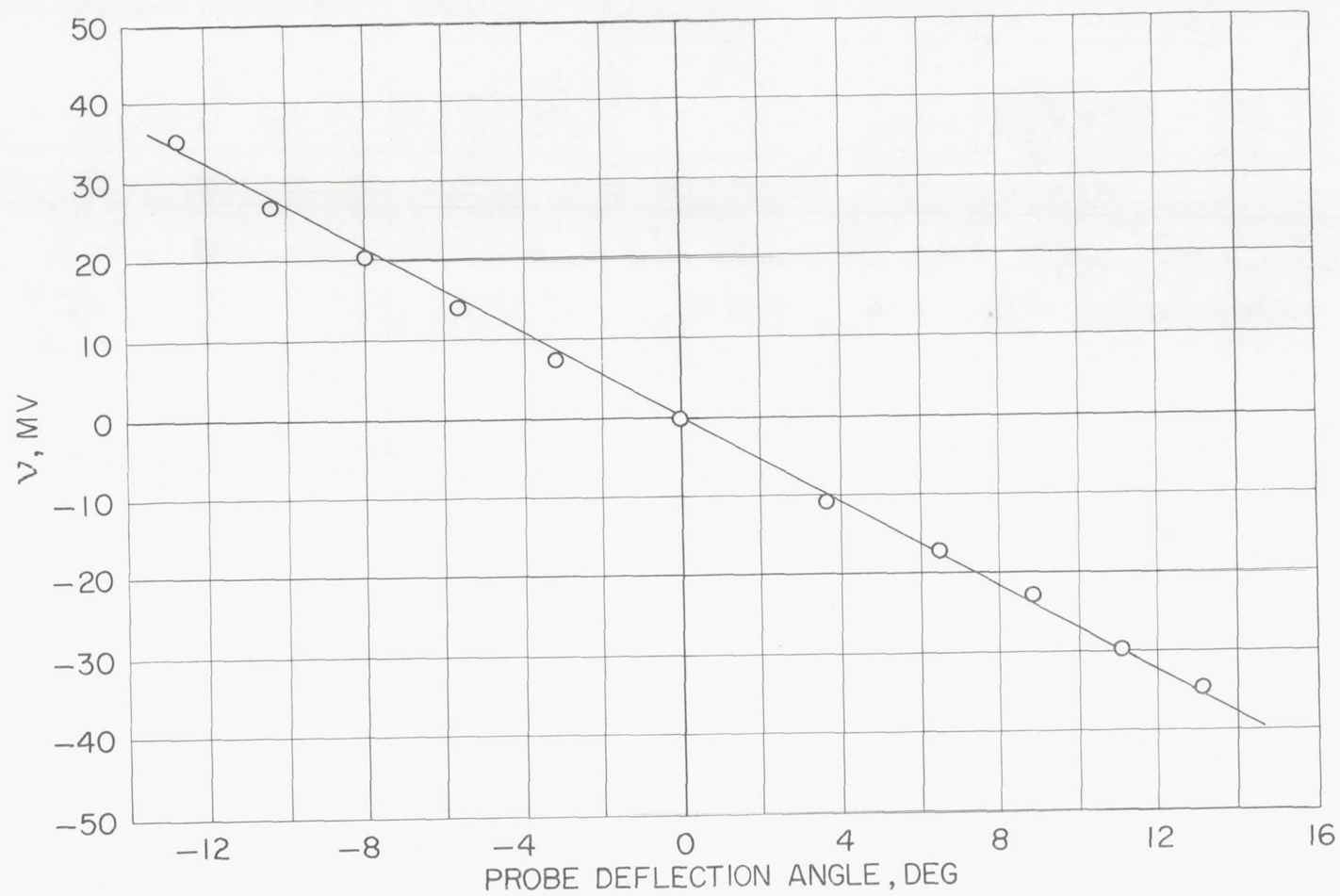
Figure 5.- Typical cross-velocity calibration of double-wire probe. Sensitivity, 2.66 \frac{\text{mv}}{\text{deg}} .
