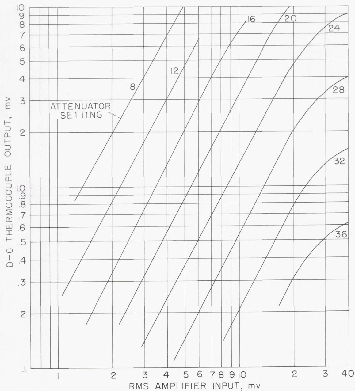
Figure 14.- Thermocouple calibration.
