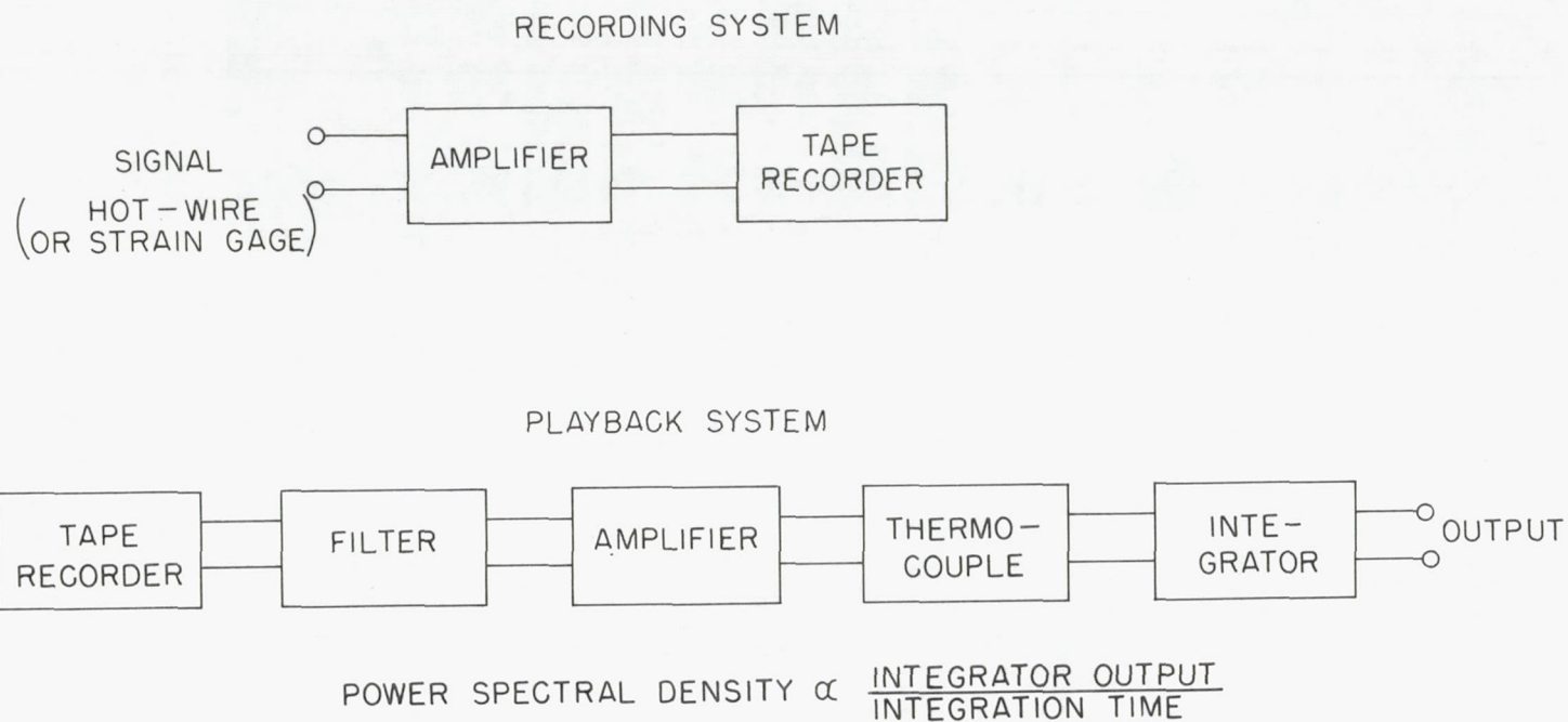
Figure 23.- System diagram for power-spectrum measurements.
