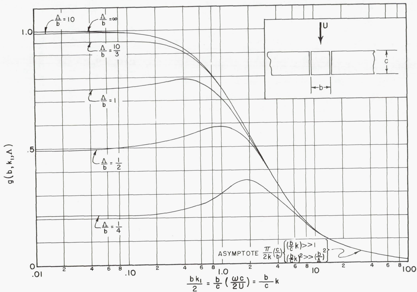
Figure 27.- Finite-span correction.
