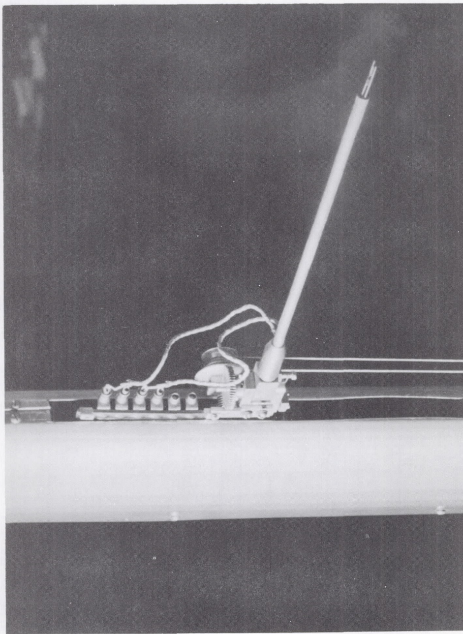
Figure 2.- Hot-wire probe.
