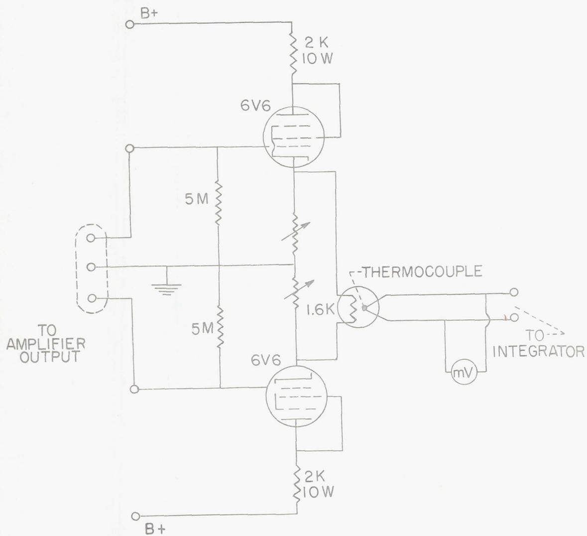
Figure 13.- Circuit for thermocouple driver.
