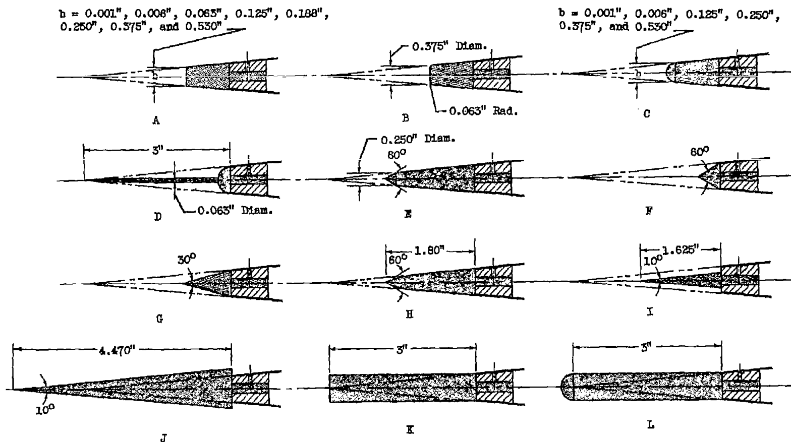
Figure 2. - Tip configurations used in investigation.
