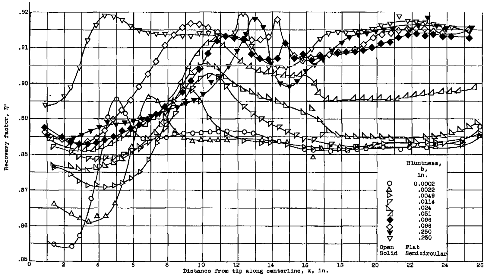
Figure 8. - Effect of cylinder bluntness on recovery-factor distribution and transition position; u_\infty/v_\infty = 3.5 \times 10^5 per inch.
