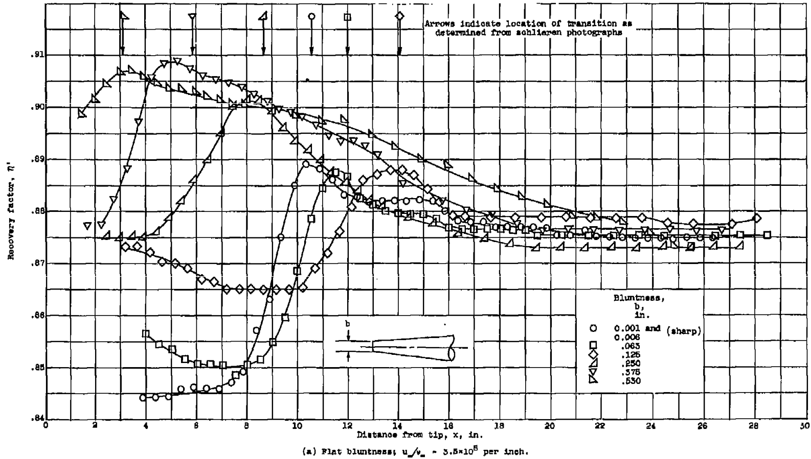
Figure 4. - Effect of cone bluntness on recovery-factor distribution and transition position.
