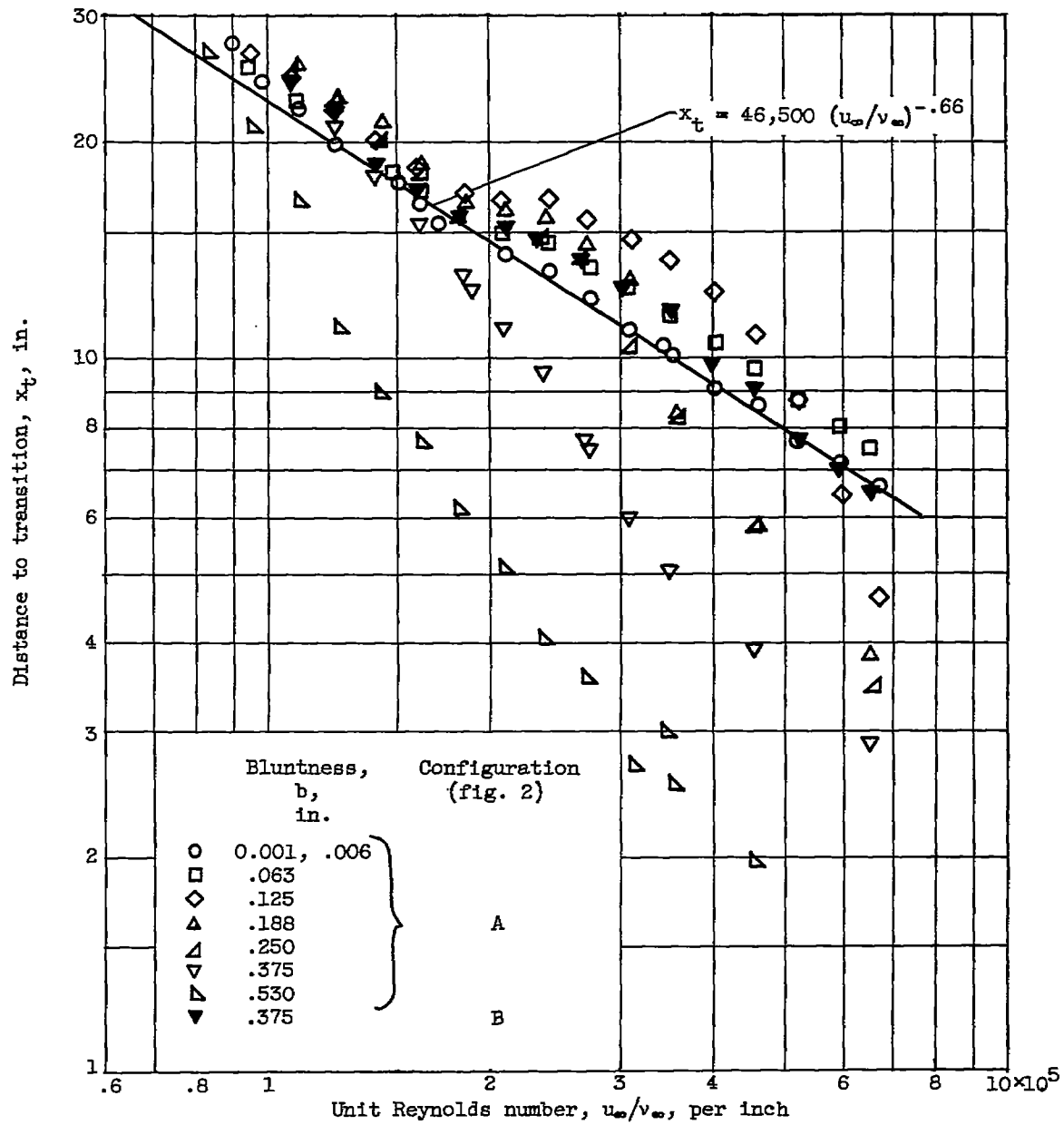
(a) Flat bluntness, configurations A and B.
