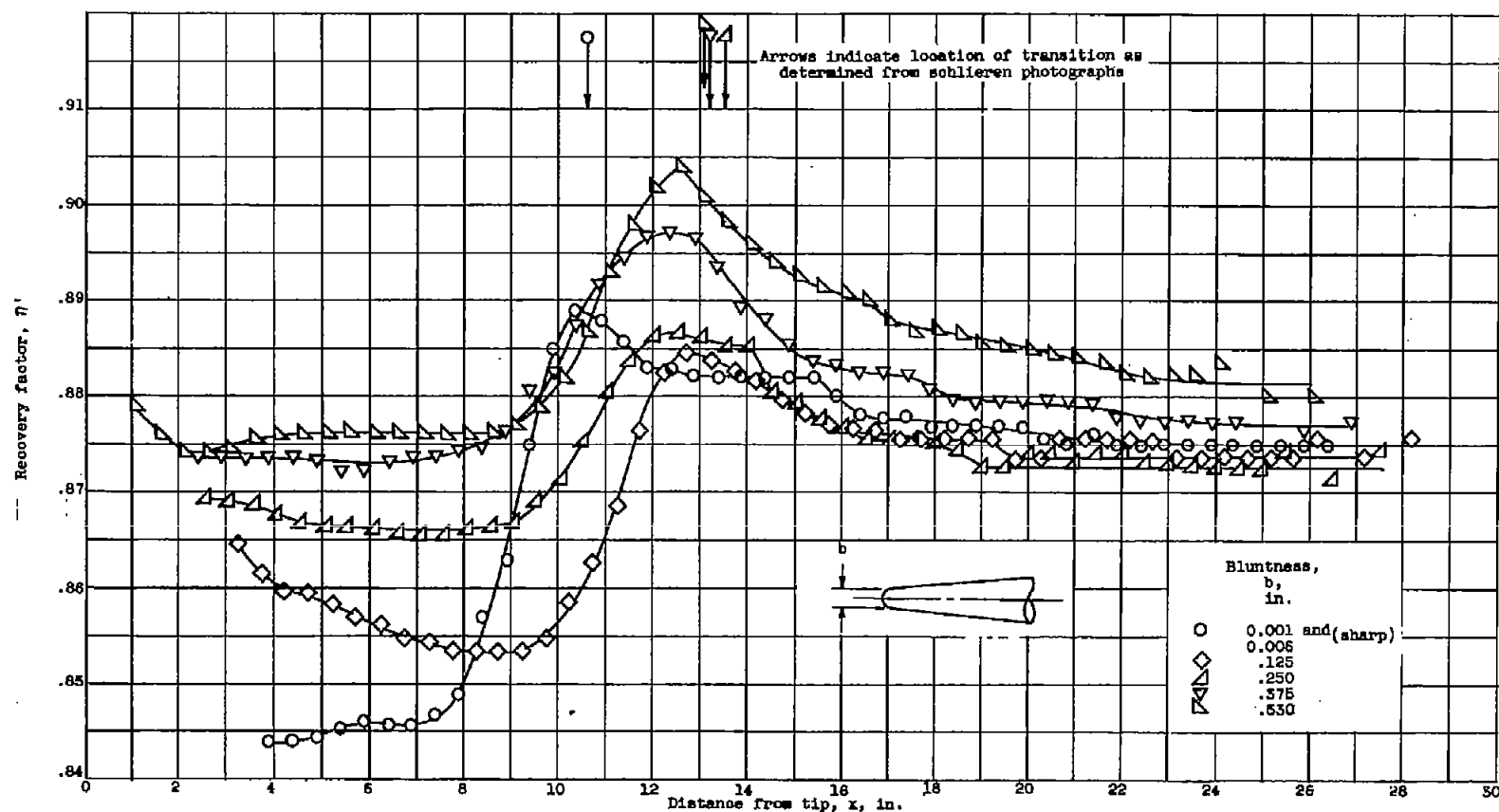
Figure 4. - Concluded. Effect of cone bluntness on recovery-factor distribution and transition position.
