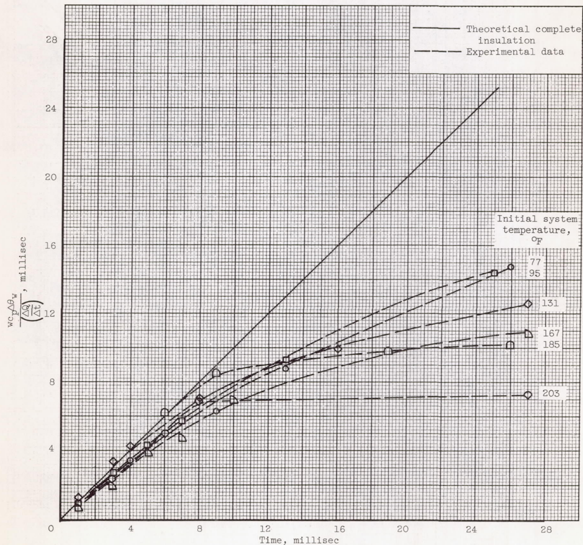
Figure 5. - Deviation of experimental data from that obtainable for complete insulation.
