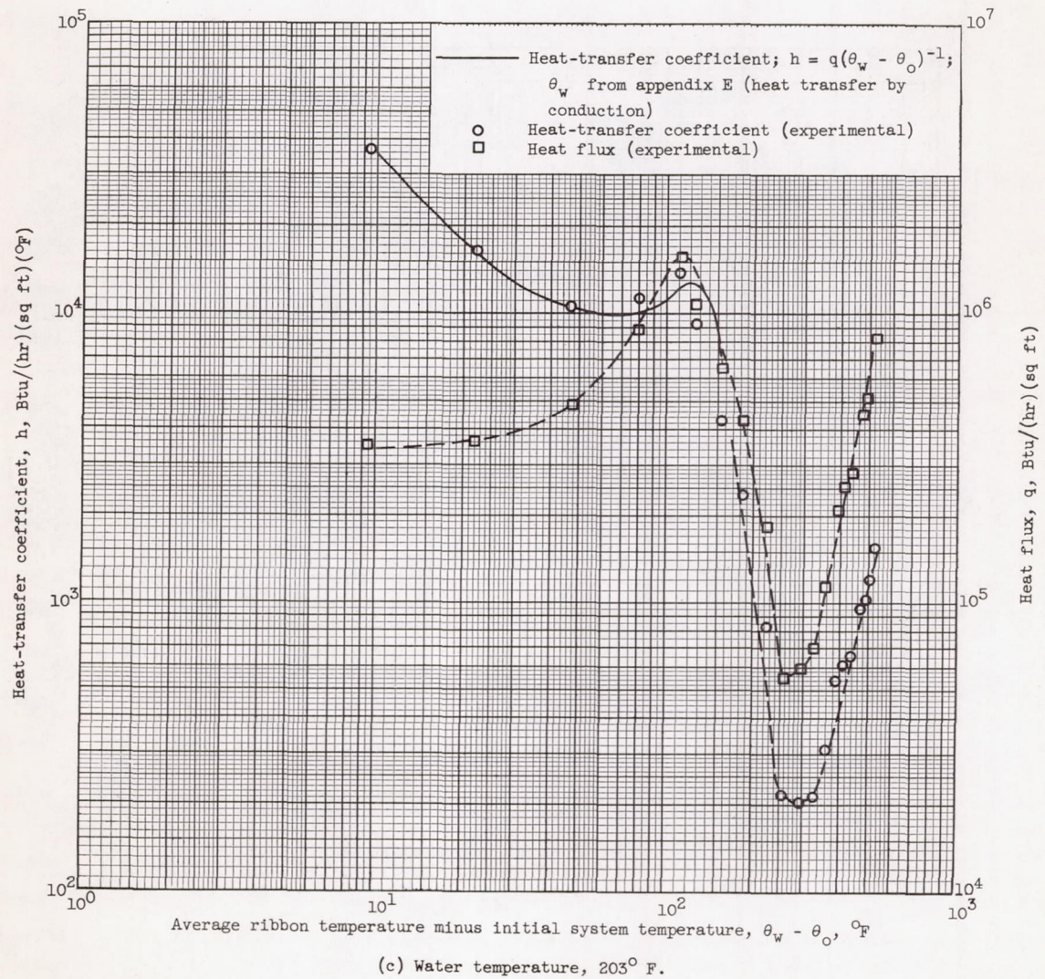
Figure 9. - Concluded. Heat flux and coefficient of heat transfer against average temperature difference.
