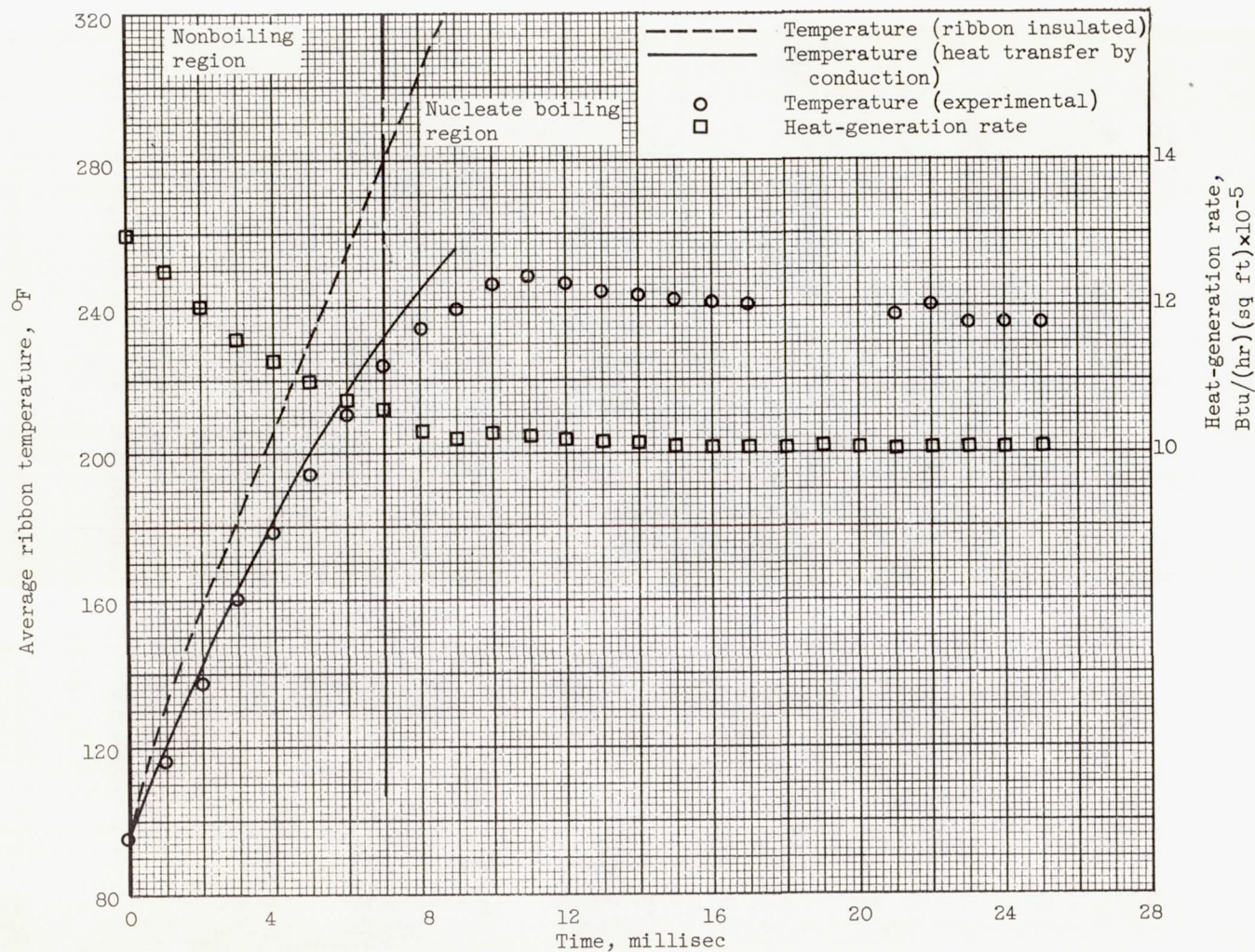
Figure 7. - Continued. Temperature - heat-generation-rate - time record for nickel ribbon in subcooled water.
