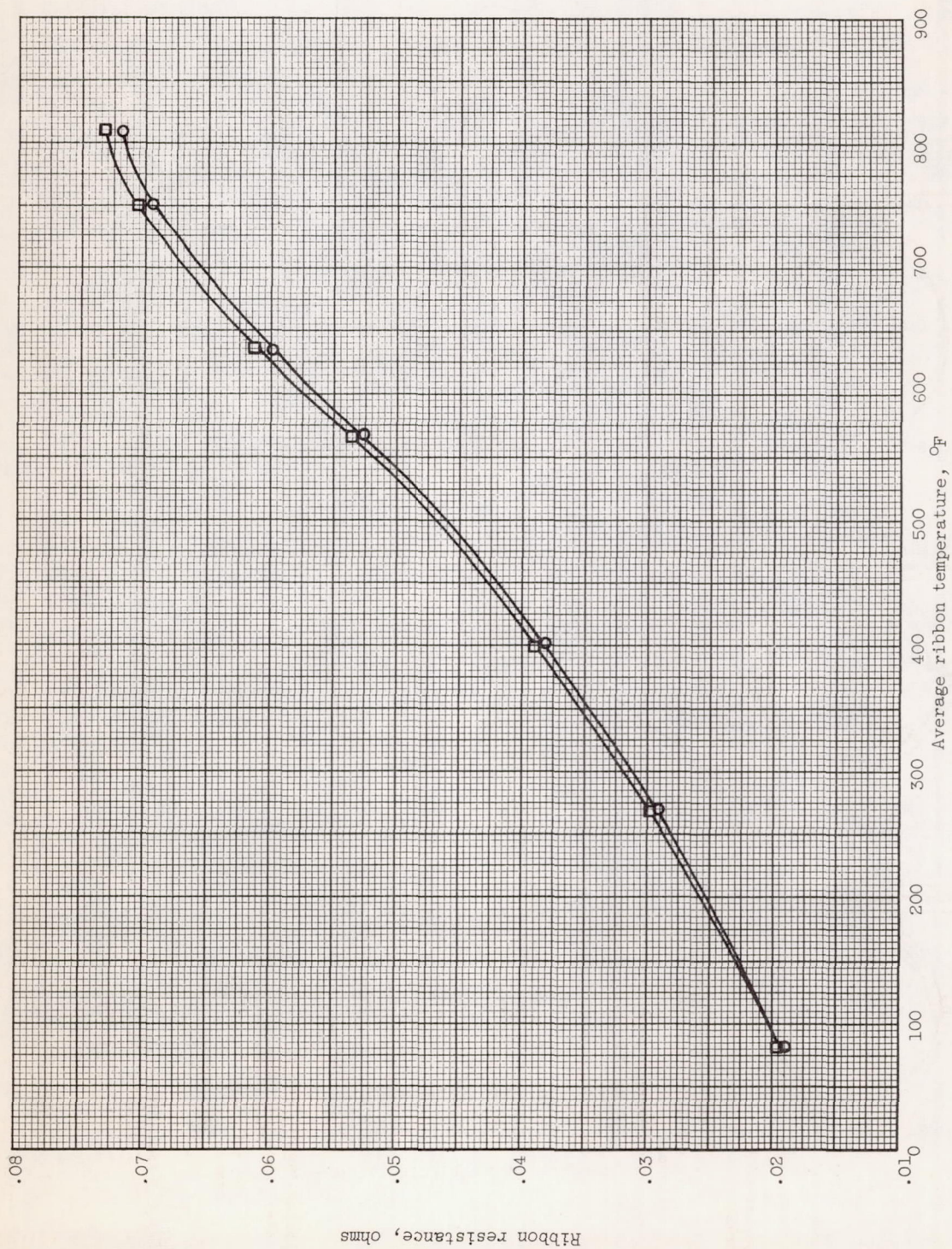
Figure 3. - Resistance-temperature calibration curves for two nickel ribbons.
