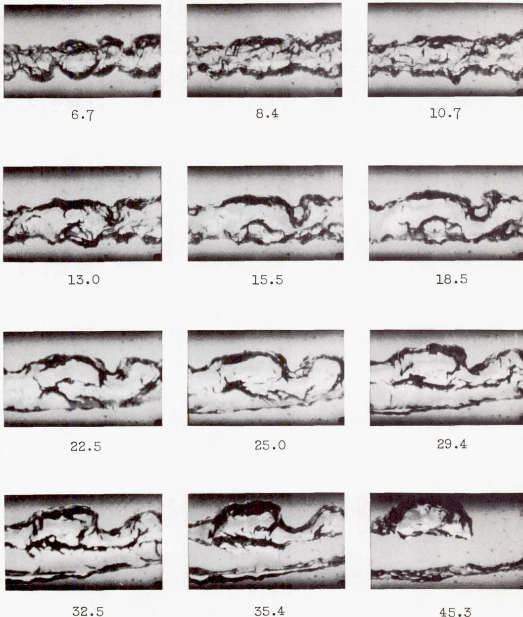
Figure 11. - Concluded. Transient bubble formation resulting from sudden large power surge. Water temperature, 203° F.
