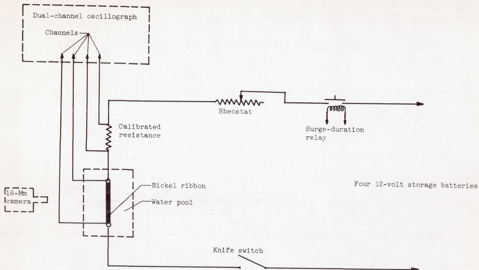
Figure 1. - Schematic diagram of main circuit.
