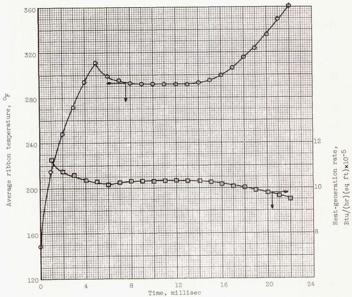
Figure 10. - Temperature - time - heat-generation-rate - time record for nickel ribbon in subcooled water. Initial water temperature, 149° F.
