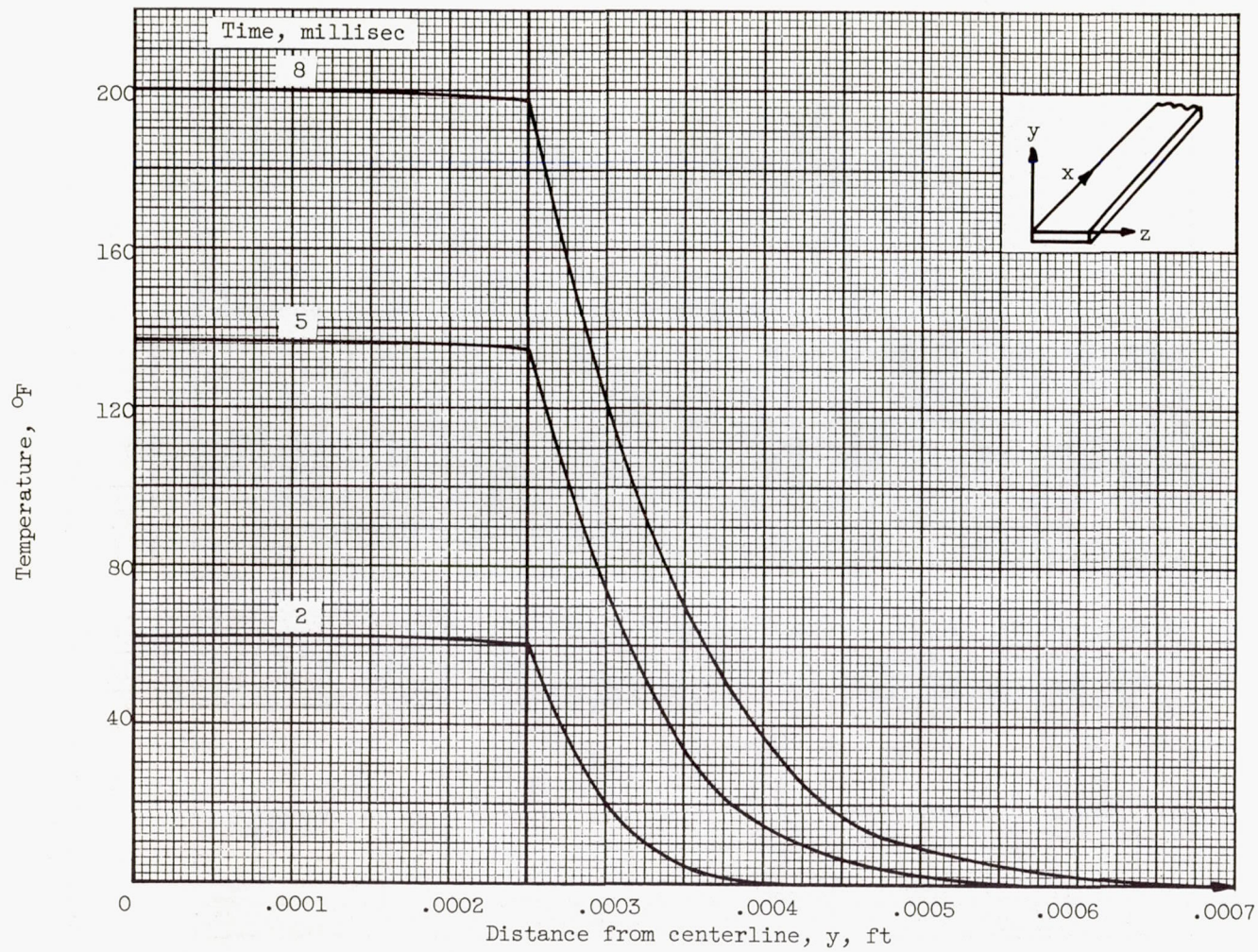
Figure 6. - Temperature gradient along y-axis for heat generation rate \frac{d(Q)}{dt} of (-5 \times 10^{14})t + 8 \times 10^9 Btu per hour per cubic foot. (See appendix B.)
