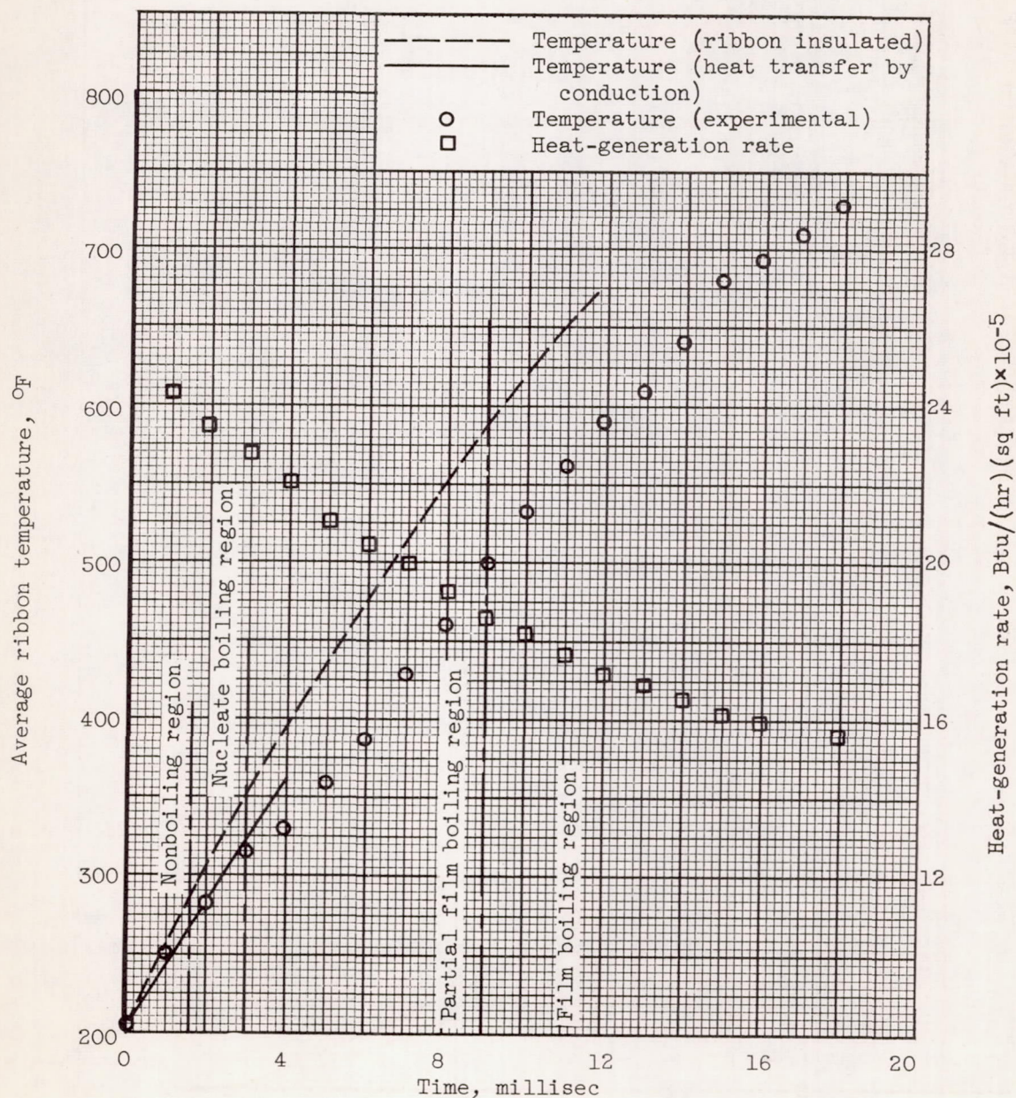
Figure 7. - Concluded. Temperature - heat-generation-rate - time record for nickel ribbon in subcooled water.
