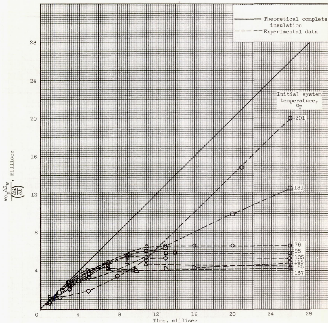
Figure 5. - Continued. Deviation of experimental data from that obtainable for complete insulation.
