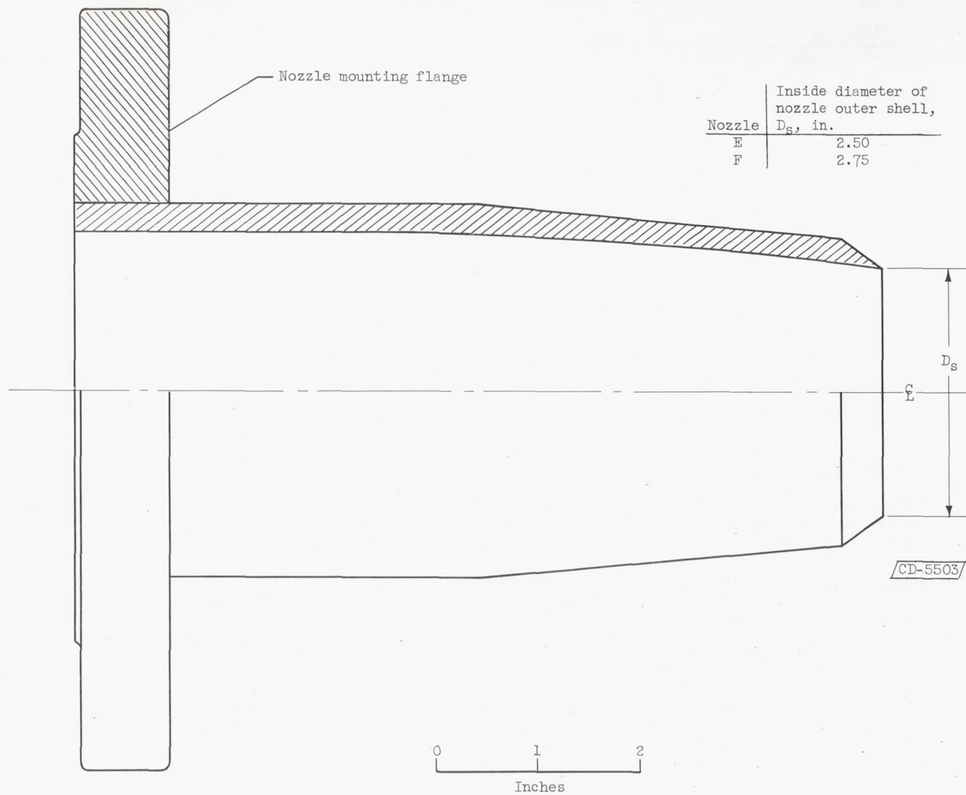
Figure 5. - Cross section of typical circular nozzle.
