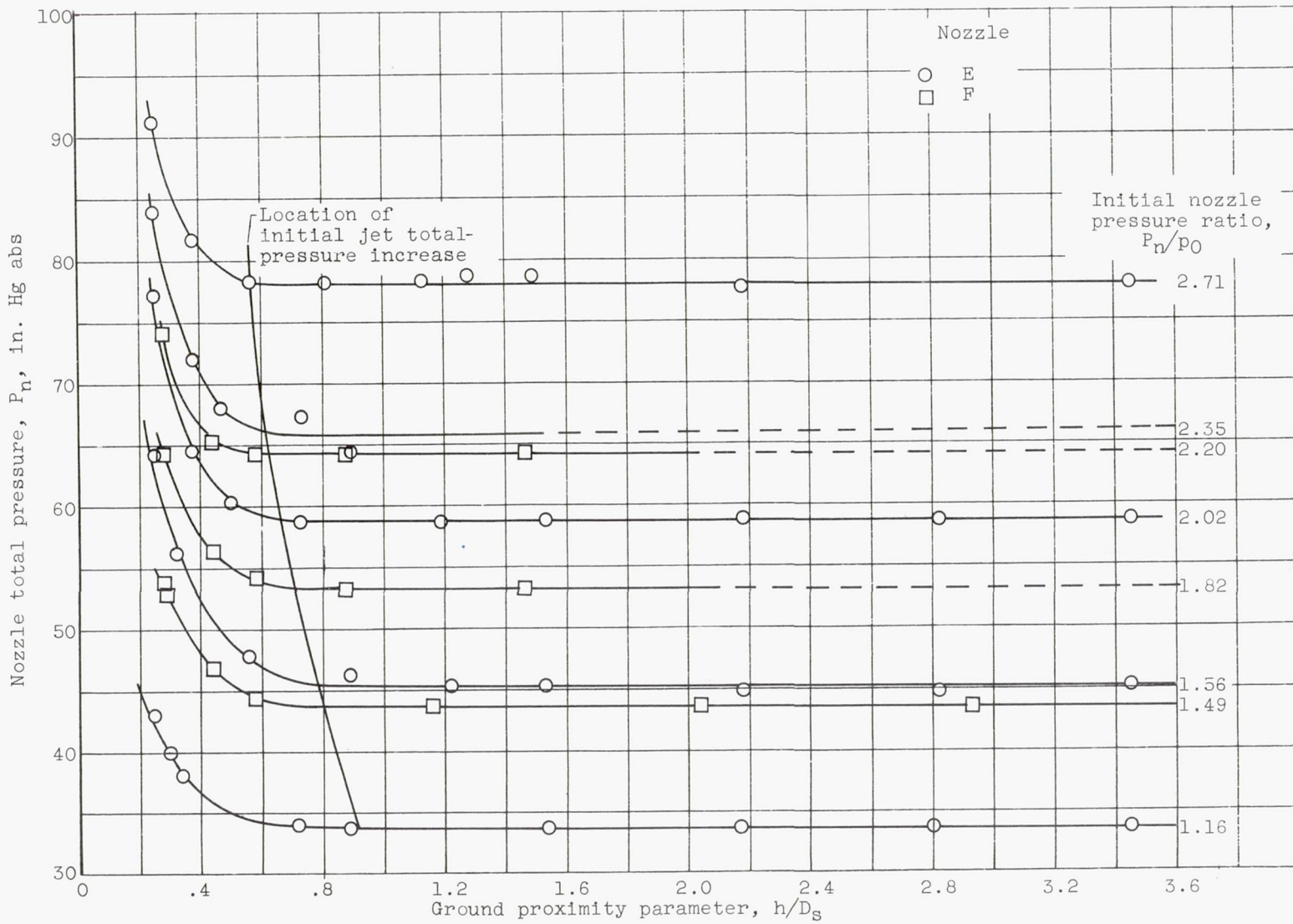
Figure 21. - Effect of ground proximity on jet total pressure for circular nozzle.
