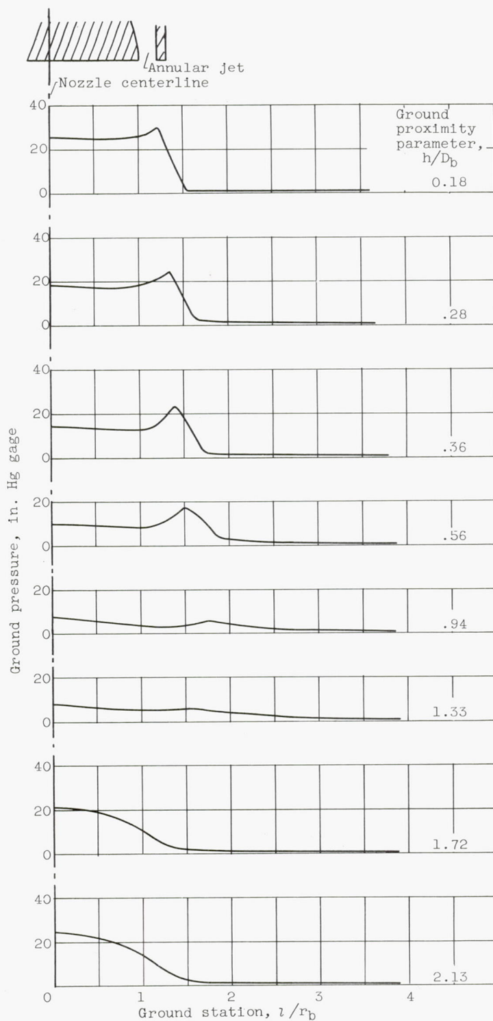
(b) Nozzle pressure ratio, 2.1.
