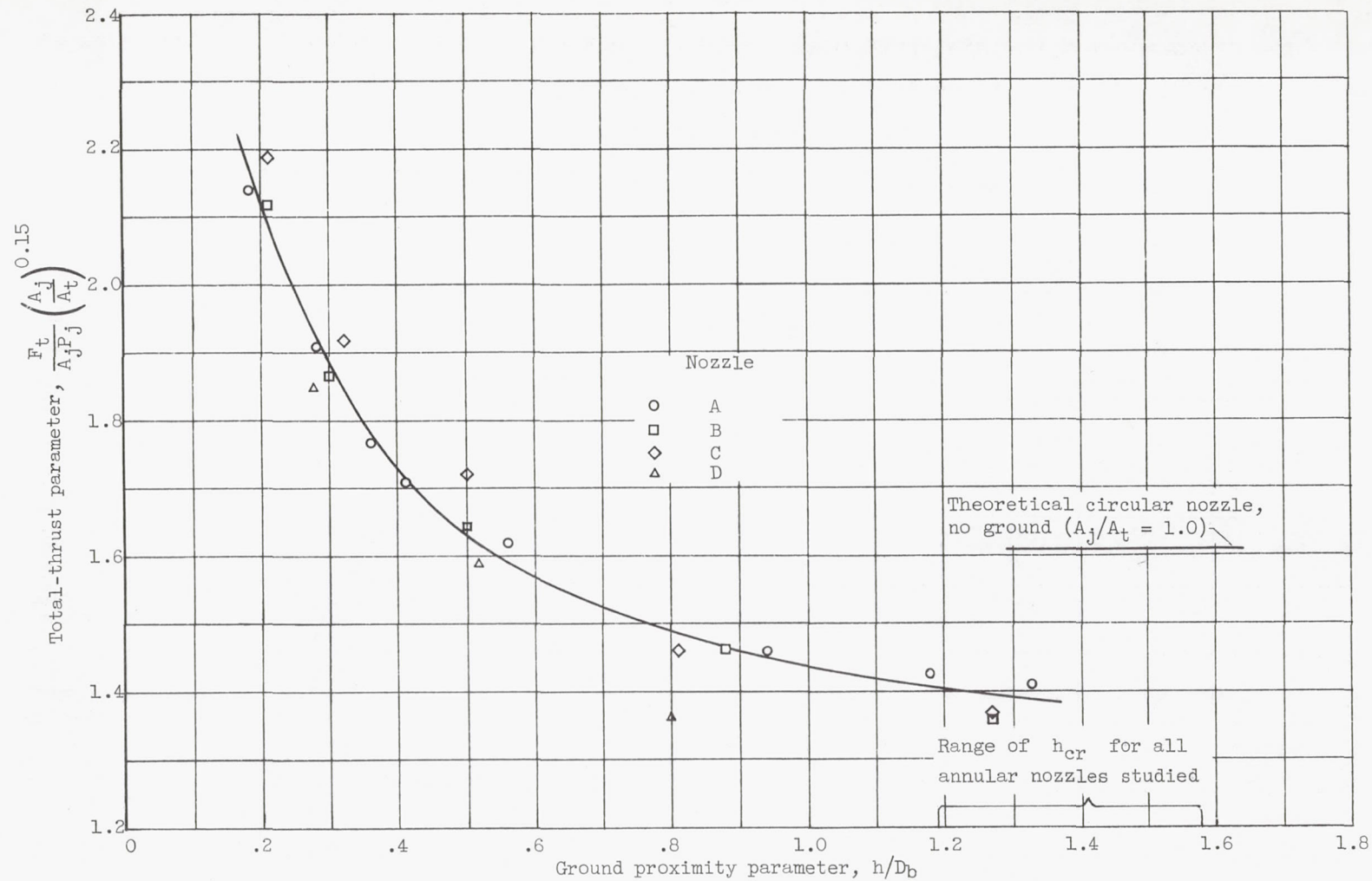
(b) Nominal nozzle pressure ratio, 1.8.
