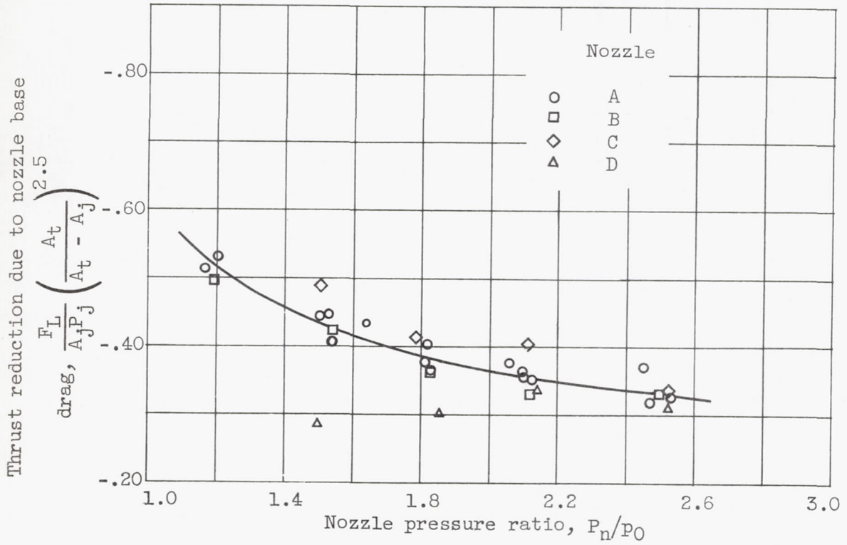
Figure 11. - Effect of nozzle pressure ratio on thrust loss for annular nozzle without ground effect.
