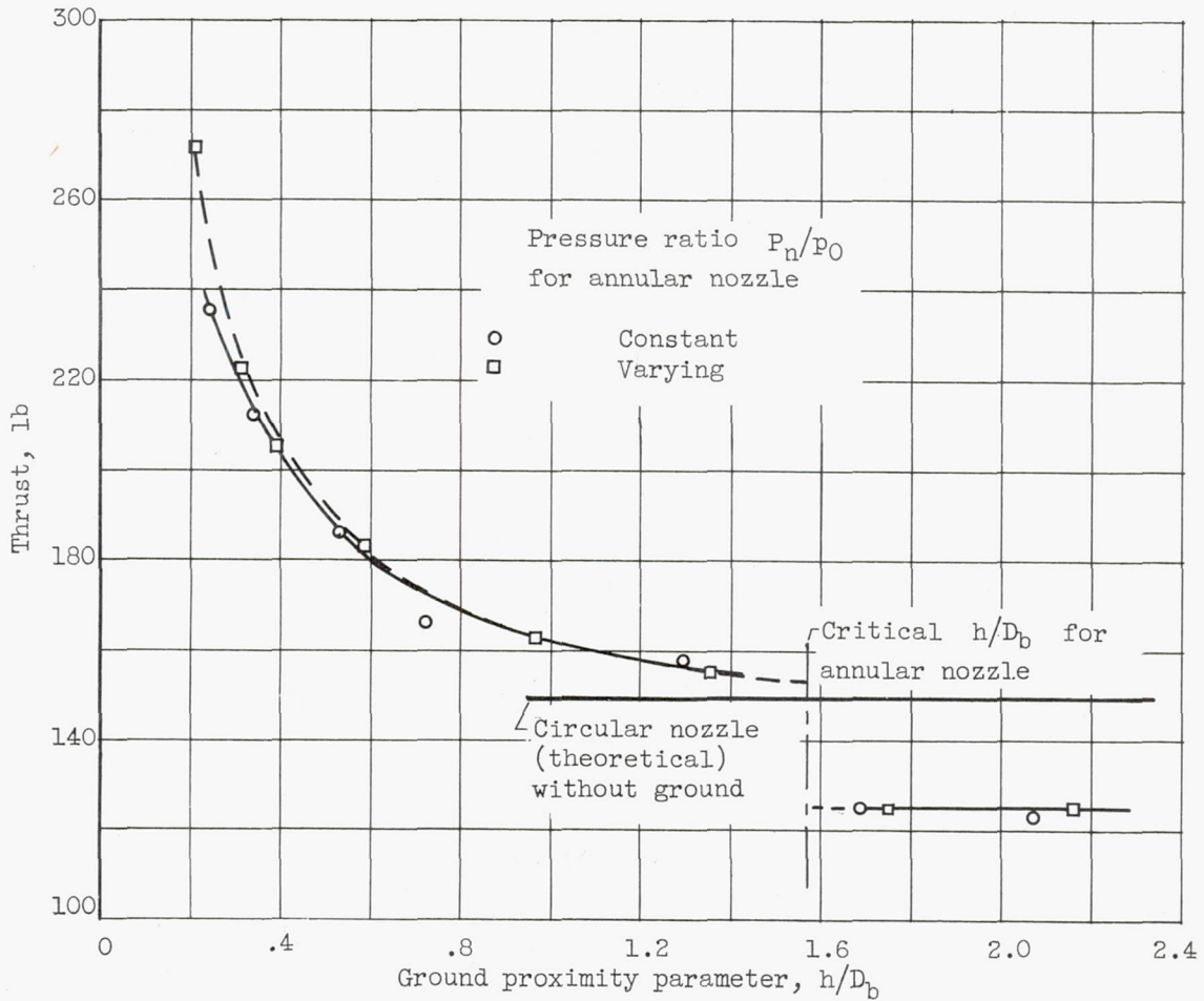
Figure 6. - Typical thrust augmentation obtainable with annular nozzle as function of nozzle-to-ground height. Nozzle configuration, A; initial nozzle pressure ratio, approximately 2.0; offset from shell to base plate \delta , 0.125 inch.
