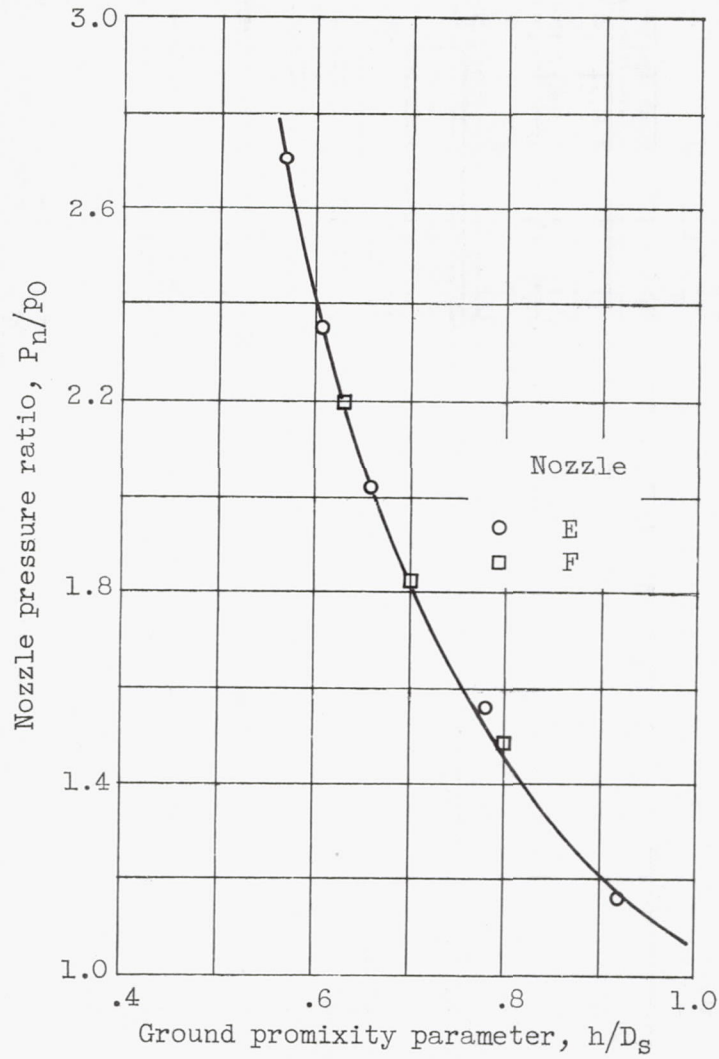
Figure 20. - Effect of nozzle pressure ratio on ground distance at which thrust losses occur with circular nozzle.
