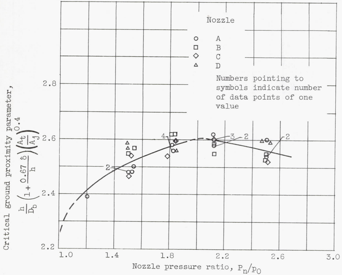
Figure 13. - Critical ground proximity parameter at which thrust augmentation begins as function of nozzle pressure ratio.
