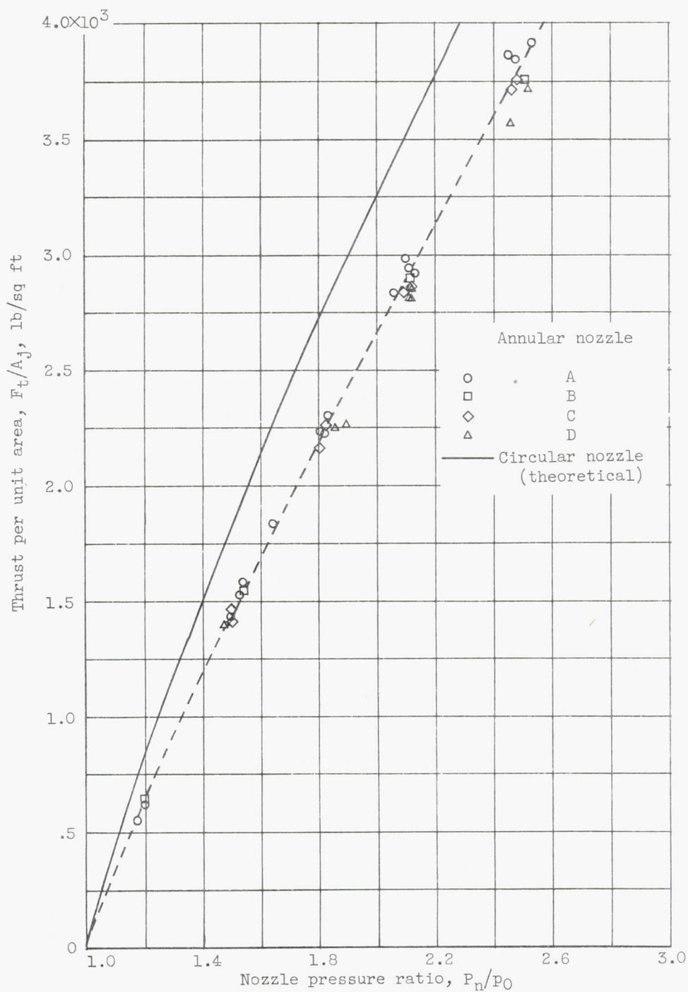
(a) F_t/A_j against P_n/P_0 .
