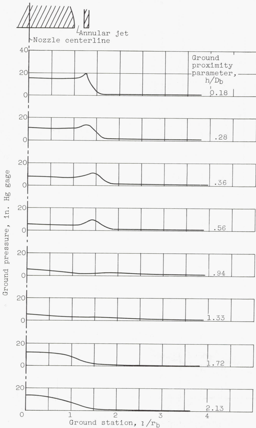
(a) Nozzle pressure ratio, 1.8.
