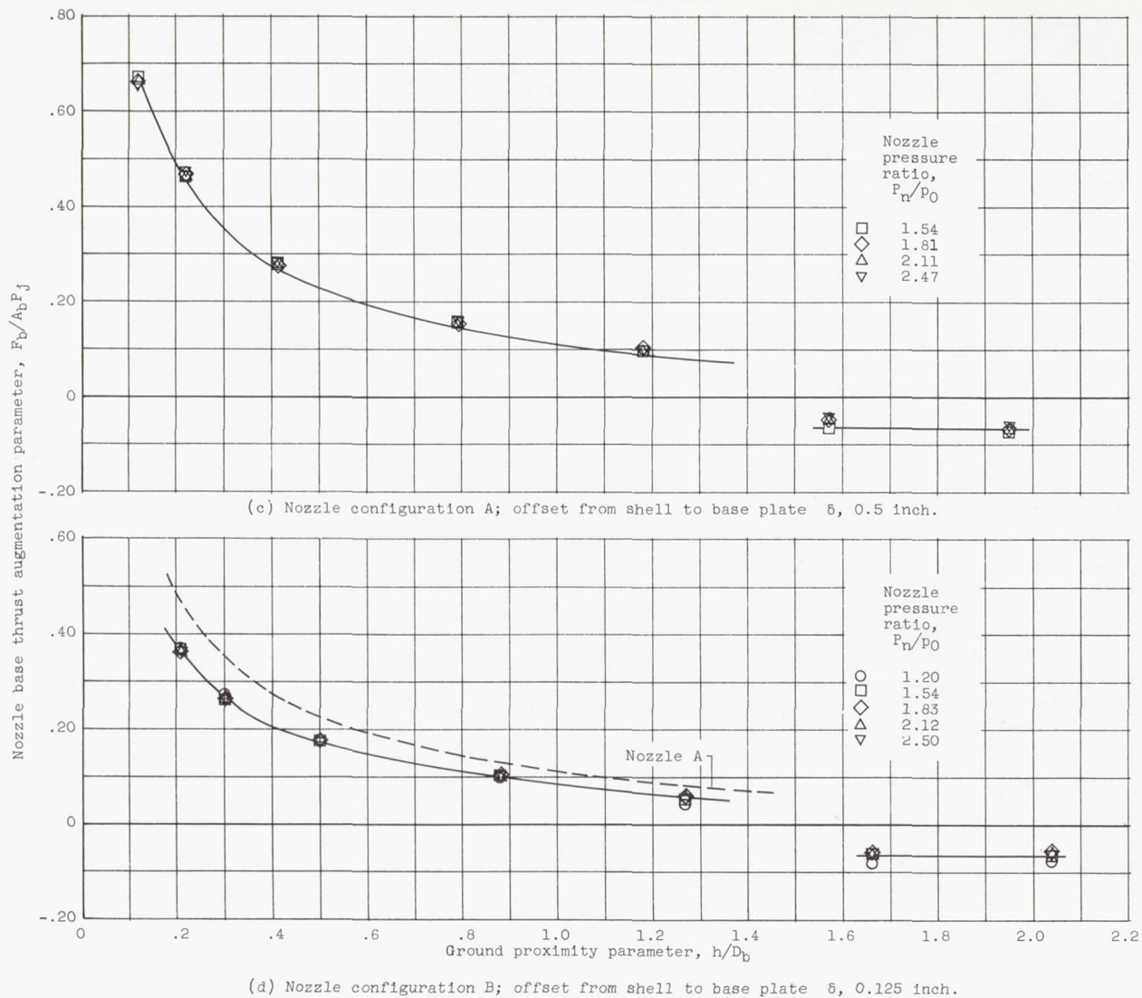
Figure 8. - Continued. Variation of thrust parameter determined from pressure integration over nozzle base with ground proximity parameter.
