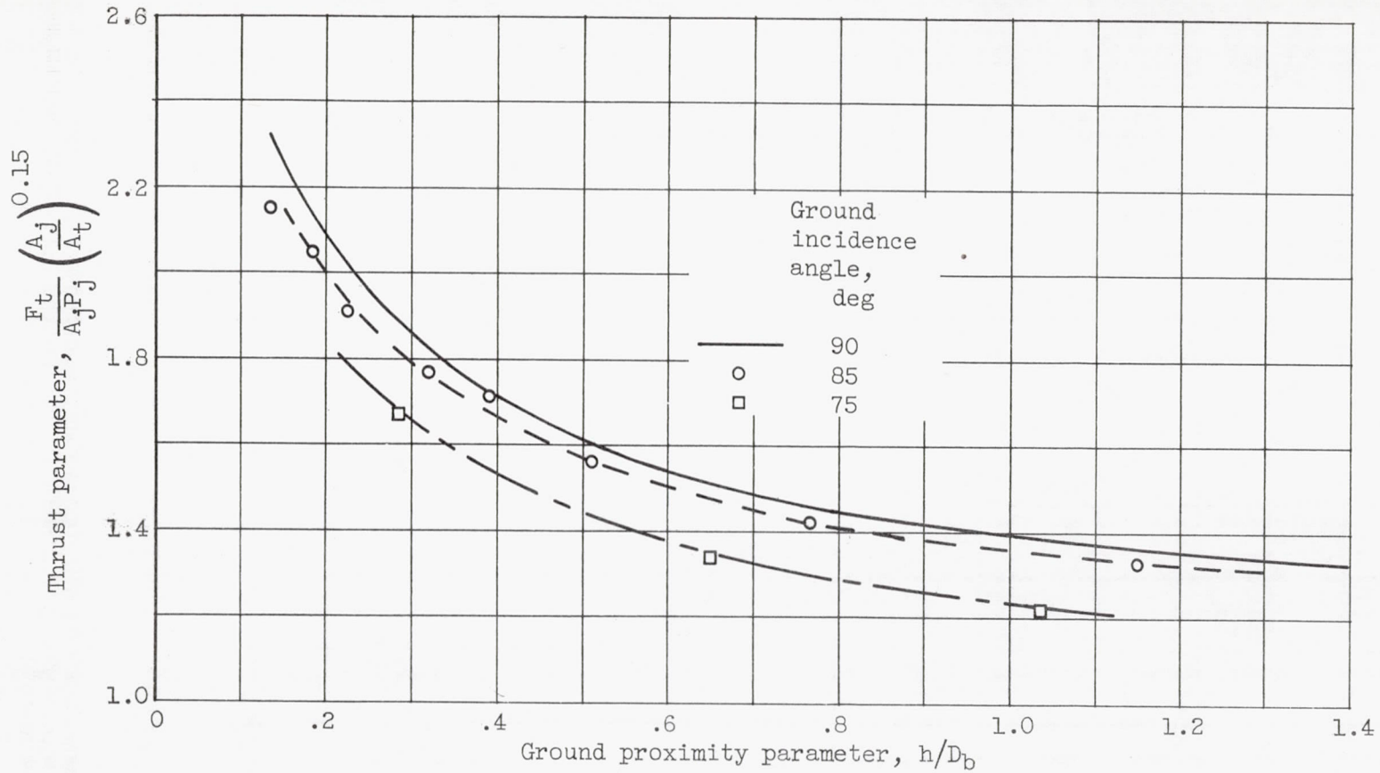
Figure 17. - Effect of ground incidence angle on thrust of annular nozzle. Nozzle configuration A; nozzle pressure ratio, 2.1.
