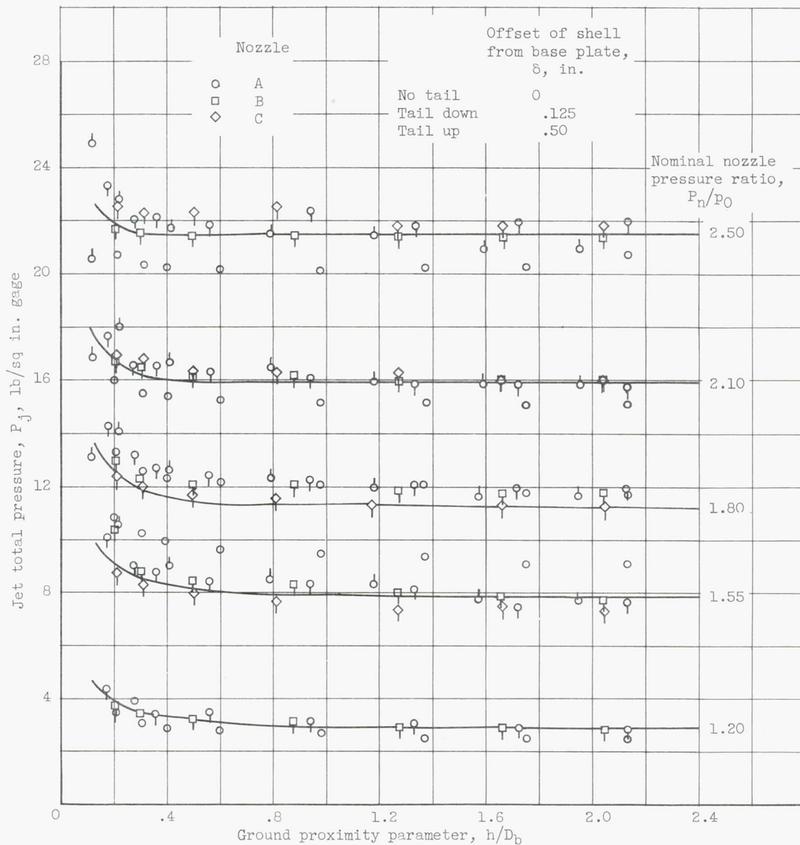
(a) Typical variation of P_j with ground proximity parameter for various pressure ratios.
