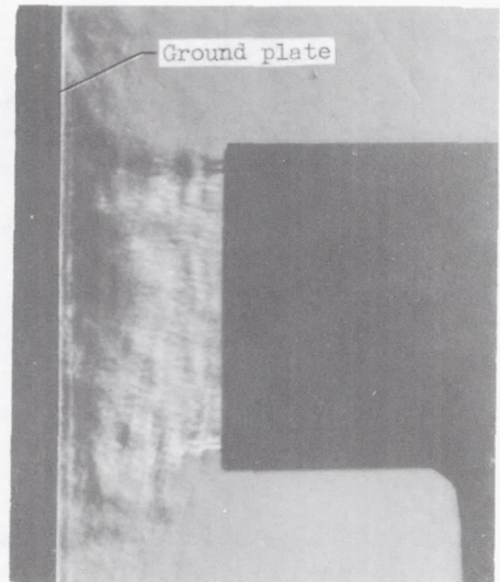
(c) With ground; thrust augmented.
