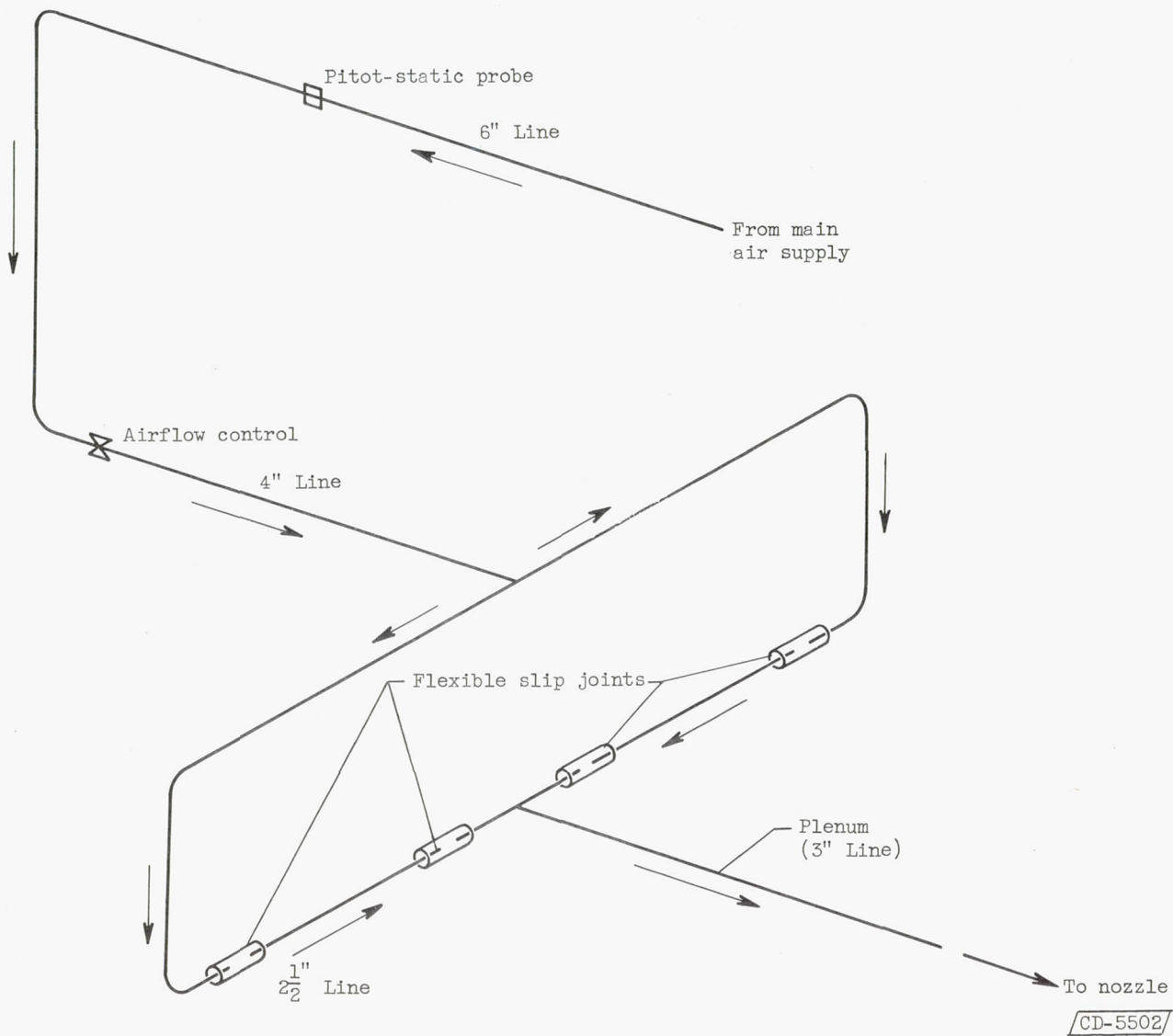
Figure 2. - Schematic diagram of airflow in supply system.
