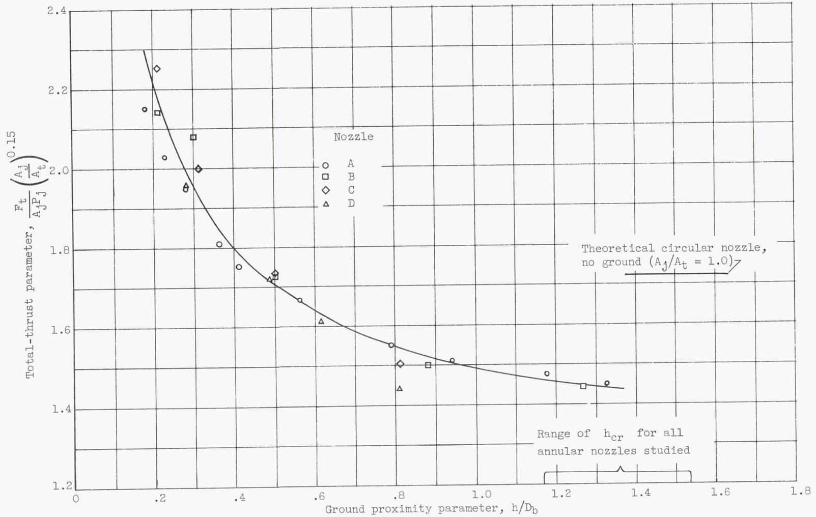
(a) Nominal nozzle pressure ratio, 1.5.
