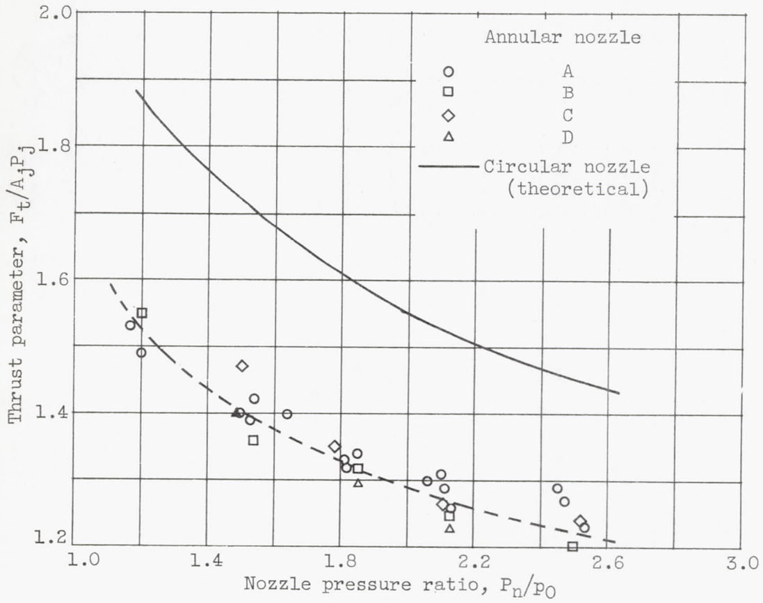
(b) F_t/A_j P_j against P_n/p_0 .
