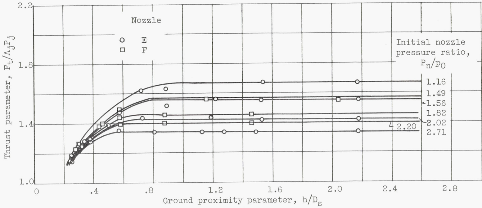
Figure 19. - Effect of ground proximity on thrust of circular nozzle.
