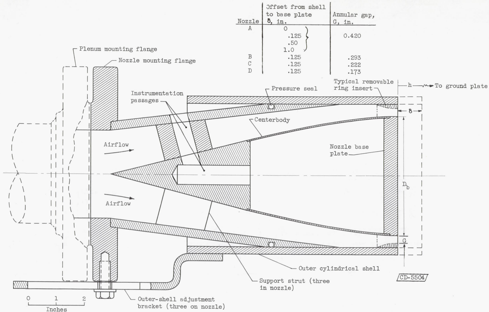
Figure 3. - Sketch of typical annular nozzle.
