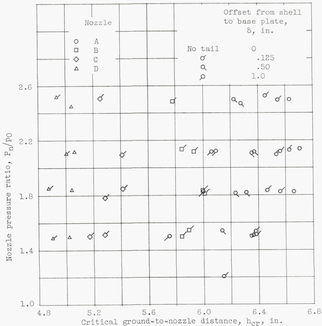
Figure 12. - Variation of critical ground-to-nozzle distance at which thrust augmentation begins with nozzle pressure ratio and nozzle configuration.
