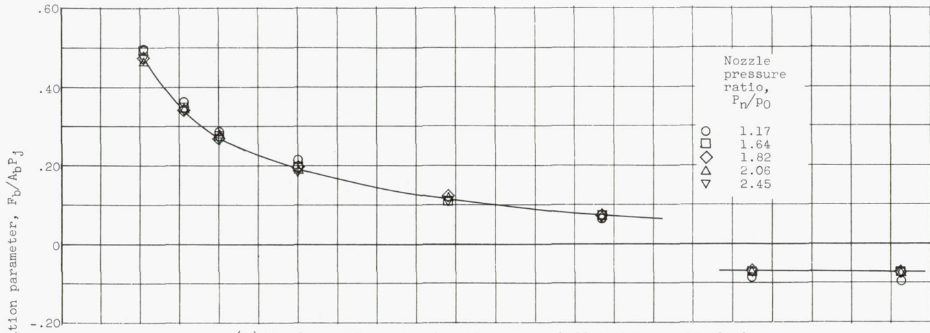
(a) Nozzle configuration A; offset from shell to base plate \delta , 0.
