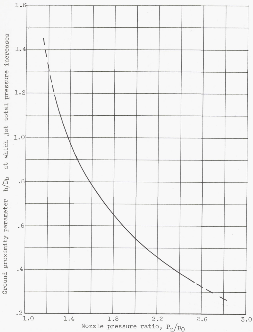
(b) Initial h/D_b values at which jet total pressure increases as function of nozzle pressure ratio for nozzles A, B, and C.
