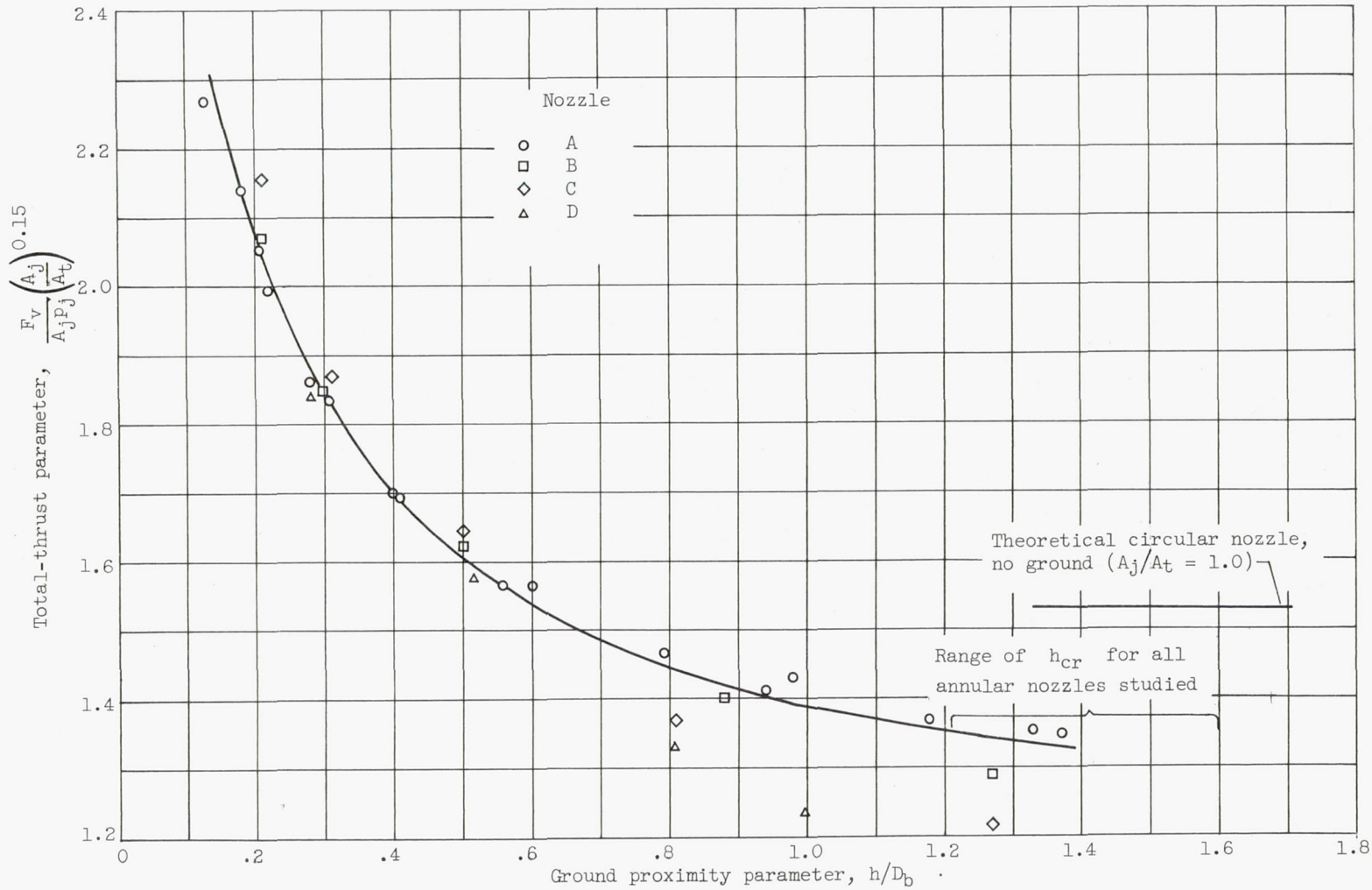
(c) Nominal nozzle pressure ratio, 2.1.
