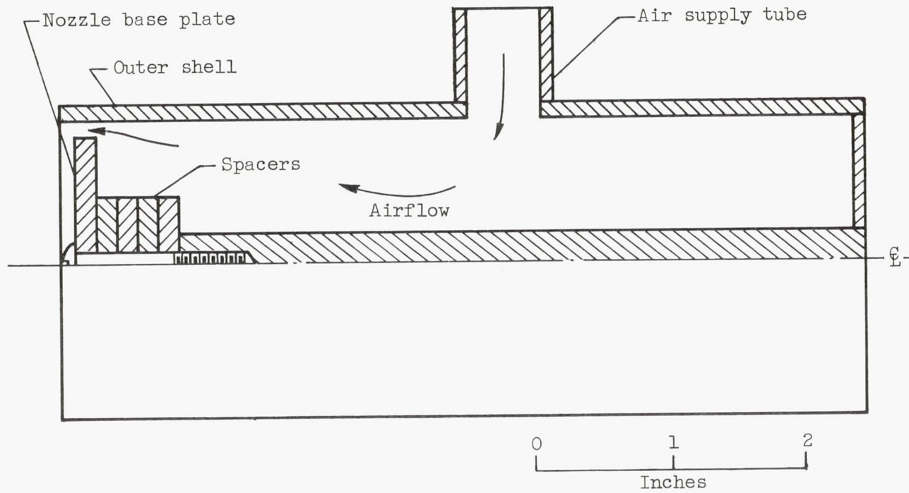
Figure 4. - Annular nozzle used to obtain schleiren photographs of jet shape in proximity of ground.
