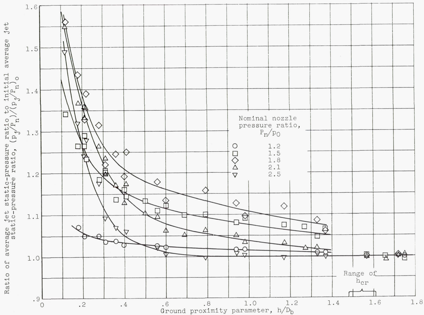
Figure 15. - Effect of ground proximity on jet static pressure. Nozzle A; offset of shell from base plate \delta , 0, 0.125, and 0.5 inch.
