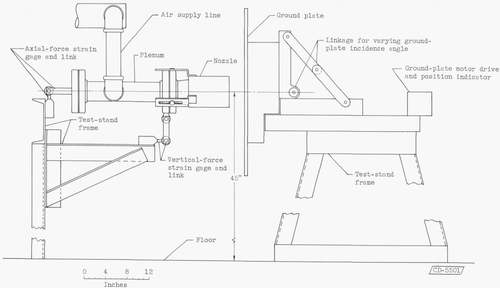
Figure 1. - Sketch of setup for annular nozzle and ground plate.
