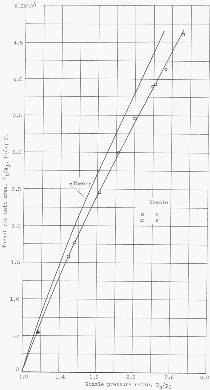
(a) F_t/A_j against P_n/P_0 .
