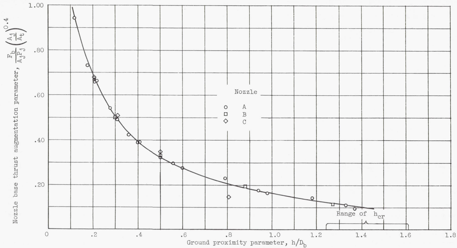
Figure 9. - Variation of thrust augmentation parameter \frac{F_b}{A_j P_j} \left( \frac{A_j}{A_t} \right)^{0.4} with ground proximity parameter. Annular nozzles.
