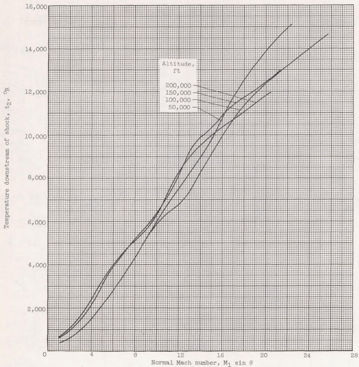
Figure 6. - Temperature downstream of shock wave.
