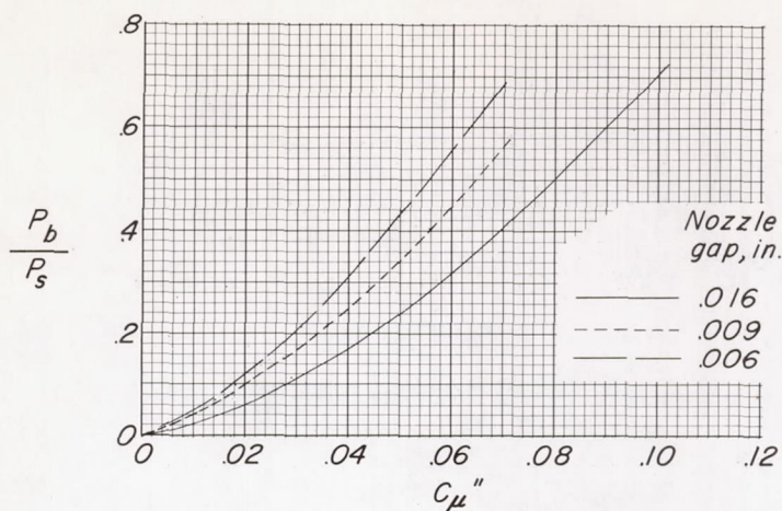
(a) Ratio of power in blowing system to power in slipstream.
