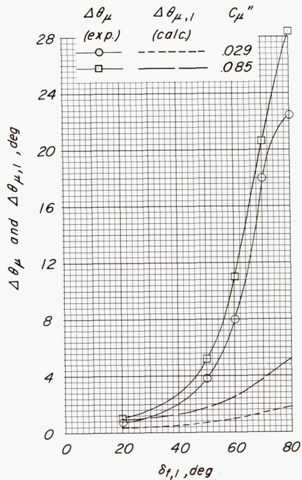
(b) Increment in turning angle.
