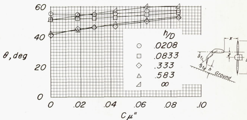
(c) Turning angle.
