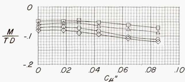
(a) Pitching moment.
