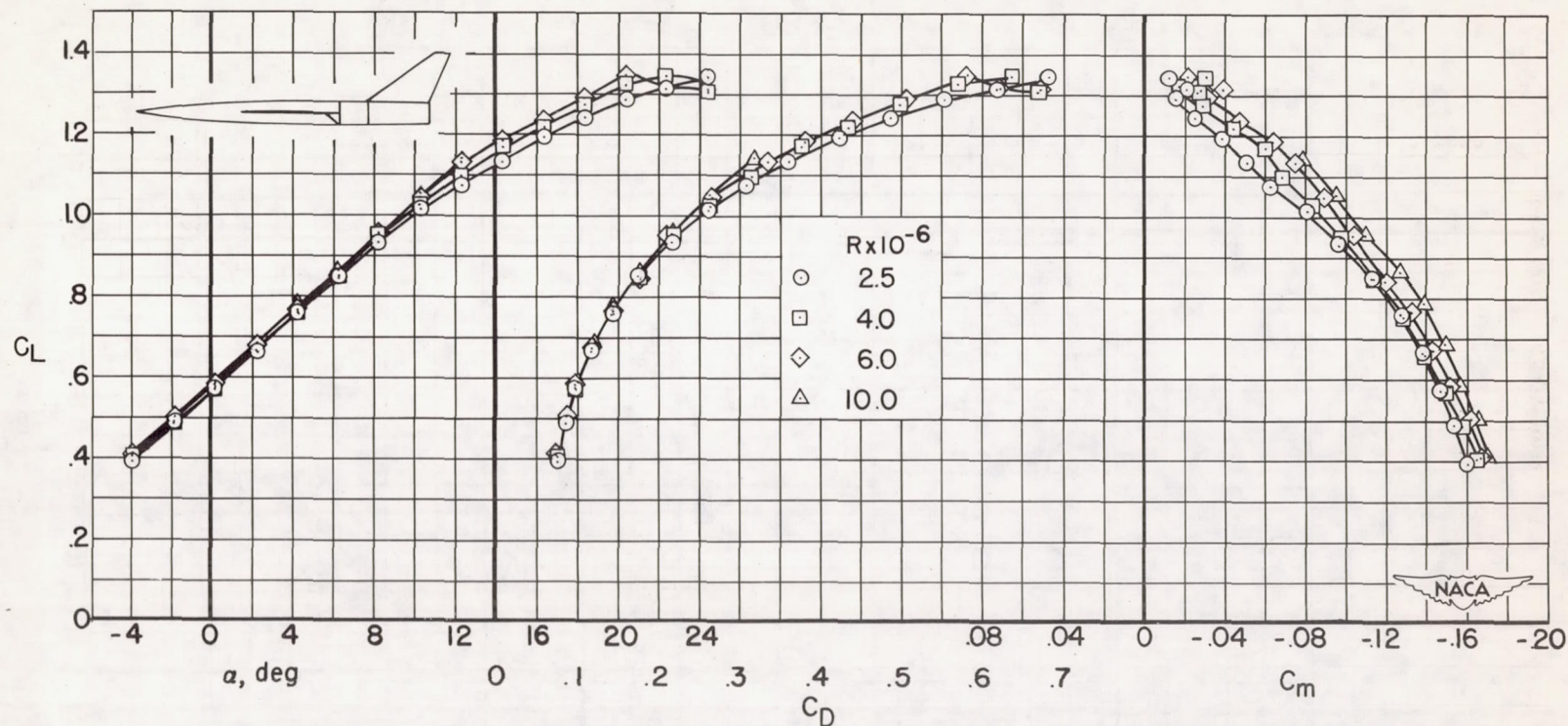
Figure 5.- The effect of Reynolds number on the aerodynamic characteristics of the wing-fuselage combination with the slotted flaps deflected 40^\circ ; mid wing; moment center at 0.415\bar{c} ; M = 0.25 .
