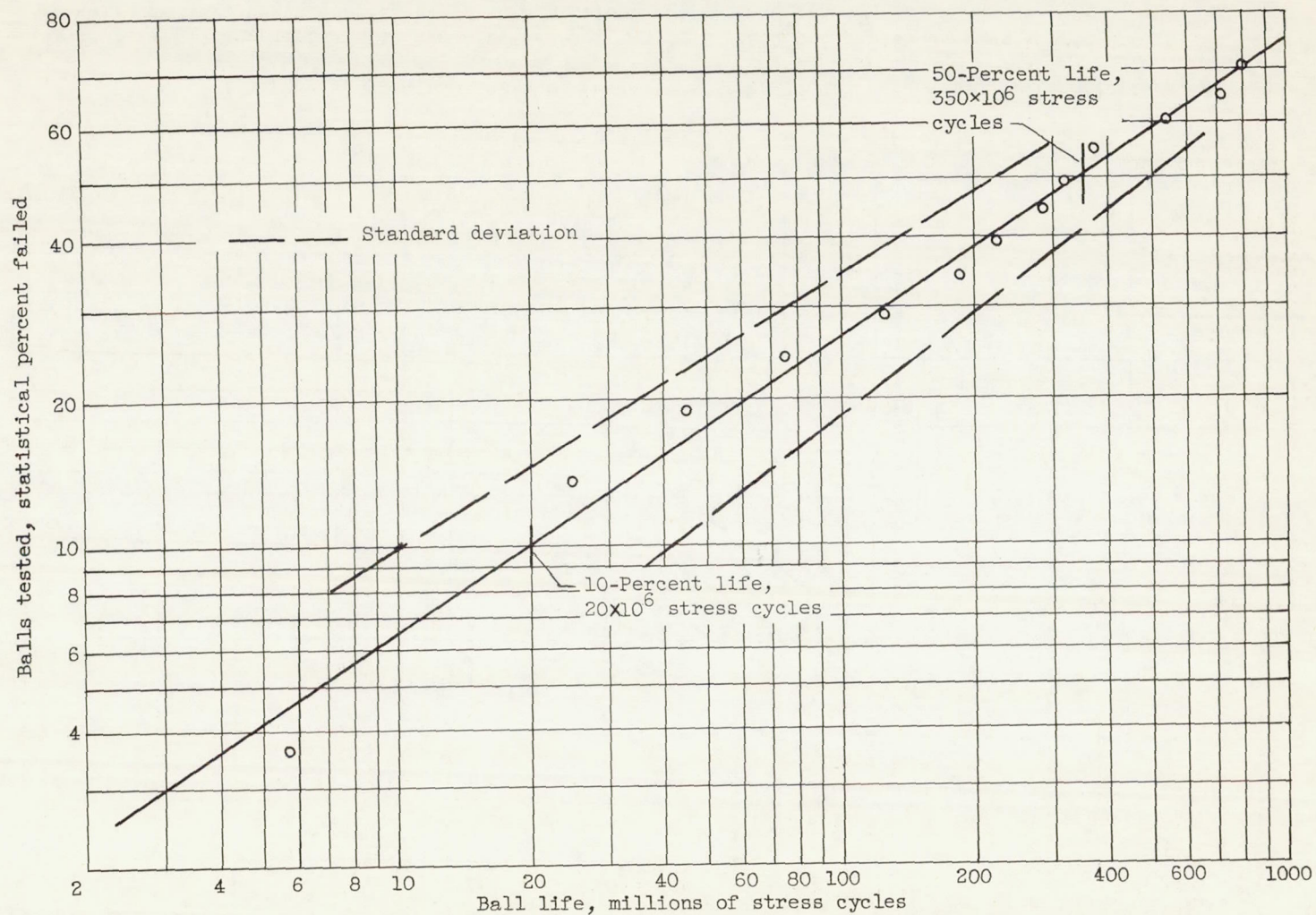
Figure 3. - Continued. Rolling-contact fatigue life of AISI M-1 tool-steel balls with various lubricants. Test temperature, 100° F; maximum Hertz compressive stress, 725,000 psi.
