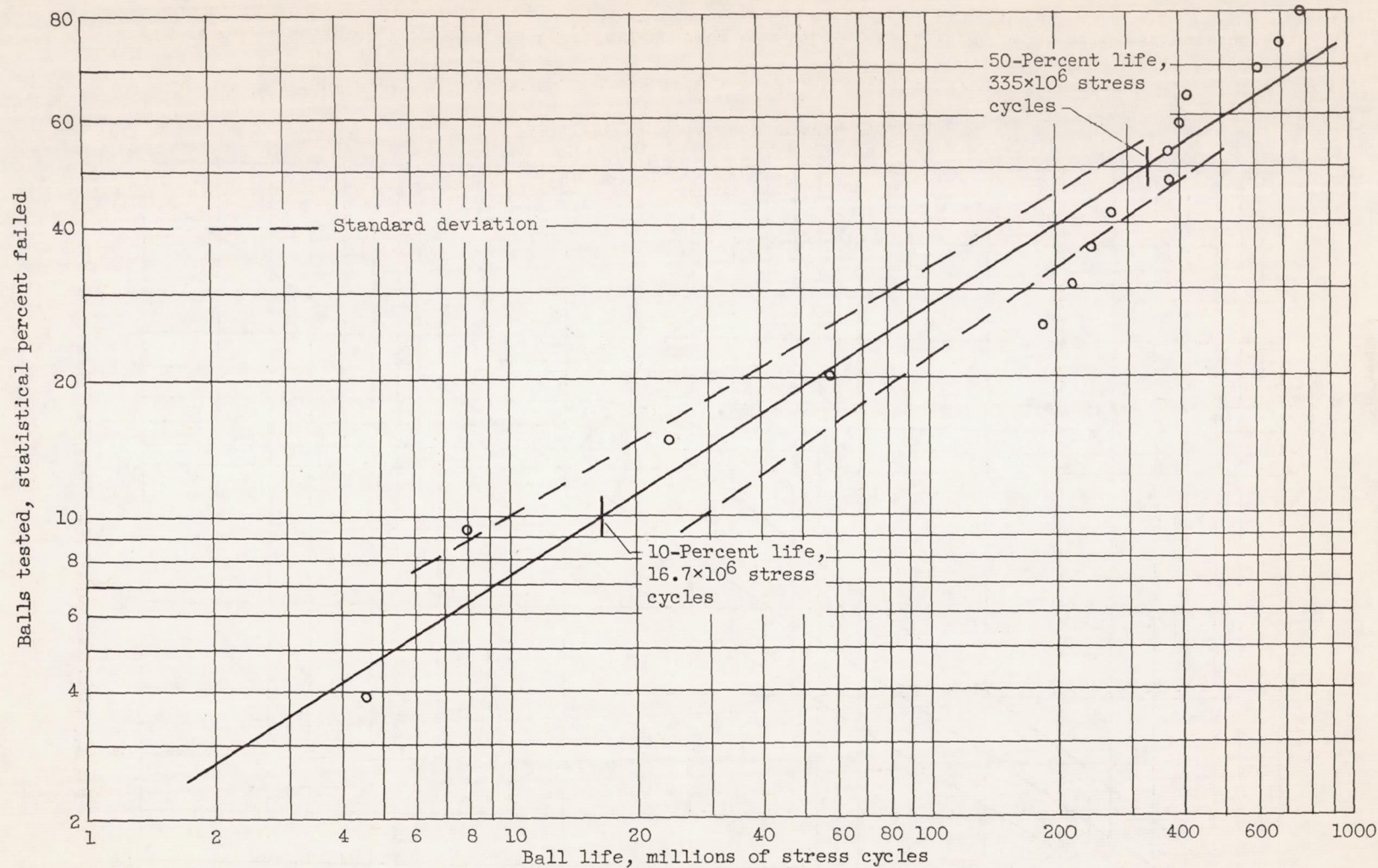
Figure 3. - Rolling-contact fatigue life of AISI M-1 tool-steel balls with various lubricants. Test temperature, 100^\circ\text{F} ; maximum Hertz compressive stress, 725,000 psi.
