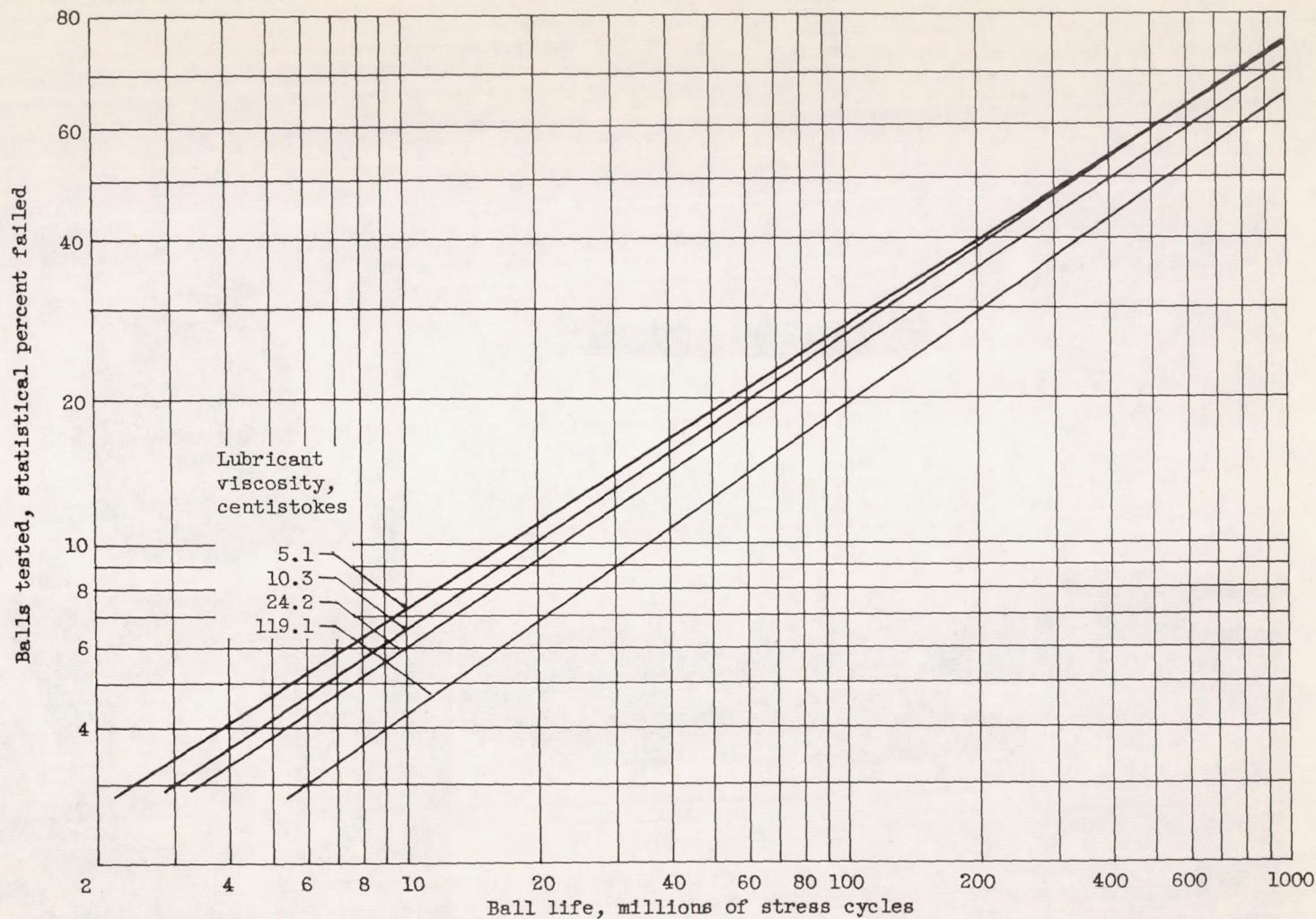
(e) Summary of fatigue lives with four mineral-oil lubricants.
