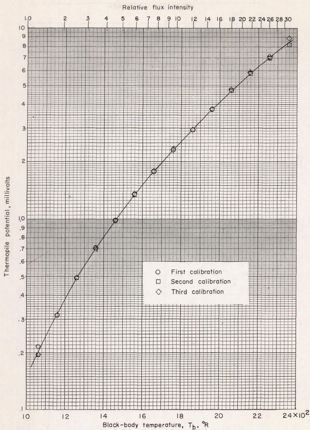
Figure 12.- Calibration of the thermopile radiation-flux measuring system.
