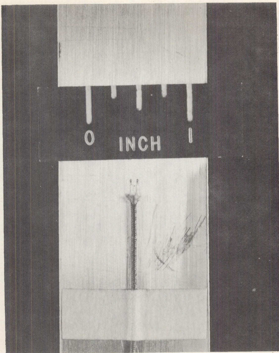
Figure 7.- Typical thermocouple installation on a test specimen.
