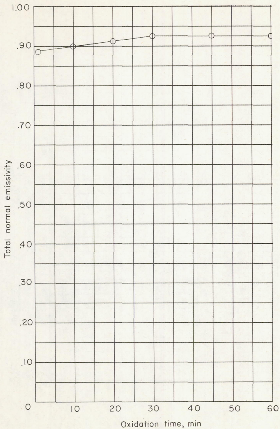
Figure 17.- Variation of total normal emissivity of Inconel X with time of oxidation at 2,000° F in quiescent air.
