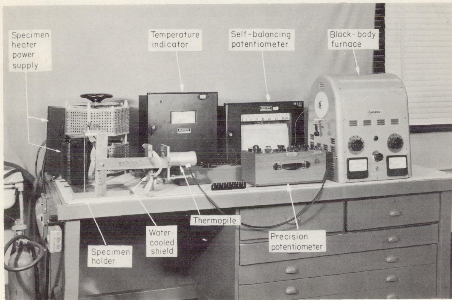
L-96503.1 Figure 3.- General view of emissivity-measuring apparatus with identification of principal components.
