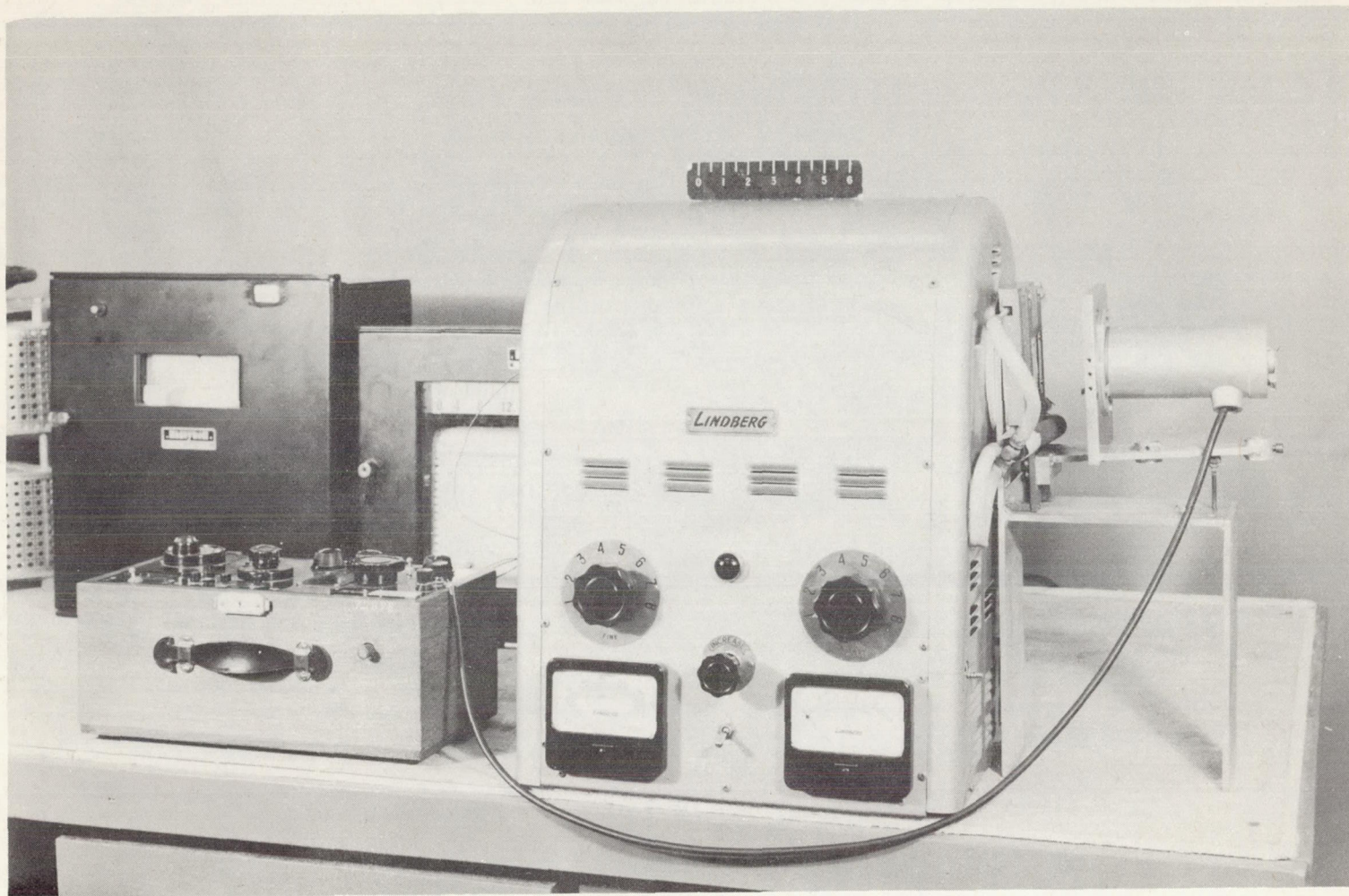
L-96505 Figure 9.- Reference-black-body furnace with thermopile and water-cooled shield in position for viewing black body and precision potentiometer used with thermopile.
