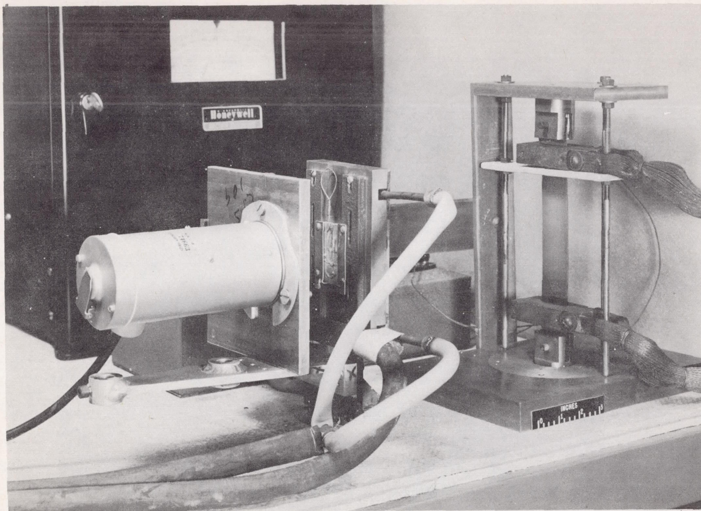
Figure 6.- Thermopile and water-cooled shield mounted on pivoted arm of test specimen holder with test specimen installed.
