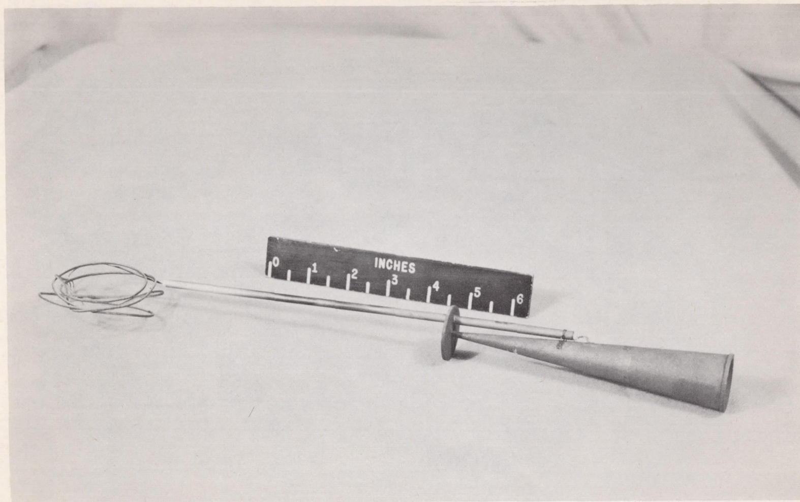
L-96506 Figure 8.- Reference-black-body conical target with thermocouple.
