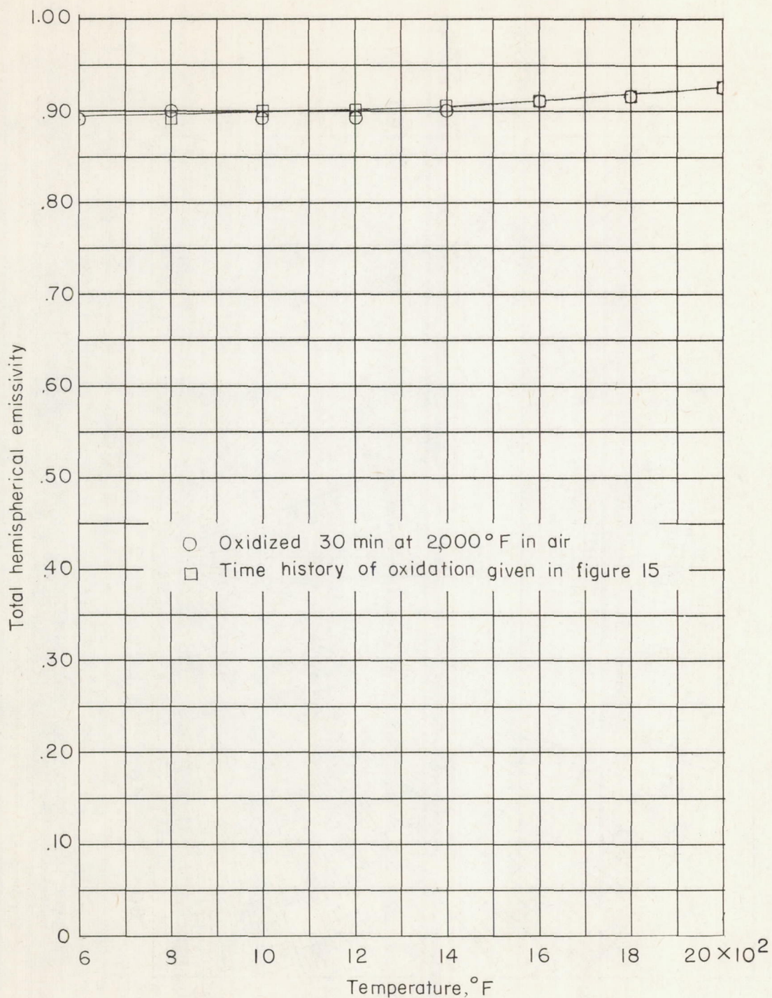
Figure 19.- Measurements of total hemispherical emissivity of stably oxidized Inconel X as function of temperature.
