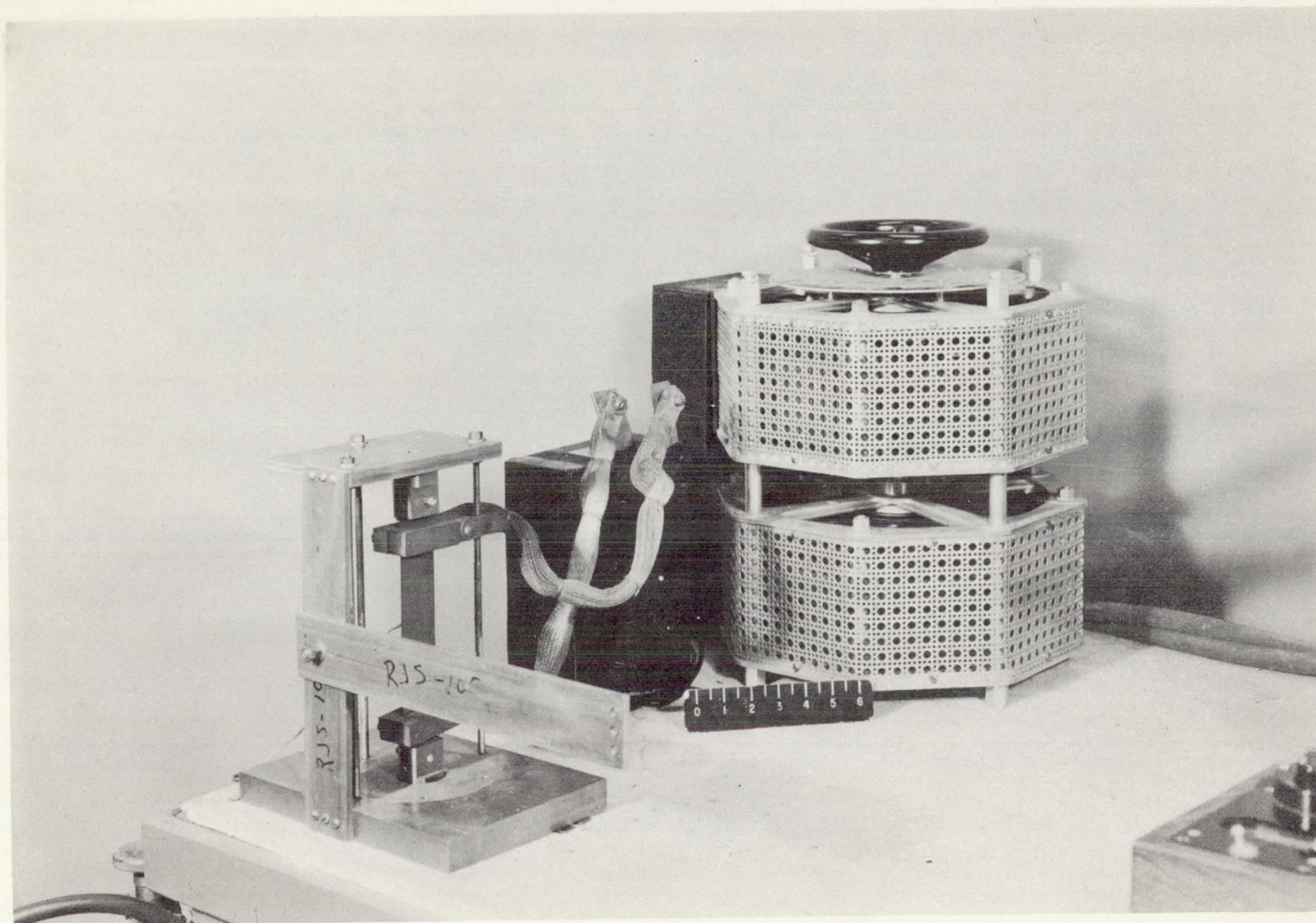
Figure 5.- Test specimen holder with specimen installed and electric power supply for heating specimen.
