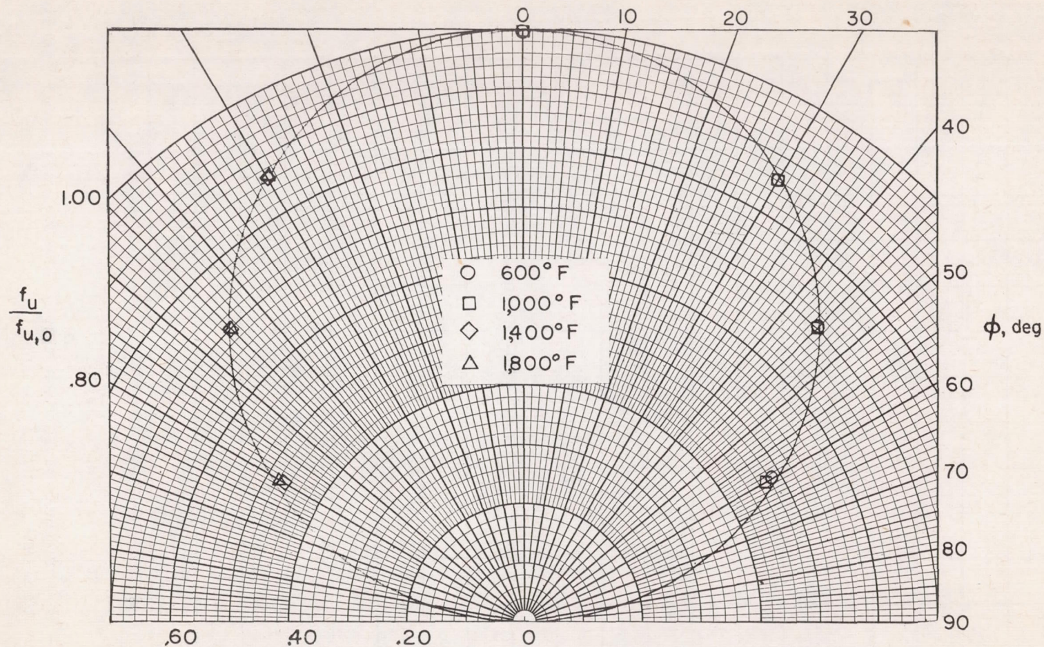
Figure 18.- Comparison of emission of Inconel X oxidized 30 minutes at 2,000° F with Lambert cosine law of diffuse emission at temperatures from 600° F to 1,800° F.
