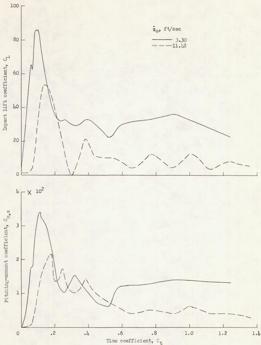
Figure 4.- Sample variations of lift and pitching-moment coefficients with time coefficient for vertical-drop tests without forward speed. \tau = 0^\circ ; C_\Delta = 18.59 .
