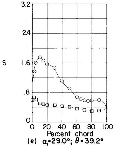
Figure 70.- Blade-surface pressure distributions and blade section characteristics for the cascade combination, \beta_1 = 60^\circ , \sigma = 1.50 , and blade section, NACA 65-(24)10.
