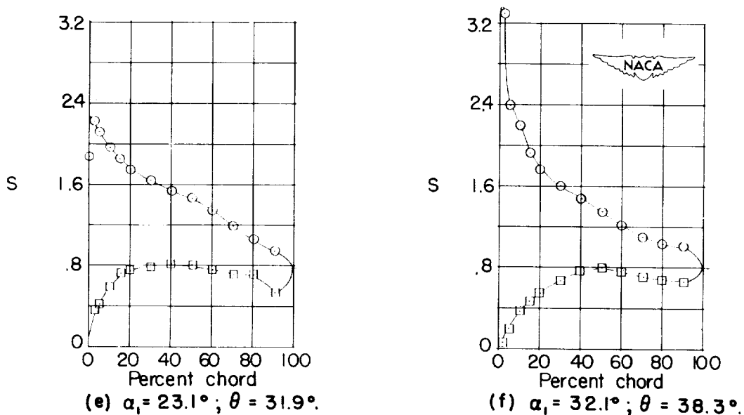
Figure 13.- Blade-surface pressure distributions and blade section characteristics for the cascade combination, \beta_1 = 30^\circ , \sigma = 1.25 , and blade section, NACA 65-(12)10.
