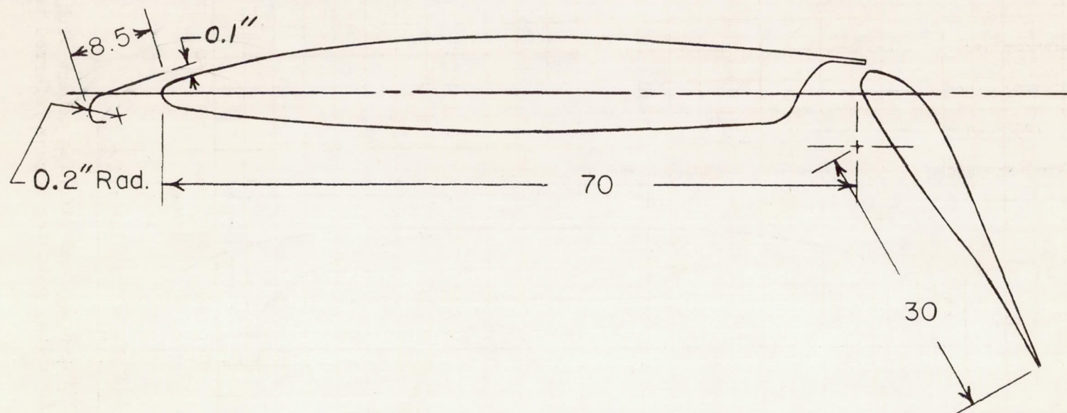
(c) Typical wing section showing flap and slat details. Flap at 60^\circ . All dimensions in percent chord except as shown.
