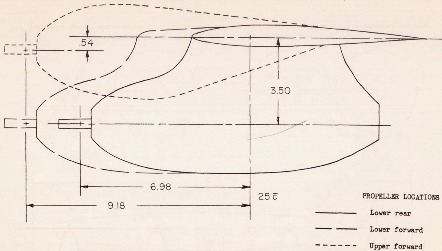
(b) Relative locations of the three propeller configurations tested. All dimensions are in inches.
