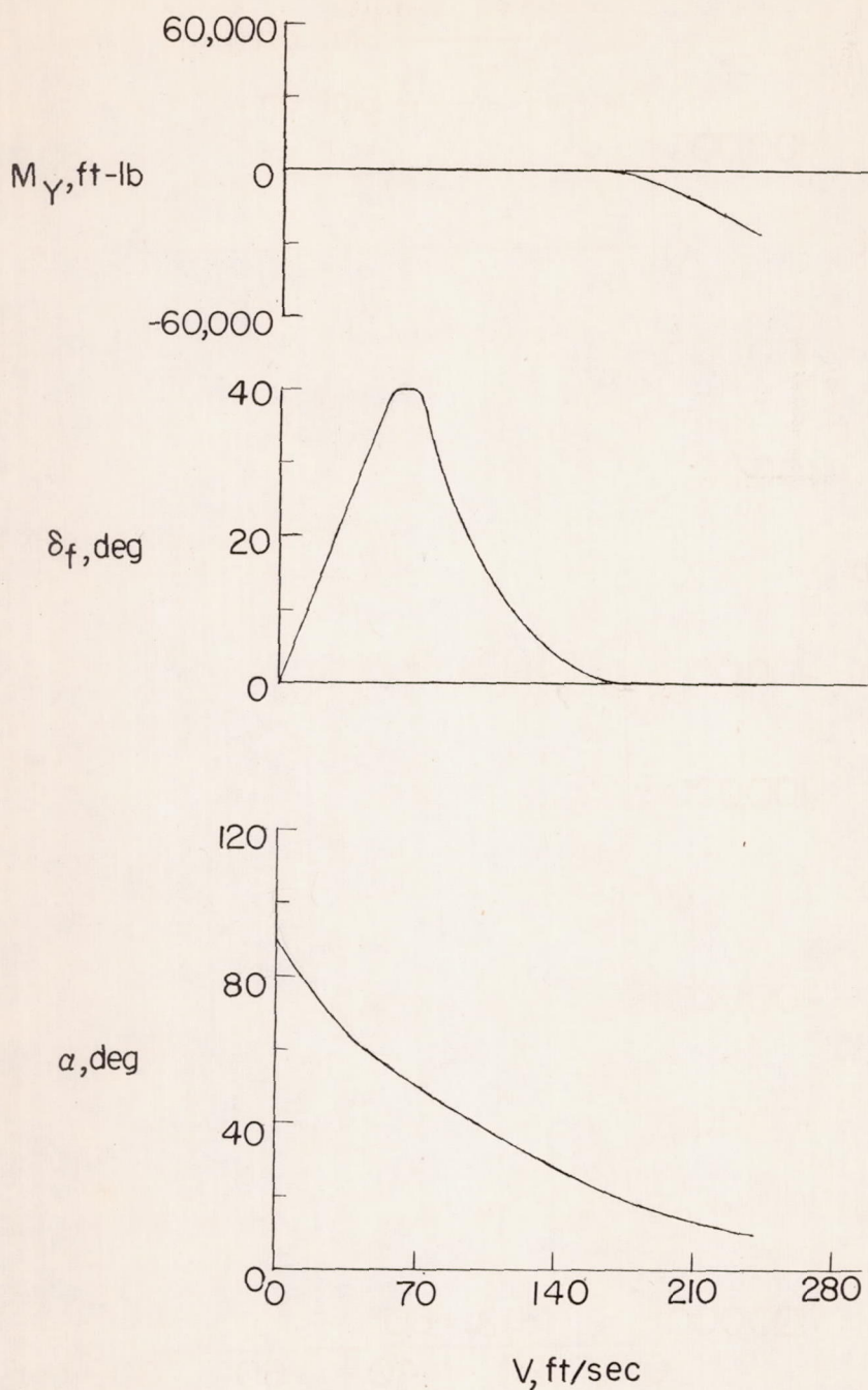
Figure 10.- Variation of pitching moment, flap deflection, and wing angle of attack of wing-propeller combination with velocity for the hypothetical airplane of figure 7 with an optimized propeller location and variation of flap deflection with angle of attack.
