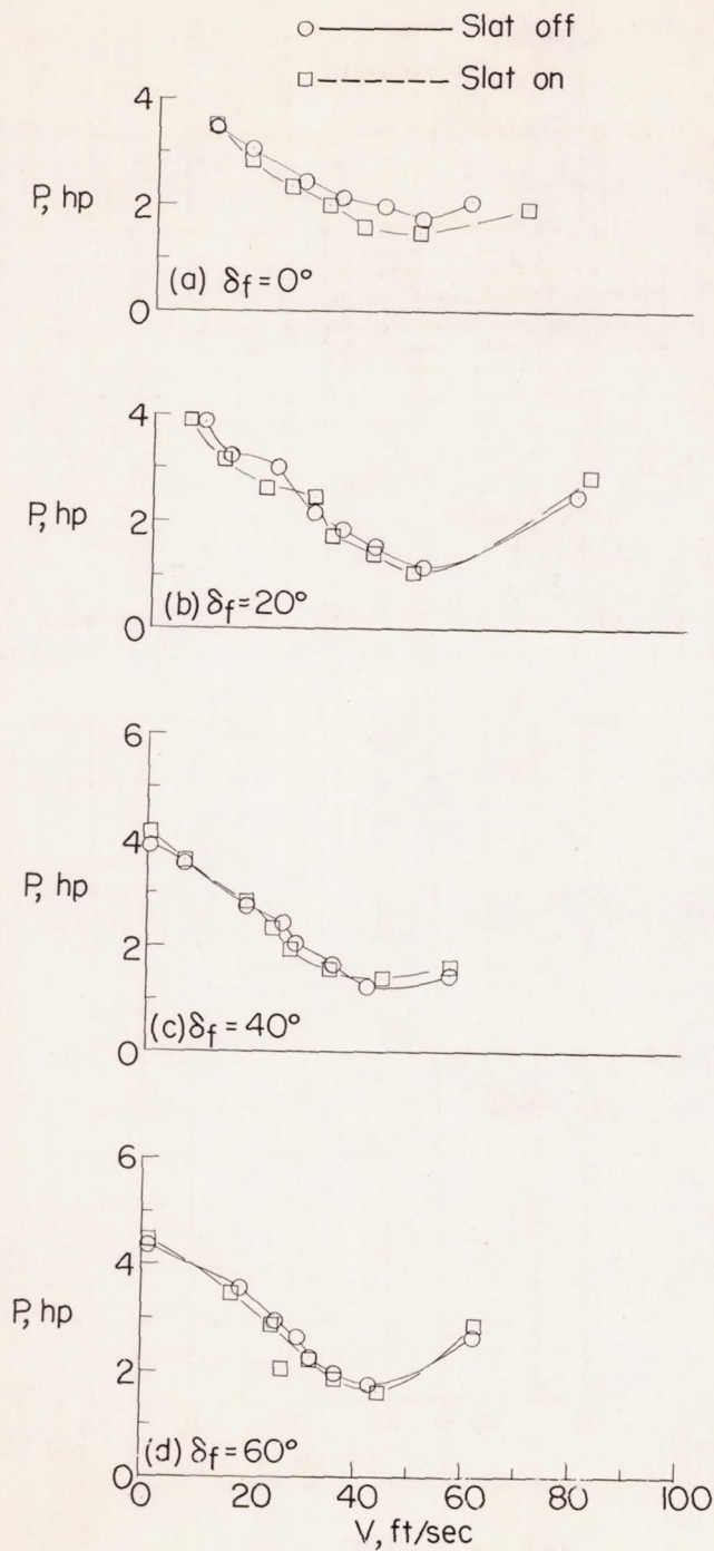
Figure 5.- Power input to model motor required through transition scaled up for a constant lift of 25 pounds. Drag = 0.
