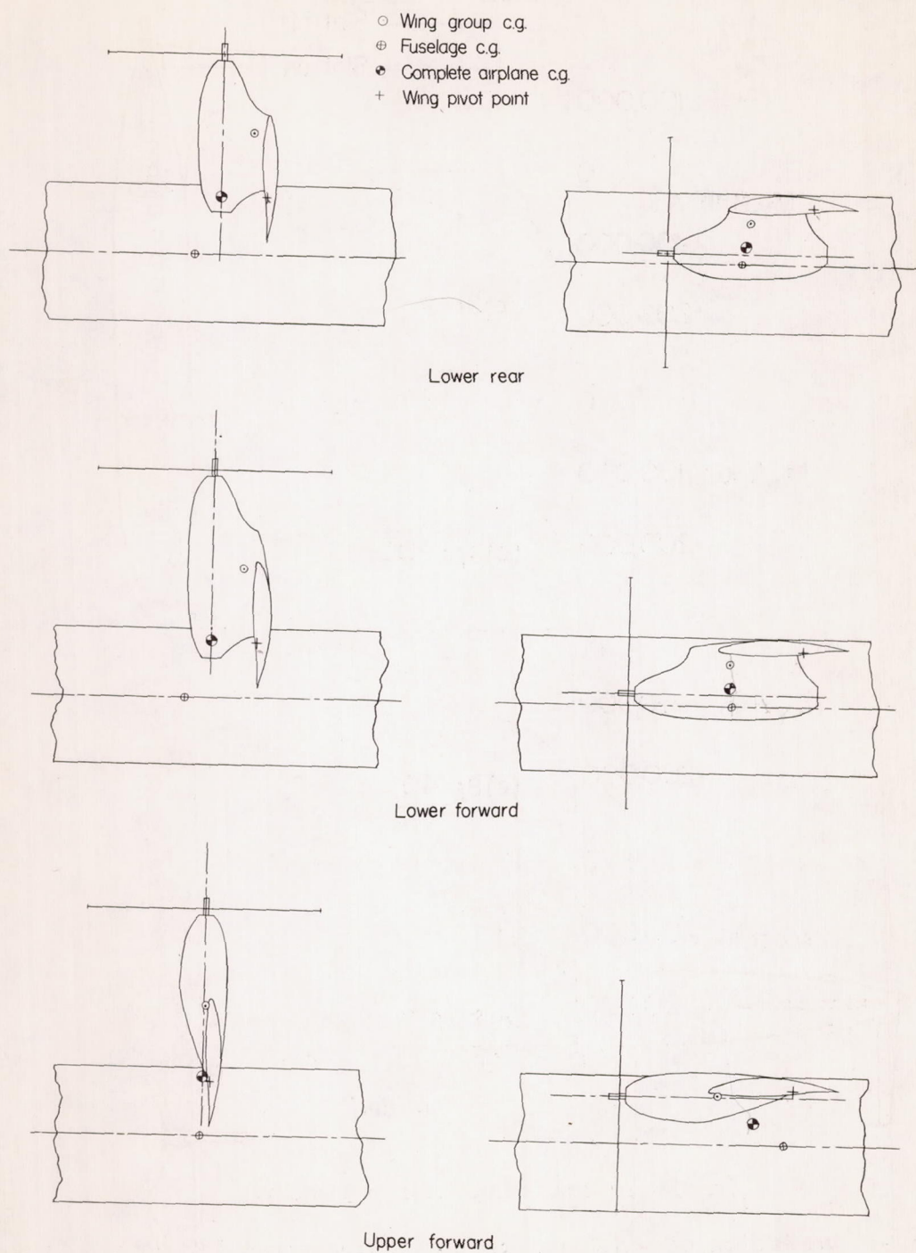
Figure 8.- Assumed center of gravity positions for various nacelle arrangements of hypothetical airplane.
