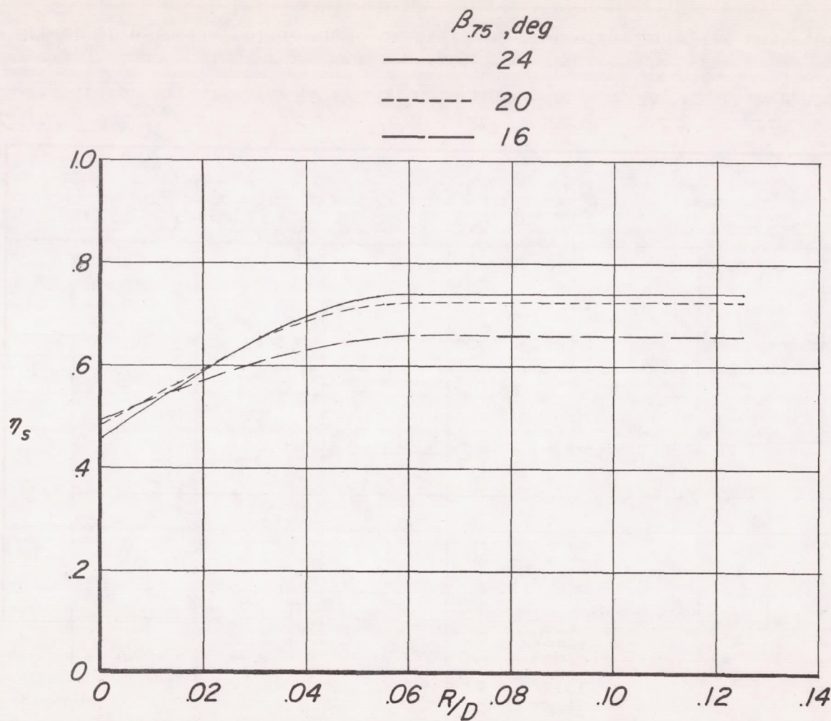
Figure 5.- Effect of lip radius ratio on static thrust efficiency at several blade angles.
