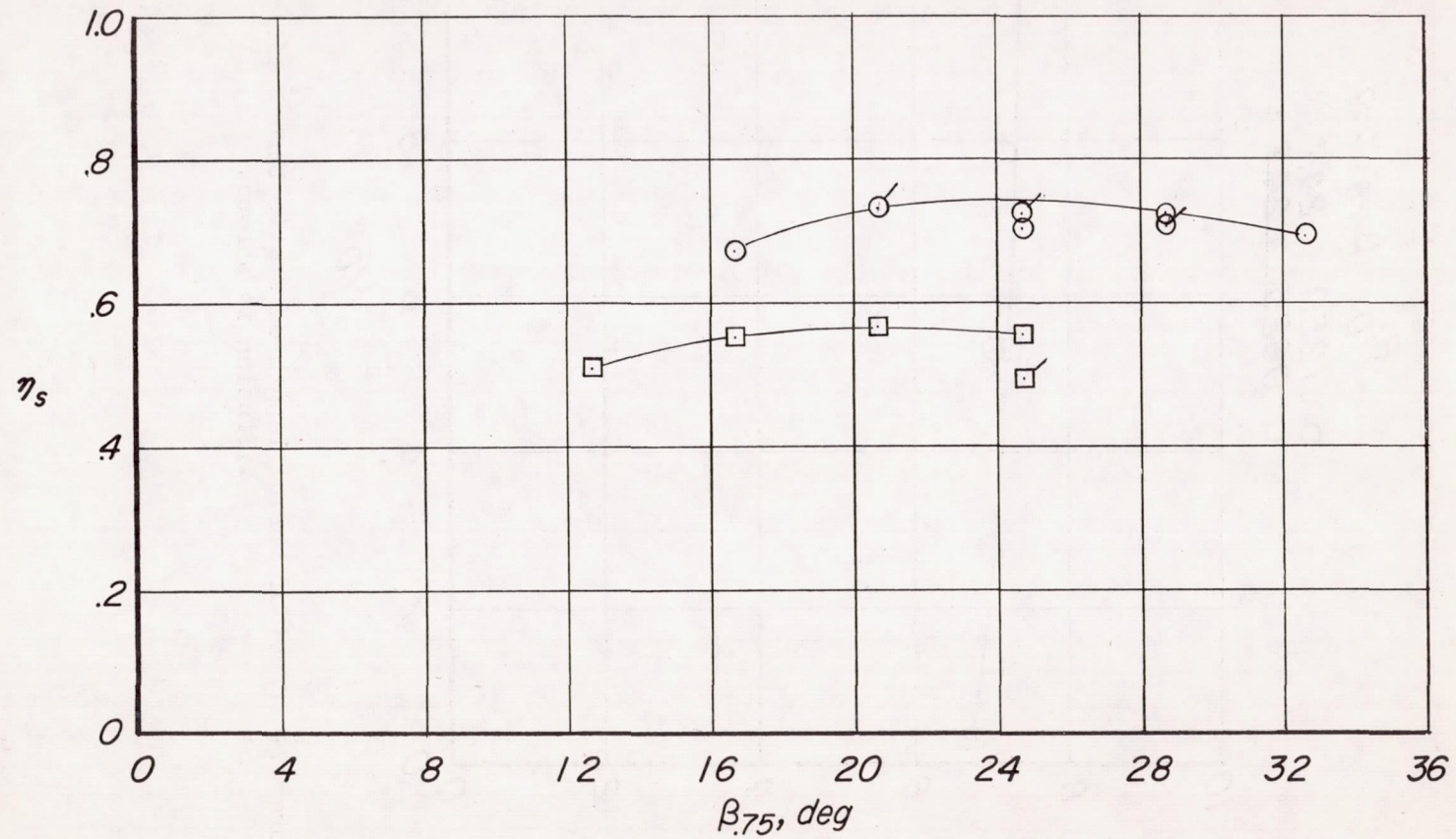
Figure 7.- Effect of propeller location downstream in shroud.
