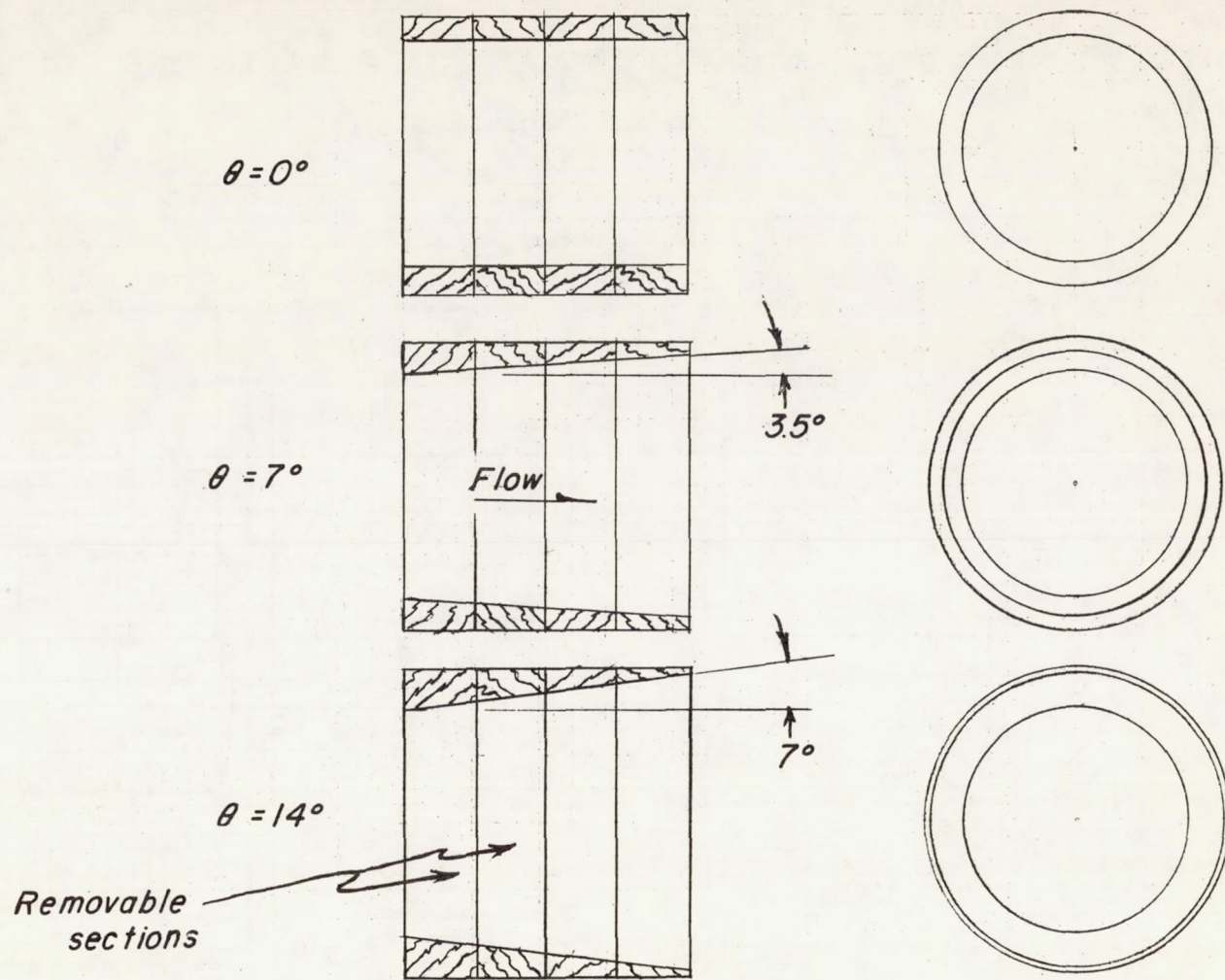
(b) Sketch of shroud configurations.
