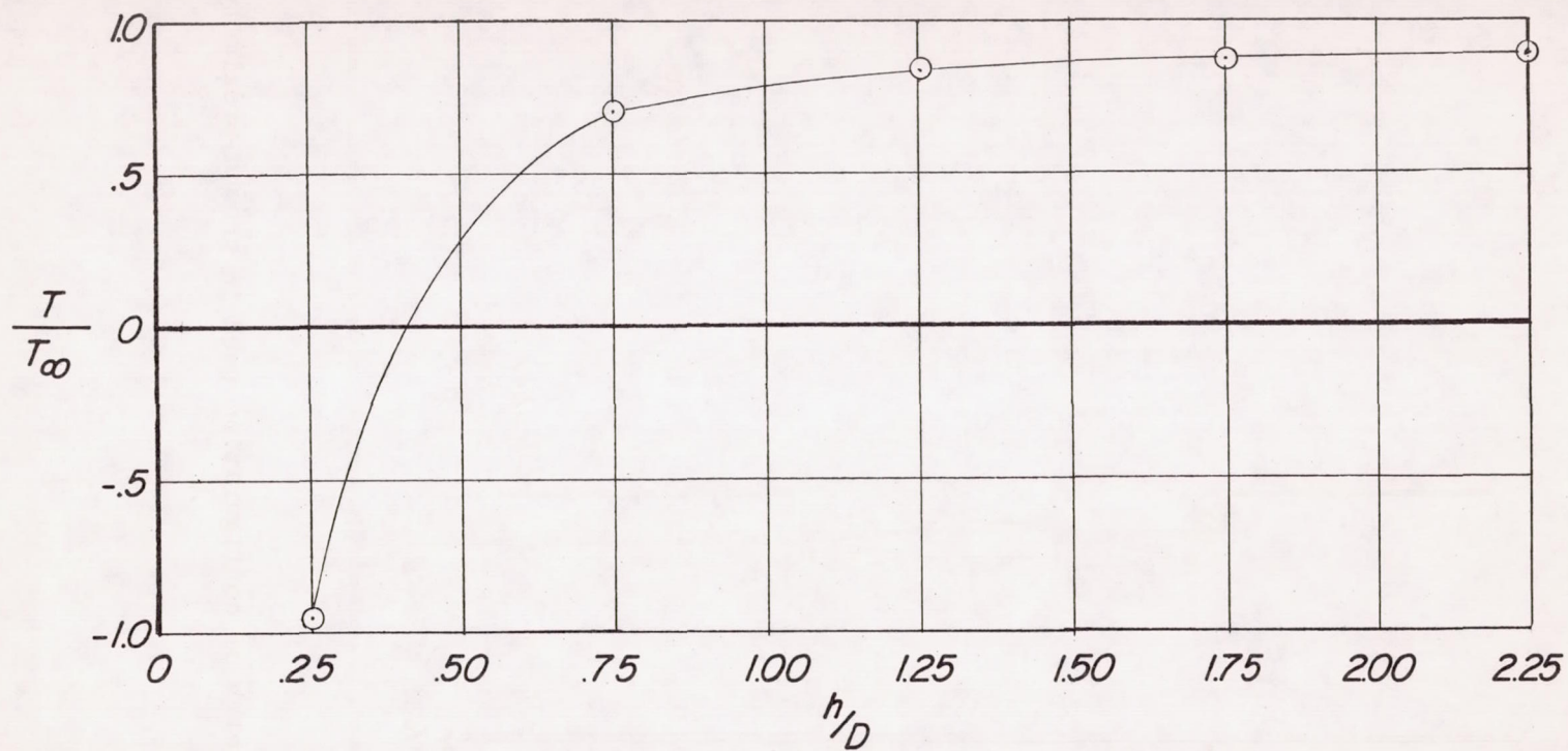
Figure 13.- Effect of proximity of ground to shroud exit on static thrust of a shrouded propeller submerged in a wing. \frac{l}{D} = 0.28 ; \frac{R}{D} = 0.125 .
