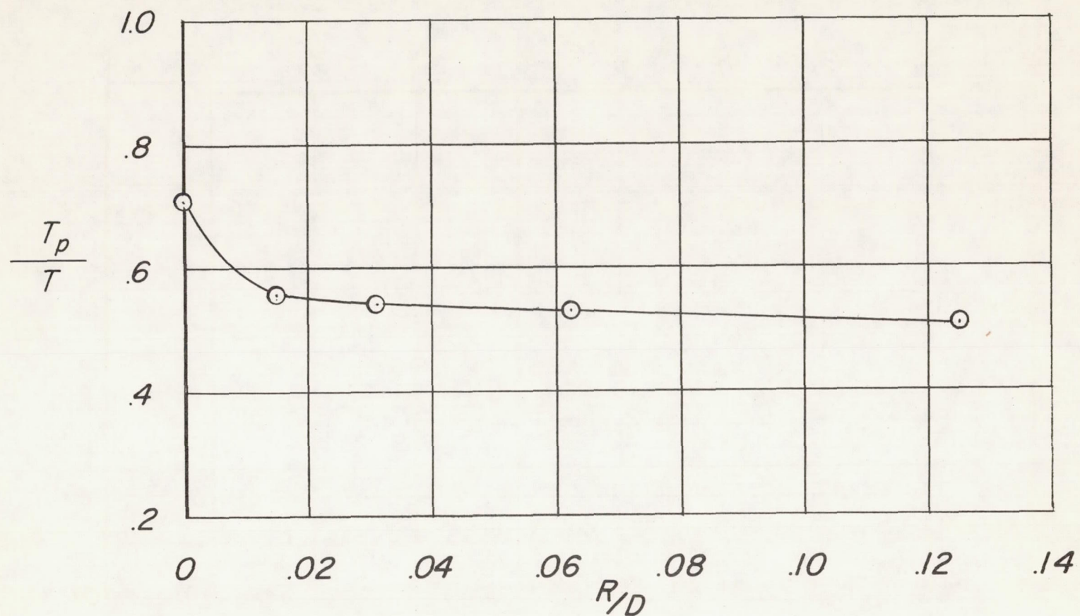
Figure 6.- Experimental variation of propeller thrust ratio T_p/T with lip radius ratio at the propeller blade angle for maximum static thrust efficiency. \frac{A_E}{A_D} = 1.0 ; \frac{l}{D} = 1.03 .
