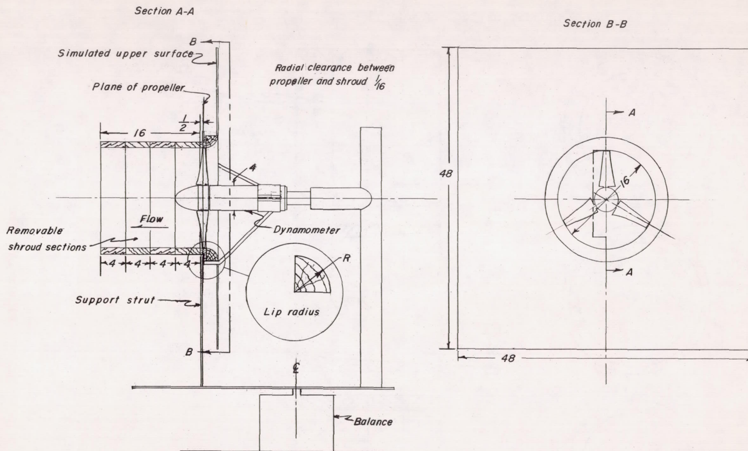
(a) Test configuration mounted on balance.
