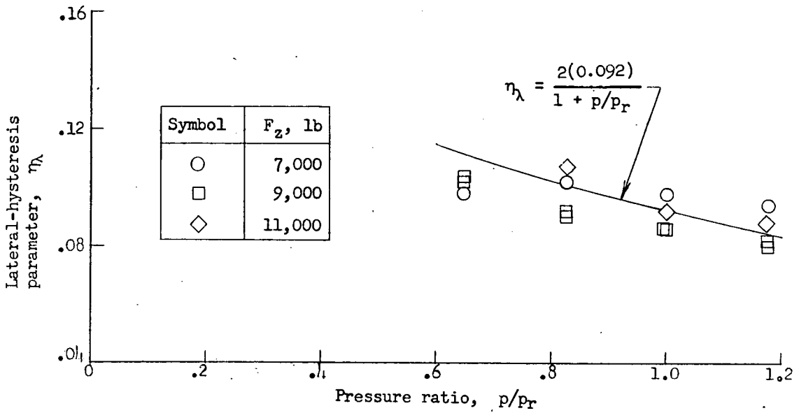
(a) 24x7.7-R25 normal-tread tires.
