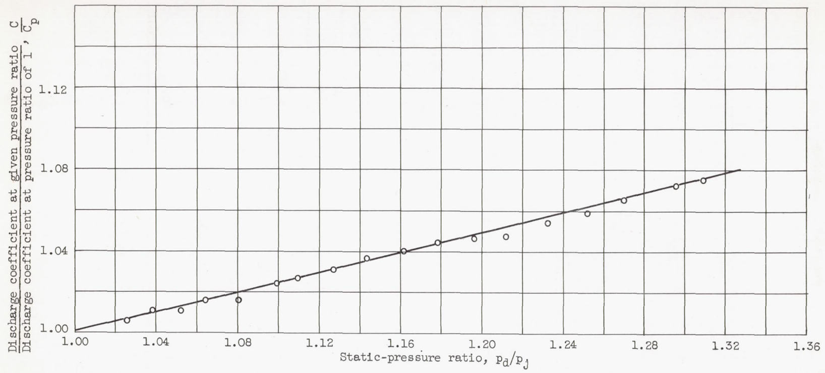
Figure 5. - Pressure-ratio correction factor for hole discharge coefficients (data from fig. 3). Hole diameter, 0.75 inch; wall thickness at hole, 0.040 inch.
