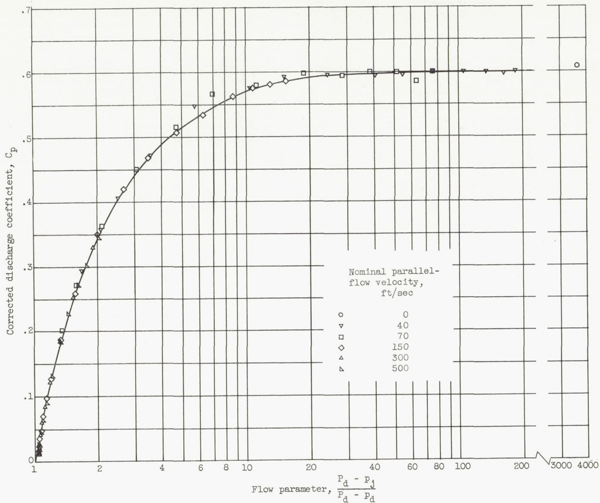
Figure 6. - Continued. Variation of corrected discharge coefficient with flow parameter.
