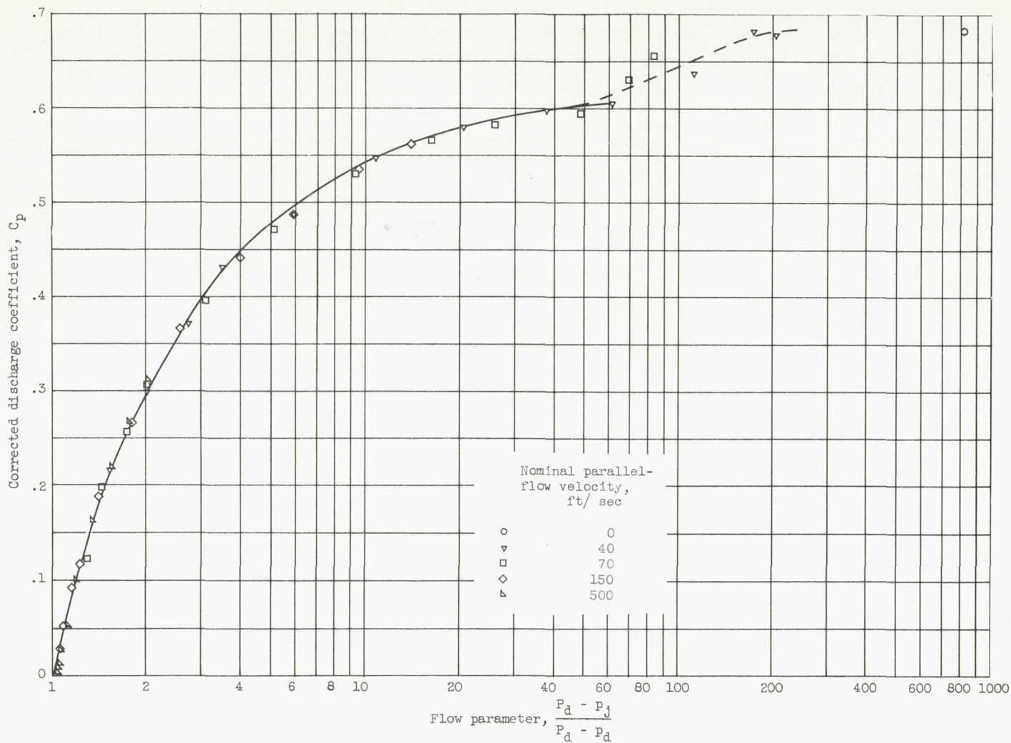
Figure 6. - Continued. Variation of corrected discharge coefficient with flow parameter.
