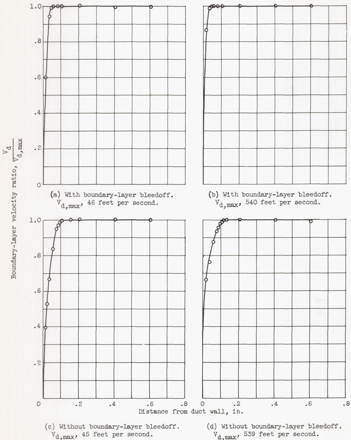
Figure 7. - Boundary-layer velocity profiles 1 inch upstream of center of test hole.
