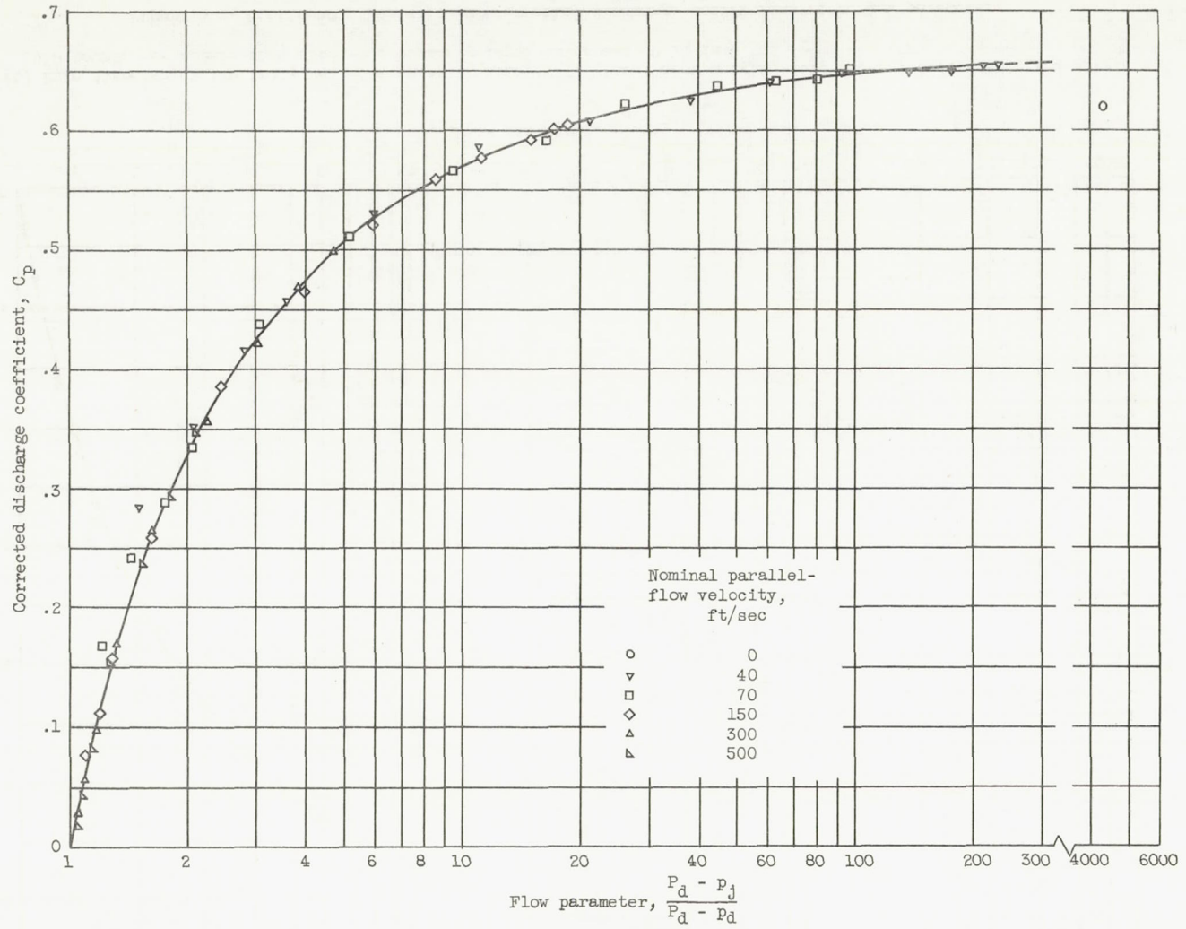
Figure 6. - Variation of corrected discharge coefficient with flow parameter.
