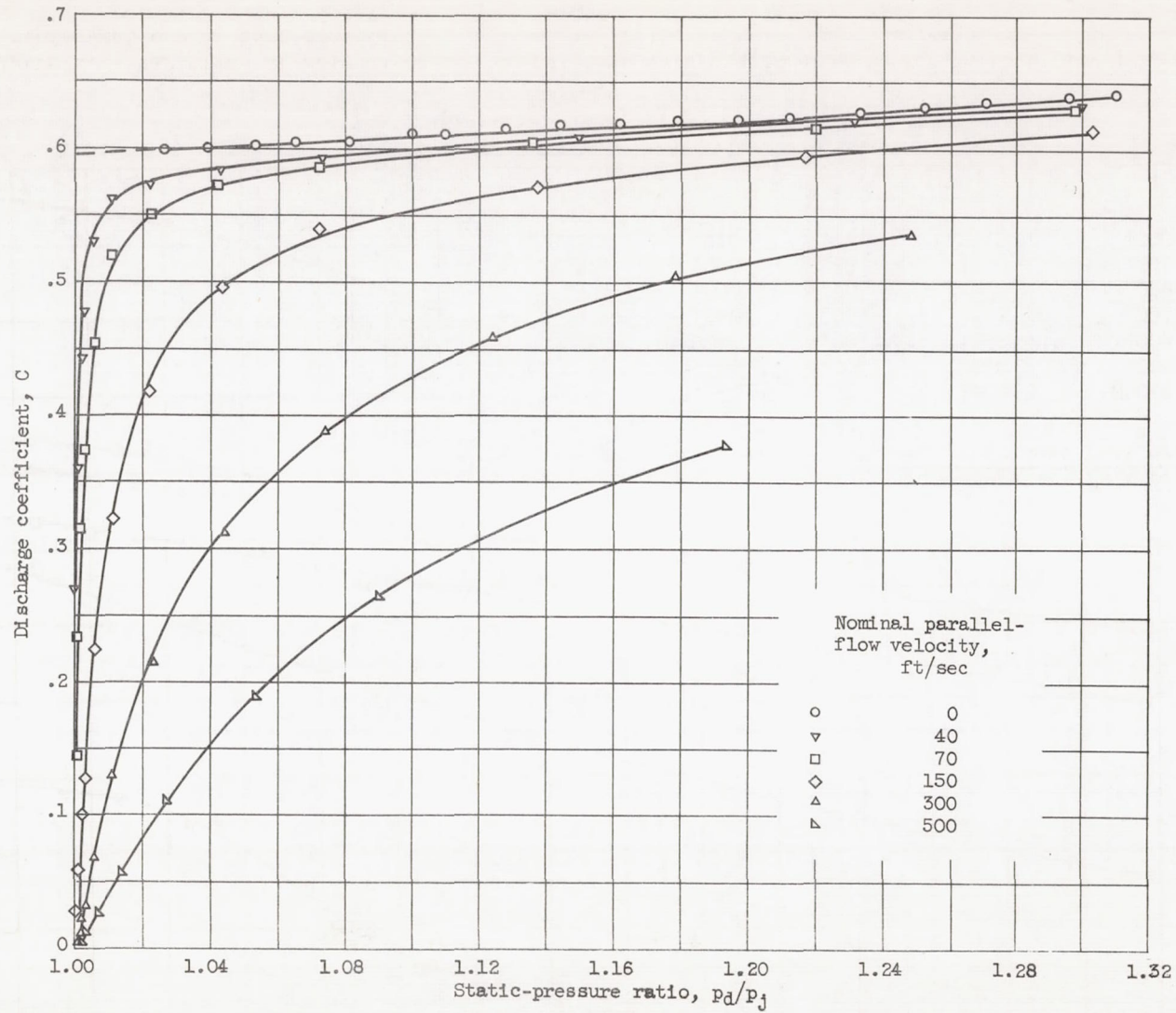
Figure 3. - Effect of static-pressure ratio on hole discharge coefficients at various parallel-flow velocities. Hole diameter, 0.75 inch; wall thickness at hole, 0.040 inch.
