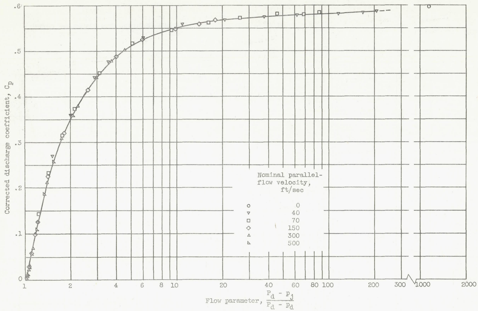
(e) Hole diameter, 0.750 inch; wall thickness at hole, 0.040 inch; duct height, 2.23 inches; duct static pressure, 1910 pounds per square foot absolute; boundary-layer thickness, 0.10 inch.
