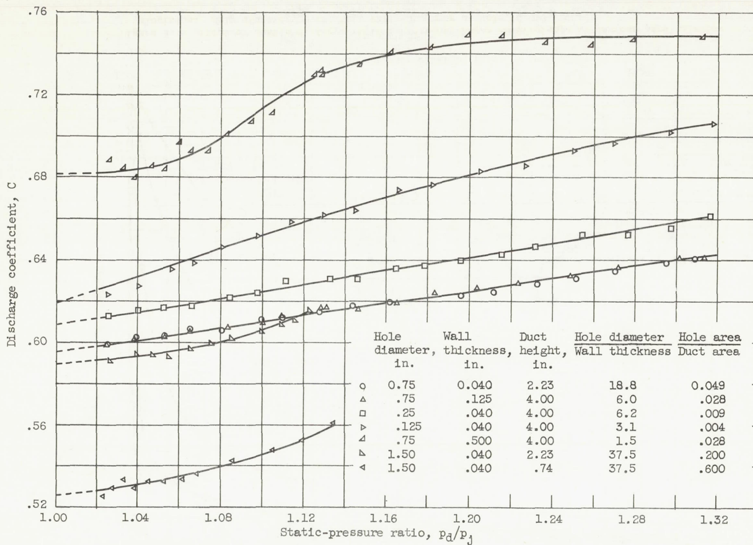
Figure 2. - Variation of hole discharge coefficient with pressure ratio for various flow passage configurations at zero crossflow.
