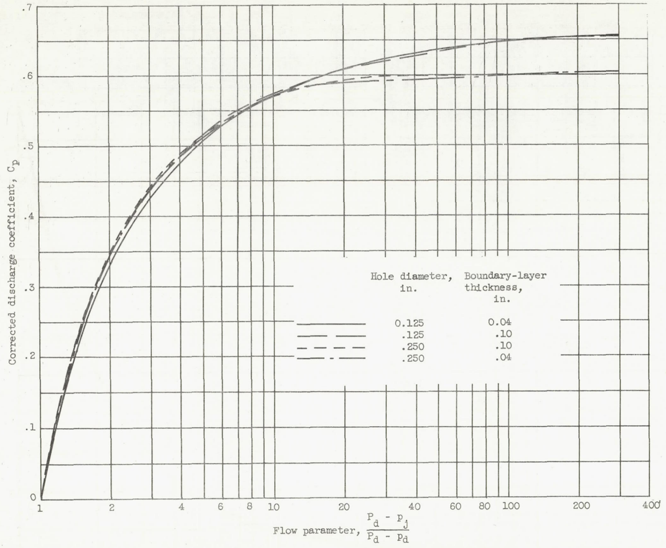
Figure 8. - Effect of boundary-layer thickness on corrected discharge coefficient of small holes.
