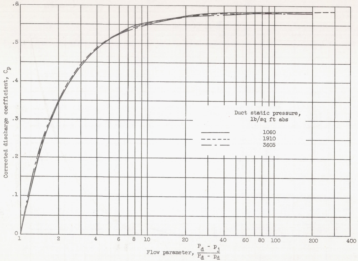
Figure 9. - Effect of duct static-pressure level on corrected discharge coefficient. Hole diameter, 0.75 inches.
