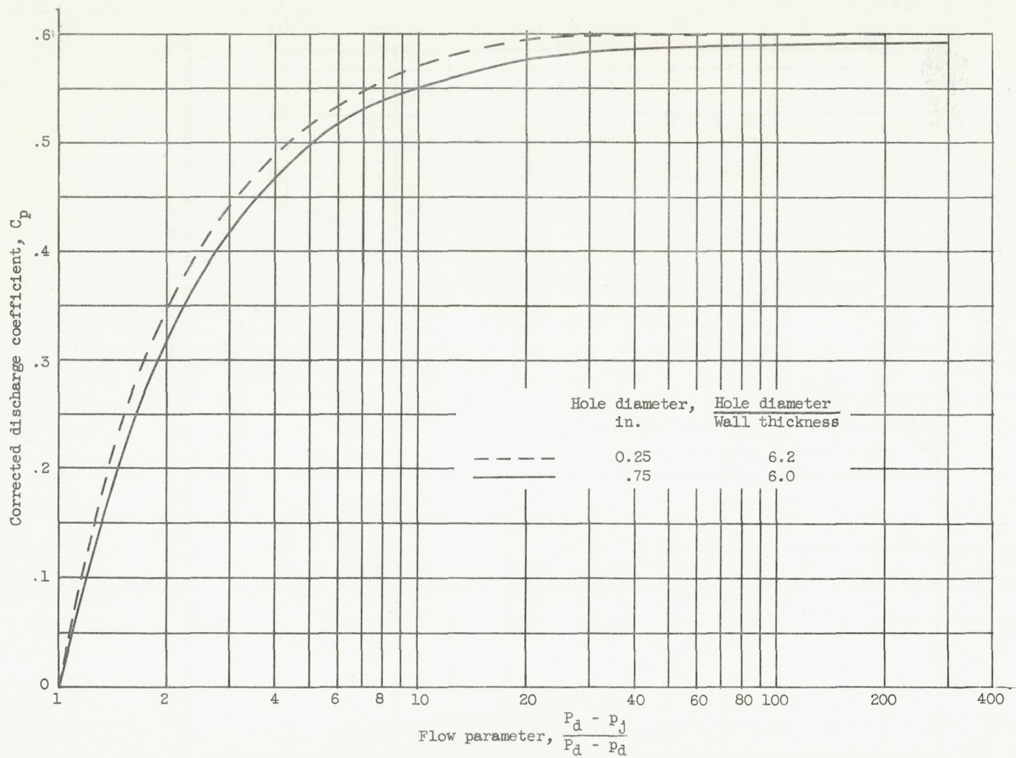
Figure 12. - Comparison of corrected discharge coefficients of holes with different diameters having constant ratio of hole diameter to wall thickness.
