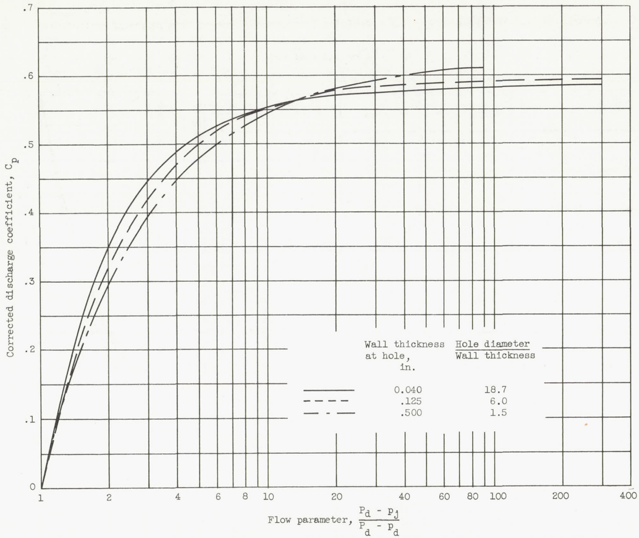
Figure 10. - Effect of wall thickness on corrected discharge coefficient. Hole diameter, 0.750 inch.
