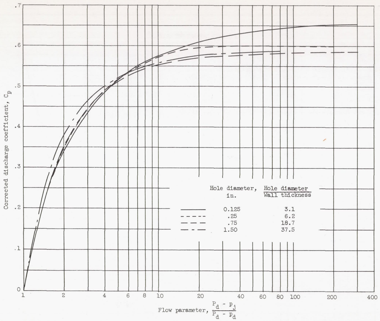
Figure 11. - Effect of hole diameter on corrected discharge coefficient. Wall thickness at hole, 0.040 inch.
