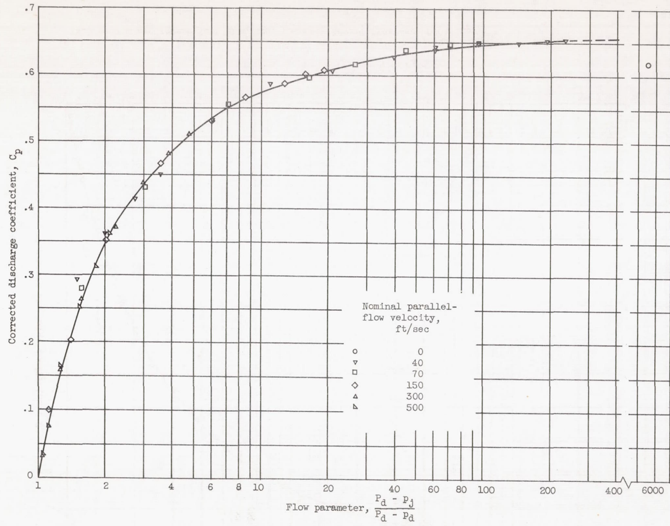
Figure 6. - Continued. Variation of corrected discharge coefficient with flow parameter.
