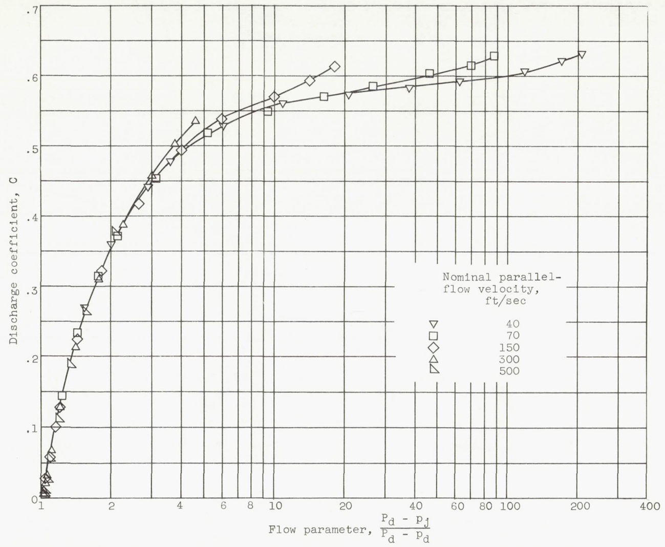
Figure 4. - Variation of hole discharge coefficient with flow parameter at various parallel-flow velocities. Hole diameter, 0.75 inch; wall thickness at hole, 0.040 inch.
