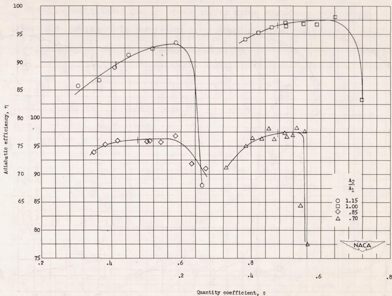
Figure 22.- Variation of adiabatic efficiency with quantity coefficient for 7\frac{1}{2}^\circ above design blade angle, solidity of 1.0, and annulus-area ratios of 1.15, 1.00, 0.85, and 0.70. (Vertical lines across curve indicate design points.)
