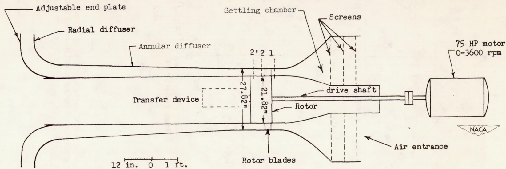
Figure 2.- Schematic diagram of test compressor showing rotor and instrumentation positions.
