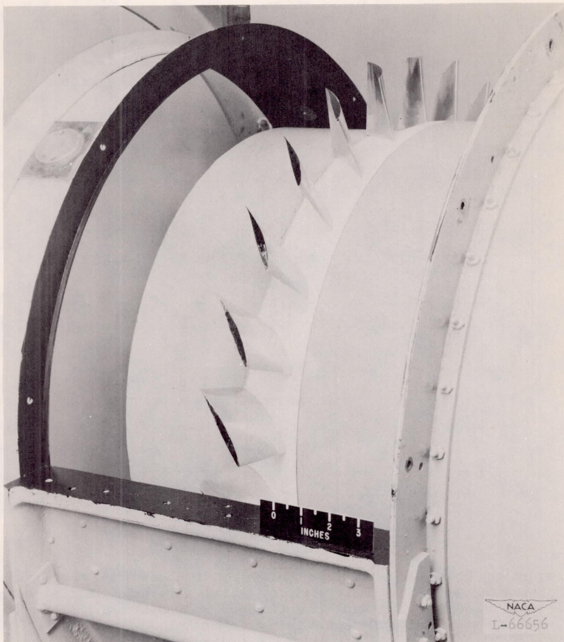
Figure 3.- Partial view of test section showing rotor configuration as altered to provide exit-to-entering annulus-area ratio of 1.15.
