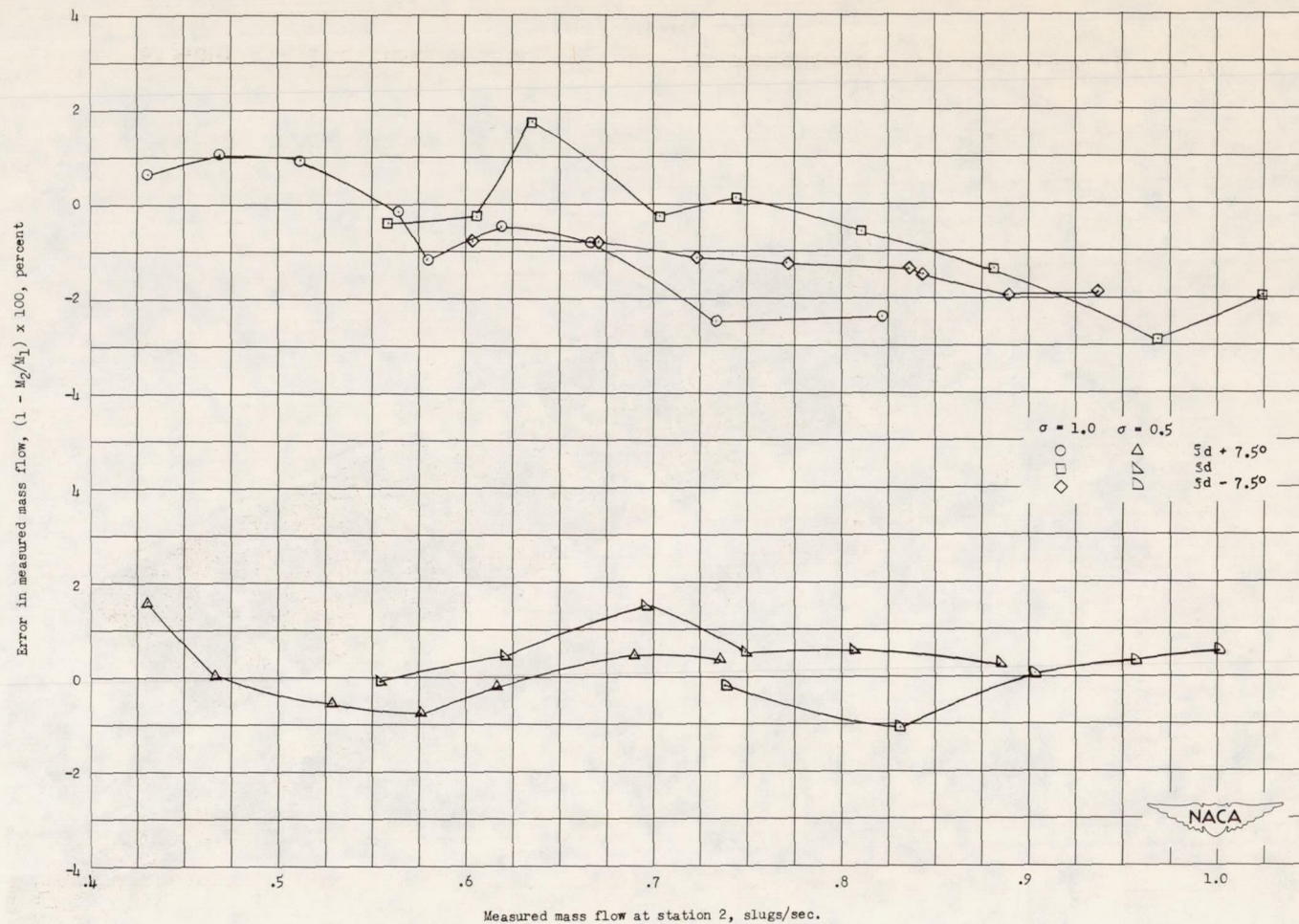
Figure 8.- Difference in measured mass flows at stations 1 and 2 for the constant-area tests with design, 7\frac{1}{2}^\circ above design, and 7\frac{1}{2}^\circ below design blade angles at solidities of 1.0 and 0.5.
