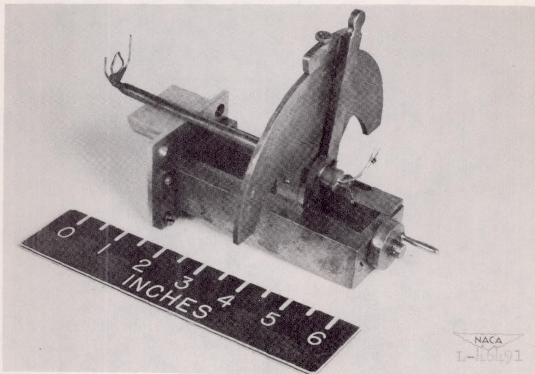
Figure 5.- Survey instrument with measuring head installed showing arrangement of yaw, total-pressure, and static-pressure tubes.
