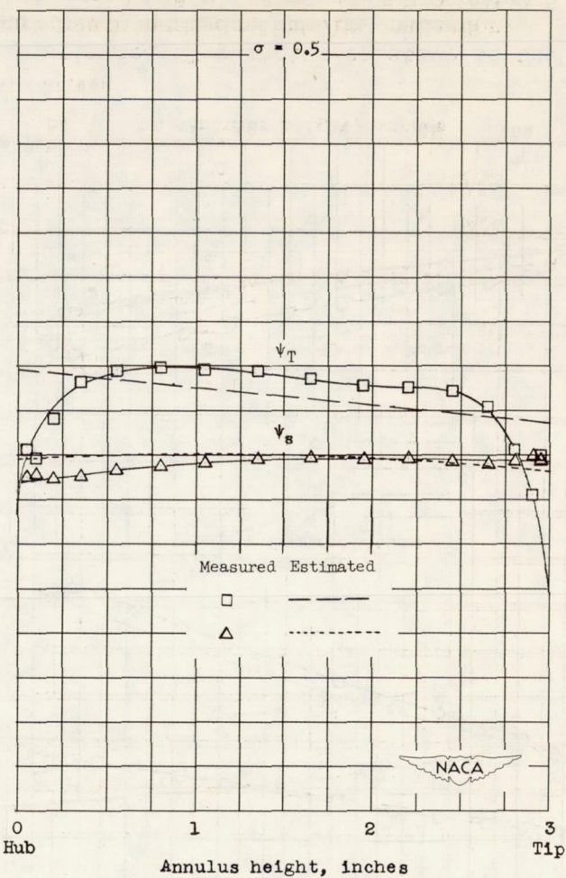
Figure 19.- Variation of measured and estimated total- and static-pressure-rise coefficients across the annulus for typical tests near design flow rate at the design blade angle, constant-annulus-area condition for solidities of 1.0 and 0.5.
