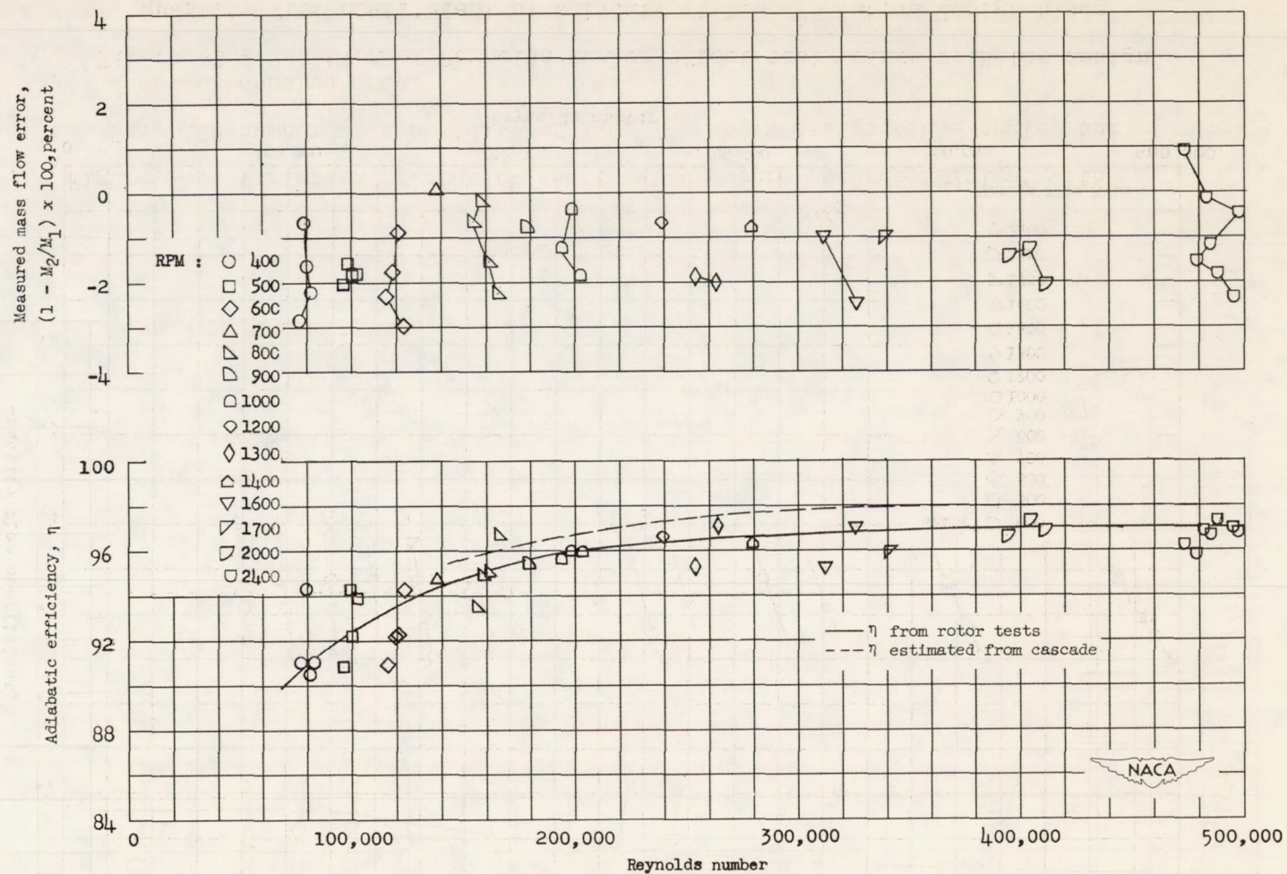
Figure 33.- Variation of measured mass flow error and measured and estimated efficiencies with Reynolds number at solidity of 1.0, 7\frac{1}{2}^\circ above design blade angle, and constant annulus area.
