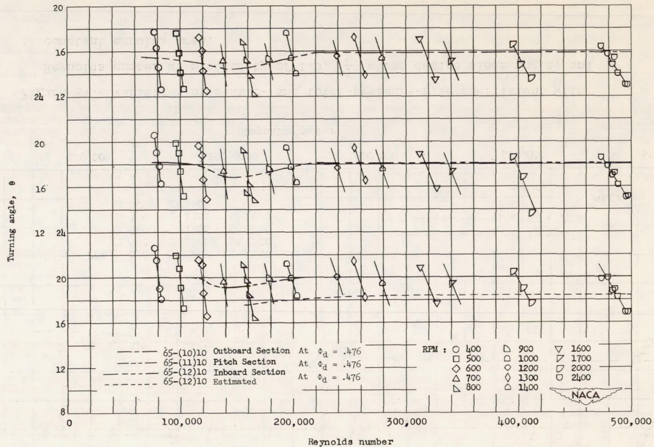
Figure 35.- Variation of measured and cascade estimated turning angles with Reynolds number at the inboard, pitch, and outboard sections for a solidity of 1.0, 7\frac{1}{2}^\circ above design blade angle, and constant annulus area.
