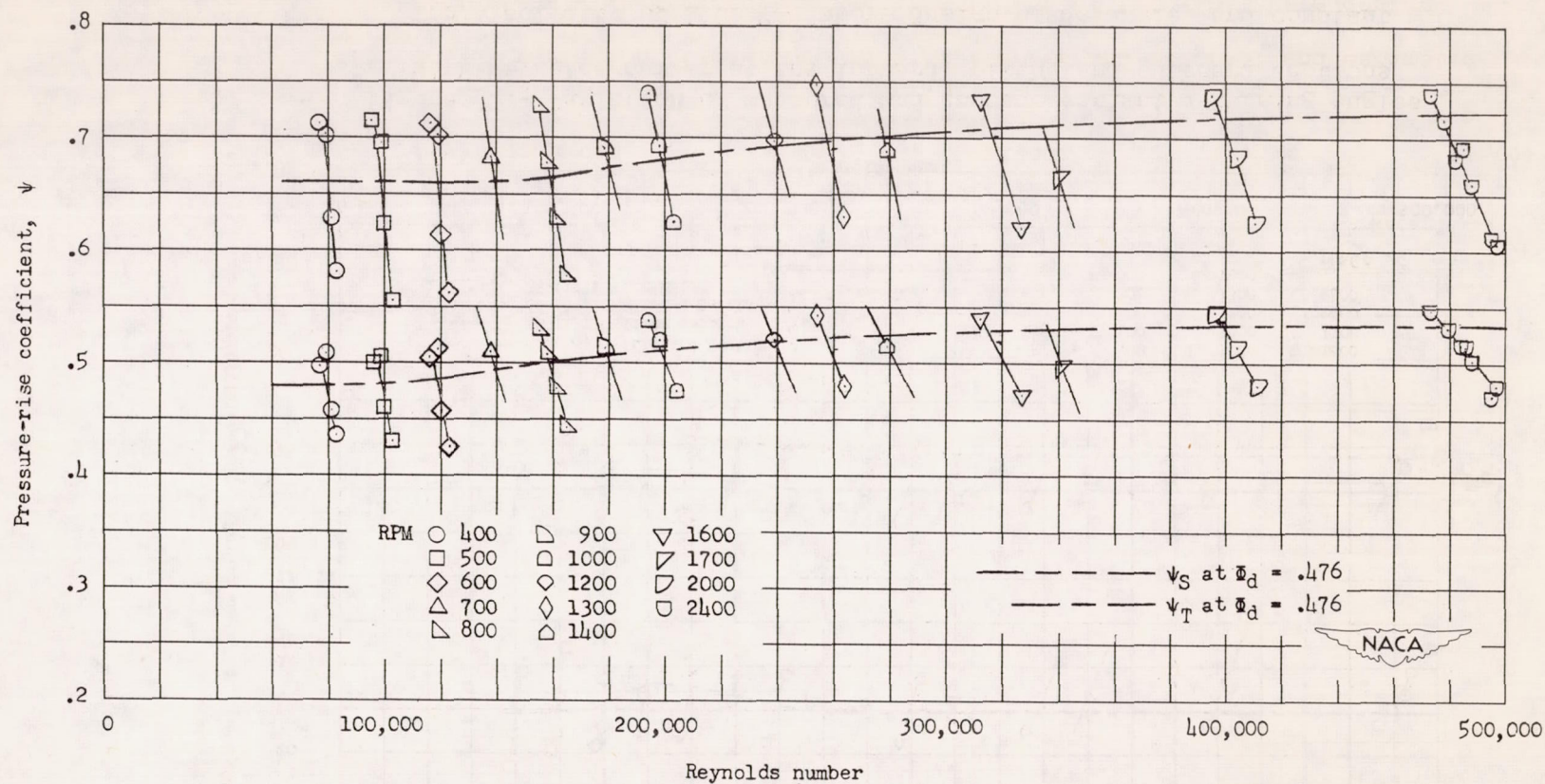
Figure 34.- Variation of static- and total-pressure-rise coefficient with Reynolds number at a solidity of 1.0, 7\frac{1}{2}^\circ above design blade angle, and constant annulus area.
