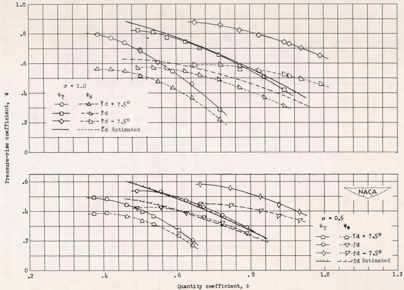
Figure 11.- Variation of total- and static-pressure-rise coefficient with quantity coefficient for the constant-annulus-area condition with design, 7\frac{1}{2}^\circ above design, and 7\frac{1}{2}^\circ below design blade angles at solidities of 1.0 and 0.5.
