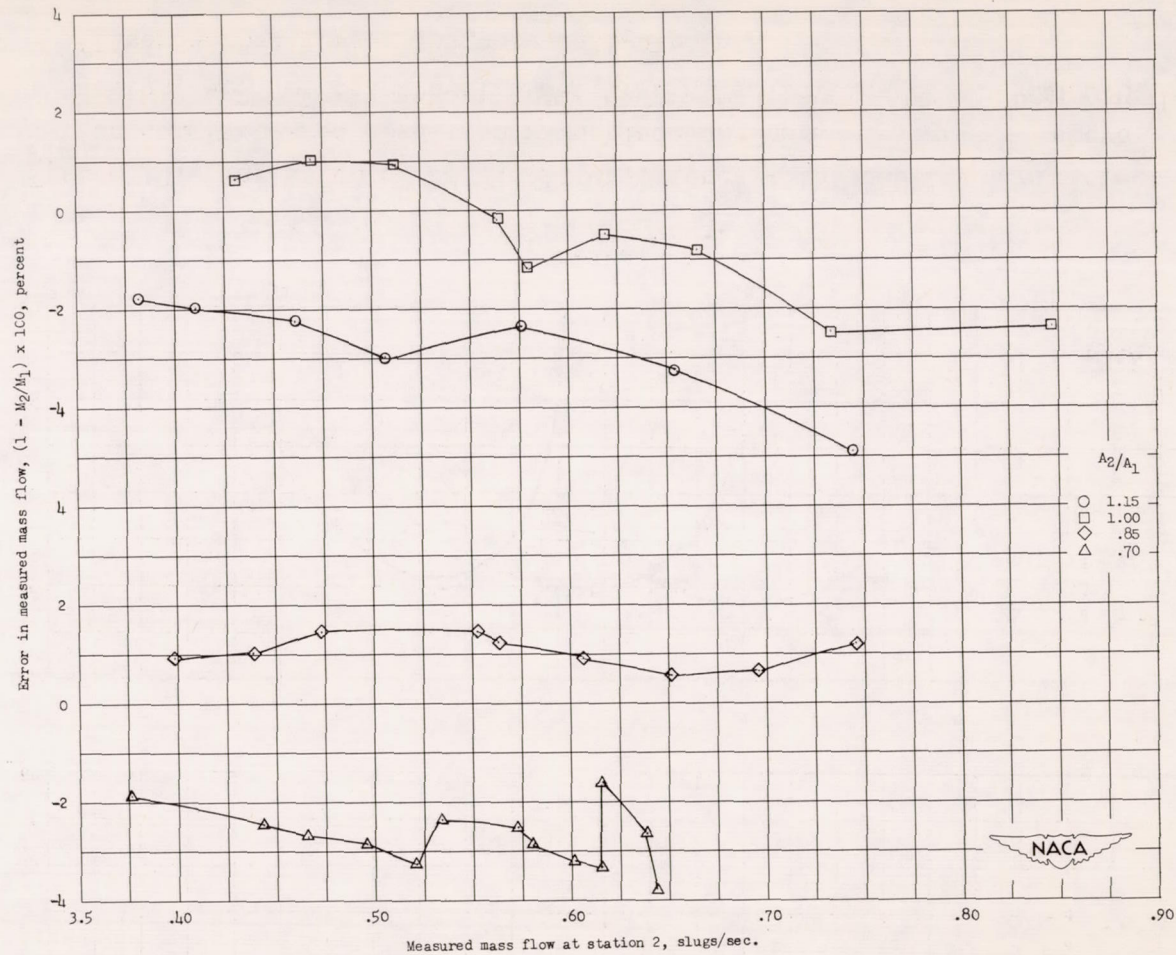
Figure 9.- Difference in measured mass flows at stations 1 and 2 for 7\frac{1}{2} above design blade angle and solidity of 1.0 with annulus-area ratios of 1.15, 1.00, 0.85, and 0.70.
