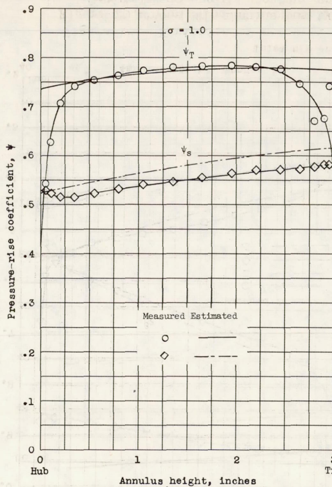
Figure 19.- Variation of measured and estimated total- and static-pressure-rise coefficients across the annulus for typical tests near design flow rate at the design blade angle, constant-annulus-area condition for solidities of 1.0 and 0.5.
