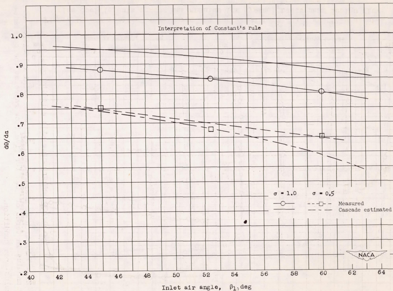
Figure 20.- Variation of average measured and estimated d\theta/da values with inlet air angle for the constant-annulus-area tests at solidities of 1.0 and 0.5.
