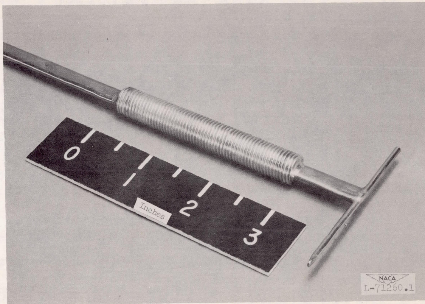
Figure 7.- Instrument used on rotor to measure static and total pressure and outlet angle.
