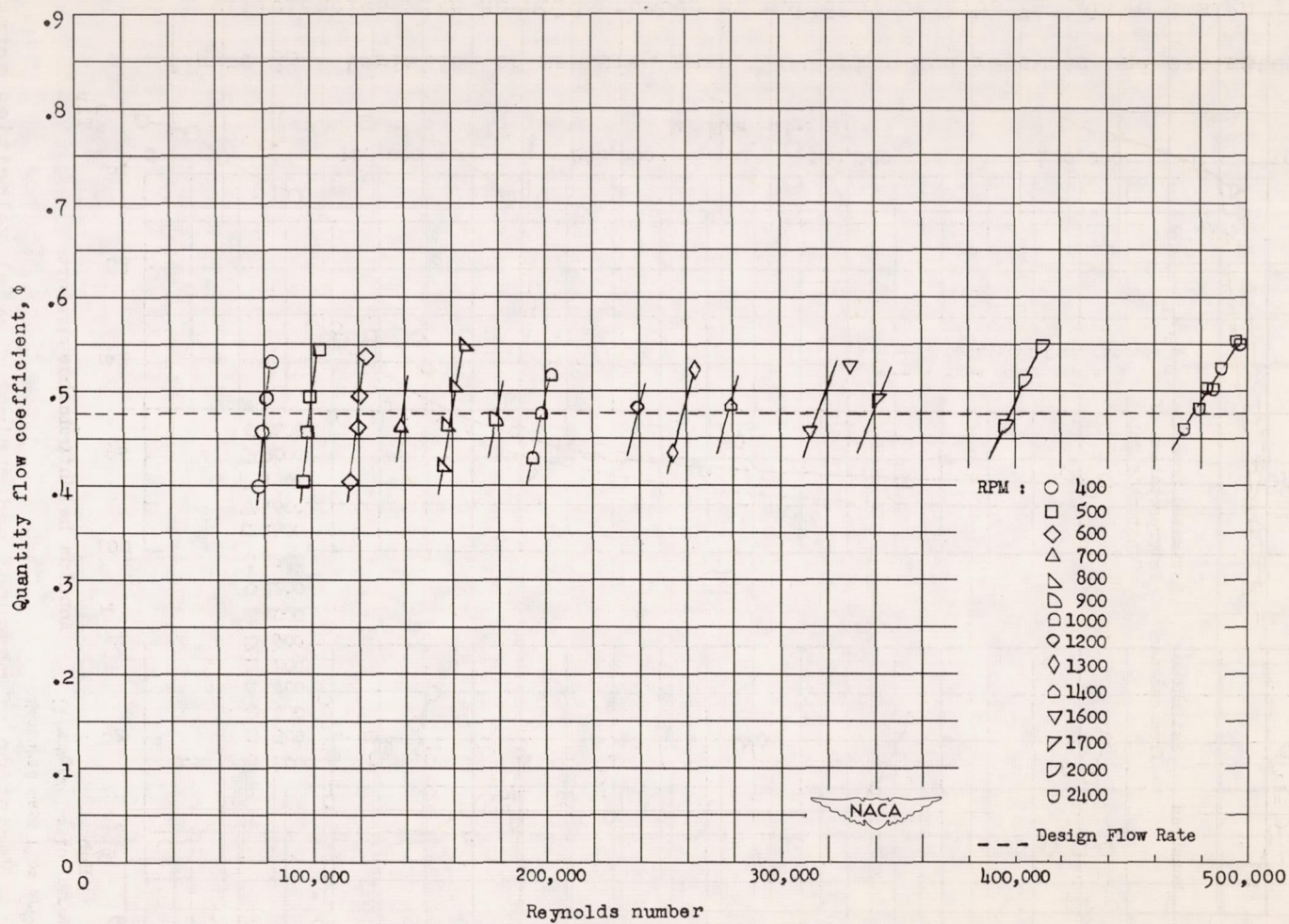
Figure 32.- Relation of Reynolds number effect test points with the design quantity flow coefficient at solidity of 1.0, 7\frac{1}{2}^\circ above design blade angle, and constant annulus area.
