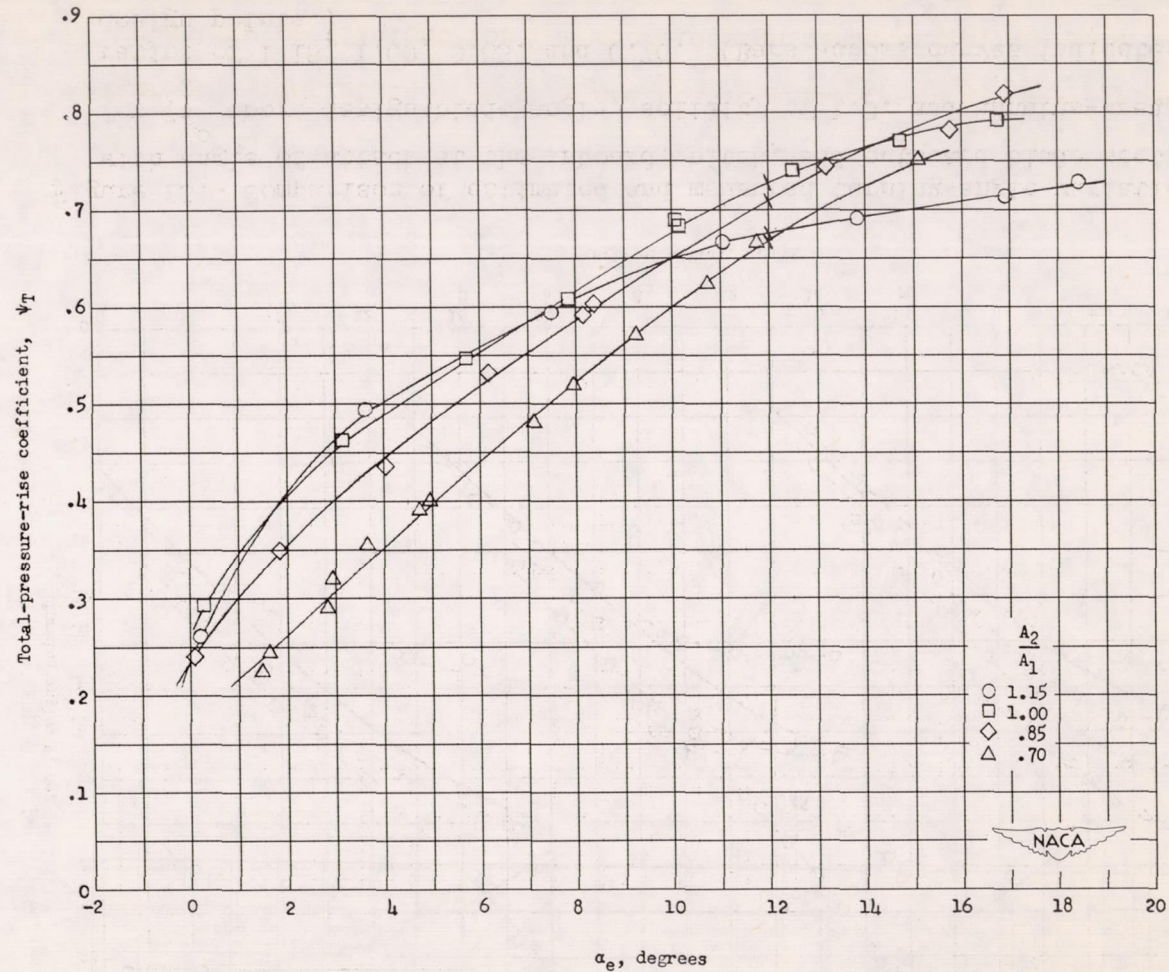
Figure 24.- Variation of total-pressure-rise coefficient \psi_T with effective angle of attack \alpha_e at the pitch diameter for the several annulus-area ratios tested. (Bars across curves indicate design points.)
