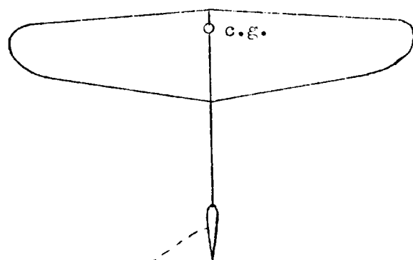
Figure 14.- Representative damping coefficients. C_{n_r} = \frac{\partial C_n}{\partial \frac{rb}{U_0}}
