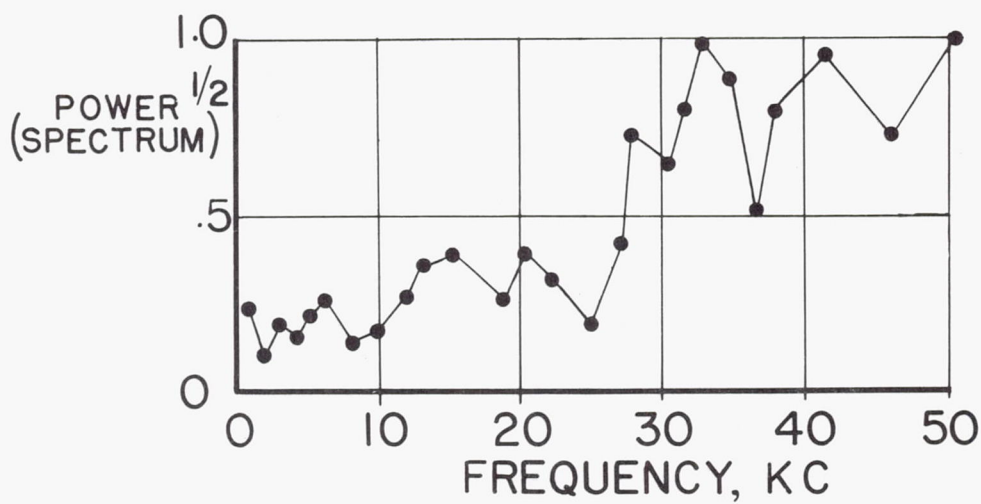
Figure 6.- Transducer response to sound field from a small air jet.
