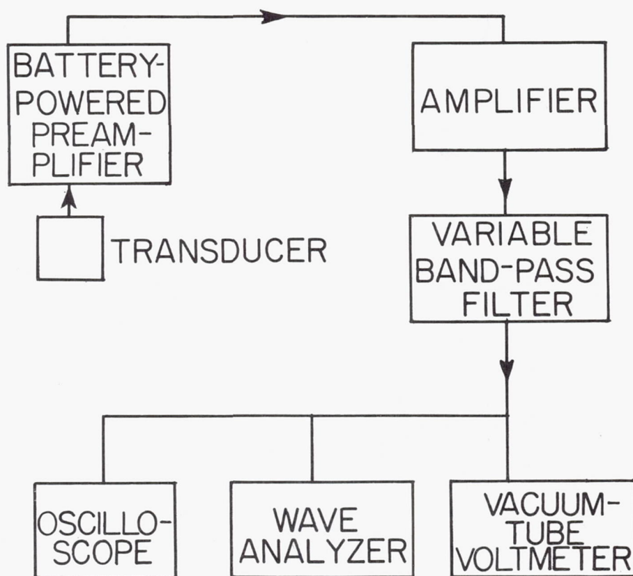
Figure 4.- Block diagram of electronic equipment.
