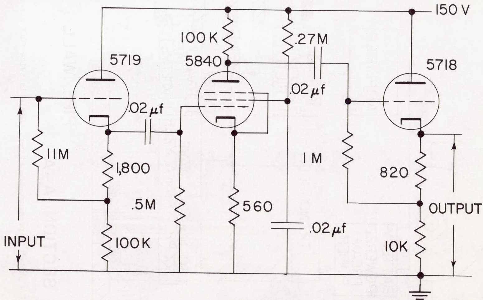
Figure 3.- Preamplifier. Battery powered; gain 50:1. (All resistances are in ohms; K = 1,000 ohms; M = 1,000,000 ohms.)
