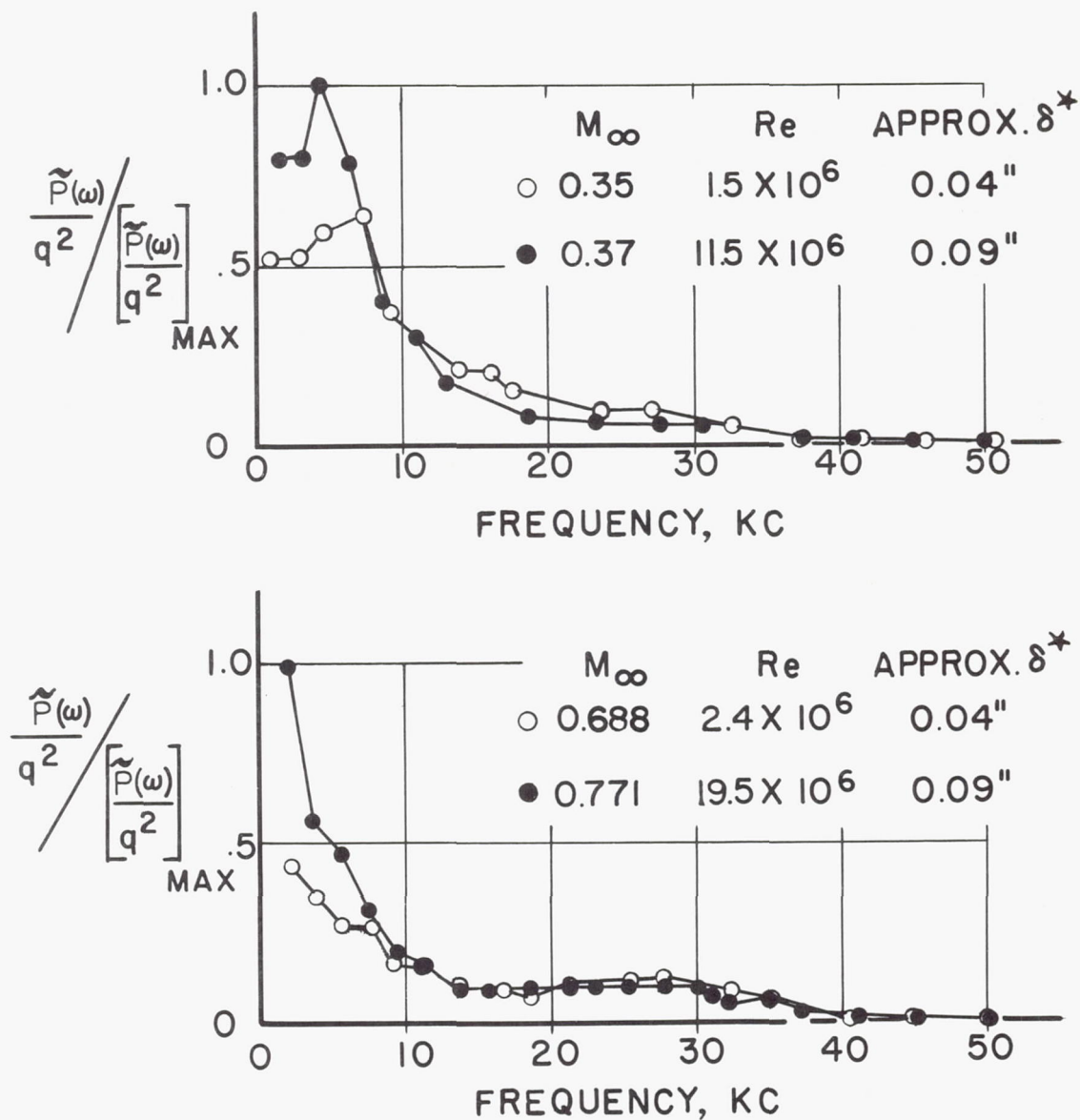
Figure 10.- Effect of boundary-layer displacement thickness on power spectrum of fluctuating pressure.
