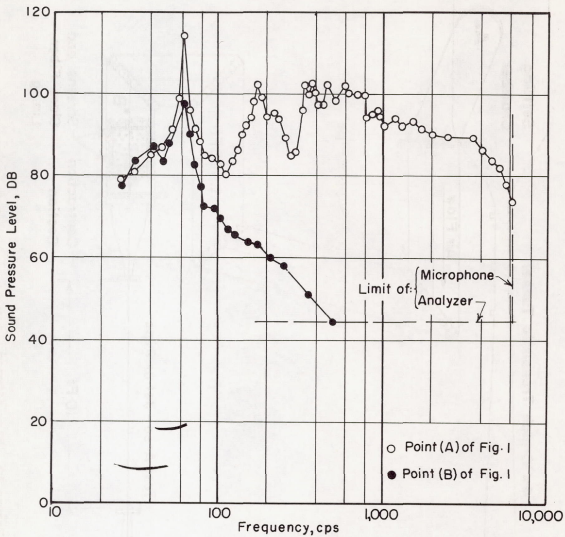
Figure 13.- Sound pressure spectrum in supply pipe.
