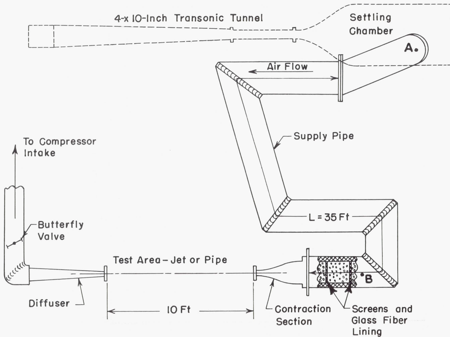
Figure 12.- Flow diagram. Scale: 1 inch = 4 feet.
