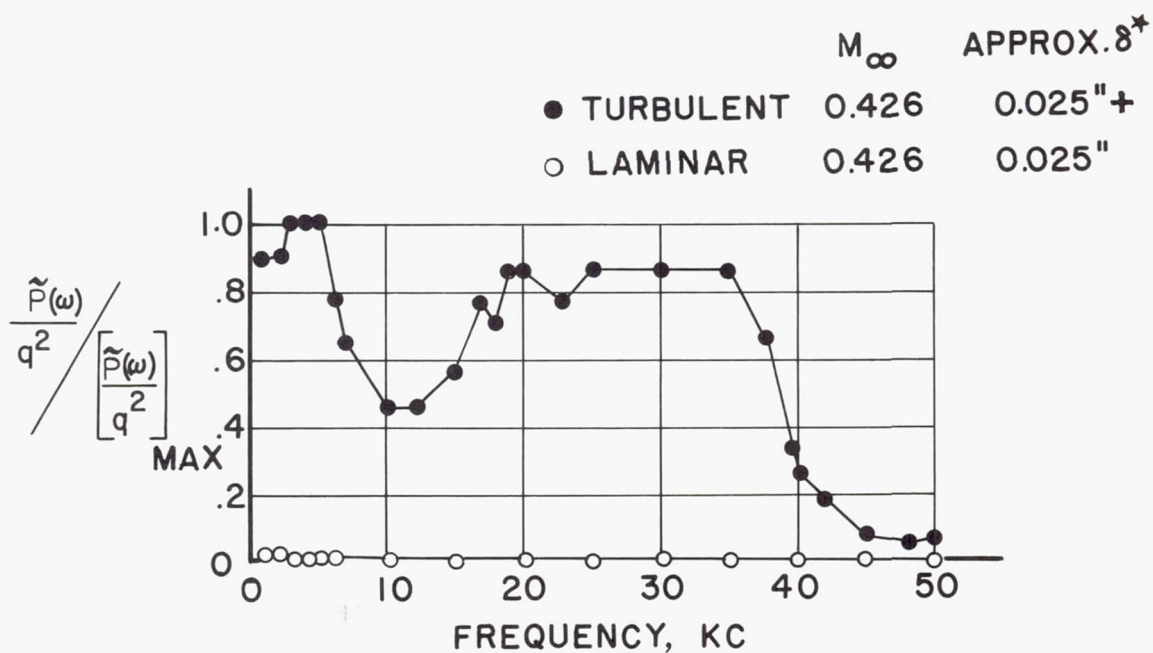
Figure 8.- Effect of boundary-layer tripping on power spectrum of fluctuating pressure.
