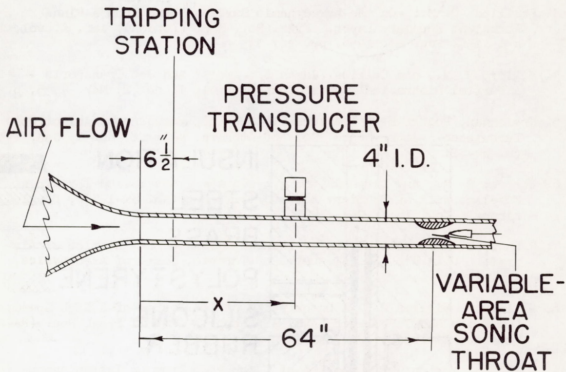
Figure 1.- Sketch of pipe test section.
