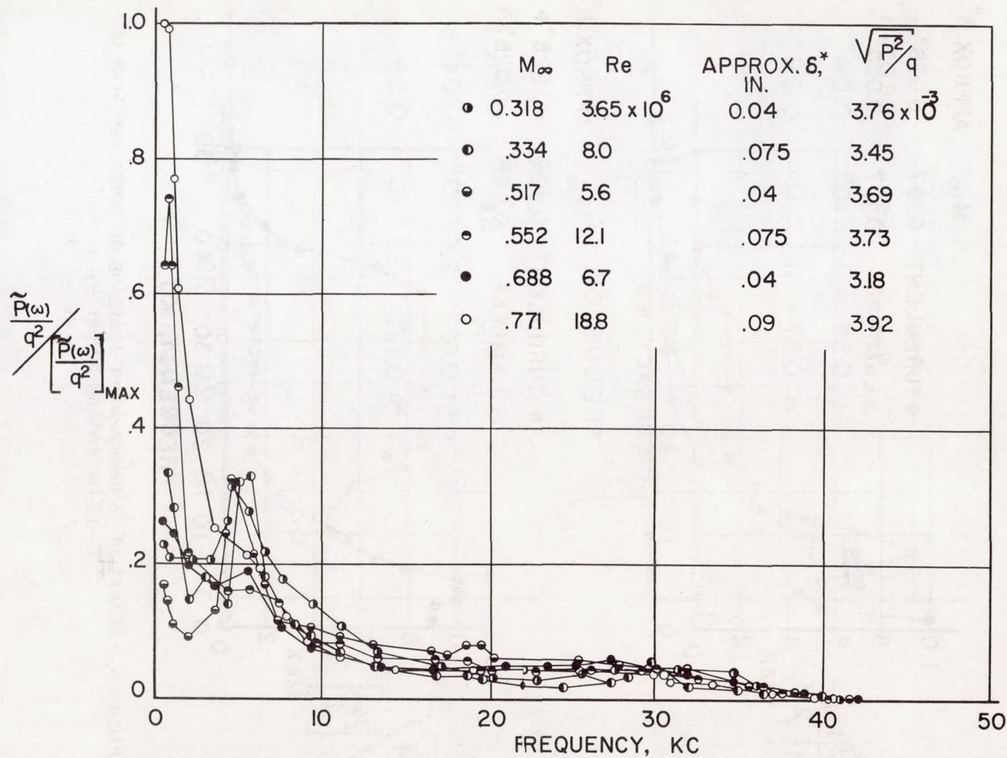
Figure 9.- Typical power spectra of fluctuating pressure.
