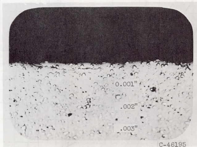
(g) Longitudinal section; X500; 53 \times 10^6 stress cycles (unetched).
