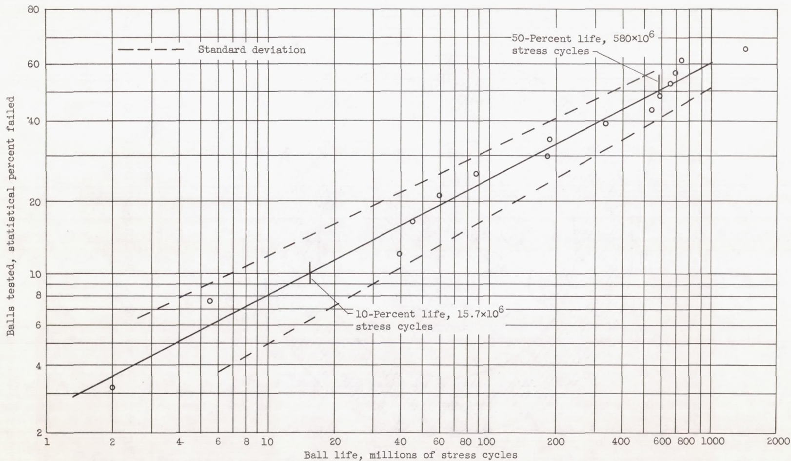
Figure 2. - Fatigue life for 1/2-inch AISI M-1 balls. Lubricant, di(2-ethylhexyl)sebacate; test temperature, 100^\circ F; maximum Hertz compressive stress, 650,000 pounds per square inch.
