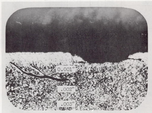
(e) Longitudinal section; X500; 330 \times 10^6 stress cycles.
