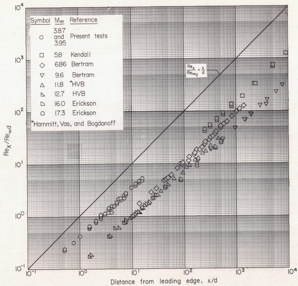
Figure 15.- Comparison of Reynolds number ratio from various sources, see table III.
