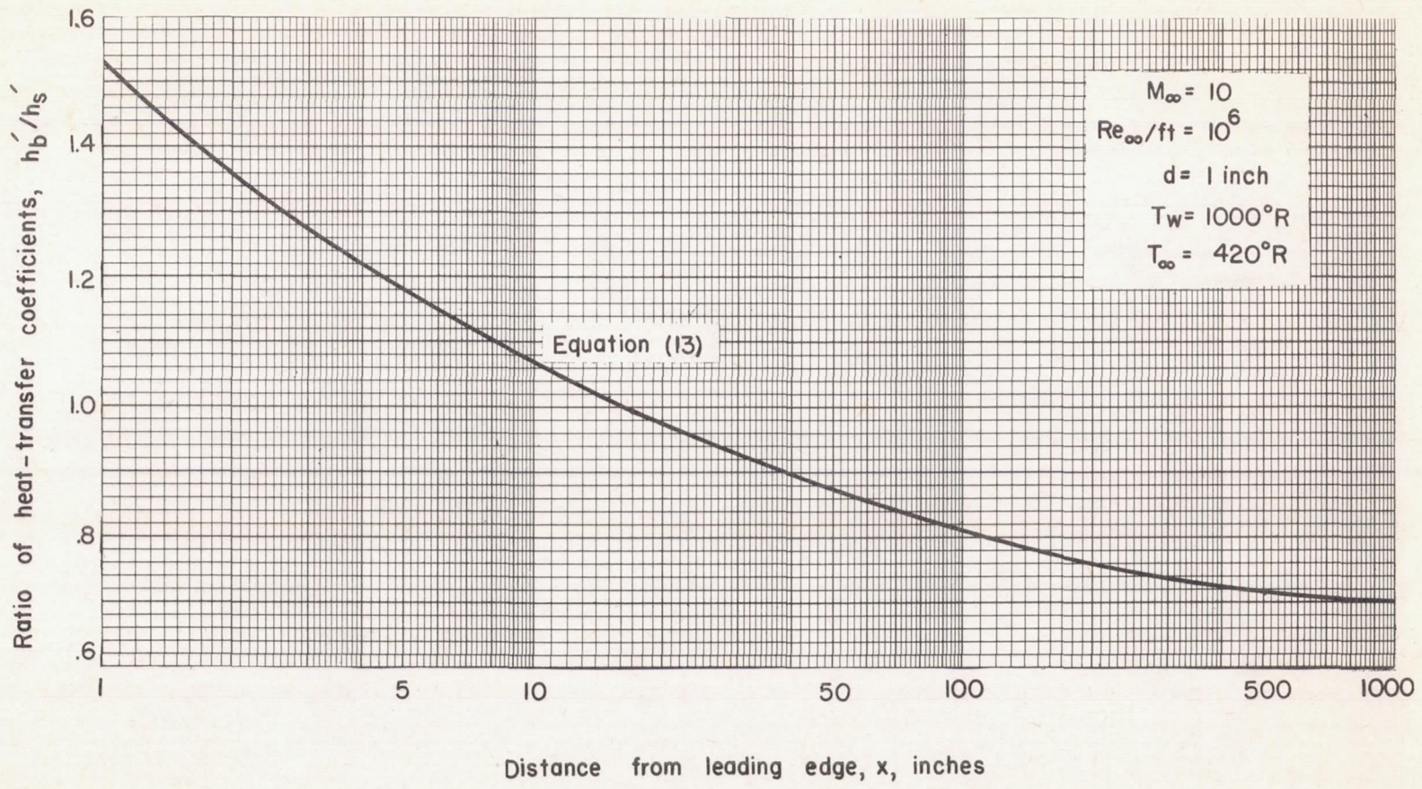
Figure 21.- Effect of blunting on the heat-transfer coefficients calculated for a flat wing for zero angles of attack and yaw at an altitude of 100,000 feet.
