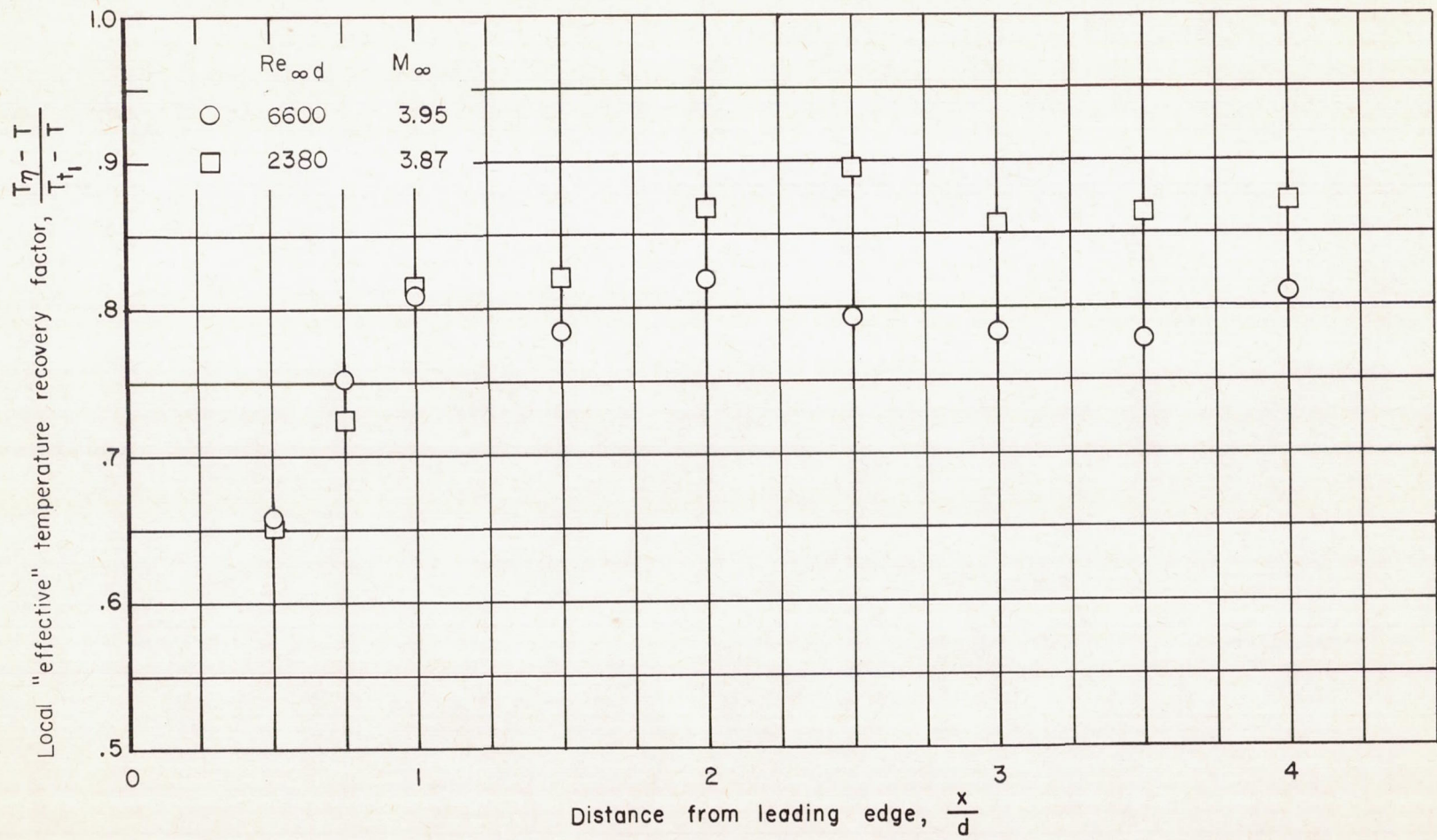
Figure 8.- Variation of the local "effective" temperature recovery factor with distance from the leading edge.
