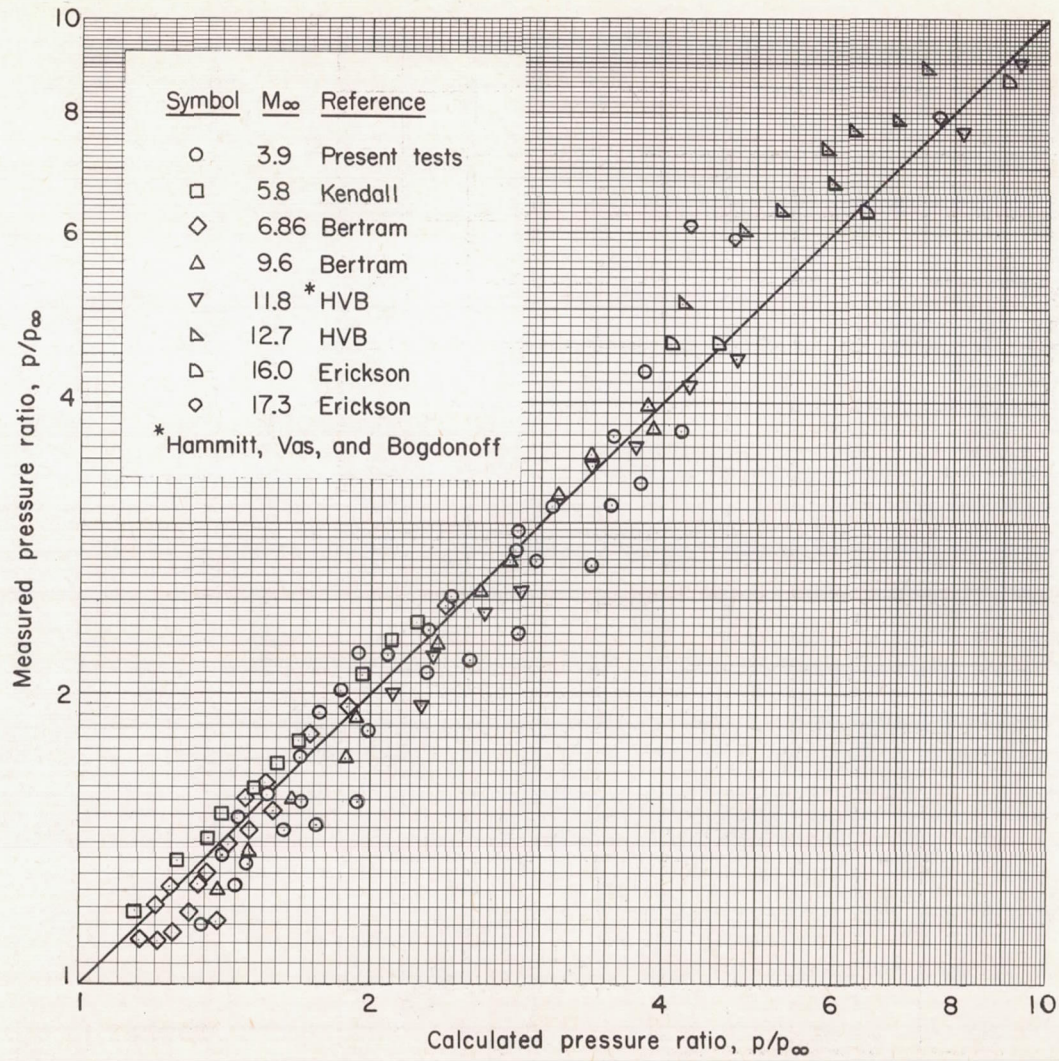
Figure 12.- Comparison of measured pressure ratios with calculated pressure ratios.
