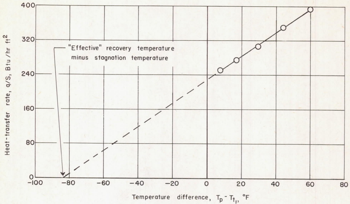
Figure 4.- Variation of heat-transfer rate with difference between surface temperature and stream stagnation temperature for free-stream conditions of M_\infty = 3.95 and Re_{\infty d} = 6600 .
