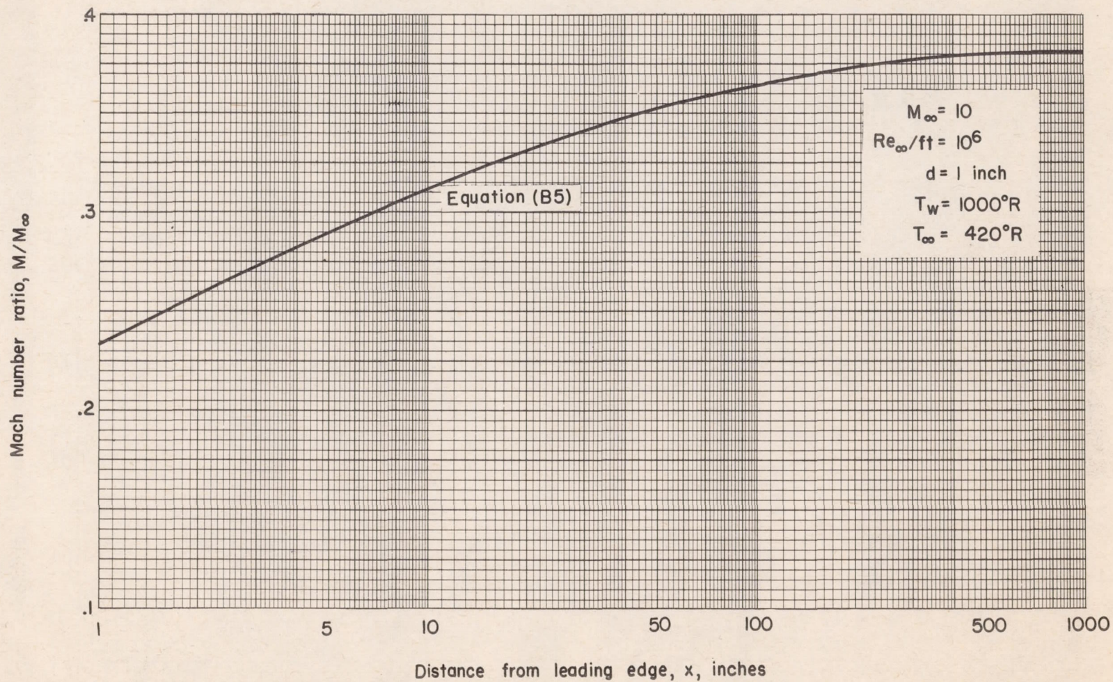
Figure 20.- Mach number ratio calculated for a cylindrically blunted flat wing for zero angles of attack and yaw at an altitude of 100,000 feet.
