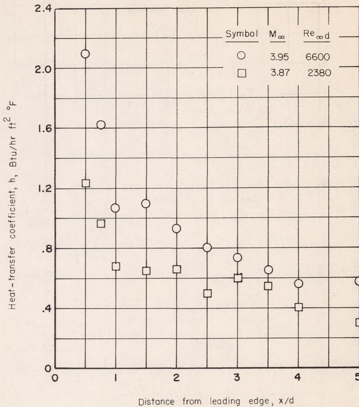
Figure 9.- Variation of heat-transfer coefficients with distance from the leading edge.
