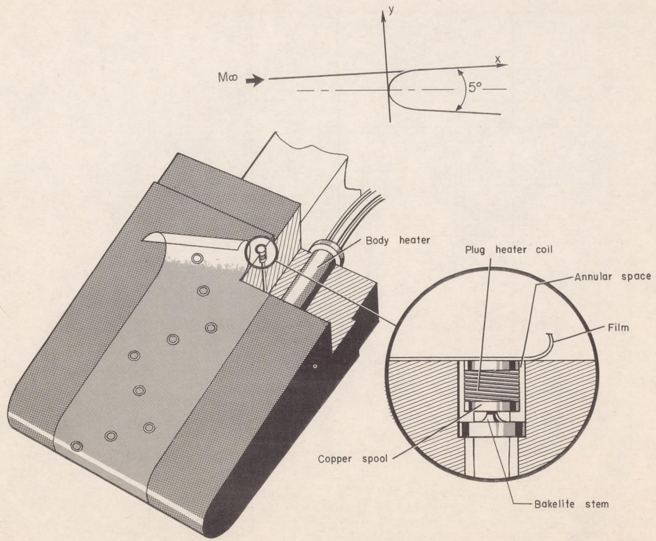
Figure 3.- Heat-transfer body.
