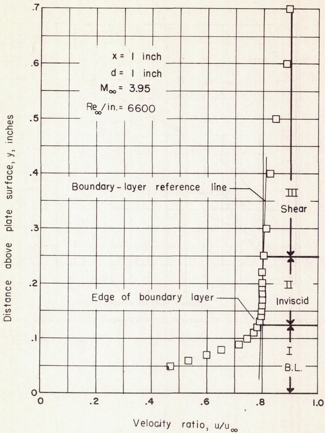
Figure 10.- Variation of the velocity ratio through the boundary layer.
