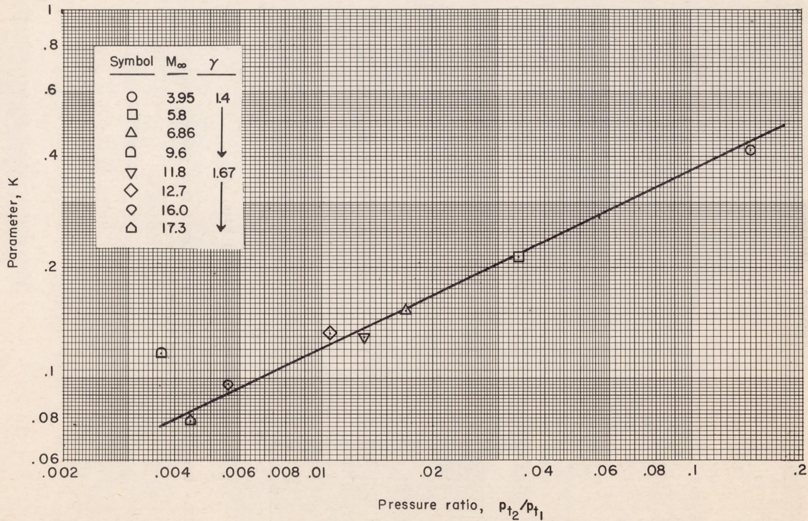
Figure 16.- Variation of the parameter K from various sources with total pressure ratio across a normal leading-edge shock wave.
