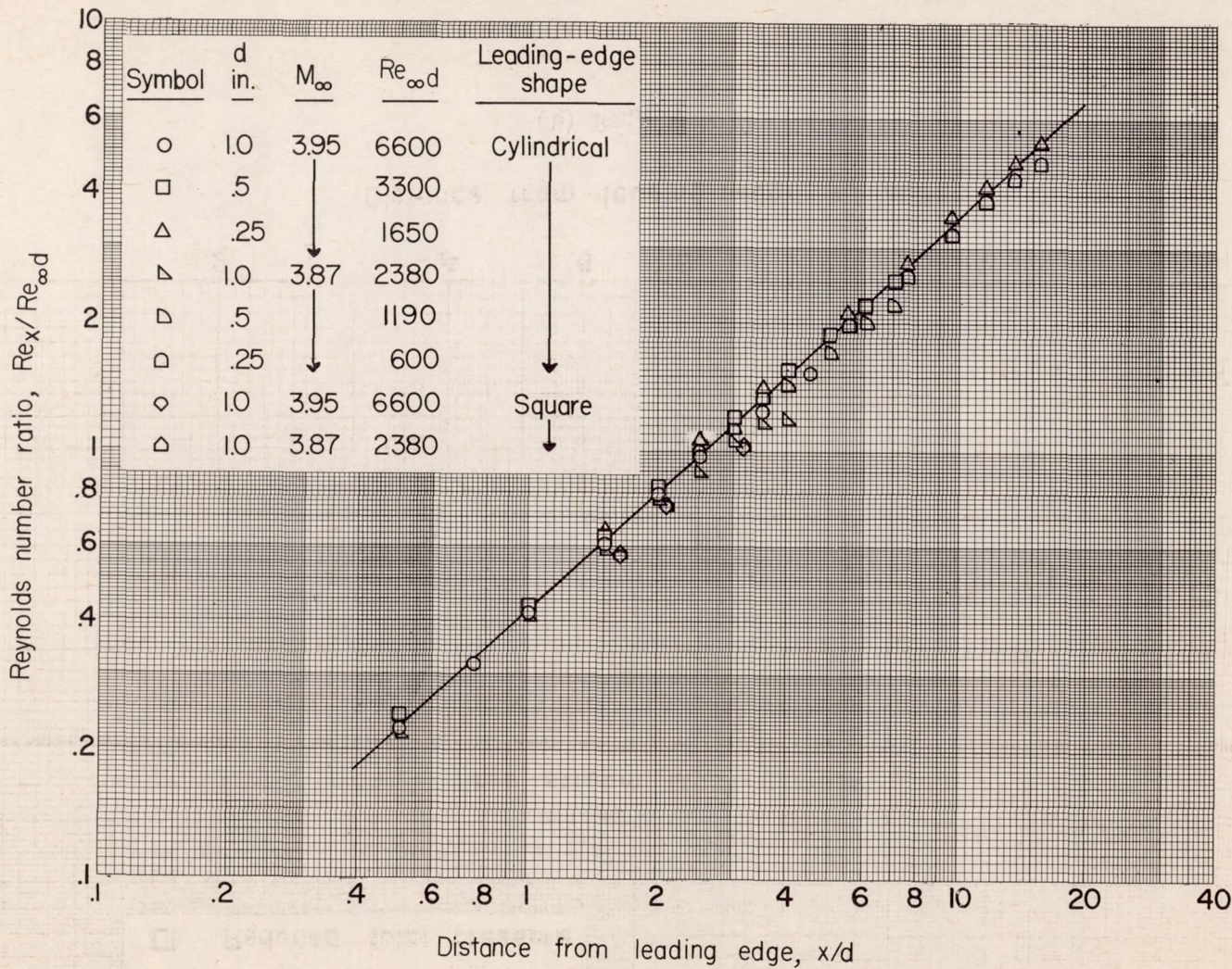
Figure 14.- Variation of the ratio of local Reynolds number at the boundary-layer edge to the free-stream Reynolds number with distance from the leading edge.
