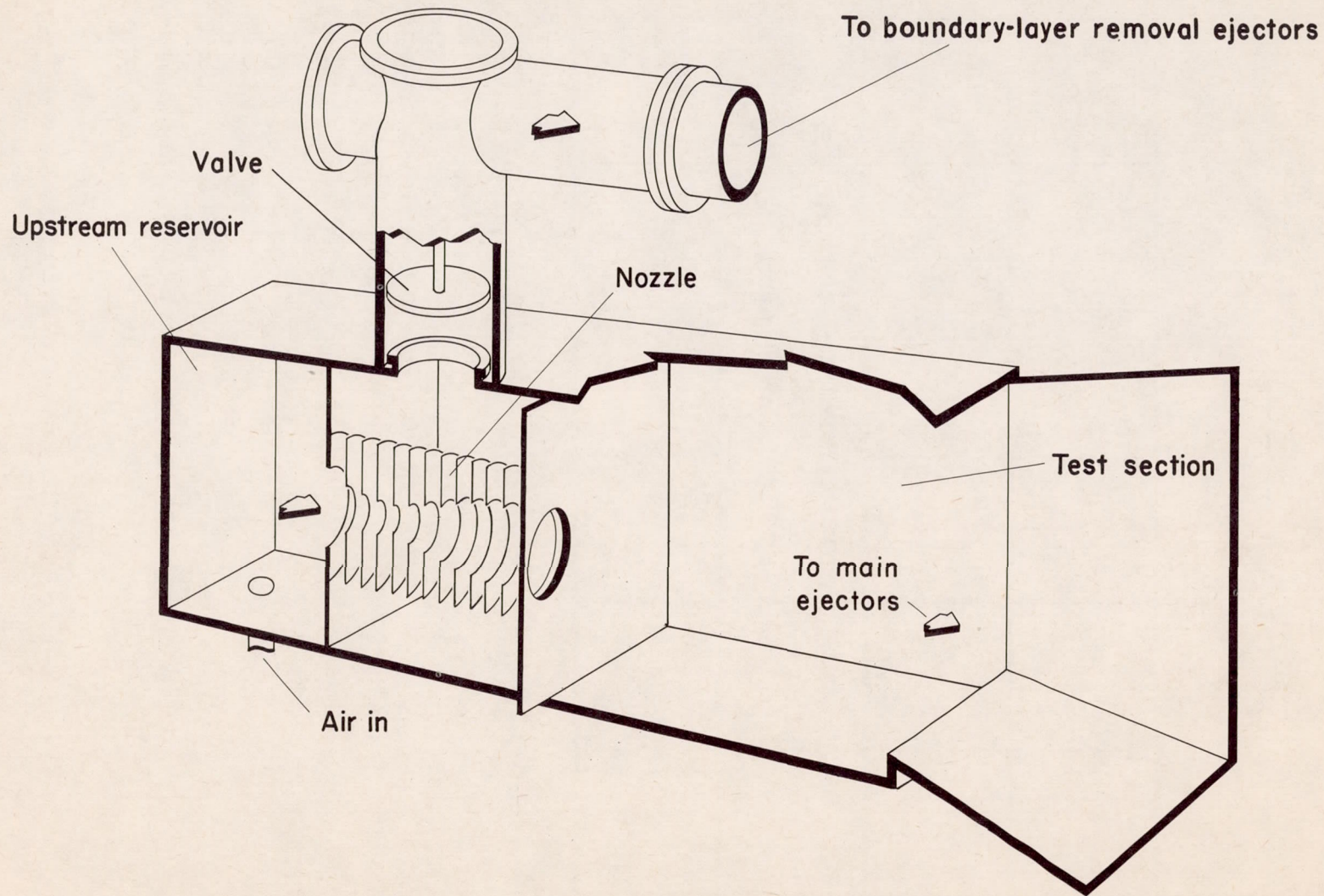
Figure 1.- General arrangement of wind-tunnel test section.
