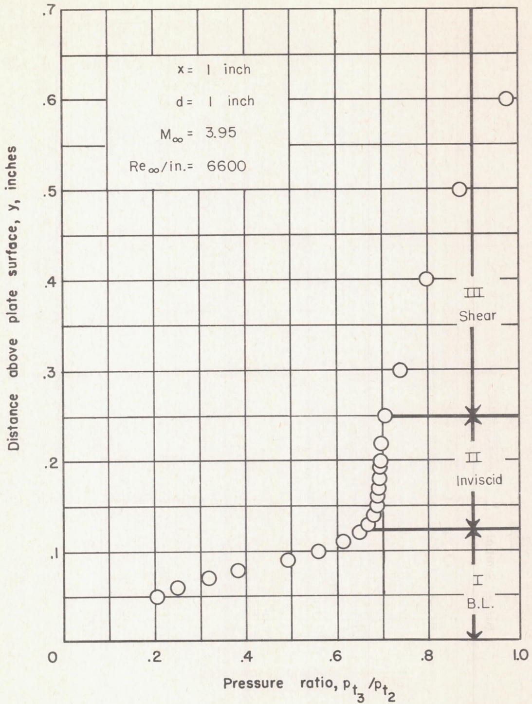
Figure 6.- Variation of the ratio of impact pressure to leading-edge stagnation pressure with distance from the plate surface.
