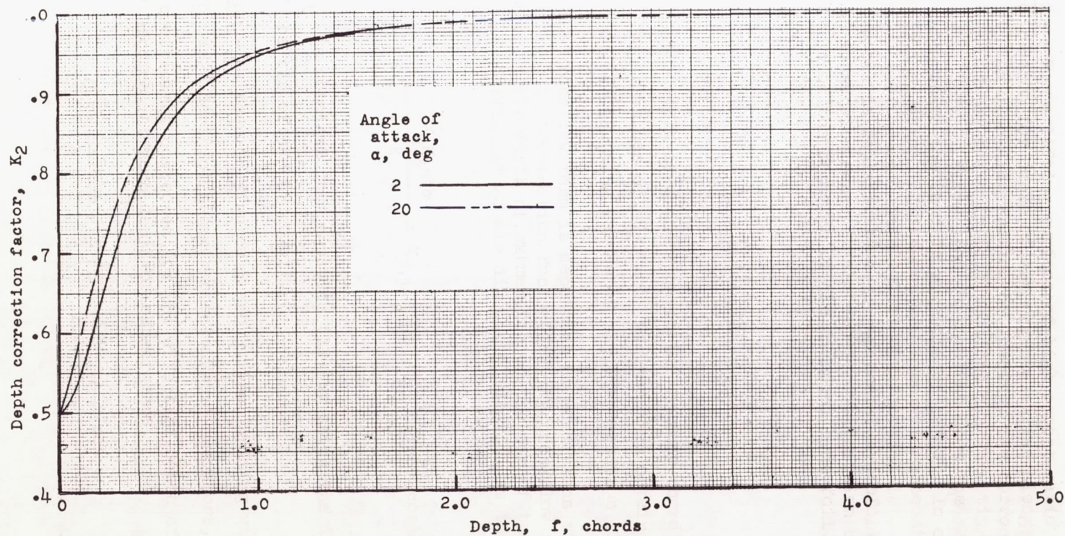
Figure 1.- Variation of the two-dimensional depth correction factor with depth.
