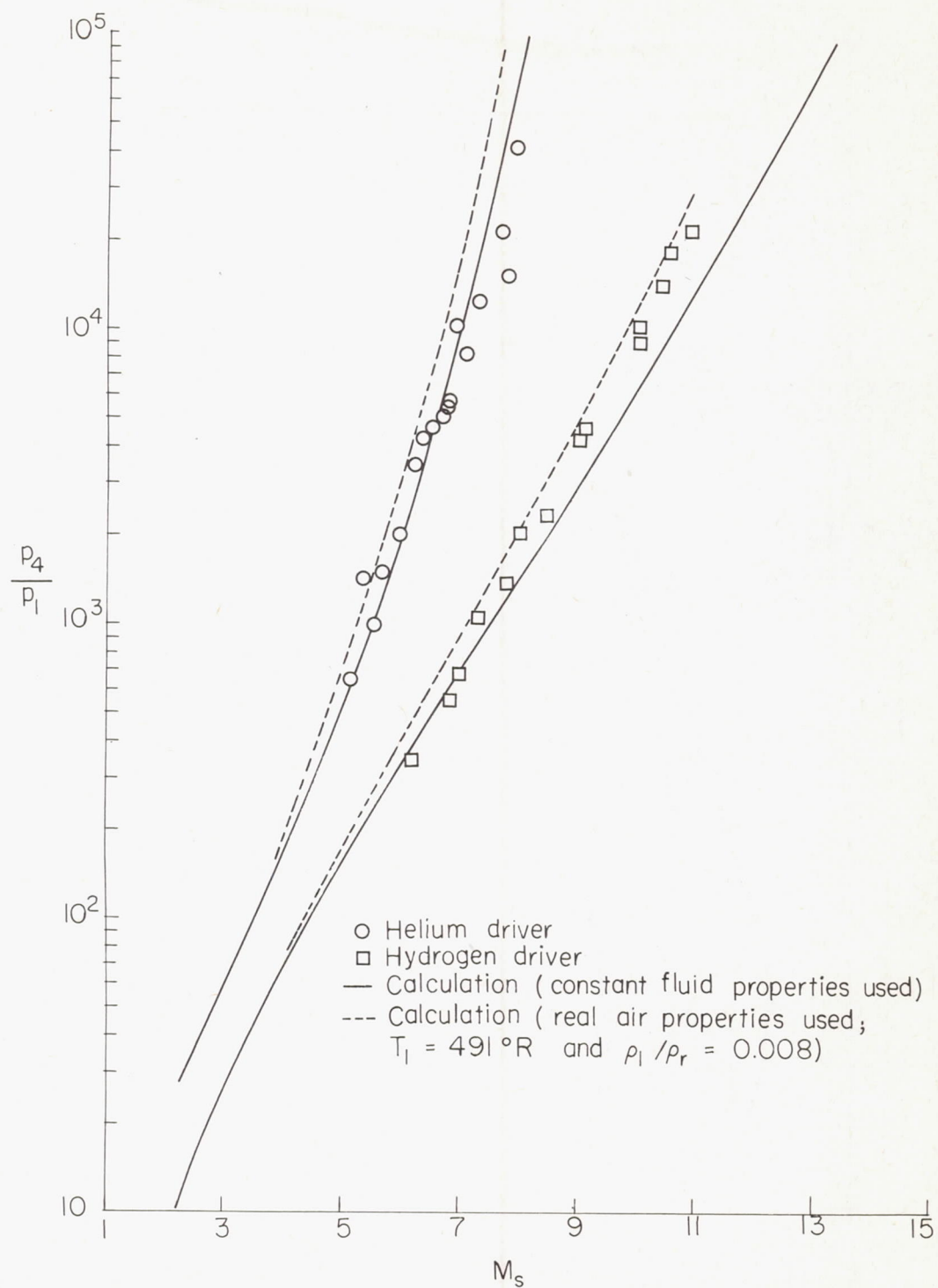
Figure 9.- Comparison of theoretical and experimental shock-wave strengths.
