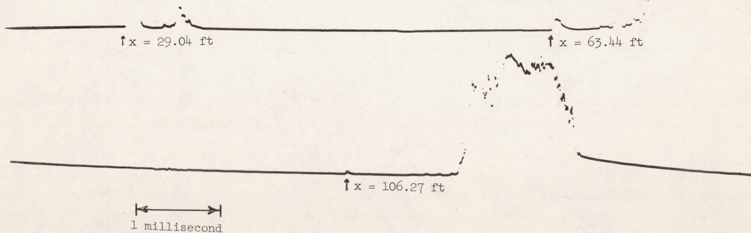
(b) Ionization-gap signals. (Arrow indicates arrival of the shock wave.)
