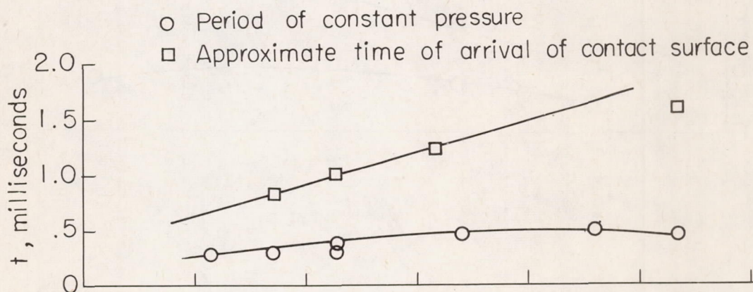
(b) p_1 = 20 millimeters of mercury; p_4/p_1 \approx 1,250 .
