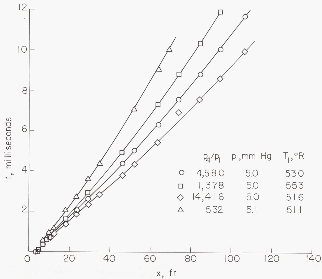
Figure 4.- Typical time-history data of the shock wave.
