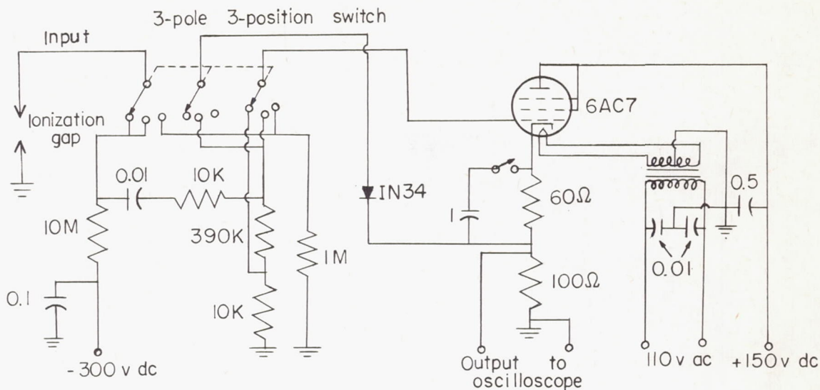
(a) Oscilloscope.
