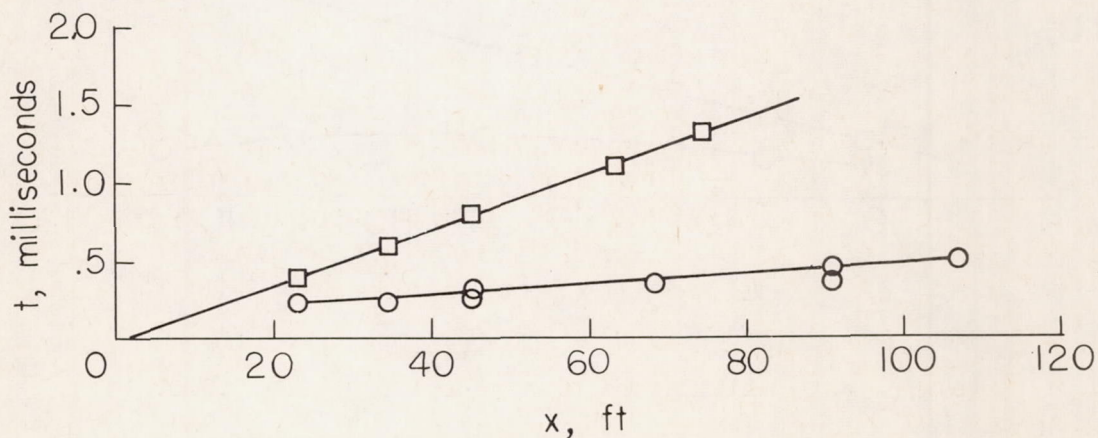
(c) p_1 = 20 millimeters of mercury; p_4/p_1 \approx 2,500 .
