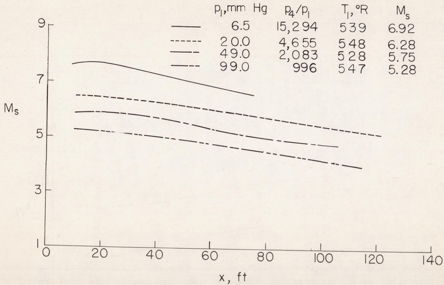
Figure 6.- Typical shock-wave attenuation data with helium as driver gas.
