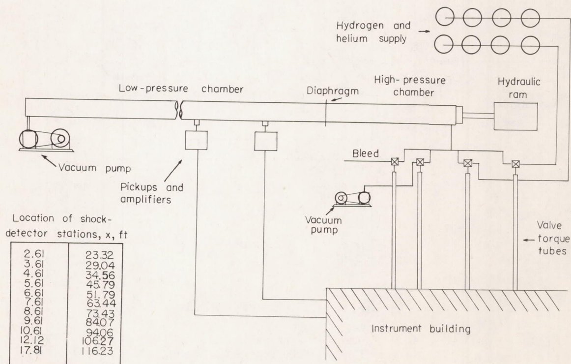
Figure 1.- Shock-tube layout.
