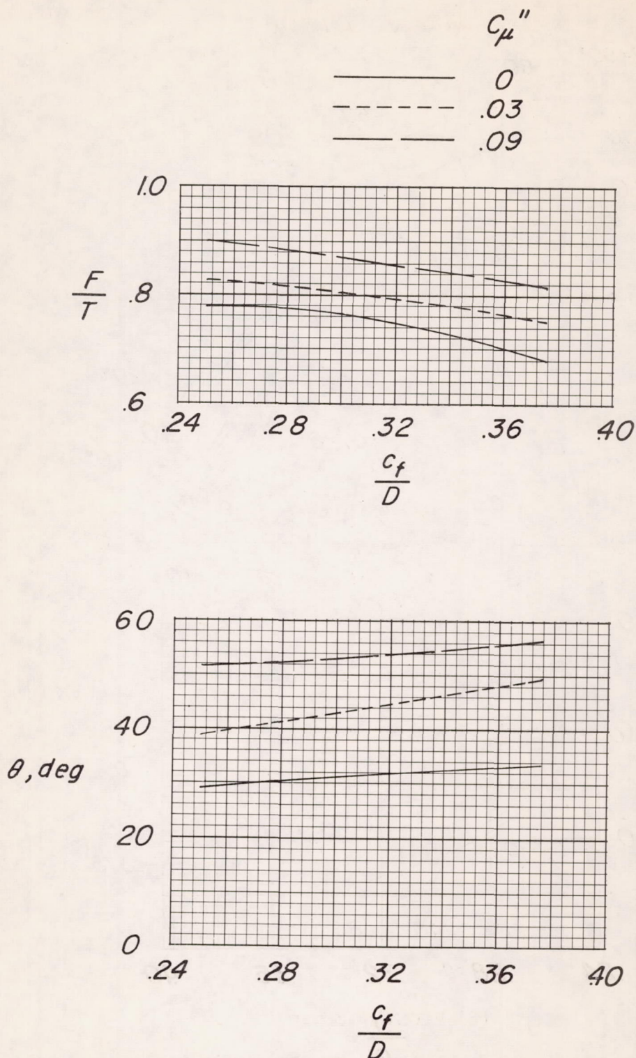
Figure 24.- Effect of ratio of flap chord to propeller diameter on the ratio of resultant force to thrust and turning angle for a range of momentum coefficients. \delta_{f,1} = 60^\circ ; \delta_{f,2} = 30^\circ ; h/D \approx \infty .
