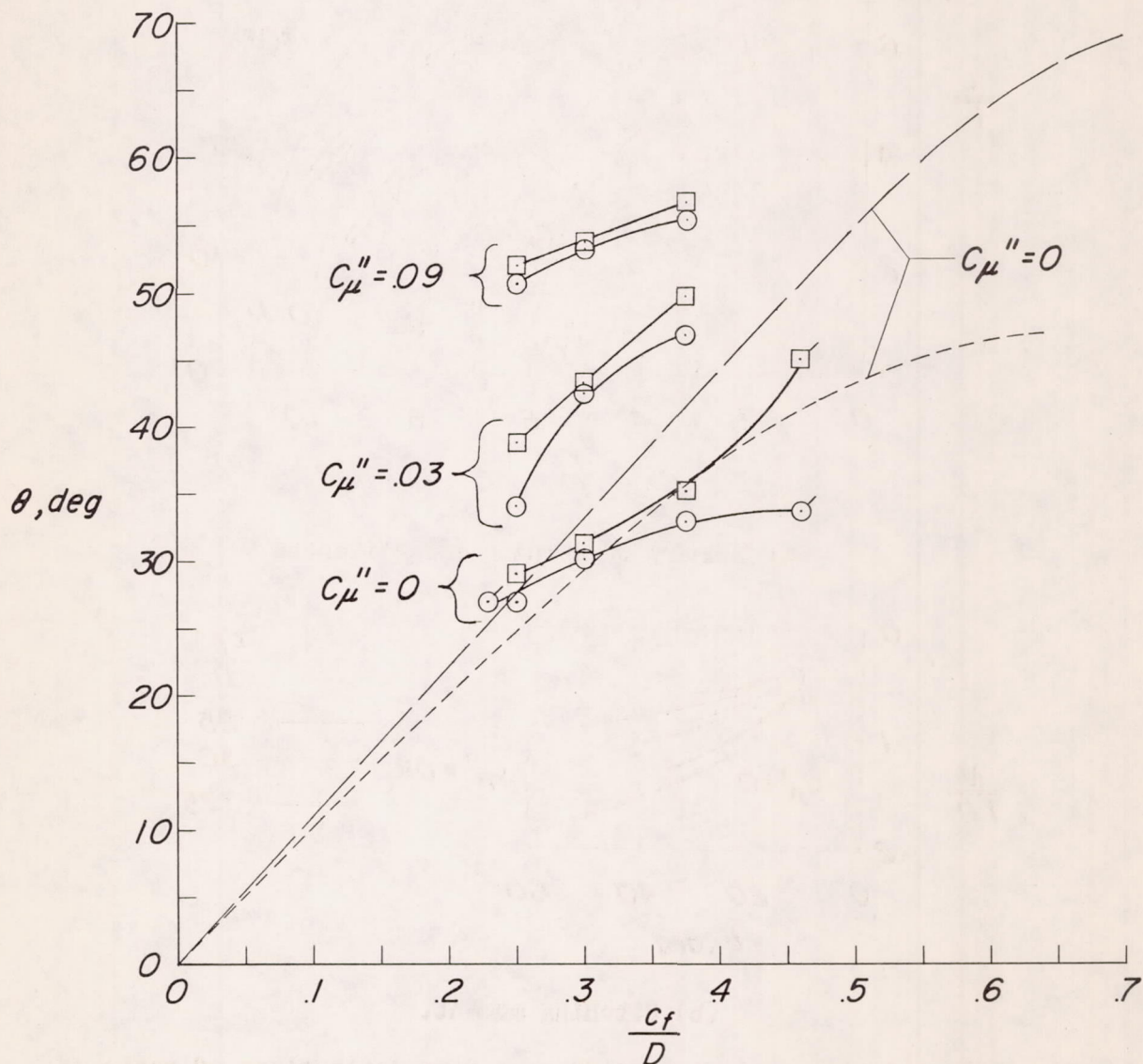
Figure 26.- Average variation of turning angle with ratio of flap chord to propeller diameter.
