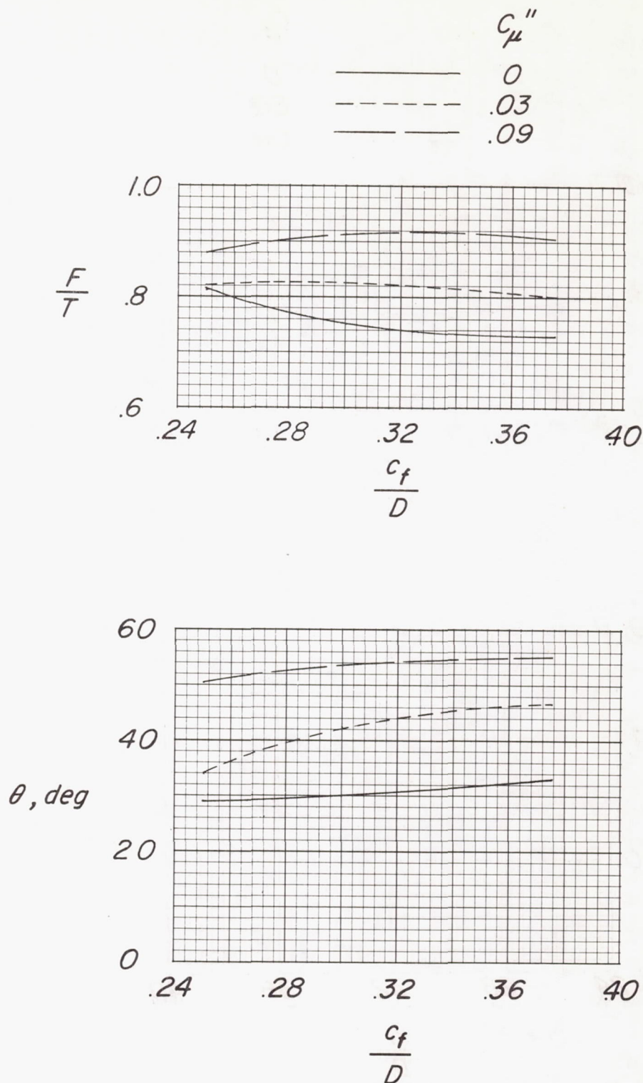
Figure 23.- Effect of ratio of flap chord to propeller diameter on the ratio of resultant force to thrust and turning angle for a range of momentum coefficients. \delta_{f,1} = 70^\circ ; \delta_{f,2} = 0^\circ ; h/D \approx \infty .
