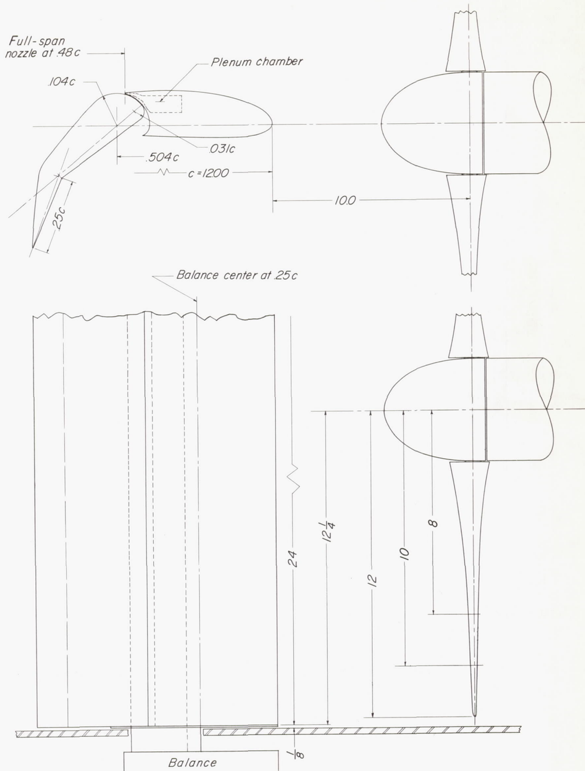
Figure 2.- Drawing of model. Dimensions are in inches unless otherwise indicated.
