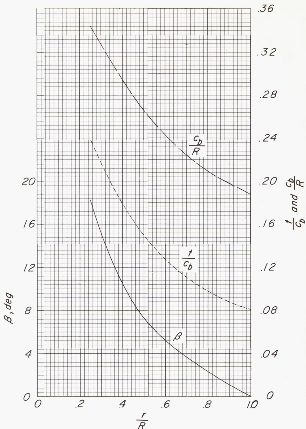
Figure 6.- Physical characteristics of 1.33-foot-diameter propeller with Clark Y airfoil section. \eta = 0.62 .
