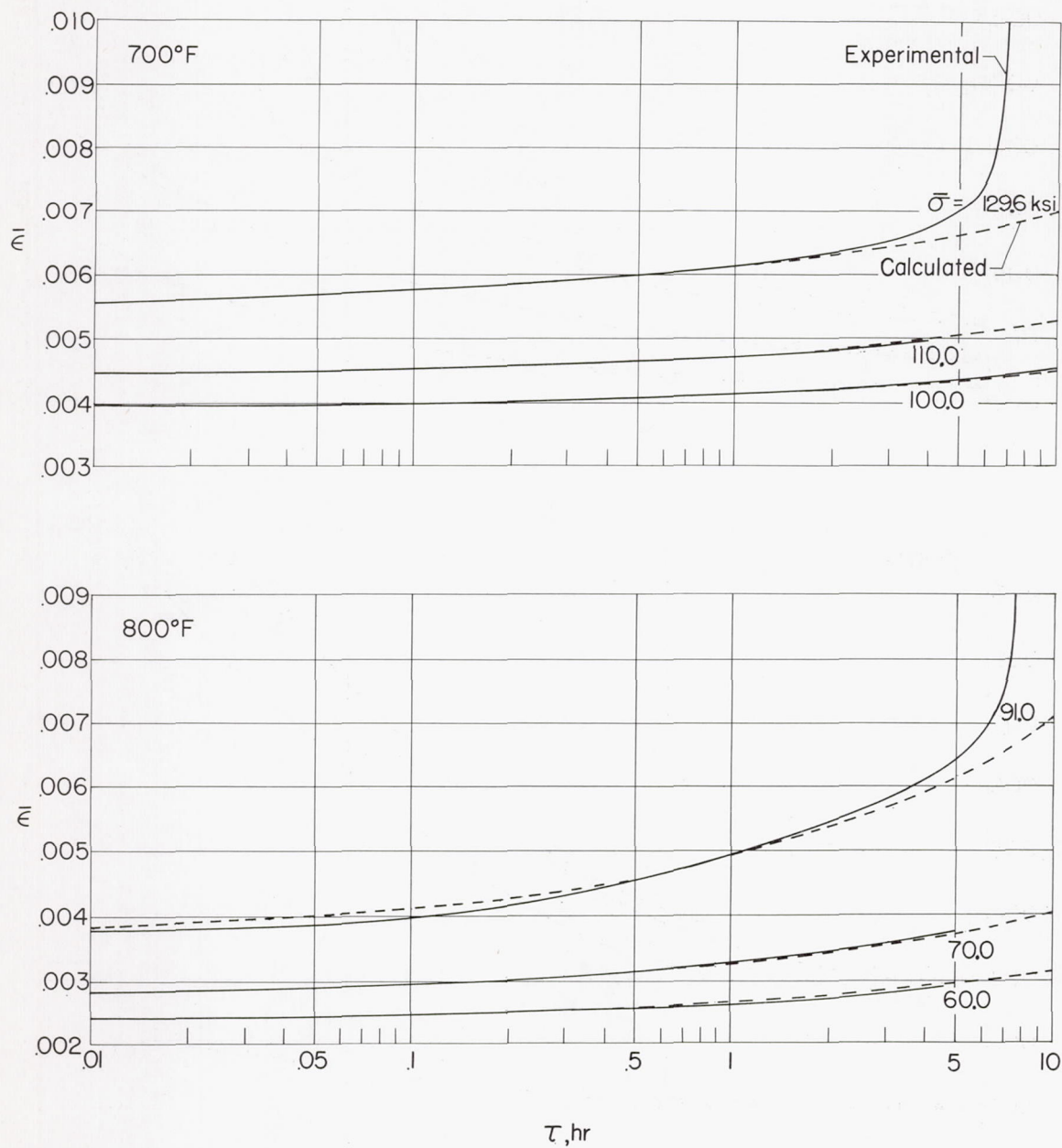
Figure 11.- Experimental material creep curves for 17-7 PH stainless steel, Condition TH 1,050, compared with creep curves calculated from equation (3).
