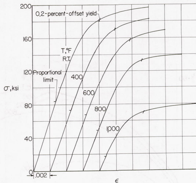
Figure 4.- Compressive stress-strain curves for 17-7 PH stainless-steel sheet, Condition TH 1,050. Strain rate, 0.002 per minute; \frac{1}{2} -hour exposure to temperature.
