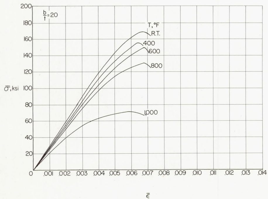
Figure 3.- Average stress against unit shortening for 17-7 PH stainless-steel plates, Condition TH 1,050; \frac{1}{2} -hour exposure to temperature.
