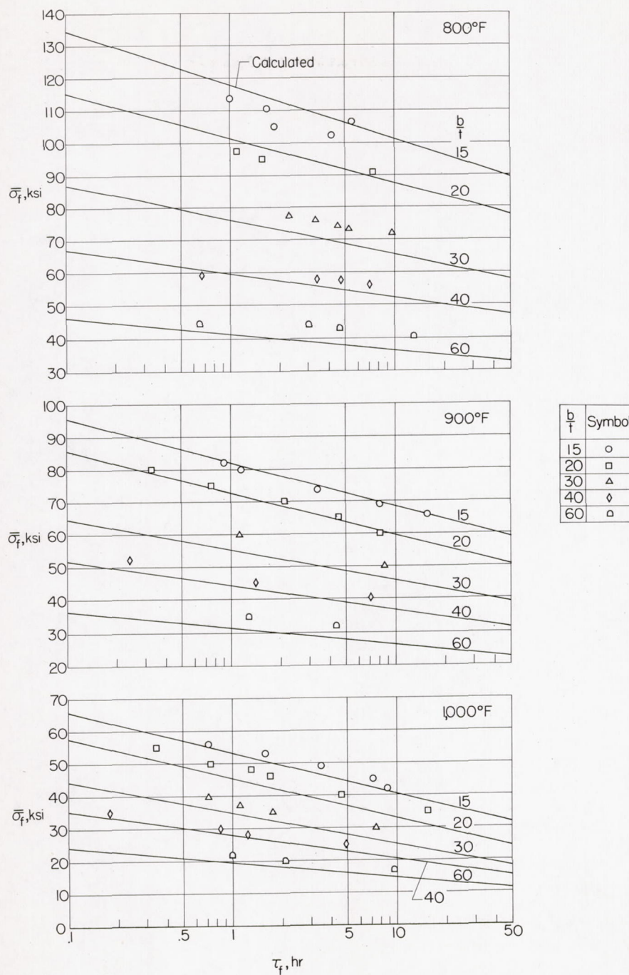
Figure 13.- Comparison of experimental and calculated compressive creep failure stresses for 17-7 PH stainless-steel plates, Condition TH 1,050.
