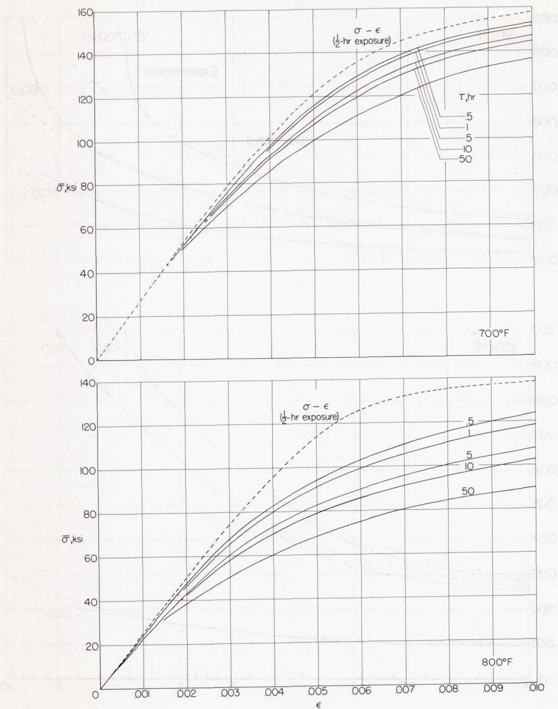
Figure 12.- Isochronous stress-strain curves for 17-7 PH stainless-steel sheet, Condition TH 1,050.
