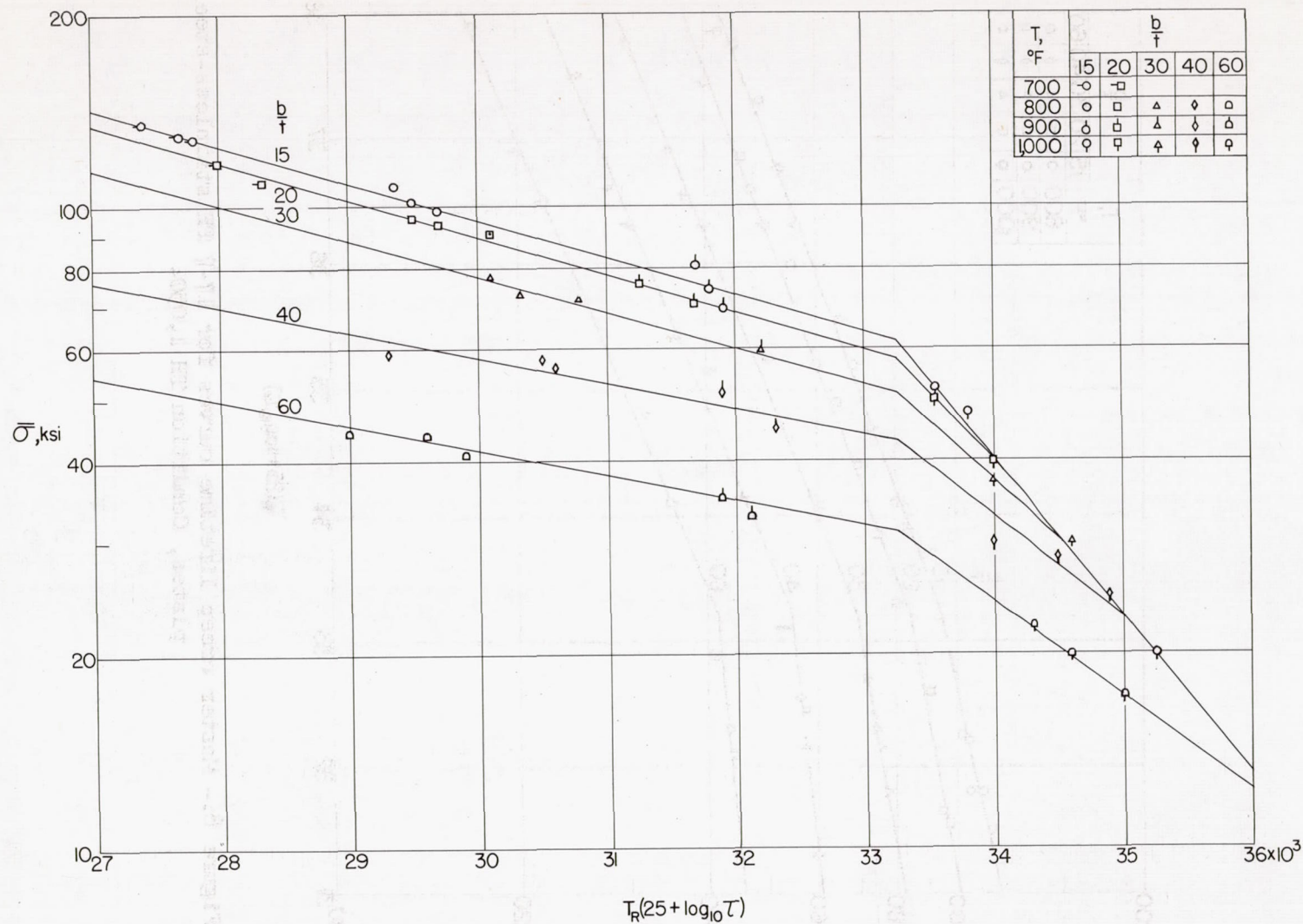
Figure 9.- Stresses at which a creep strain of 0.0002 was attained in 17-7 PH stainless-steel plates, Condition TH 1,050, for various combinations of time and temperature.
