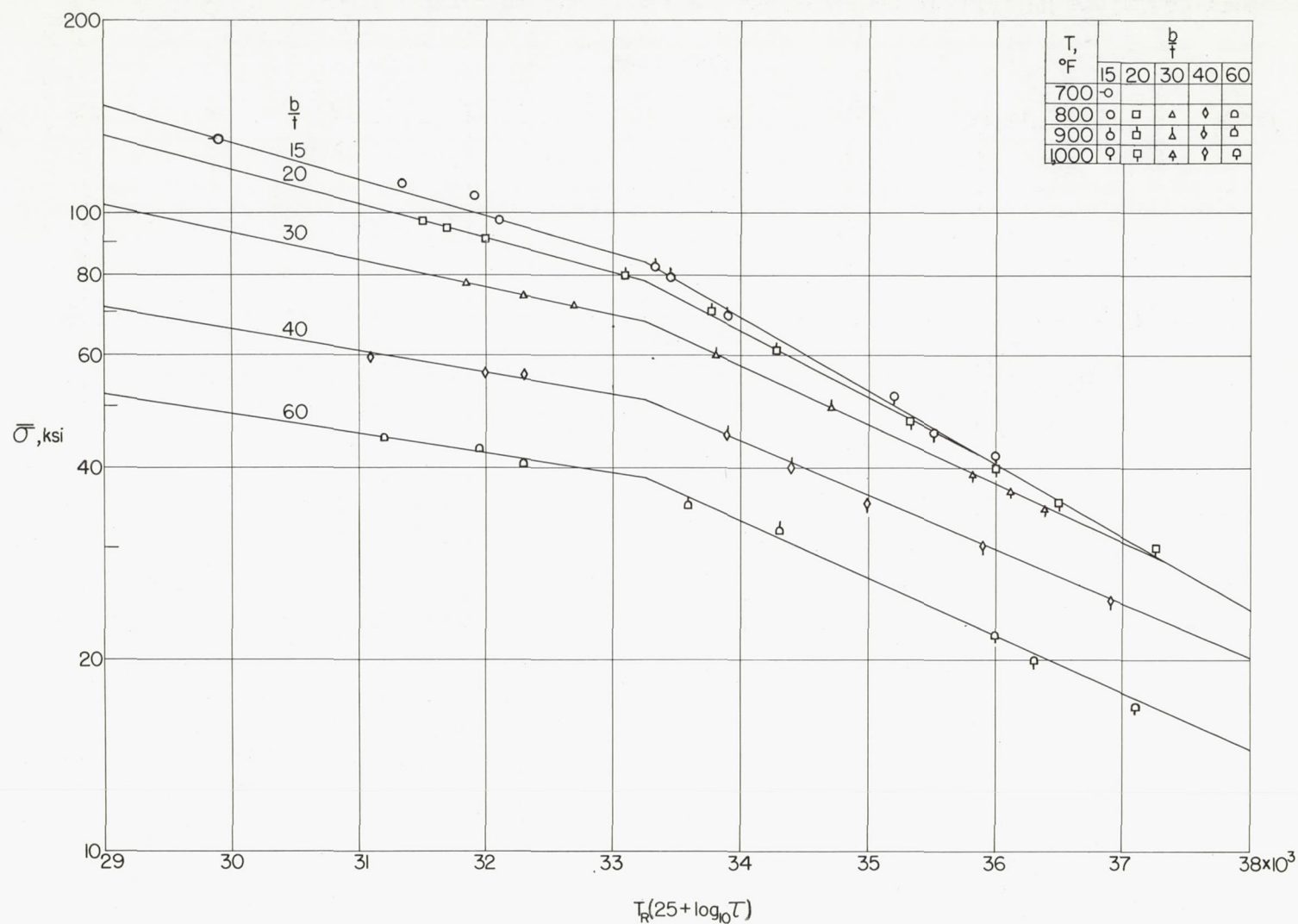
Figure 10.- Stresses at which a creep strain of 0.002 was attained in 17-7 PH stainless-steel plates, Condition TH 1,050, for various combinations of time and temperature.
