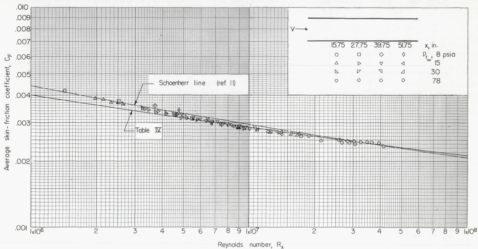
Figure 12.- Variation of average skin-friction coefficient with change in Reynolds number, R_x ; boundary-layer velocity profile measurements.
