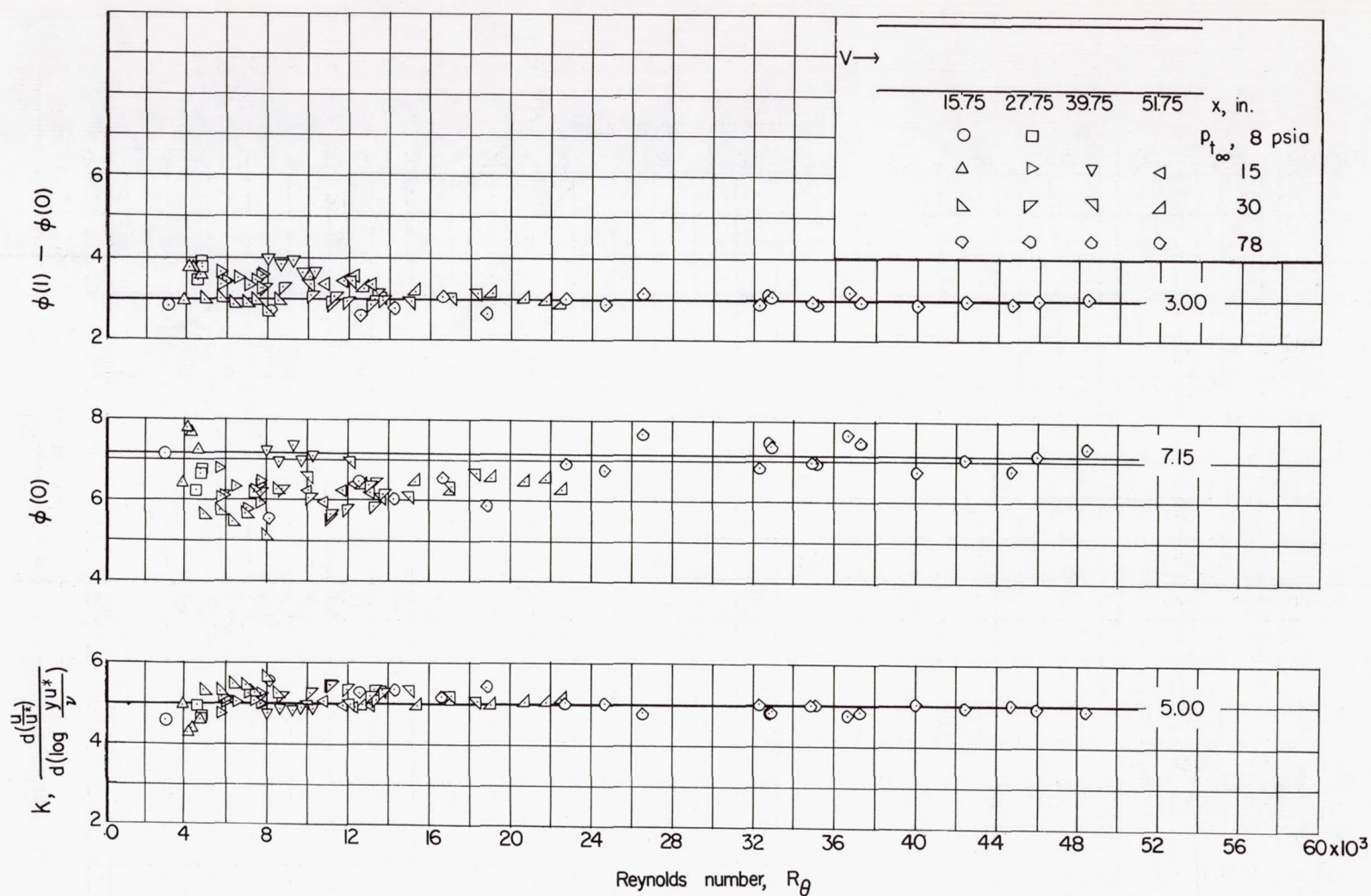
Figure 16.- Variation of K , \phi(0) , and \phi(1) - \phi(0) with change in Reynolds number, R_\theta .
