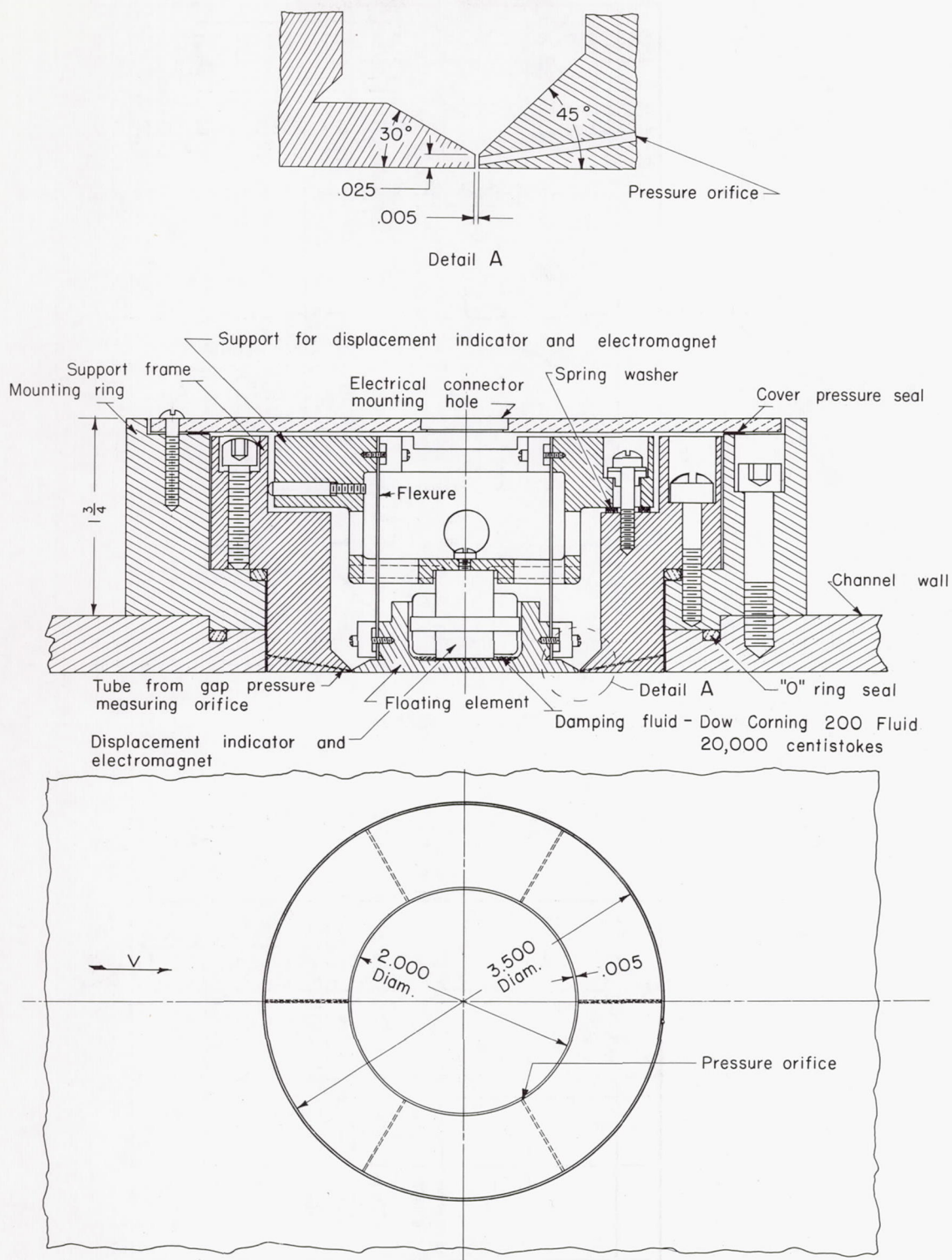
Figure 5.- Details of the floating-element skin-friction balance.
