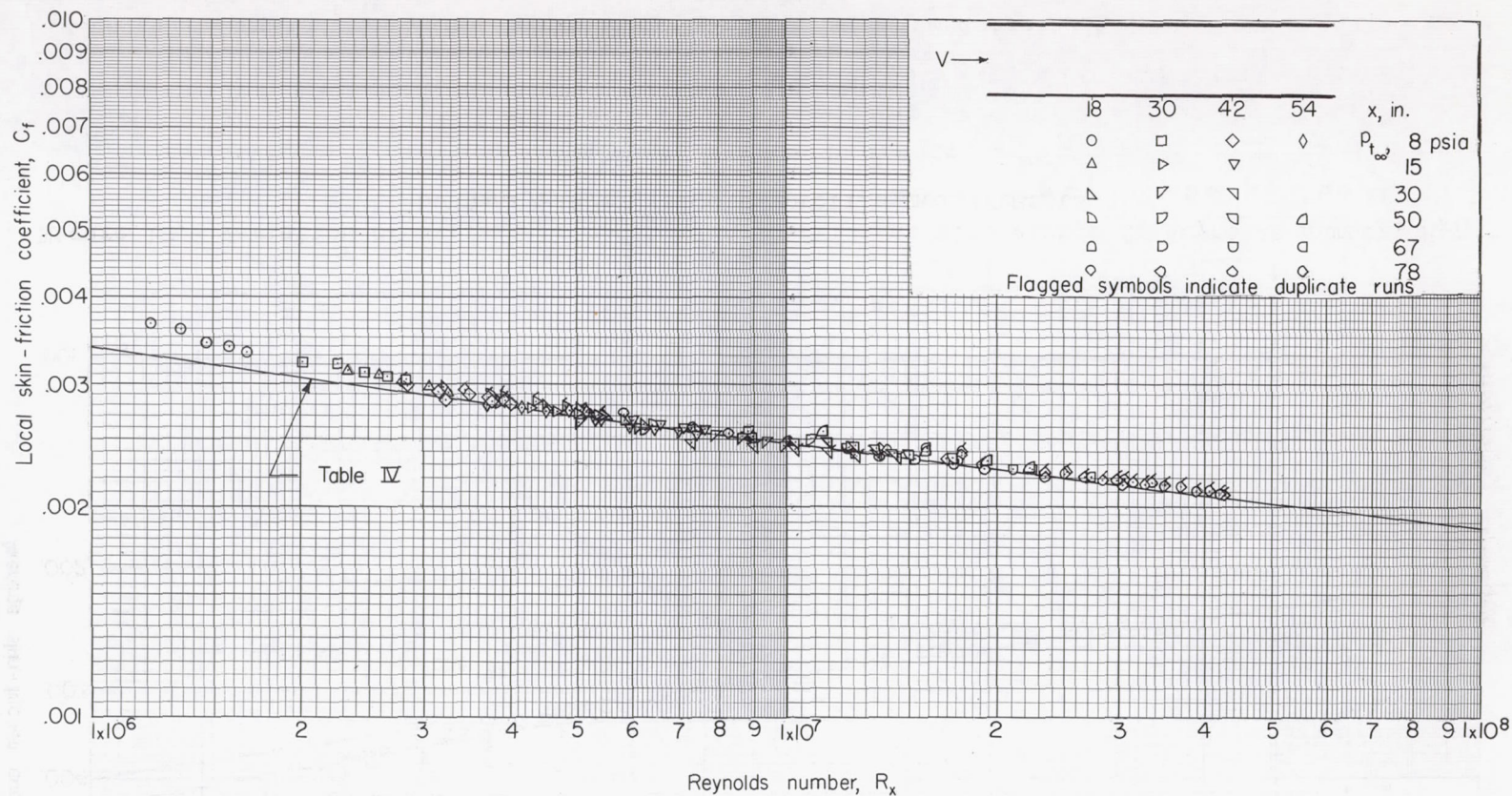
Figure 13.- Variation of local skin-friction coefficient with change in Reynolds number, R_x ; floating-element technique.
