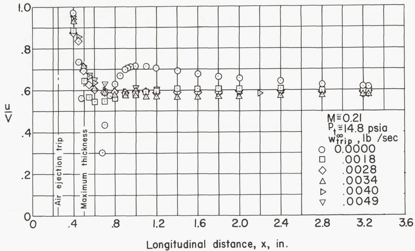
Figure 8.- Effect of varying quantity of boundary-layer-trip air on local velocity near channel wall.
