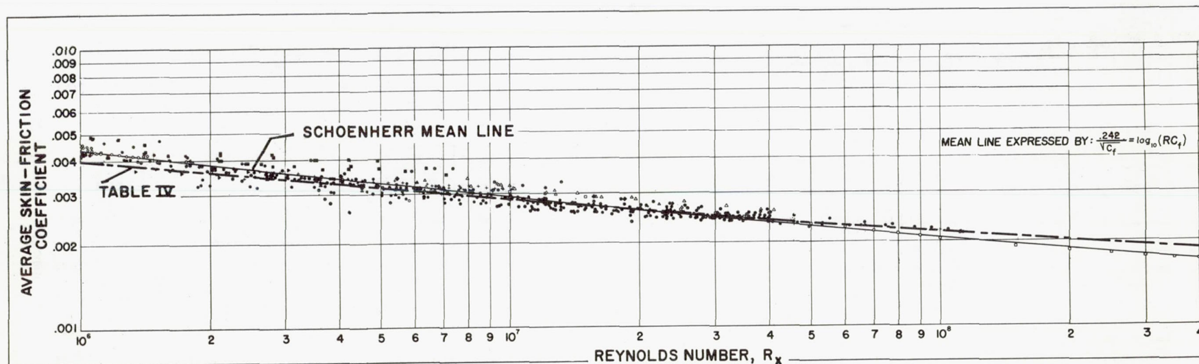
Figure 21.- Comparison of previous existing data with computed friction law (table IV).
