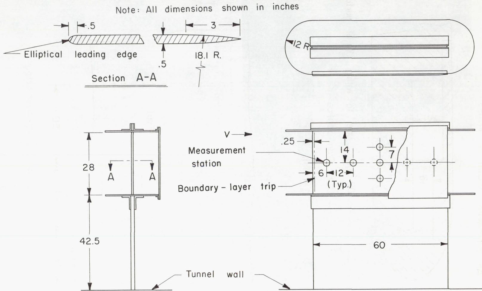
Figure 2.- Three-view drawing of boundary-layer channel.
