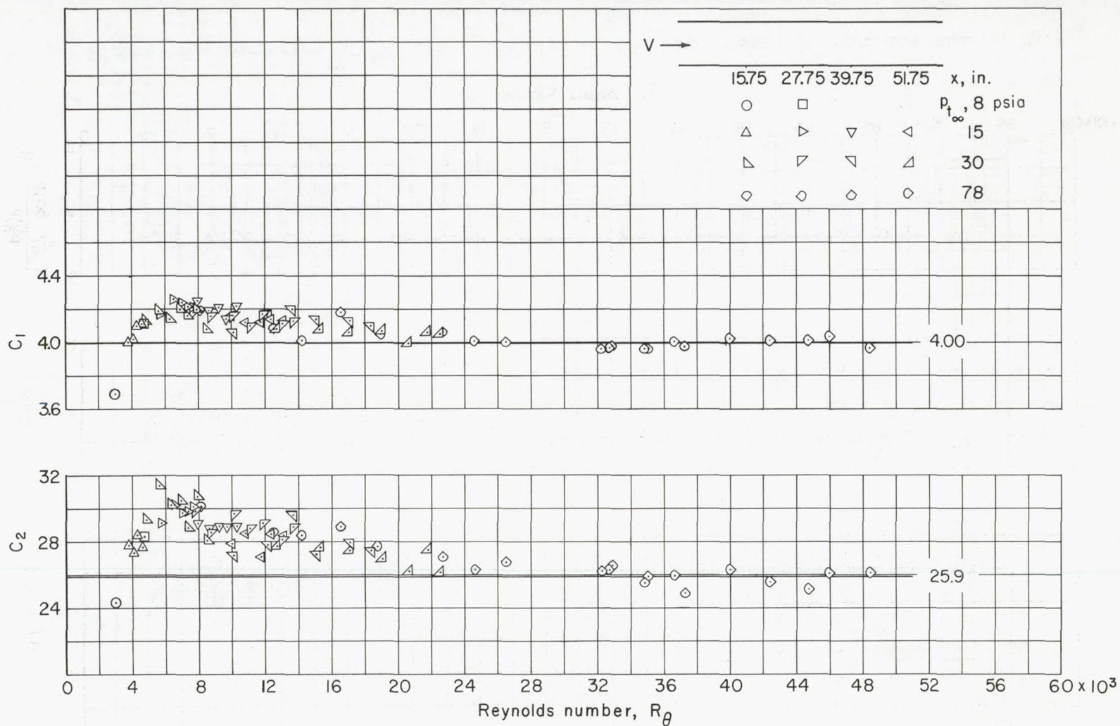
Figure 17.- Variation of C_1 and C_2 with change in Reynolds number, R_\theta .
