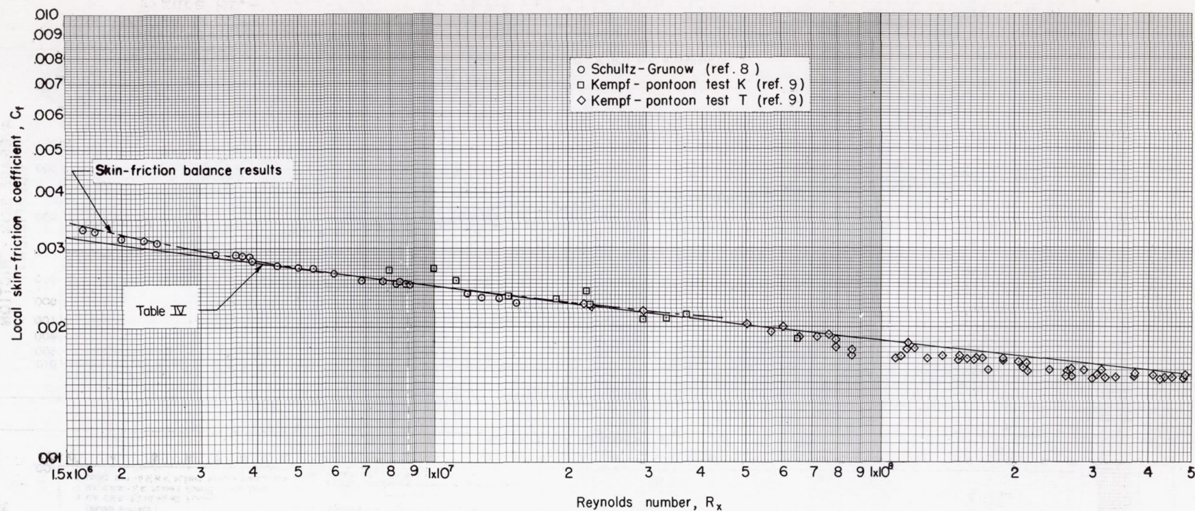
Figure 20.- Comparison of previous existing data with the measured data and with the curve computed using the constants derived from the present data.
