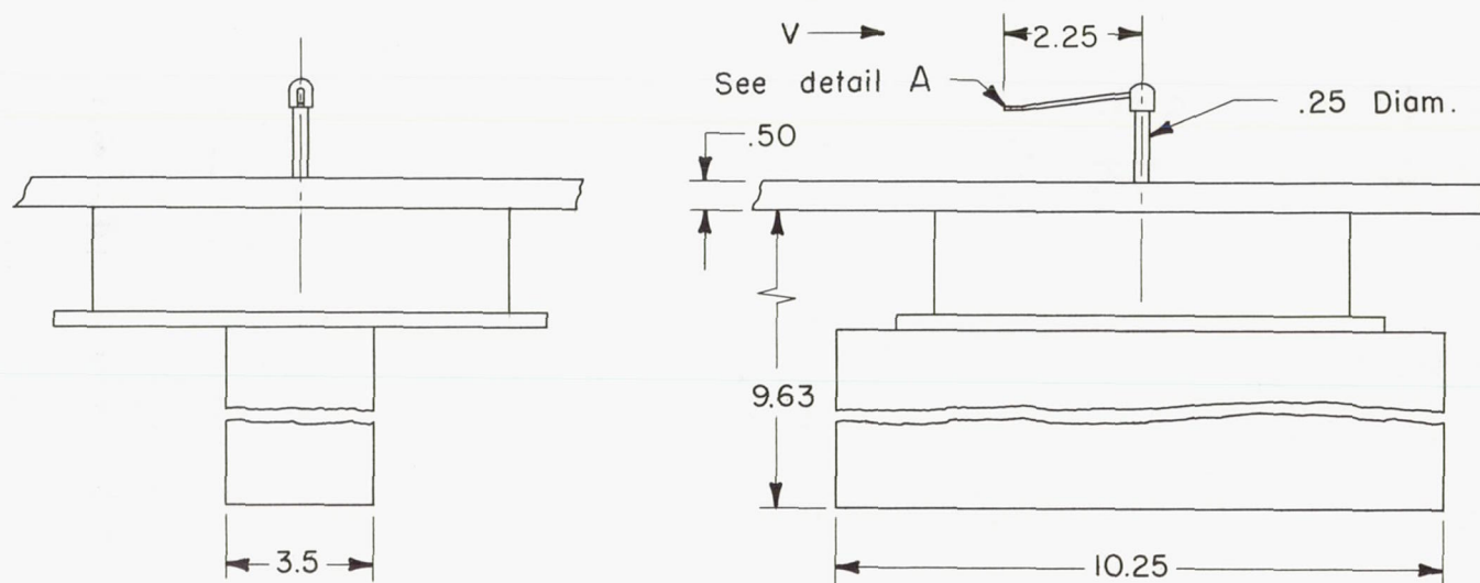
Figure 4.- Details of velocity probe and probe mounting mechanism.
