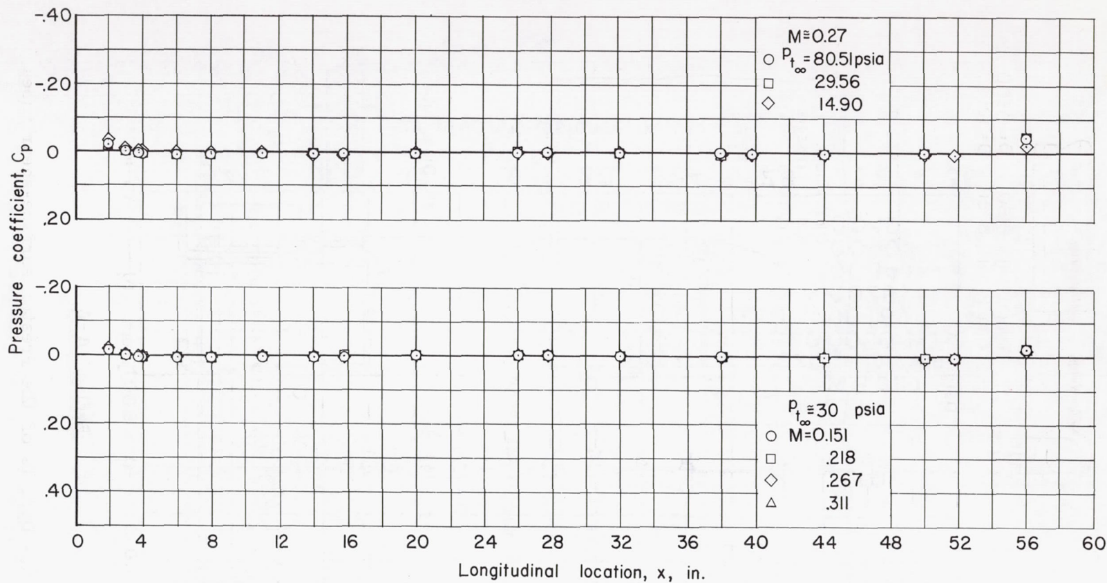
Figure 7.- Longitudinal pressure gradient in boundary-layer channel.
