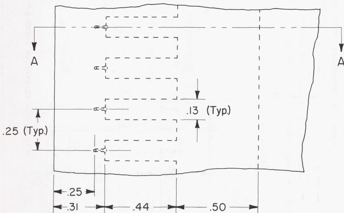
Figure 3.- Details of boundary-layer trip.
