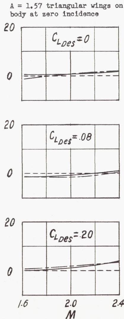
Figure 24.- Variation of center-of-pressure position of various configurations with Mach number and lift coefficient.
