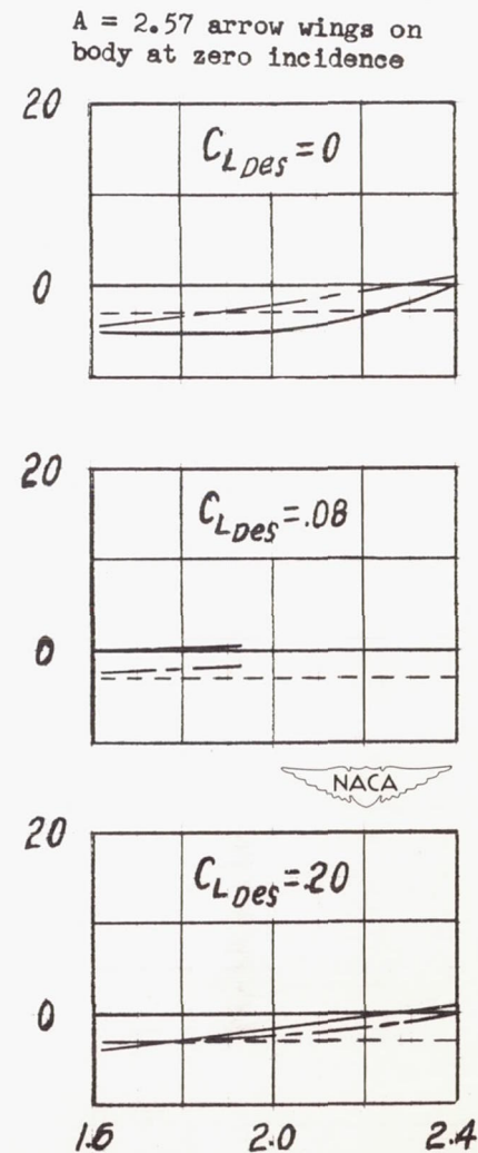
Figure 24.- Variation of center-of-pressure position of various configurations with Mach number and lift coefficient.
