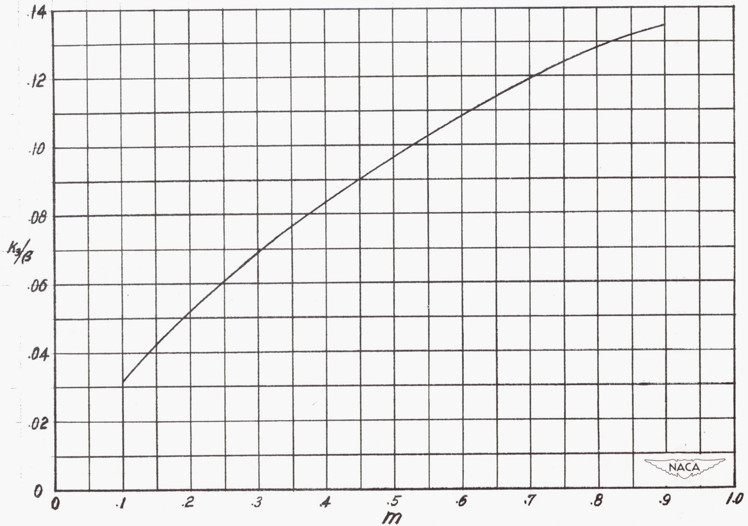
Figure 32.- Variation of the function K_3/\beta with m .
