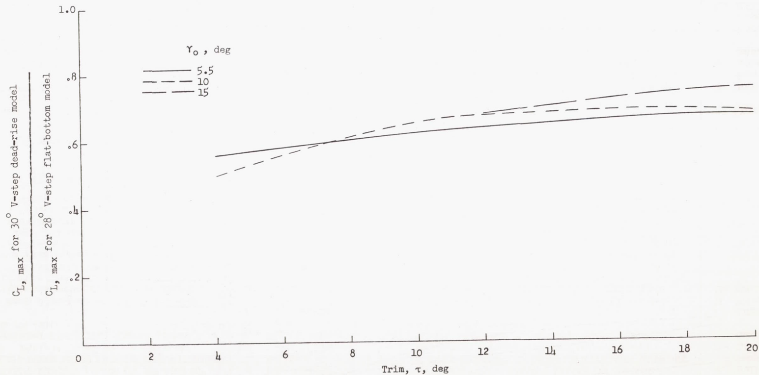
Figure 9.- Variations of ratio of maximum impact lift coefficients for dead-rise and flat-bottom models with V-step plan forms with trim angle.
