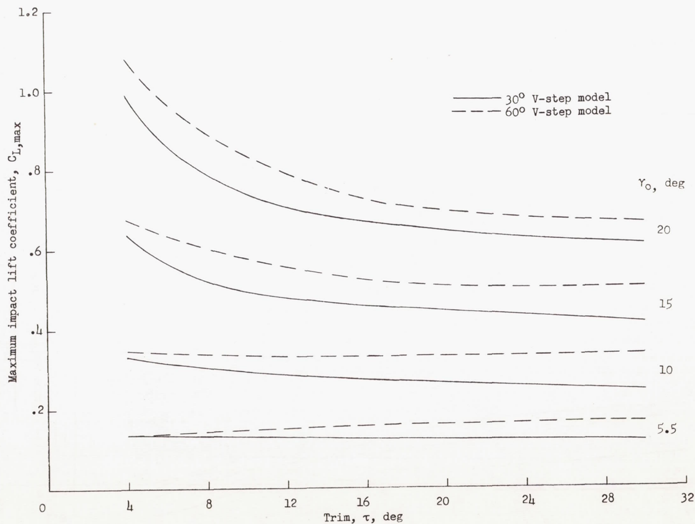
Figure 7.- Variations of faired values of maximum impact lift coefficient with trim angle for 30° and 60° V-step models.
