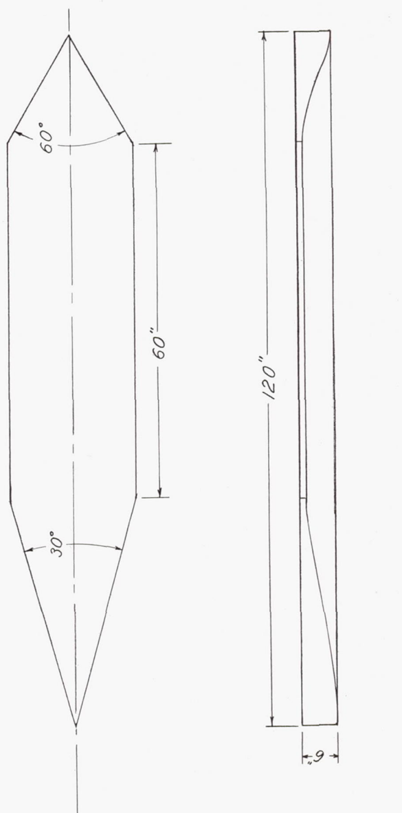
Figure 1.- Drawing of model.
