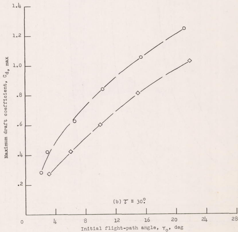
Figure 6.- Variations of draft coefficient with initial flight-path angle.
