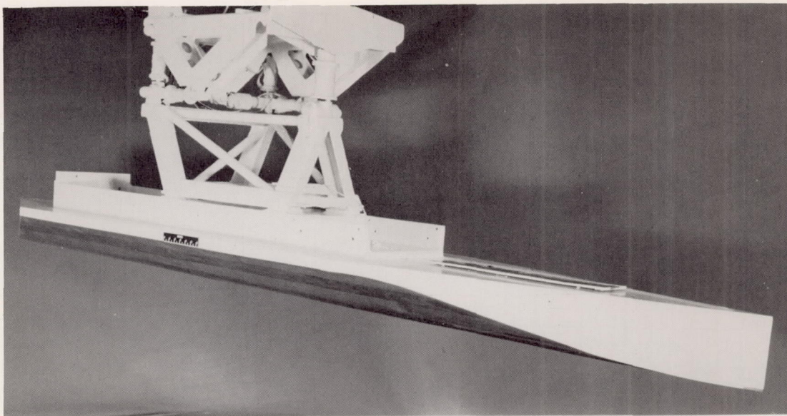
(a) 30° V-step model.
