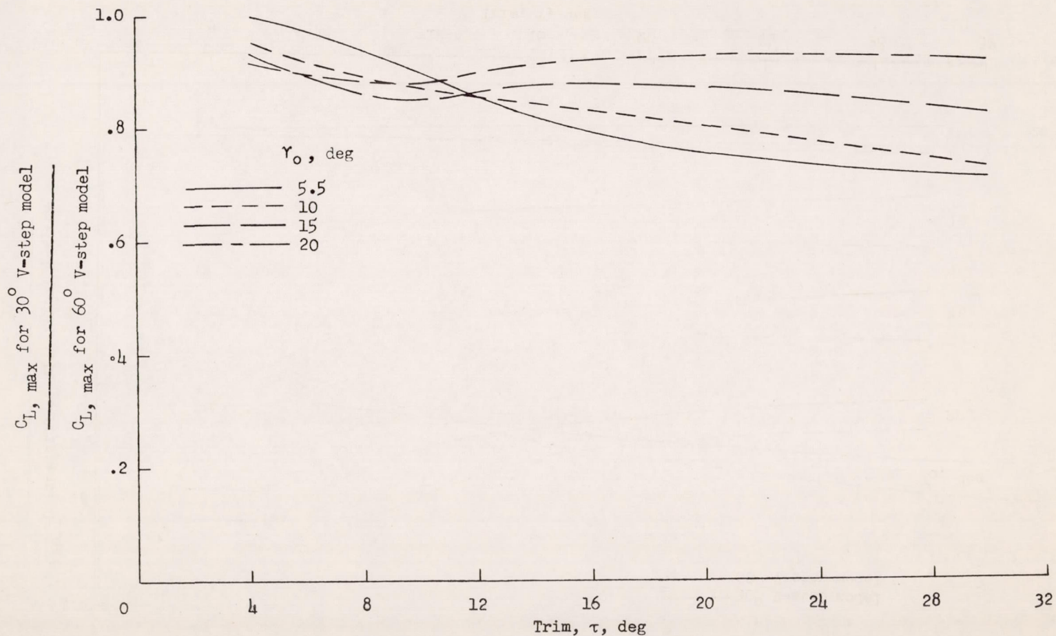
Figure 8.- Variations of ratio of maximum impact lift coefficients for 30^\circ and 60^\circ V-step models with trim angle.
