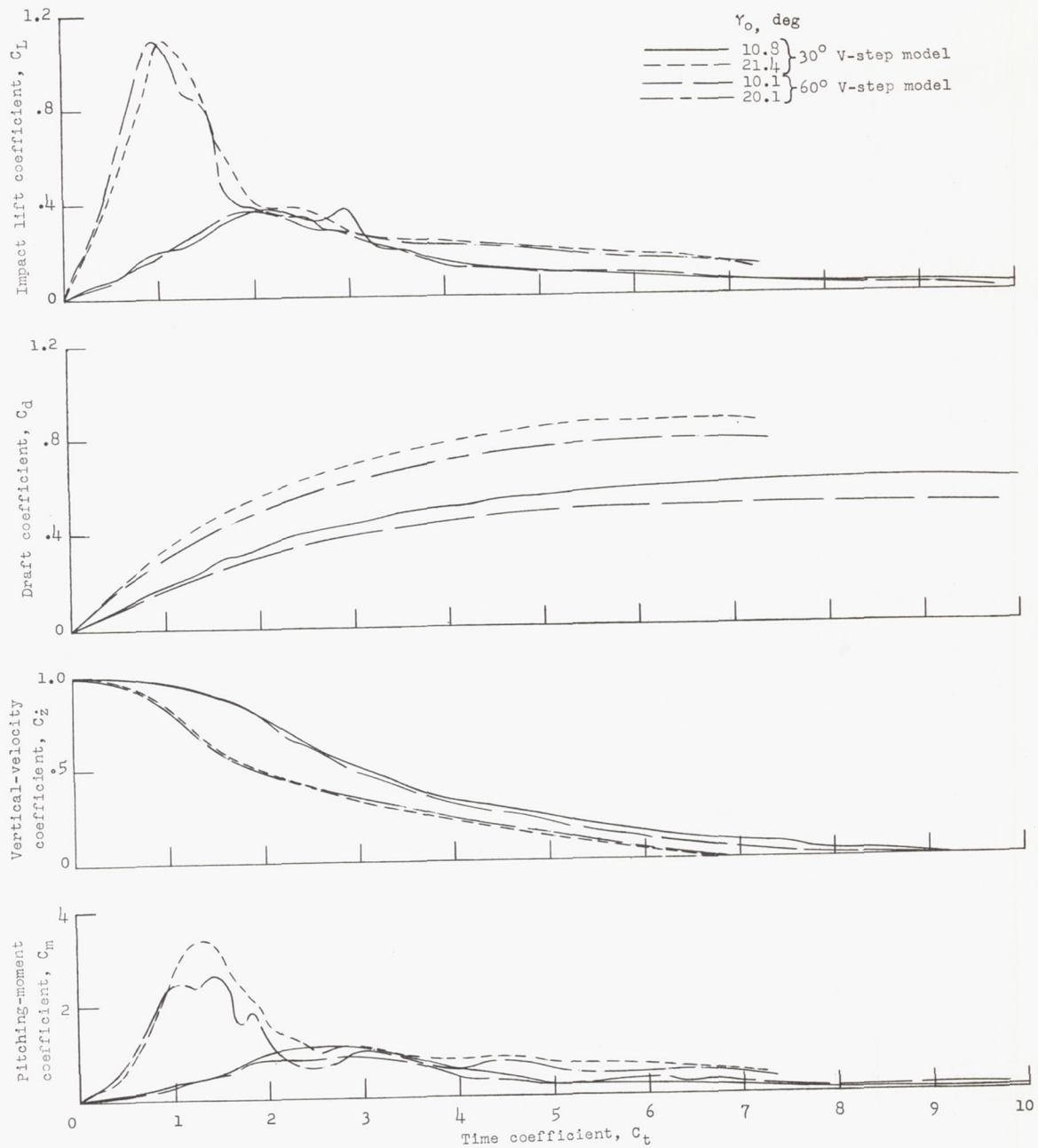
Figure 4.- Variations of load and motion coefficients with time coefficient for impacts with forward speed.
