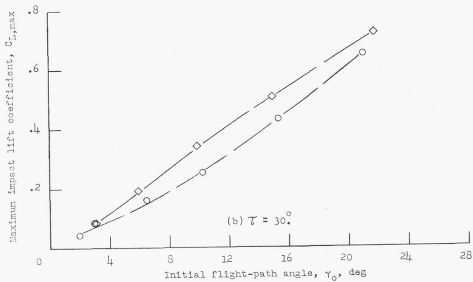
Figure 5.- Variations of impact lift coefficient with initial flight-path angle.
