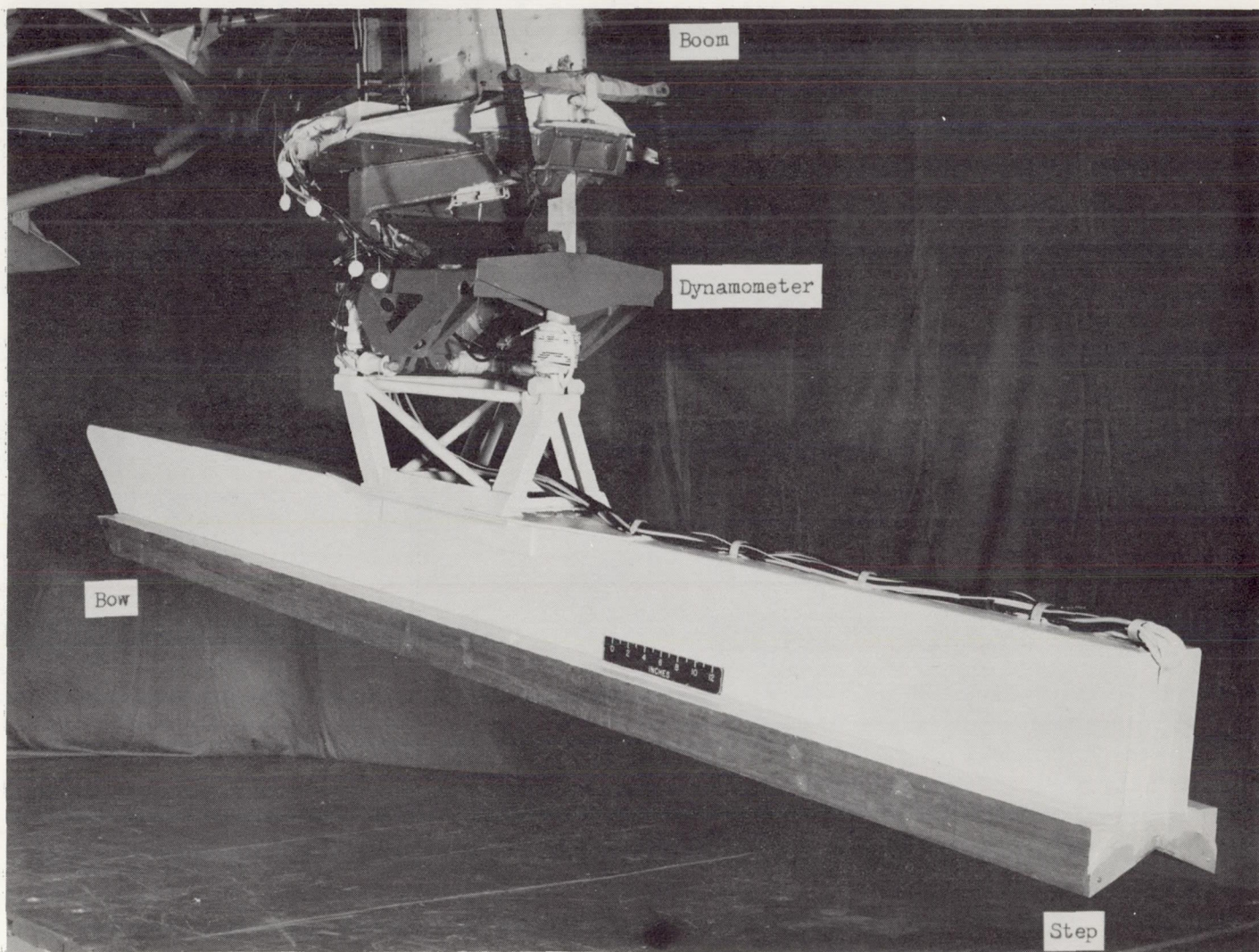
Figure 2.- Inverted-V model mounted on carriage in Langley impact basin. L-93869.1
