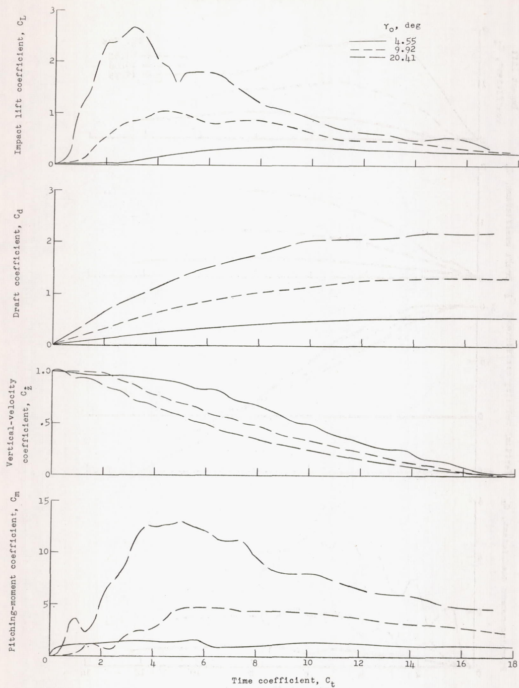
Figure 7.- Variations of the load and motion coefficients with time coefficient for impacts with forward speed. \tau = 8^\circ ; C_\Delta = 36.07 .
