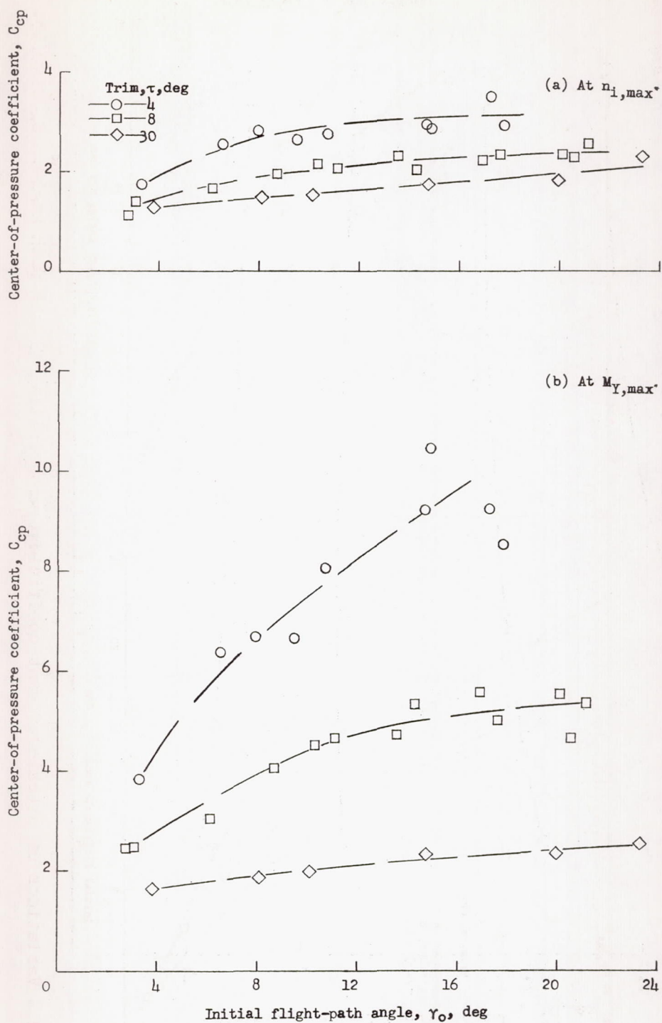
Figure 13.- Variations of center-of-pressure coefficient with initial flight-path angle. C_{\Delta} = 19.15 .
