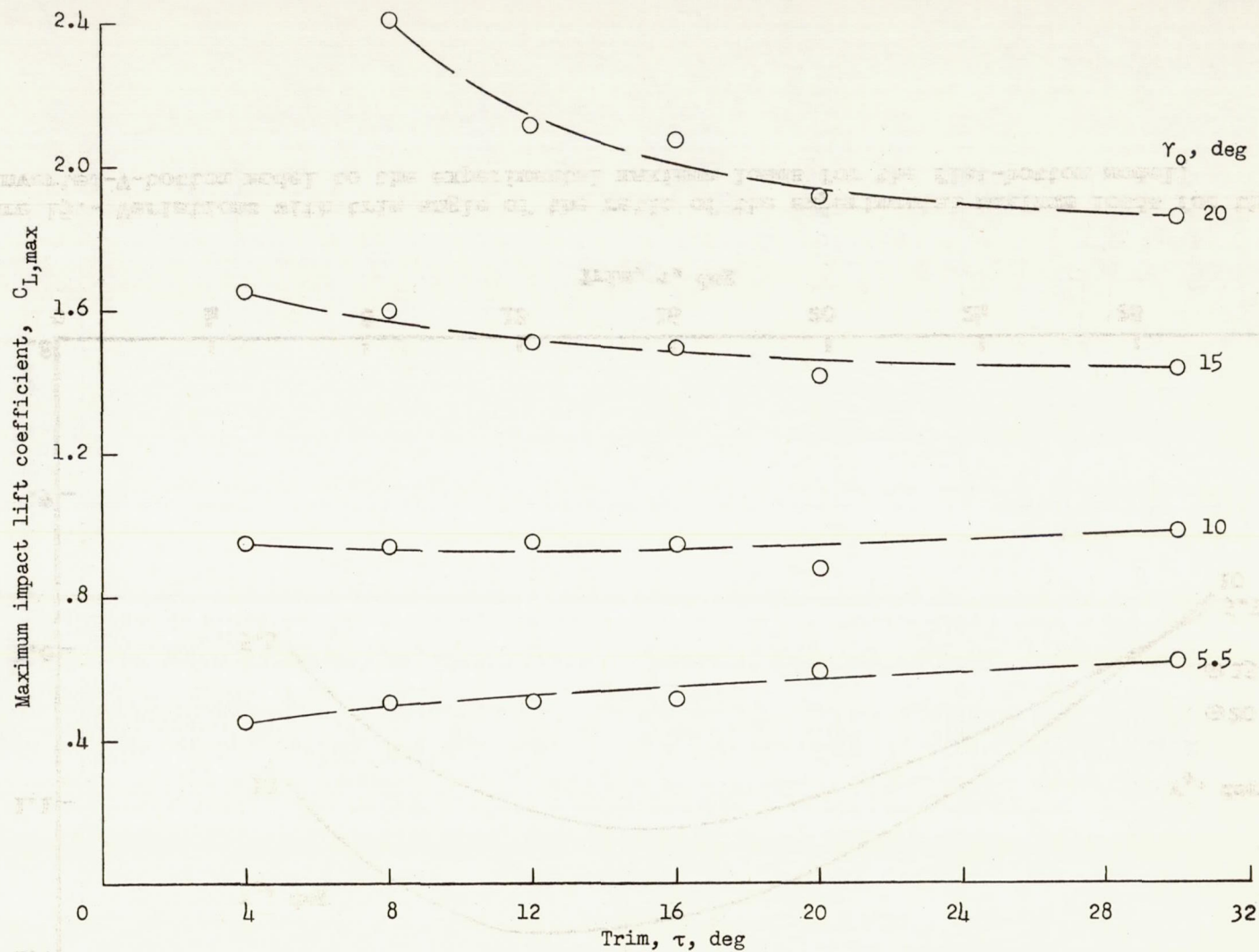
Figure 14.- Variations of faired values of maximum impact lift coefficient with trim angle. C_{\Delta} = 19.15 .
