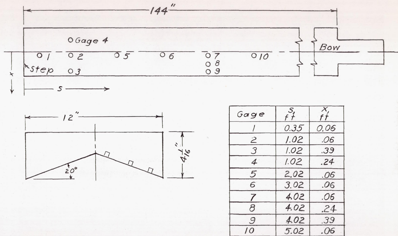
Figure 3.- Locations of pressure gages in bottom of inverted-V model having -20^\circ angle of dead rise.
