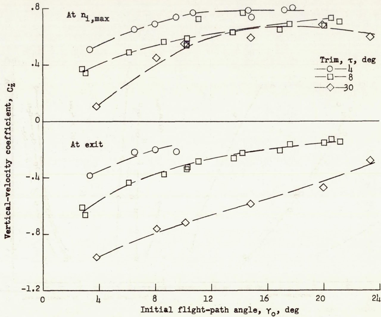
Figure 10.- Variations of vertical-velocity coefficient with initial flight-path angle. C_{\Delta} = 19.15 .
