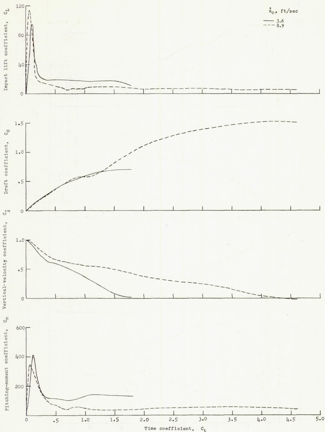
Figure 4.- Variations of load and motion coefficients with time coefficient for impacts without forward speed. \tau = 0^\circ ; C_\Delta = 19.15 .
