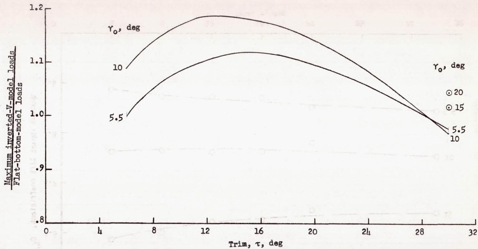
Figure 15.- Variations with trim angle of the ratio of the experimental maximum loads for the inverted-V-bottom model to the experimental maximum loads for the flat-bottom model.
