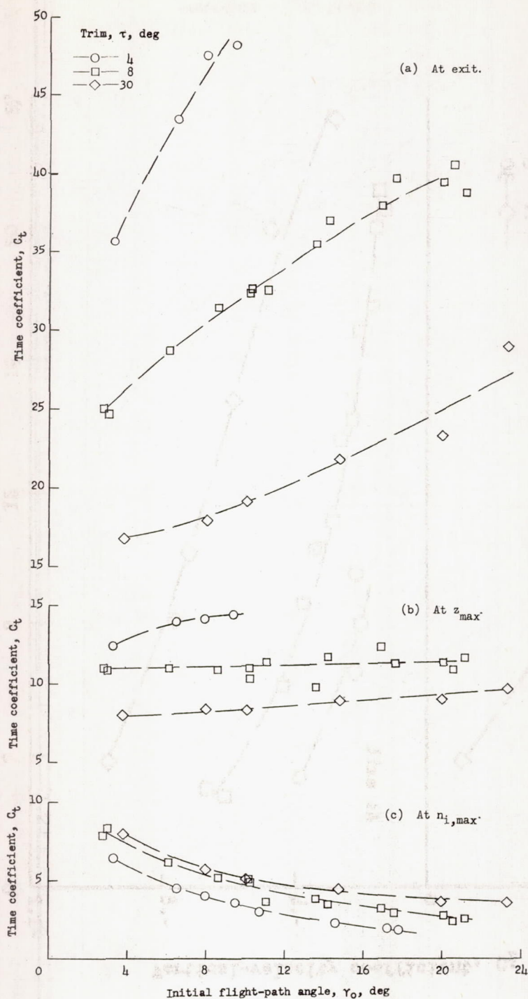
Figure 11.- Variations of time coefficient with initial flight-path angle. C_{\Delta} = 19.15 .
