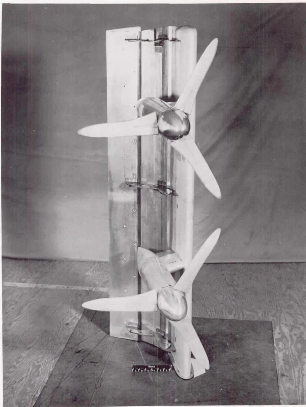
L-96515 Figure 4.- Model installed in a static-test facility at the Langley Laboratory. \frac{X}{D} = 0.500 ; \frac{Y}{D} = -0.01 ; \frac{Z}{D} = -0.229 .
