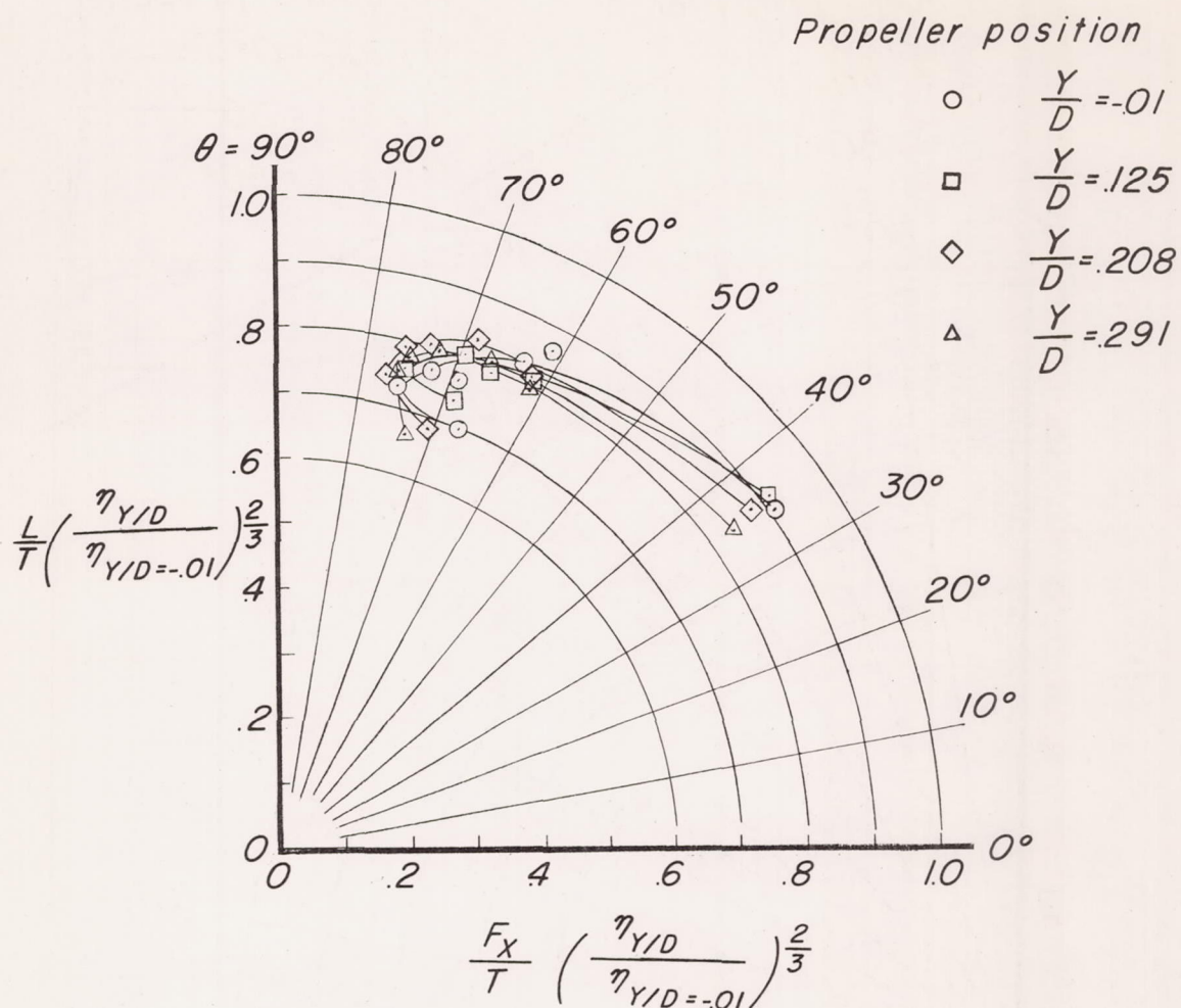
Figure 31.- Summary of turning effectiveness based on constant power. \delta_{f,s} = 50^\circ .
