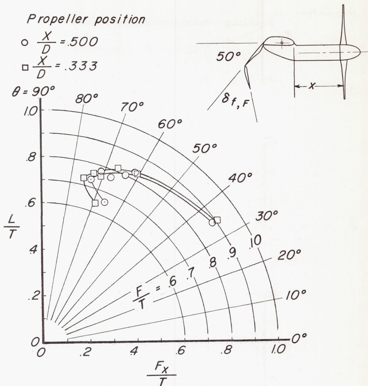
(a) Summary of turning effectiveness.
