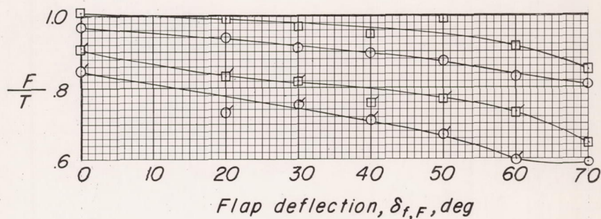
(c) Thrust-recovery factor.
