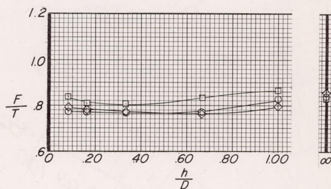
(c) Thrust-recovery factor.
