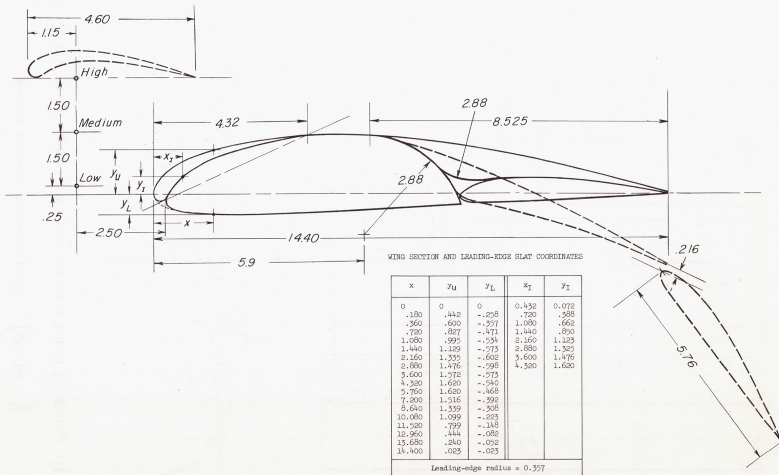
Figure 2.- Geometric characteristics of wing section. All dimensions are in inches.
