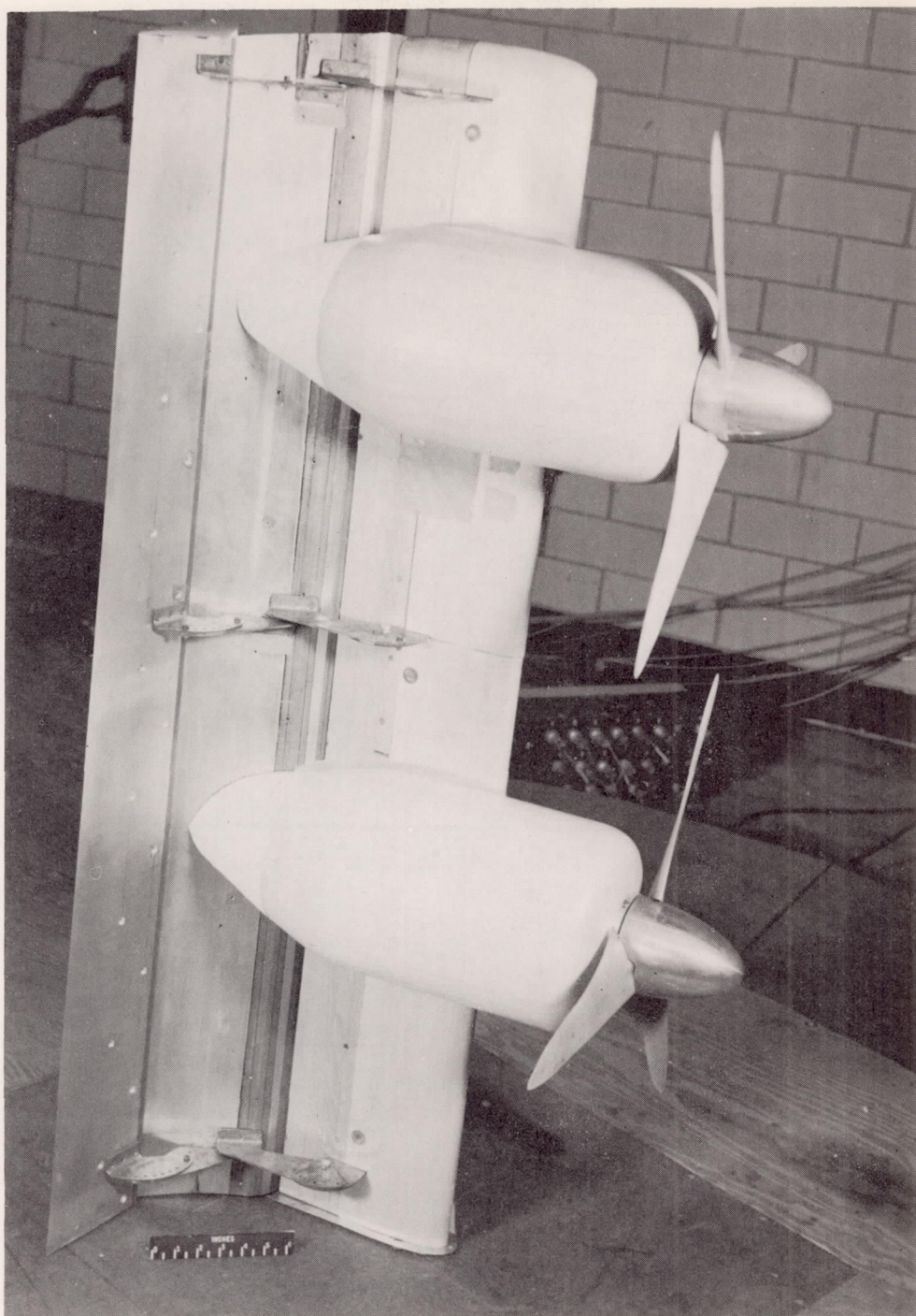
Figure 39.- Model with large nacelles. L-96617
