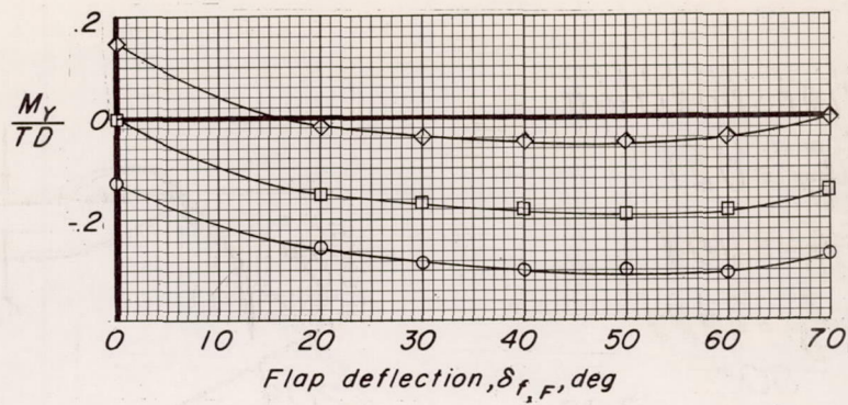
(b) Pitching moment.
