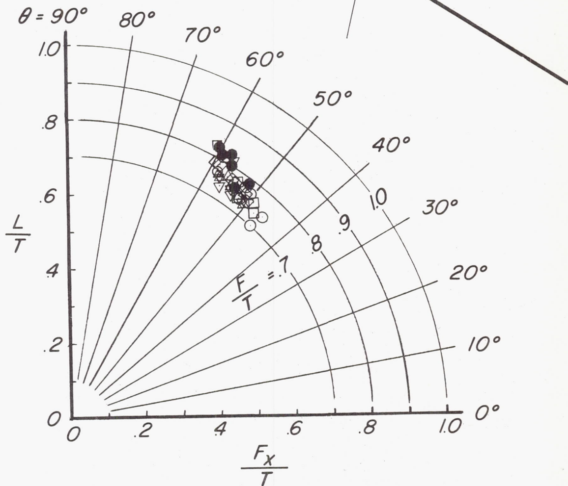
(a) Summary of turning effectiveness.
