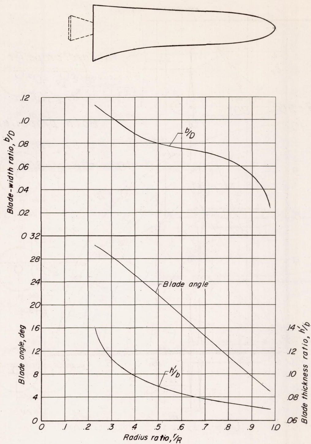
Figure 7.- Propeller blade-form curves. NACA 16-series section.
