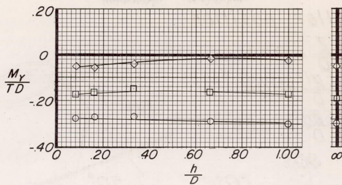
(b) Pitching moment.
