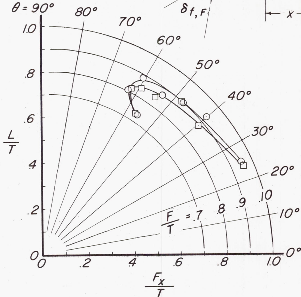
(a) Summary of turning effectiveness.
