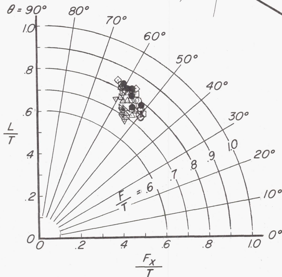
(a) Summary of turning effectiveness.
