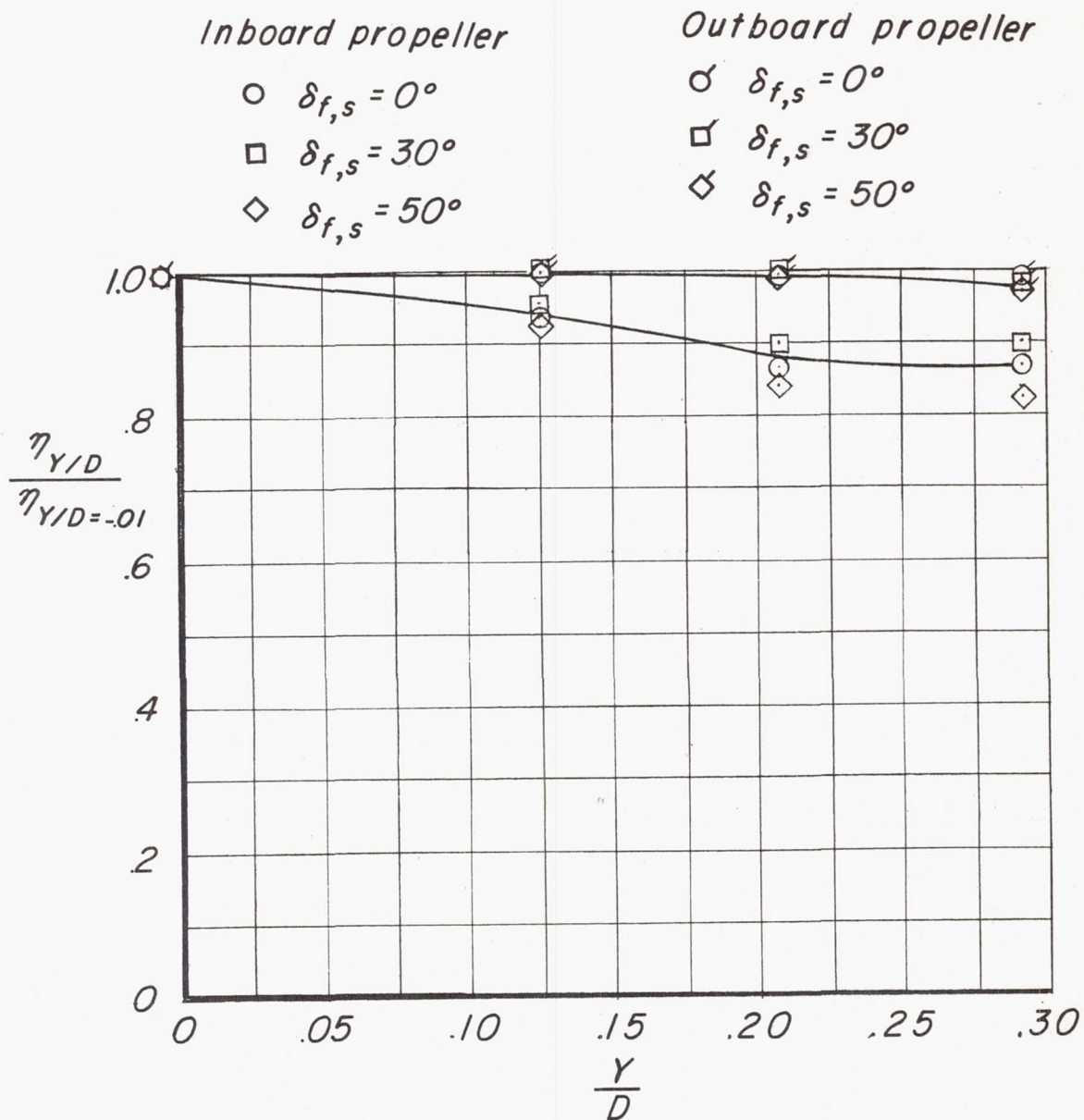
Figure 30.- Variation of average efficiency of propellers with overlap (averaged over \delta_{f,F} range).
