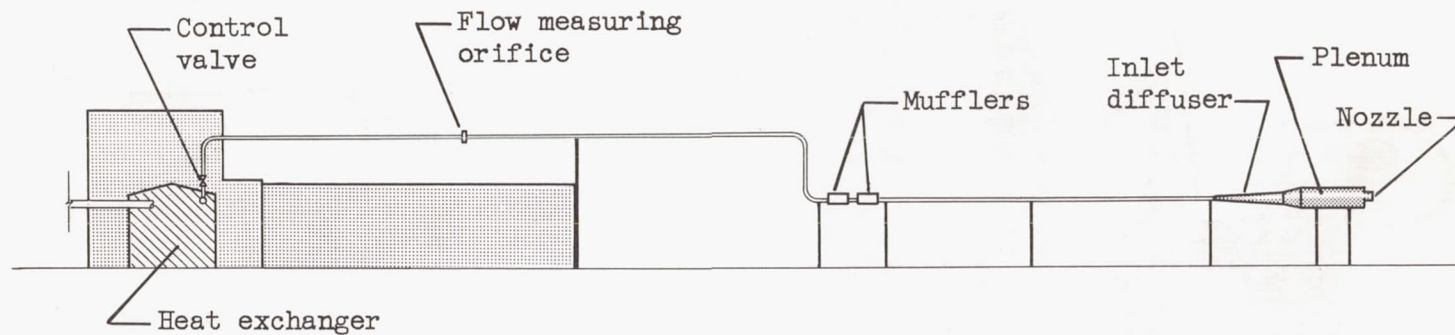
(a) Elevation.
