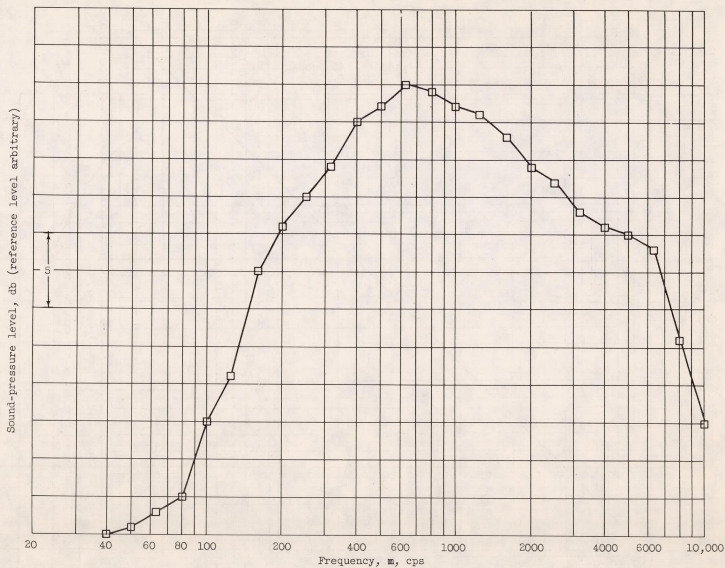
Figure 16. - Sound-pressure-level spectrum at distance of 20 feet from nozzle exit. Run 65; azimuth, 30°; source and receiver heights, 10 feet.
