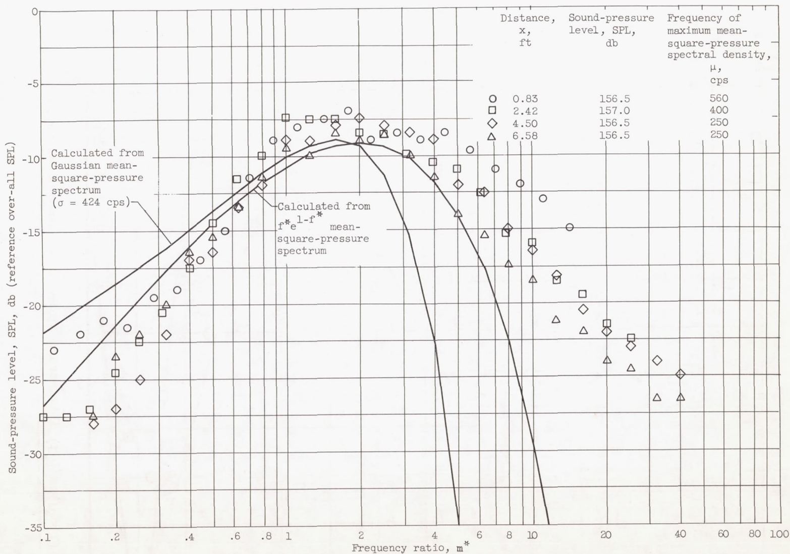
Figure 1. - Dimensionless 1/3-octave sound-pressure-level spectra along jet-engine-exhaust boundary (ref. 5).
