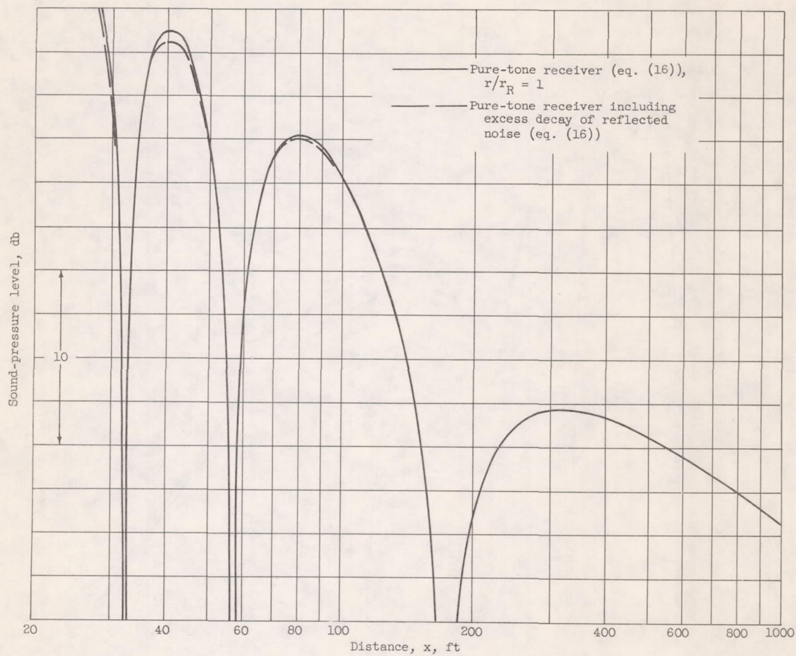
Figure 4. - Effect of excess decay of reflected noise. Pure-tone receiver; perfect reflector; acceptance frequency, 500 cycles per second; source and receiver heights above plane, 10 feet; speed of sound, 1140 feet per second.
