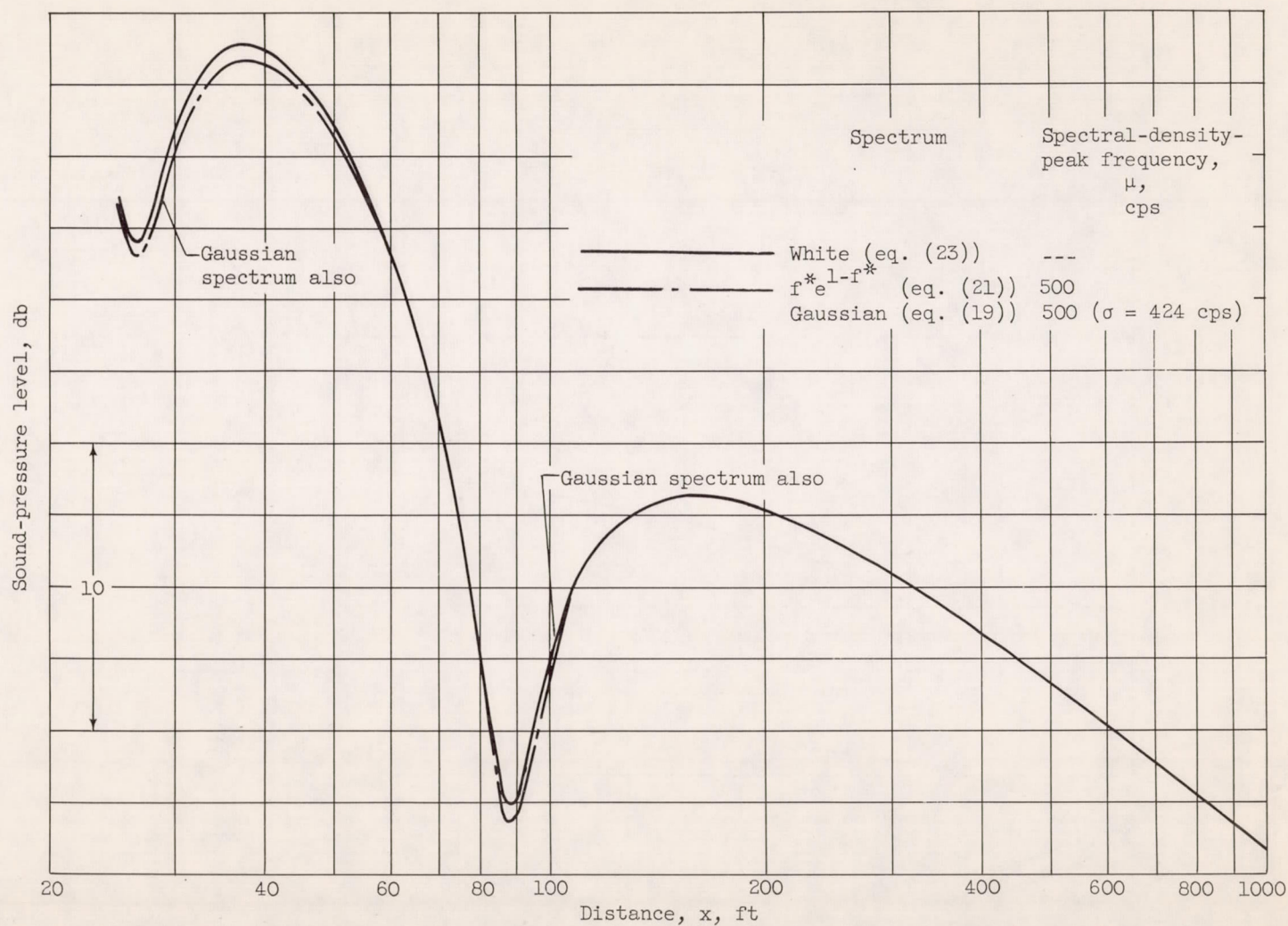
Figure 8. - Effect of spectrum shape on decay for 1/3-octave receiver. Perfect reflector; source and receiver heights above plane, 10 feet; speed of sound, 1140 feet per second.
