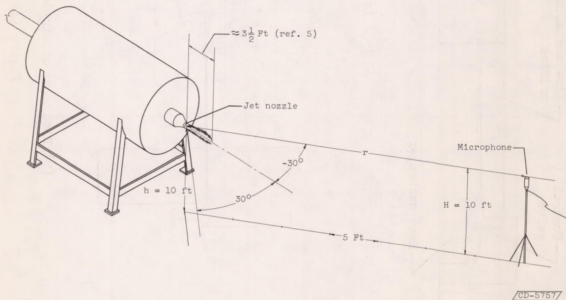
Figure 12. - Experimental geometry.
