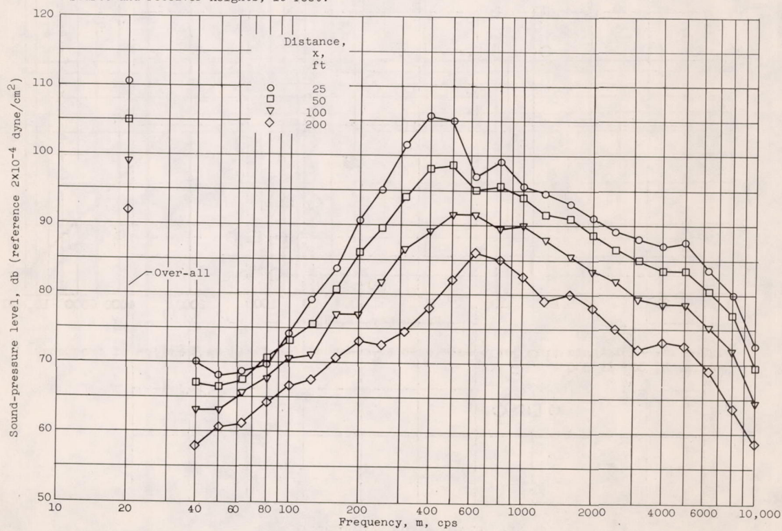
Figure 19. - Corrected sound-pressure-level spectra at various distances from source. Source and receiver heights, 10 feet.
