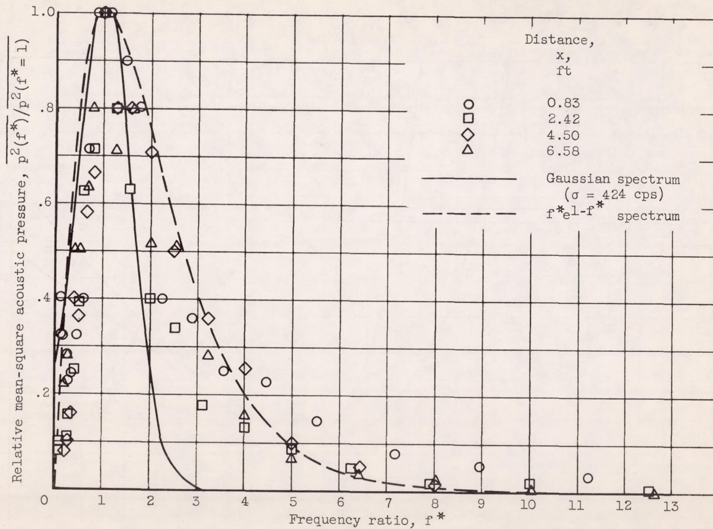
Figure 2. - Dimensionless relative mean-square-acoustic-pressure spectra along jet-engine-exhaust boundary.
