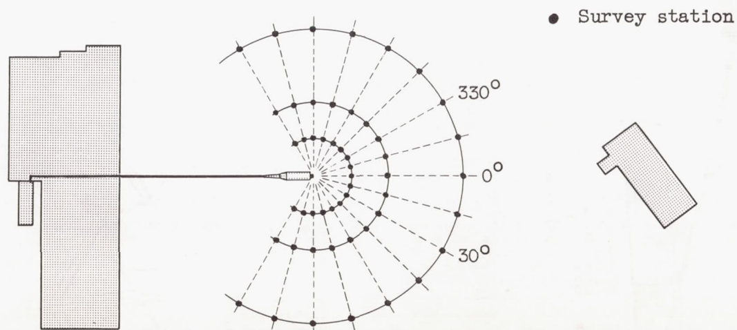
(b) Plan view of air-jet system and adjacent buildings.
