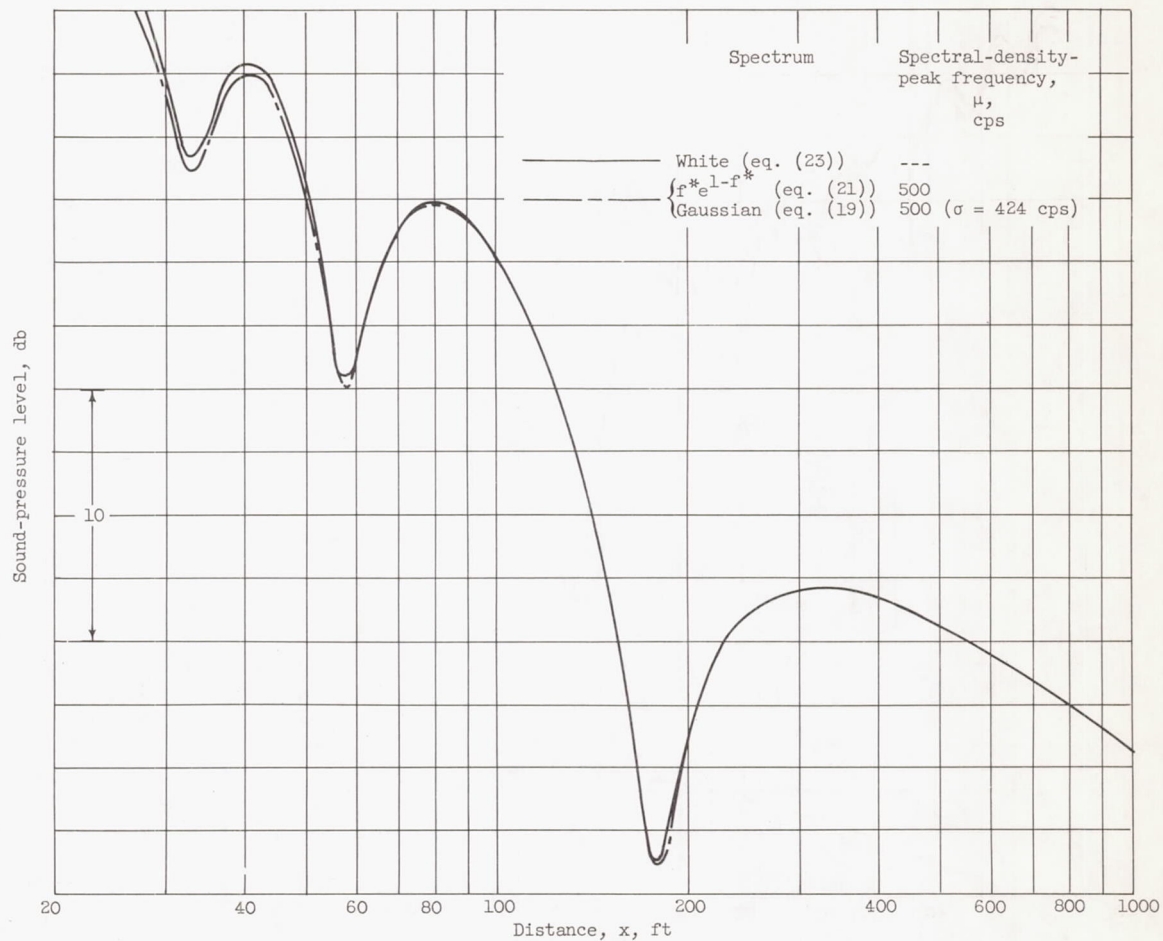
Figure 8. - Continued. Effect of spectrum shape on decay for 1/3-octave receiver. Perfect reflector; source and receiver heights above plane, 10 feet; speed of sound, 1140 feet per second.
