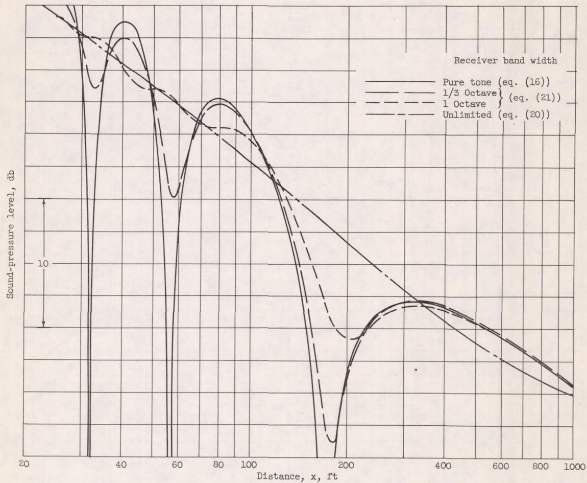
Figure 6. - Effect of receiver band width on decay of r^*e^{1-r^*} spectrum. Perfect reflector; spectral-density-peak and mean filter frequencies, 500 cycles per second; source and receiver heights above plane, 10 feet; speed of sound, 1140 feet per second.
