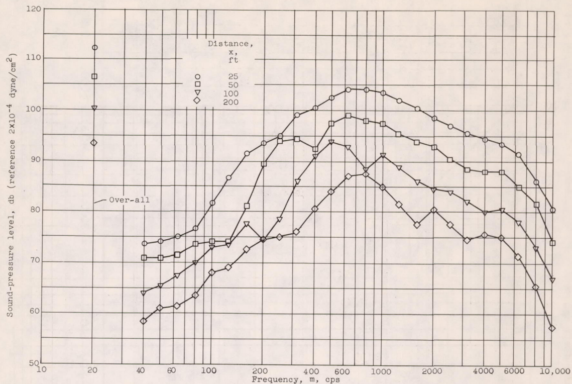
Figure 18. - Experimentally determined sound-pressure-level spectra at various distances from source. Source and receiver heights, 10 feet.
