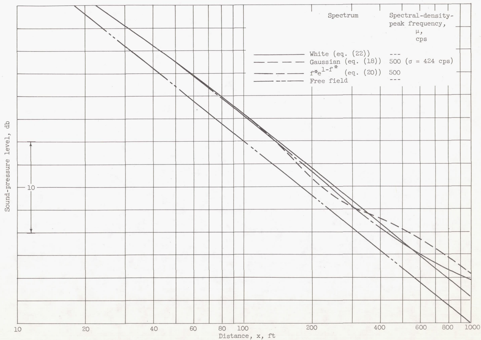
Figure 7. - Effect of spectrum shape on decay for unlimited band pass. Perfect reflector; source and receiver heights above plane, 10 feet; speed of sound, 1140 feet per second.
