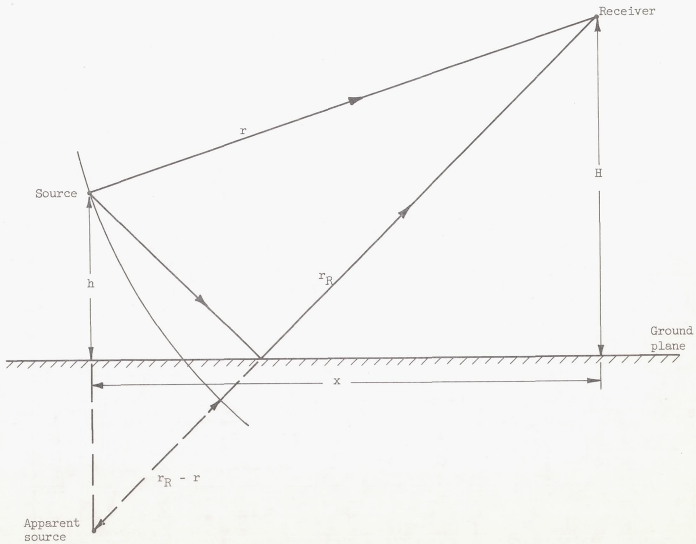
Figure 3. - Geometry of noise field in presence of plane reflector.
