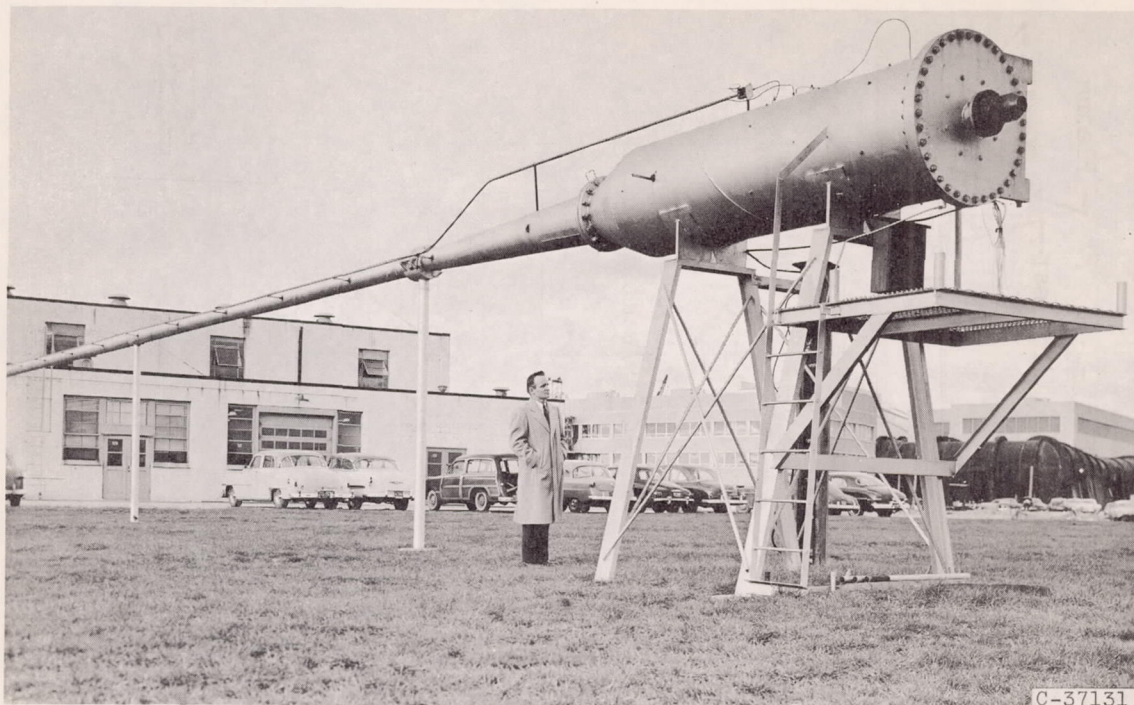
(c) Photograph of air-jet system.
