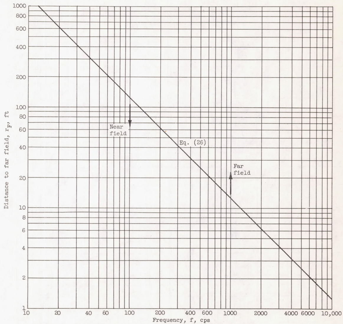
Figure 17. - Distance from jet nozzle exit to onset of far field as function of frequency. Azimuth, 30^\circ or 330^\circ .
