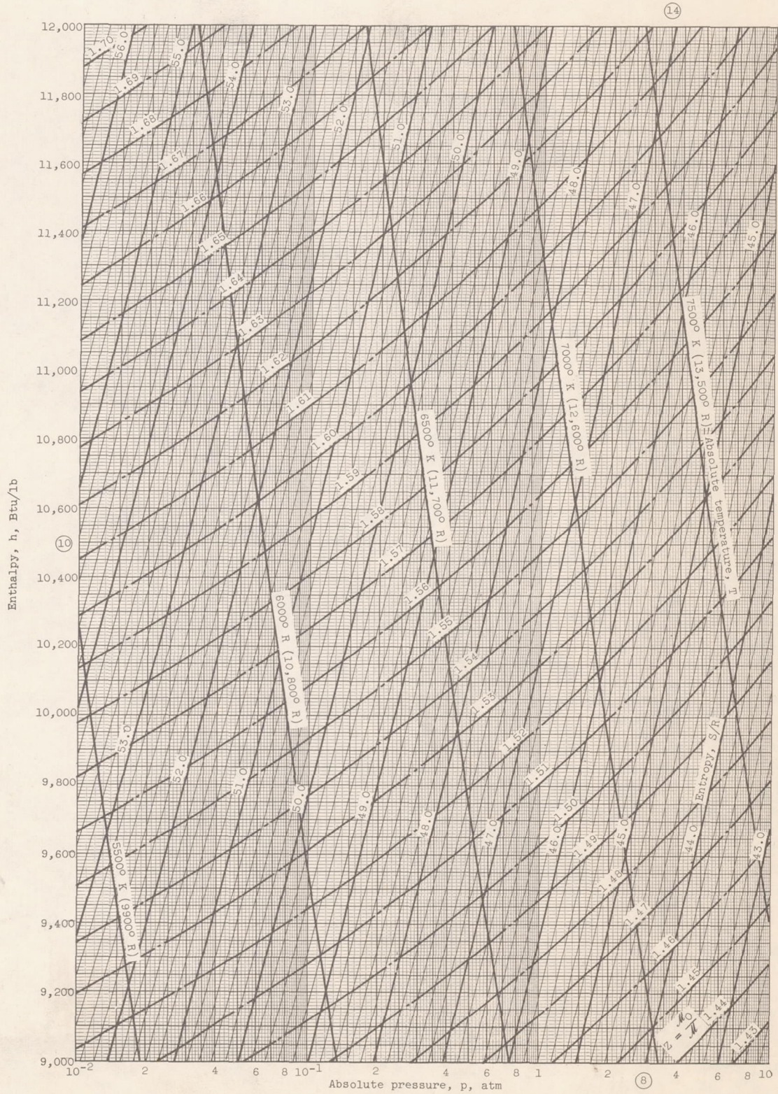
(k) Chart 11. Figure 3. - Continued. Thermodynamic charts for air.
