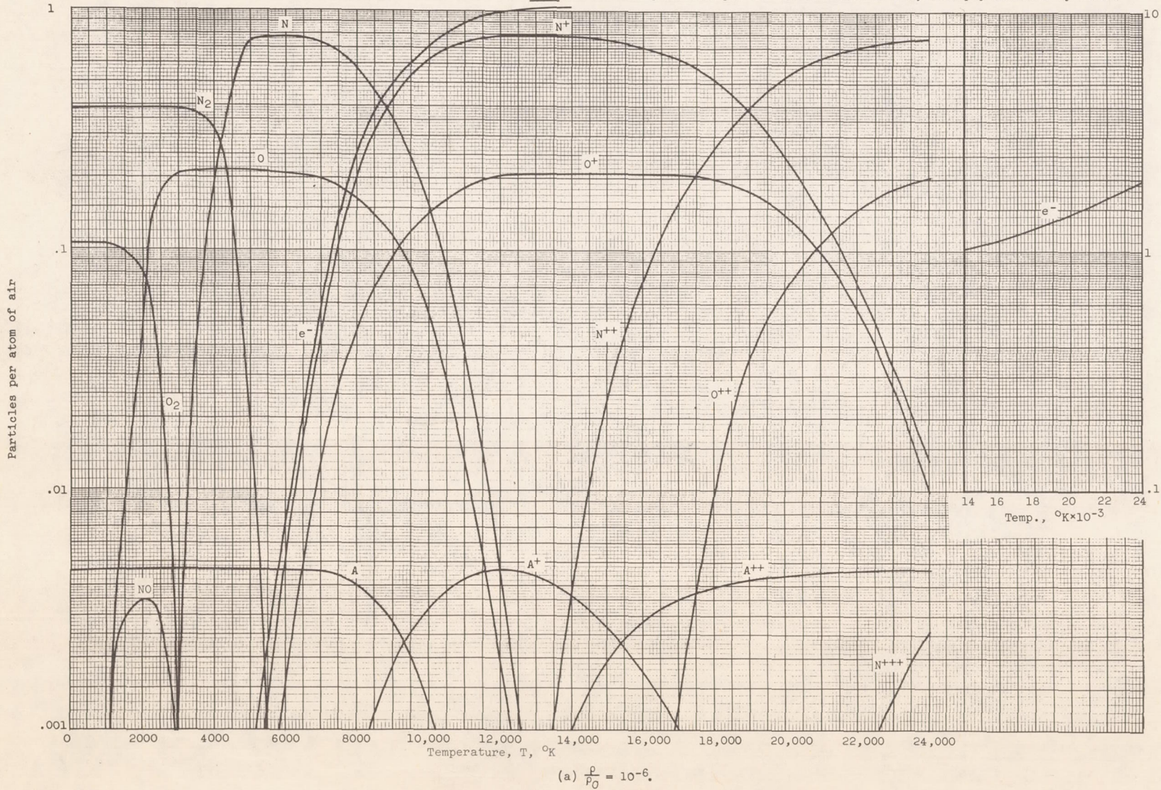
Figure 1. - Equilibrium composition of air to 24,000° K.
