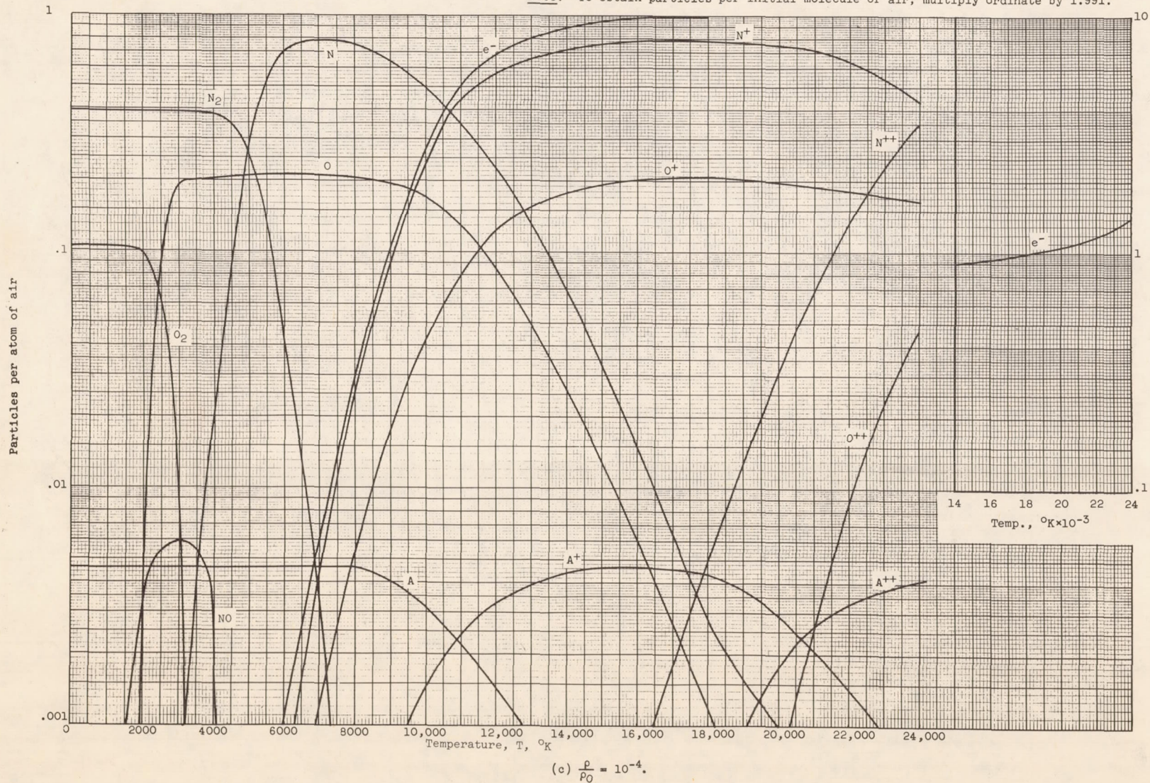
Figure 1. - Continued. Equilibrium composition of air to 24,000° K.
