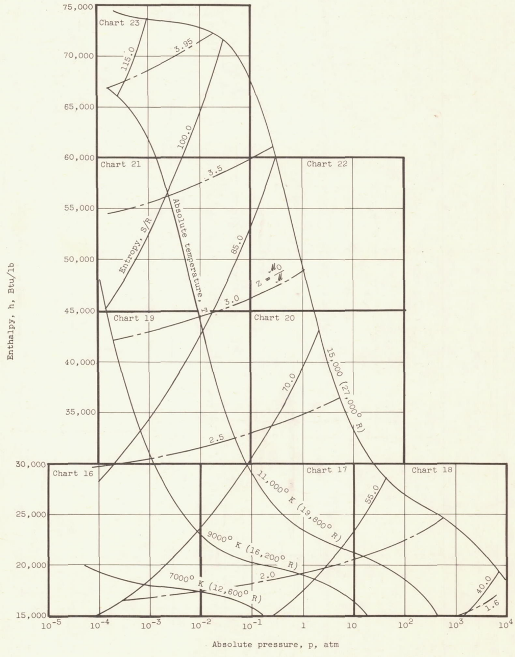
Figure 2. - Concluded. Key to thermodynamic charts for air.
