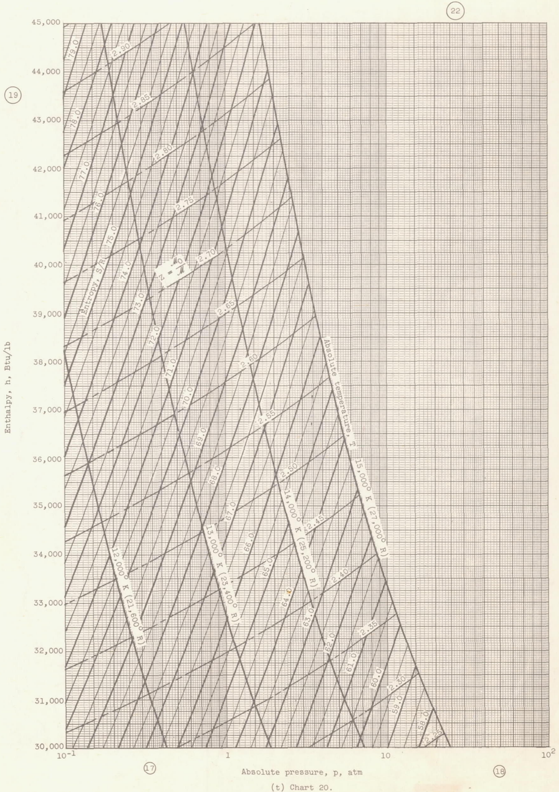
Figure 3. - Continued. Thermodynamic charts for air
