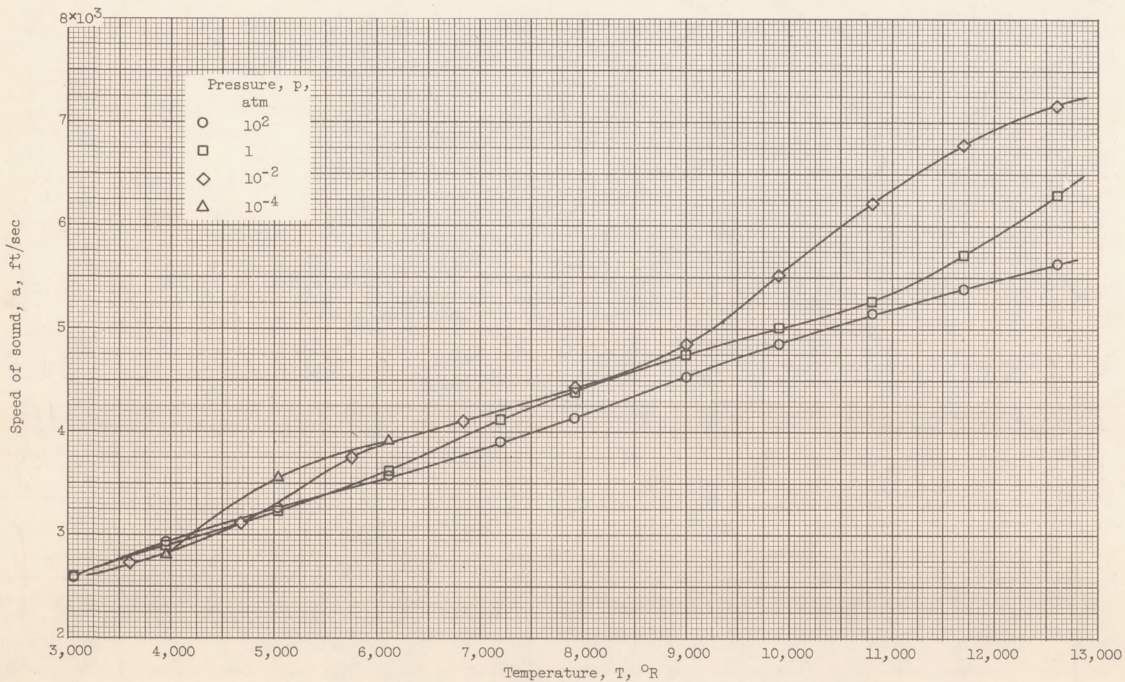
Figure 5. - Speed of sound in air against temperature. a = \sqrt{\frac{\gamma g J R T}{M}} .
