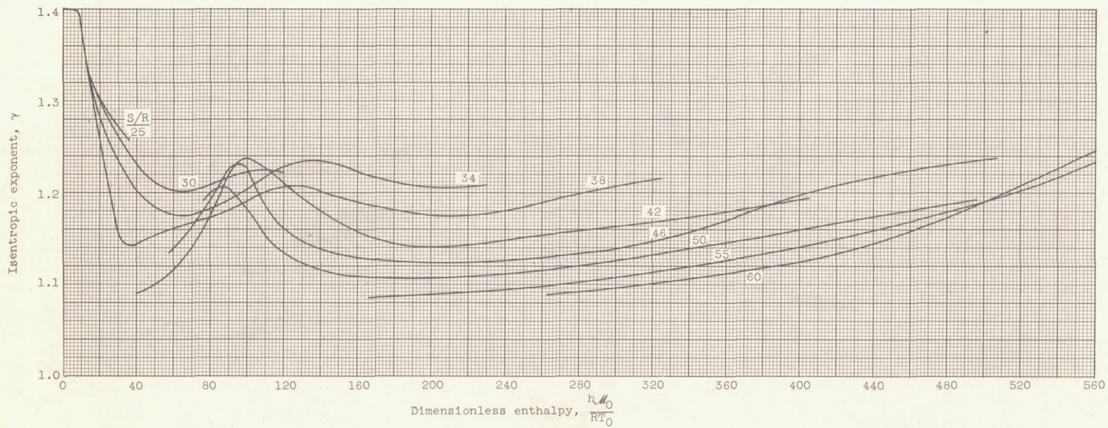
Figure 4. - Isentropic exponent for air in equilibrium.
