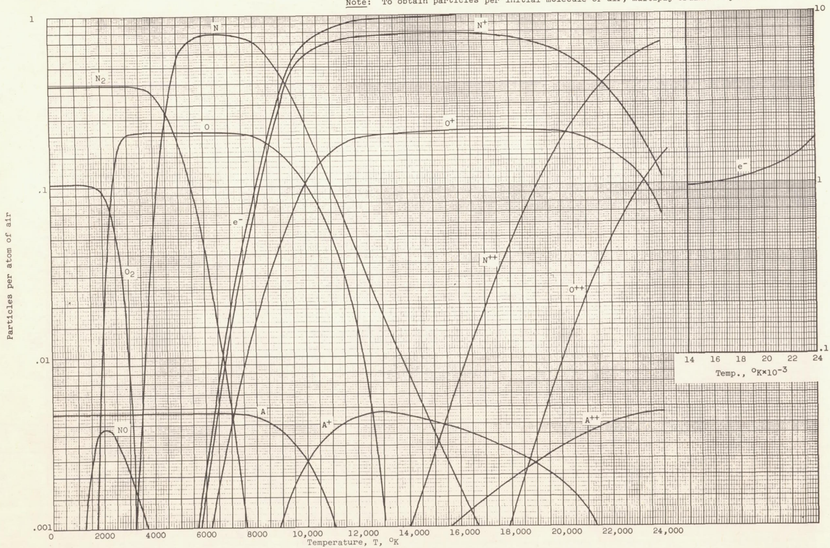
Figure 1. - Continued. Equilibrium composition of air to 24,000° K.
