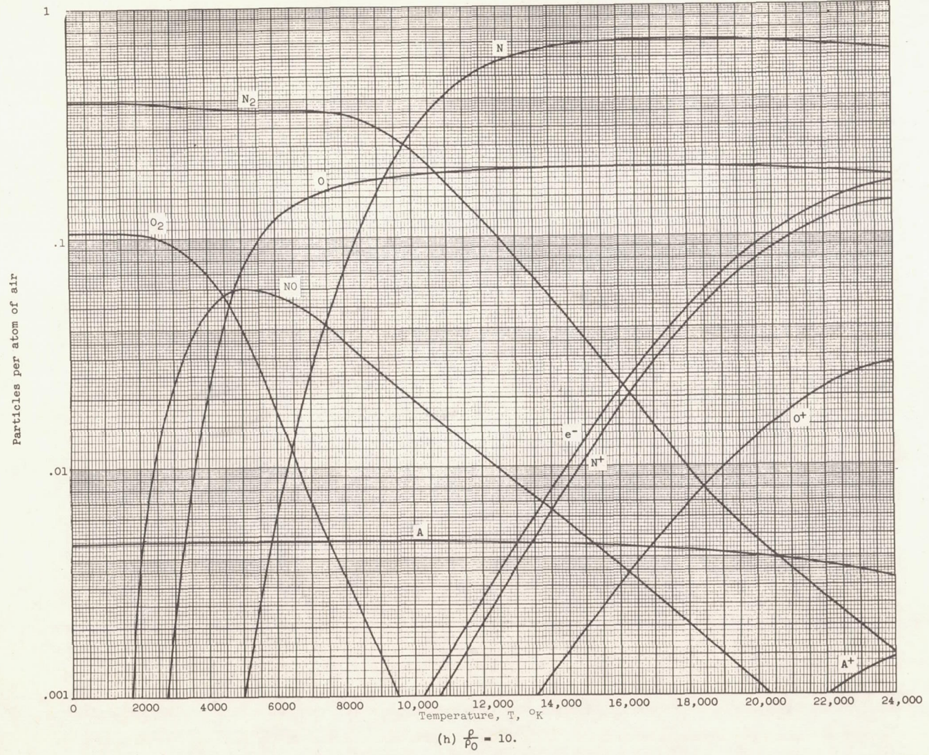
Figure 1. - Concluded. Equilibrium composition of air to 24,000° K.
