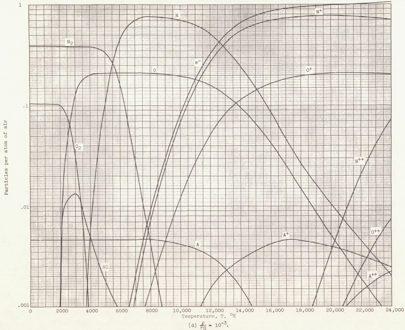
Figure 1. - Continued. Equilibrium composition of air to 24,000° K.
