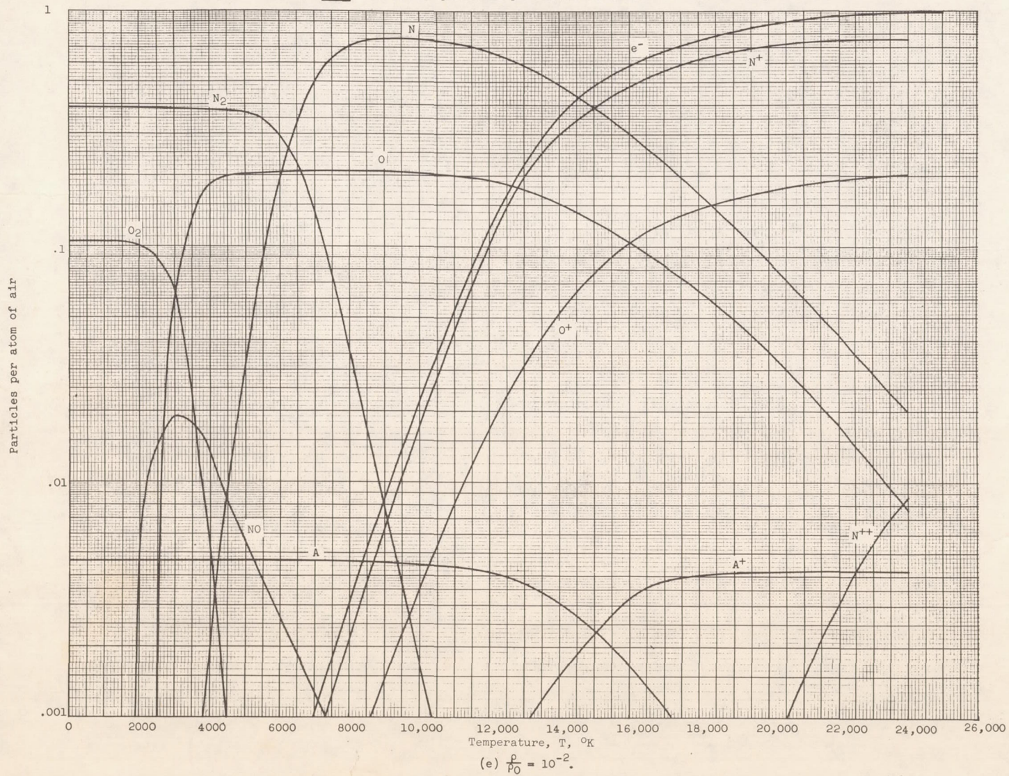
Figure 1. - Continued. Equilibrium composition of air to 24,000° K.
