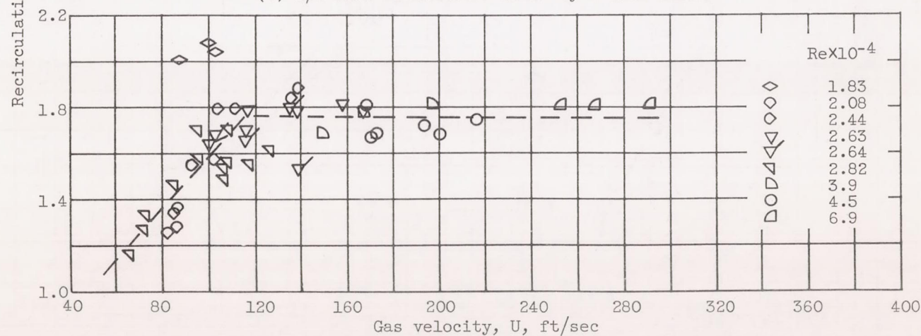
Figure 8. - Concluded. Recirculation-zone length as function of gas velocity.
