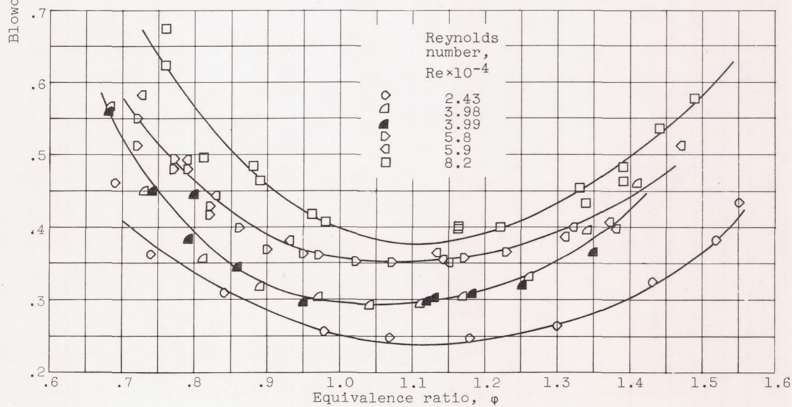
Figure 3. - Continued. Variation of blowoff pressure with fuel concentration for different Reynolds numbers.
