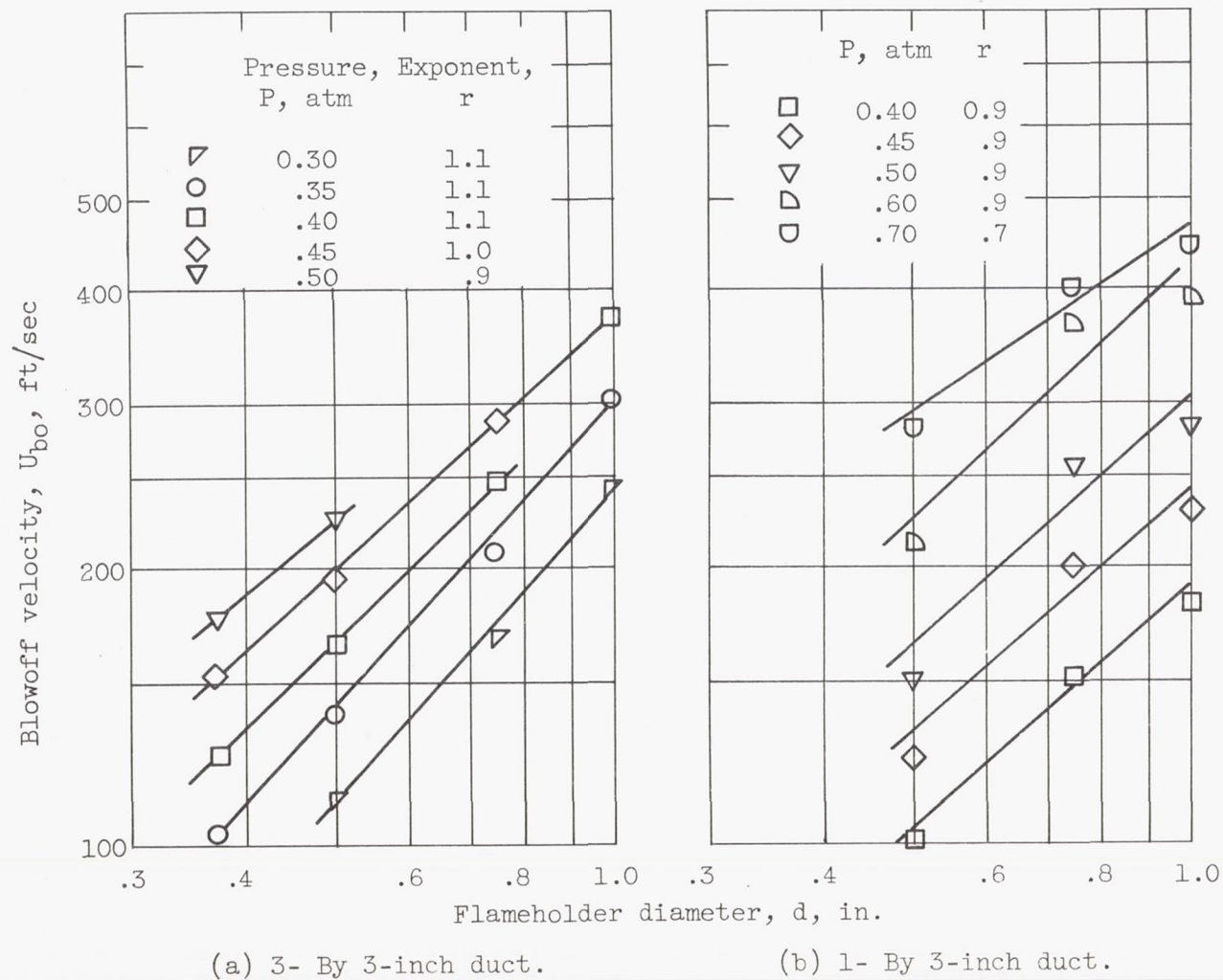
Figure 5. - Effect of flameholder diameter on blowoff velocity of stoichiometric mixtures.
