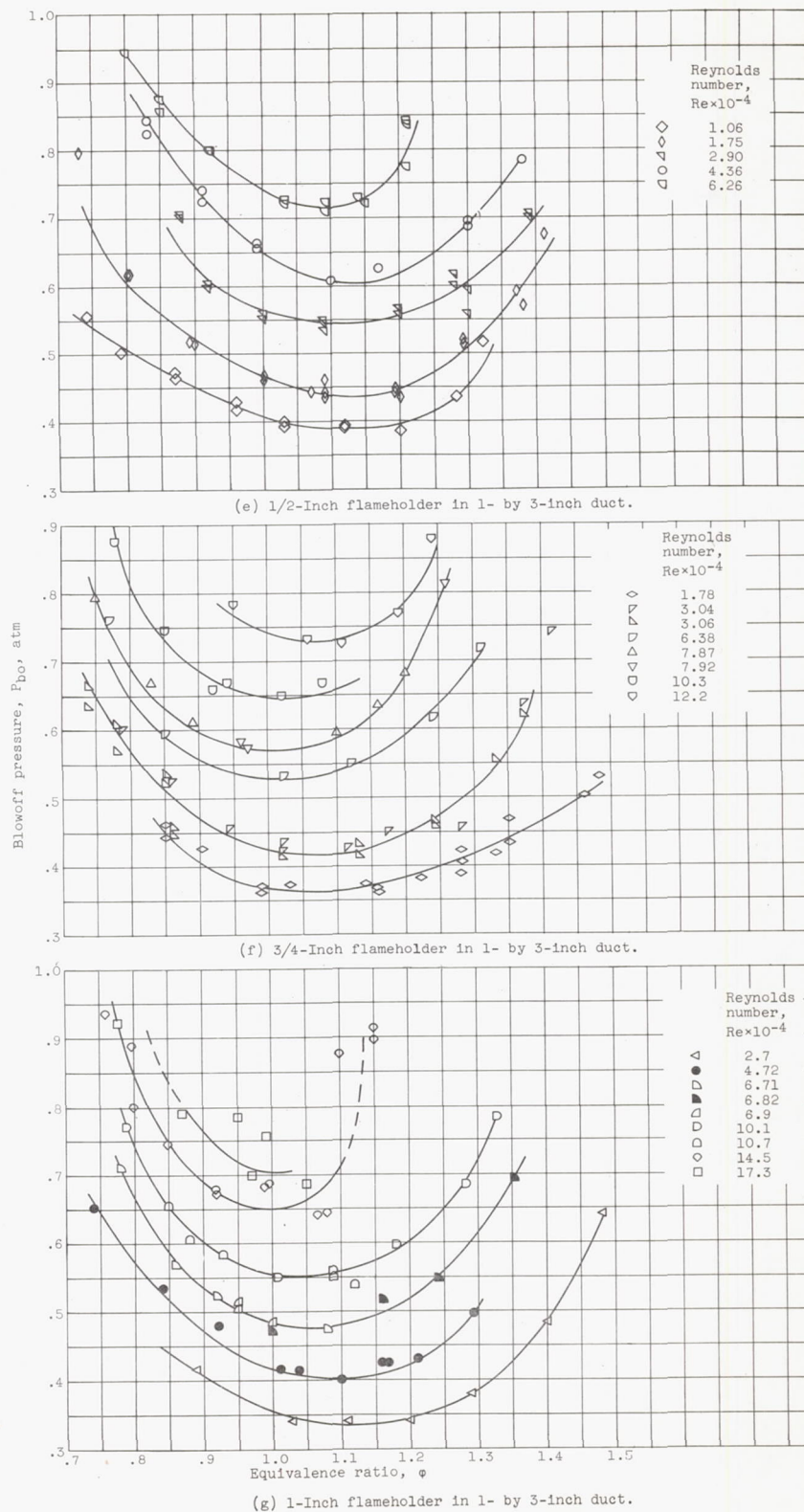
Figure 3. - Concluded. Variation of blowoff pressure with fuel concentration for different Reynolds numbers.
