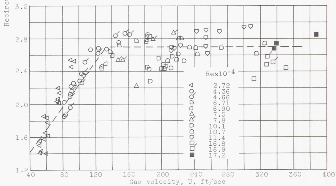
Figure 8. - Continued. Recirculation-zone length as function of gas velocity.
