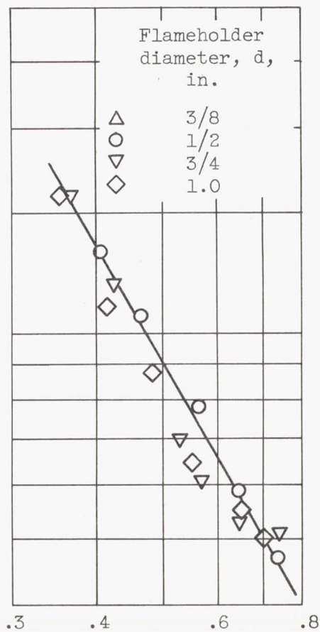
(b) 1- By 3-inch duct.
