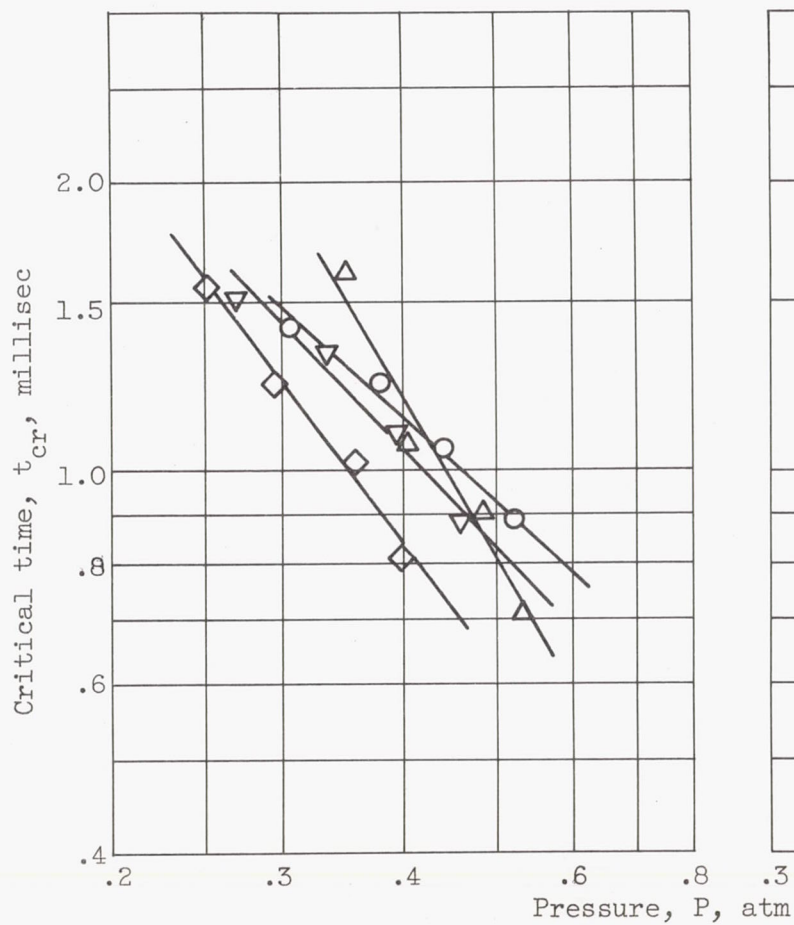
(a) 3- By 3-inch duct.
