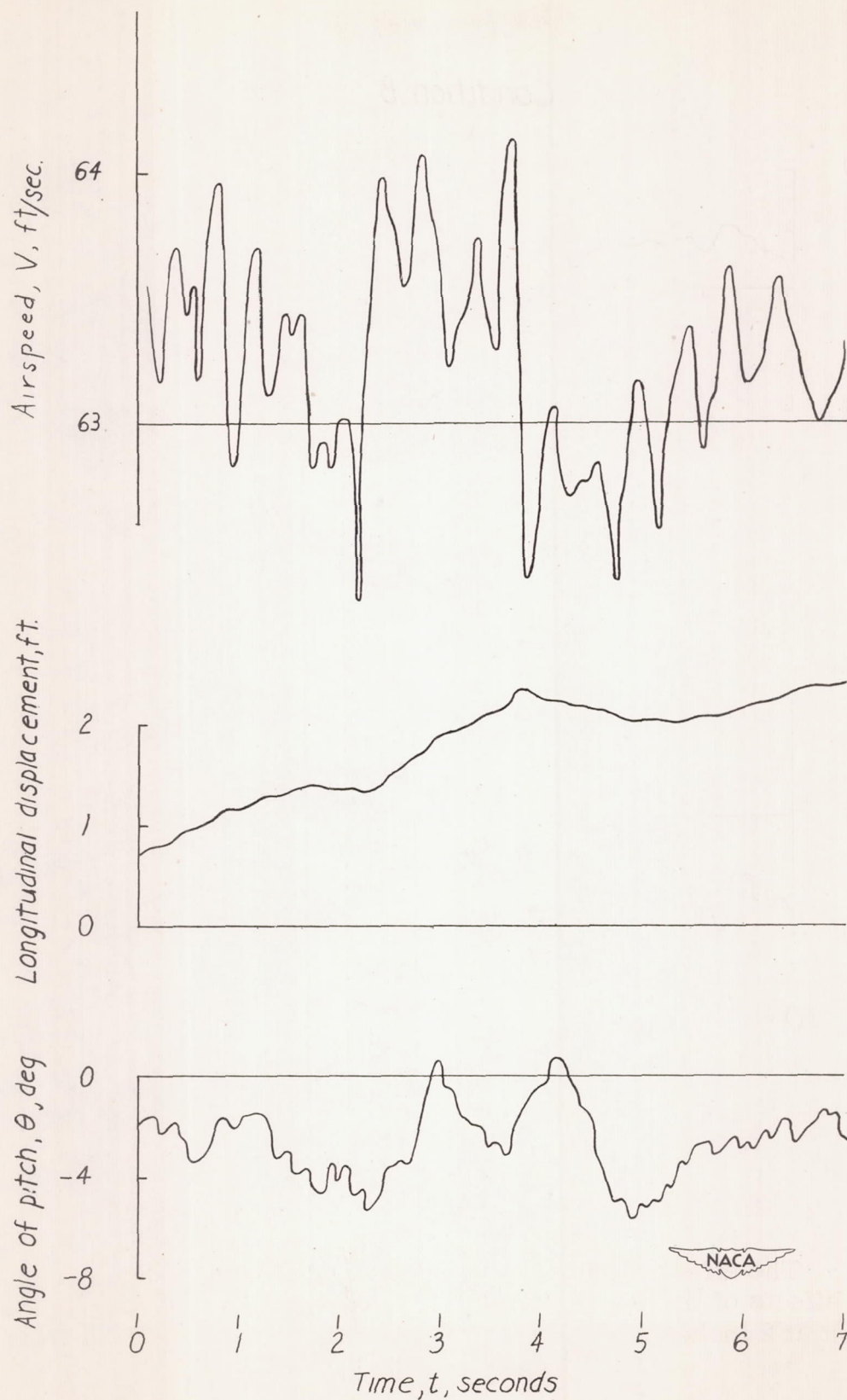
Figure 15.- Time histories of the longitudinal motions of the model for mass condition A_3 .
