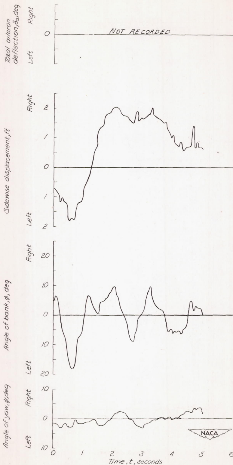
Figure 5(b).- Time histories of the lateral motions of the model for mass condition A_2 .
