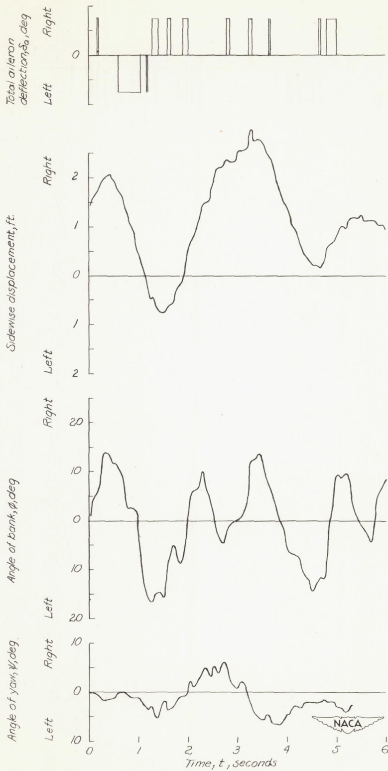
Figure 6(d).- Time histories of the lateral motions of the model for mass condition B_4 .
