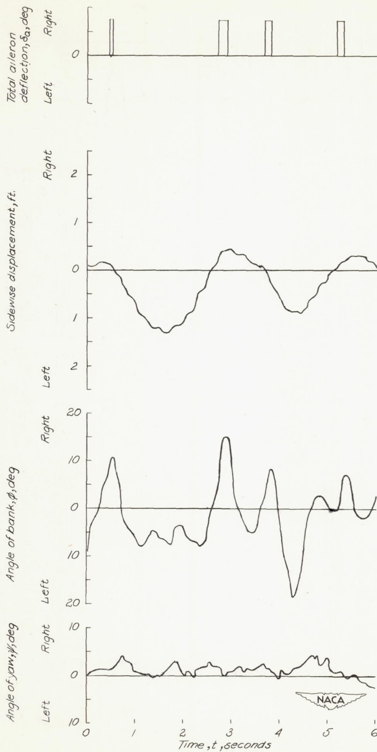
Figure 8(b).- Time histories of the lateral motions of the model for mass condition D_2 .
