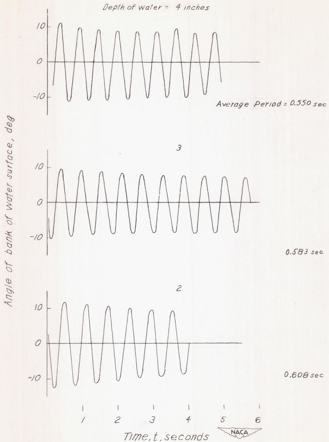
Figure 9.- Time histories of the natural motion of two, three, and four inches of water in the tanks following a disturbance.
