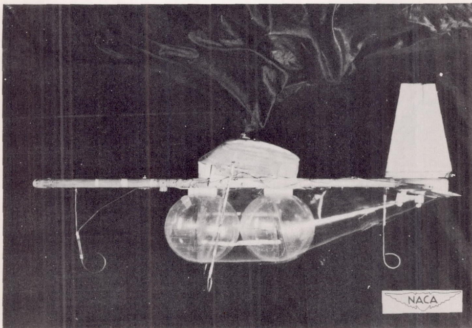
Figure 3(a).- Three-quarter-rear and side views of the model used in the fuel-sloshing investigation.
