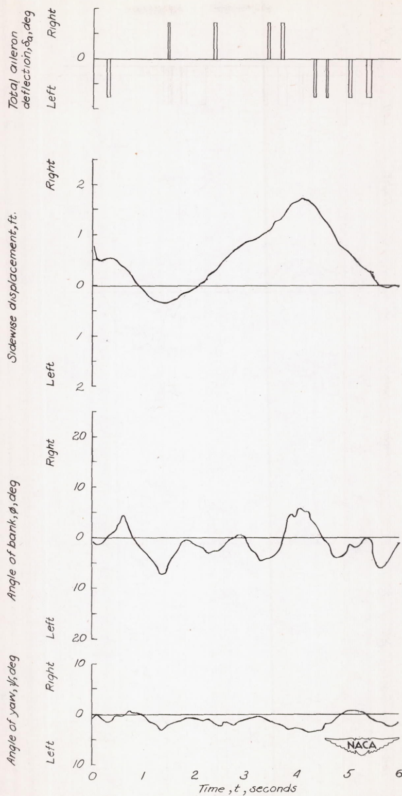
Figure 6(a).- Time histories of the lateral motions of the model for mass condition B_0 .
