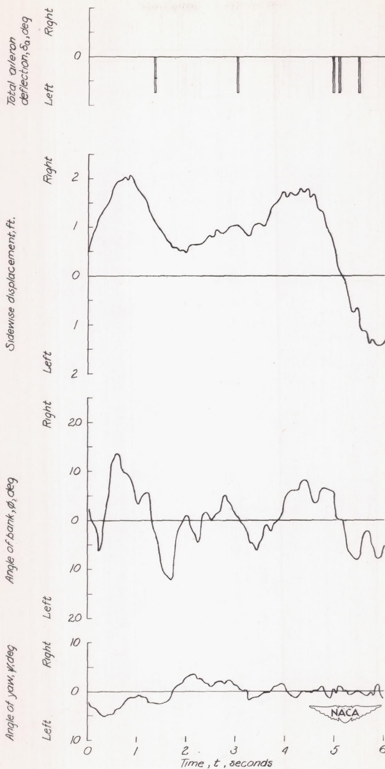
Figure 6(c).- Time histories of the lateral motions of the model for mass condition B_3 .
