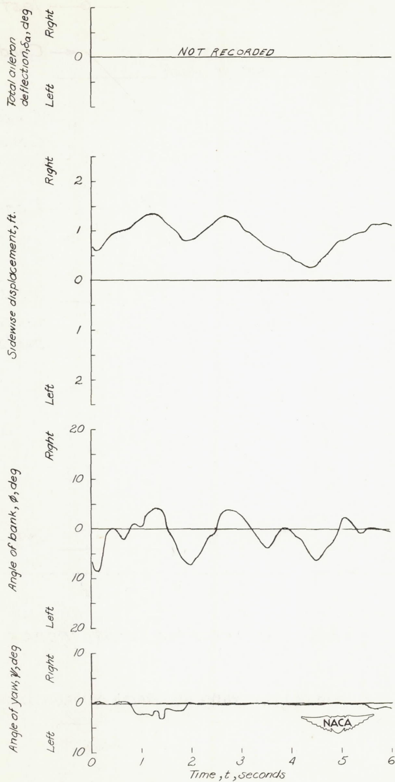
Figure 5(a).- Time histories of the lateral motions of the model for mass condition A_0 .
