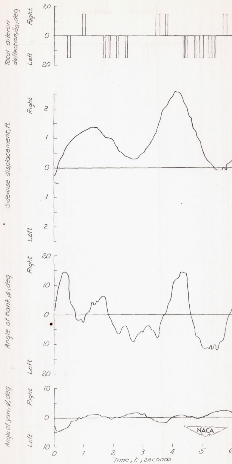
Figure 8(a).- Time histories of the lateral motions of the model for mass condition D_0 .
