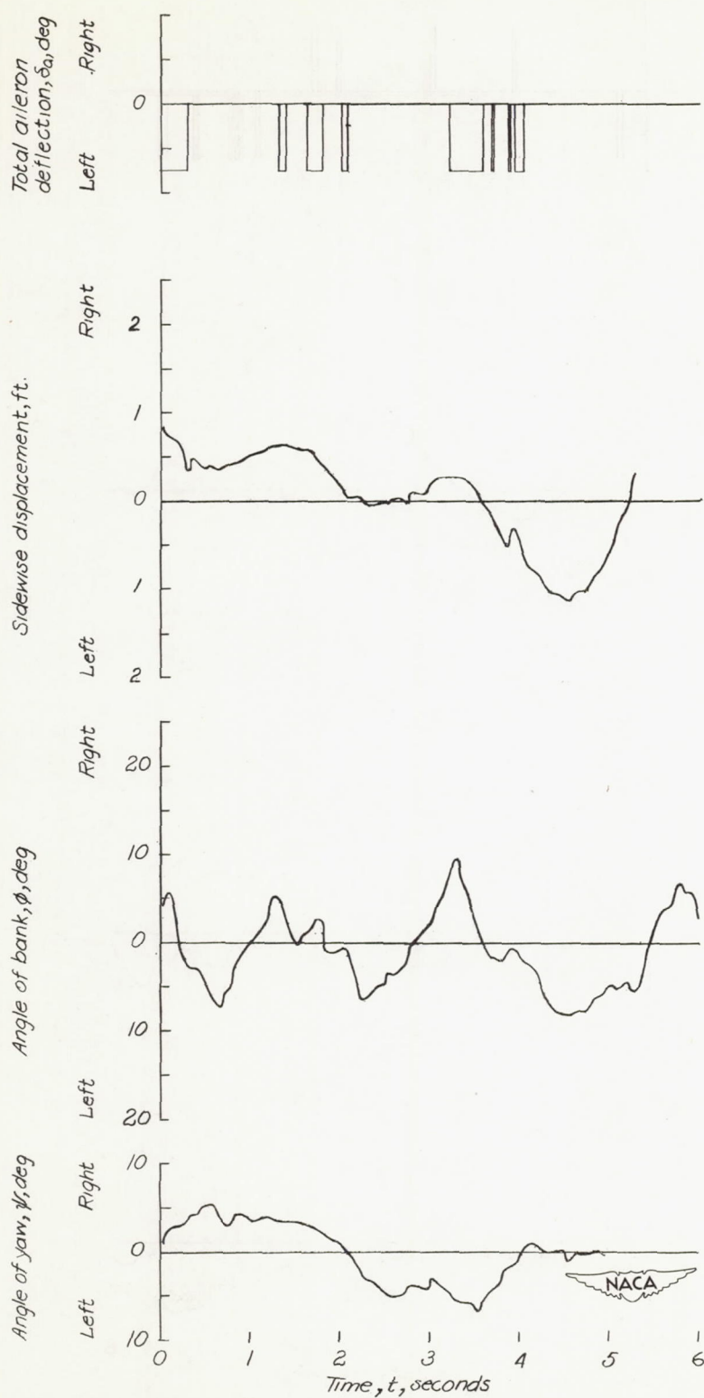
Figure 6(b).- Time histories of the lateral motions of the model for mass condition B_2 .
