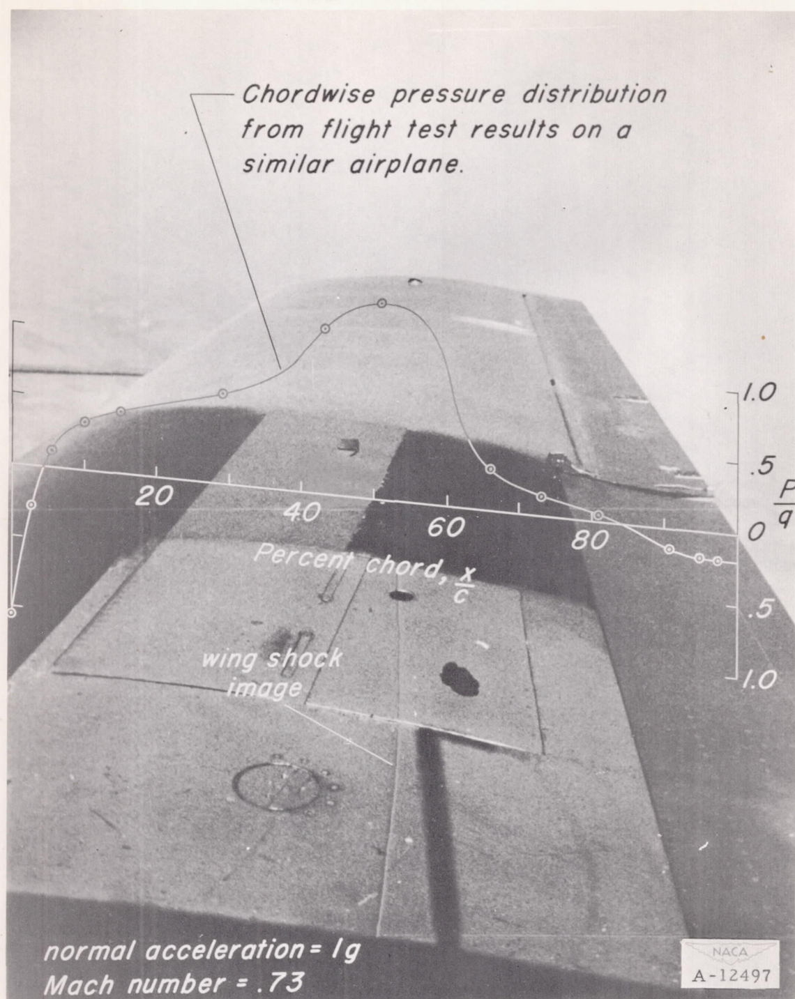
Figure 4.— Comparison of shock-wave image position with pressure distribution measured in flight on a similar airplane.
