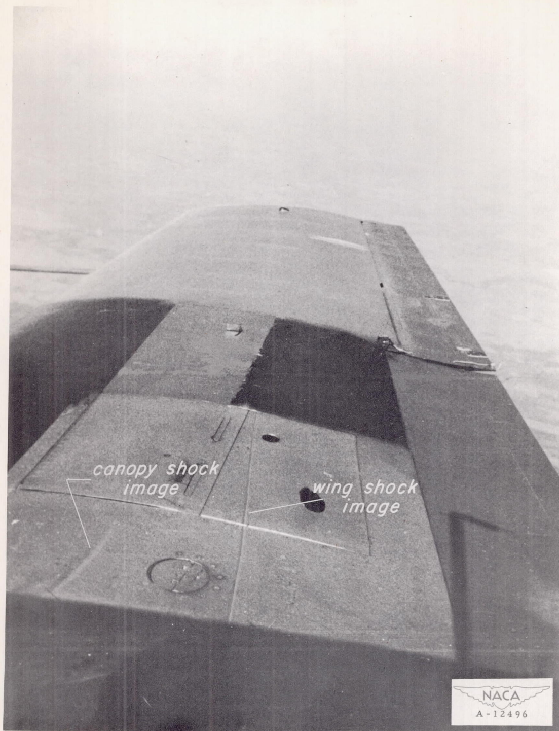
Figure 1.— Examples of shock-wave images photographed in flight.
