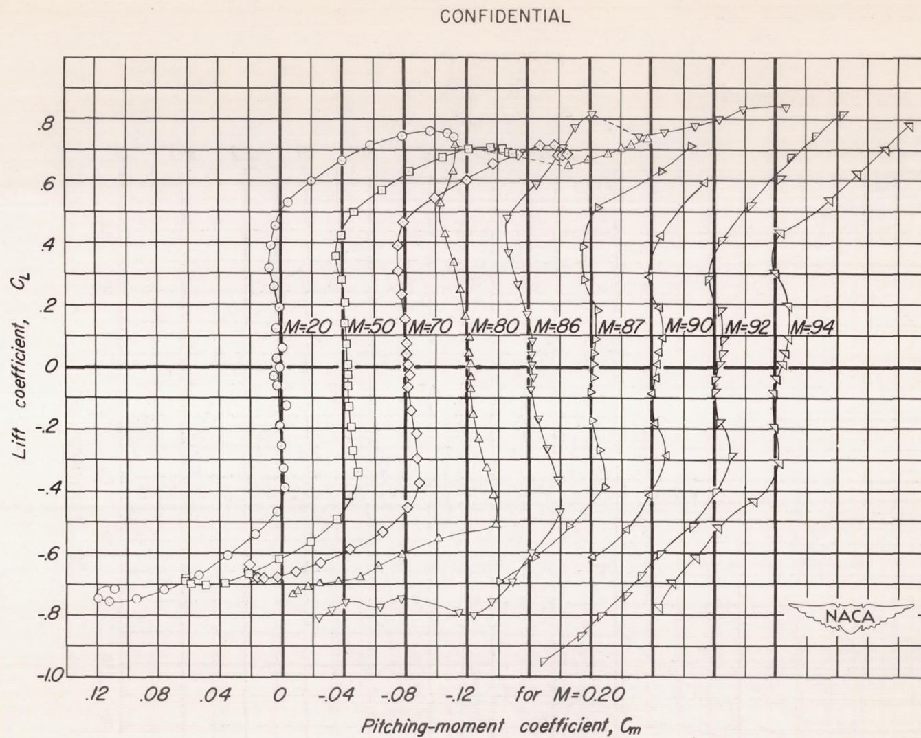
(b) C_m vs C_L Figure 10.-Continued.
