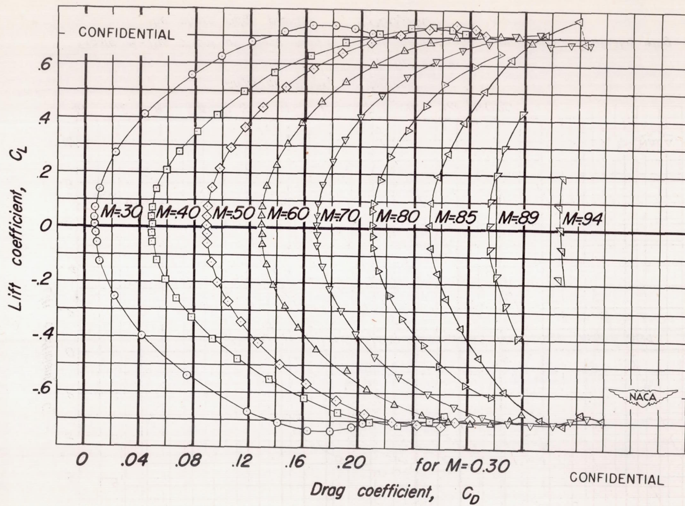
(c) C_D vs C_L Figure 3.-Concluded.
