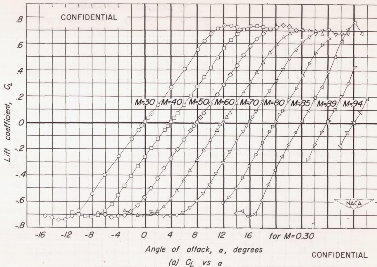
Figure 3.-The effect of Mach number on the aerodynamic characteristics of the wing with the sharp ridge profile. R , 3,000,000.
