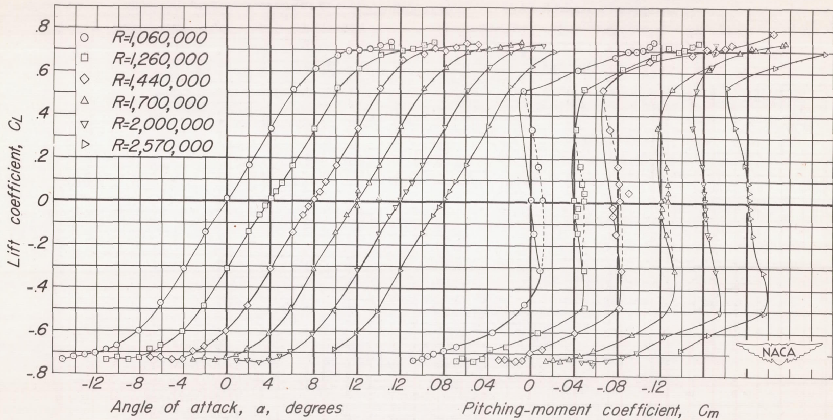
Figure 7.-The effect of Reynolds number on the aerodynamic characteristics of the wing with the sharp ridge profile. M , 0.80.
