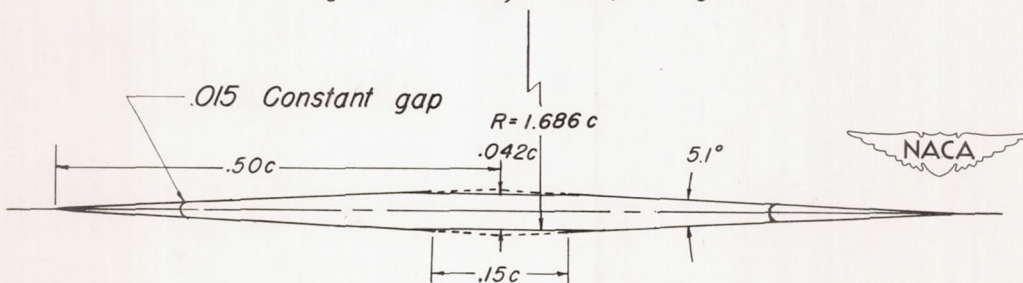
Modified section, round ridge
