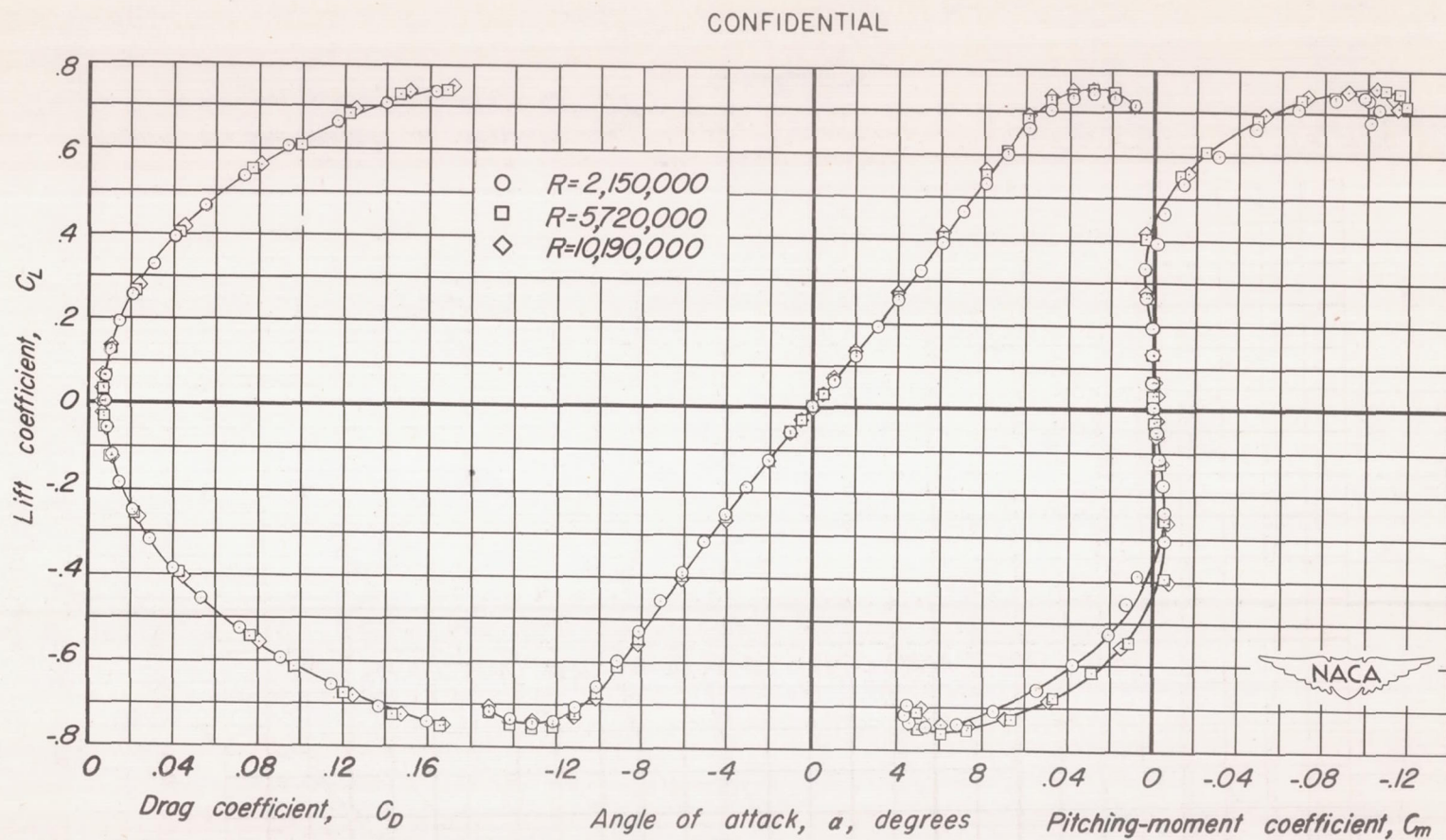
Figure 5.-The effect of Reynolds number on the aerodynamic characteristics of the wing with the sharp ridge profile. M, 0.20 .
