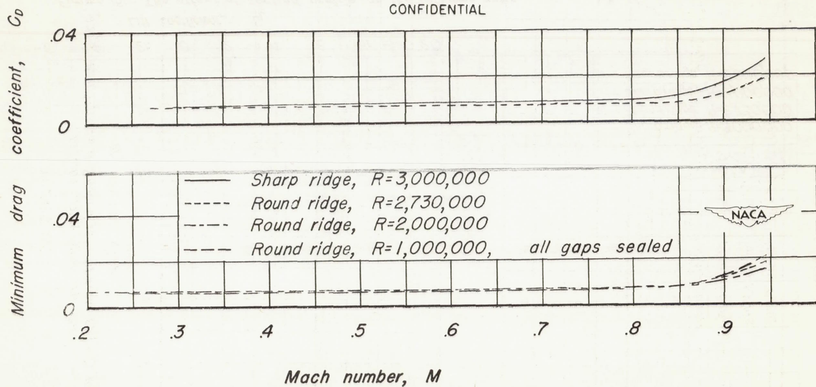
Figure 14.- The variation of minimum drag coefficient with Mach number.
