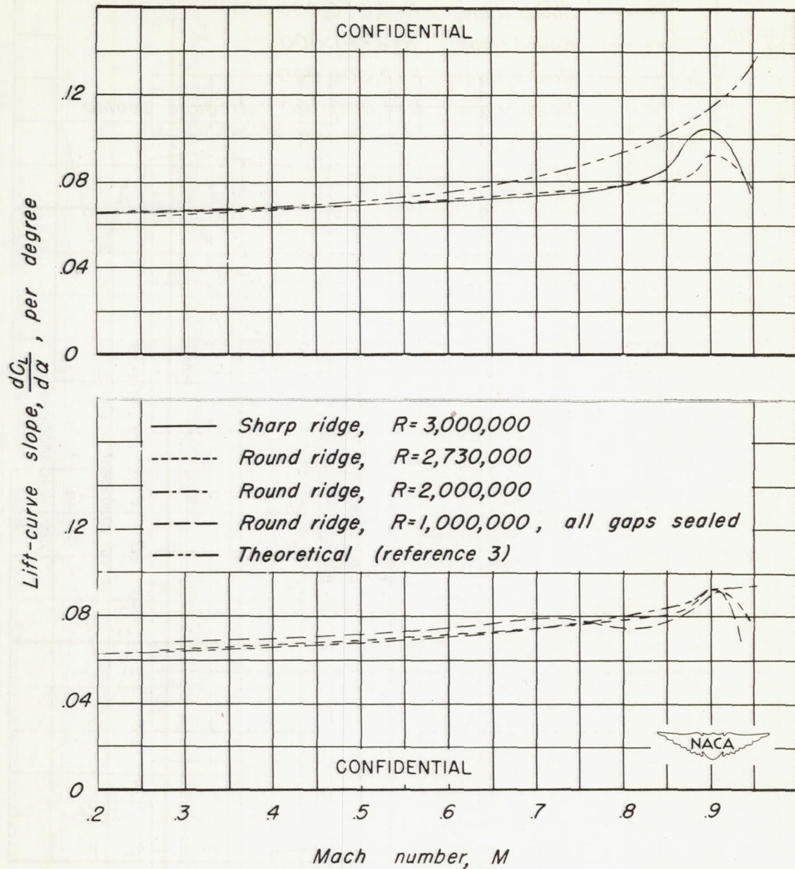
Figure 12.-The variation of lift-curve slope at zero lift with Mach number.
