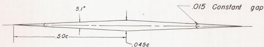
Original section, Sharp ridge
