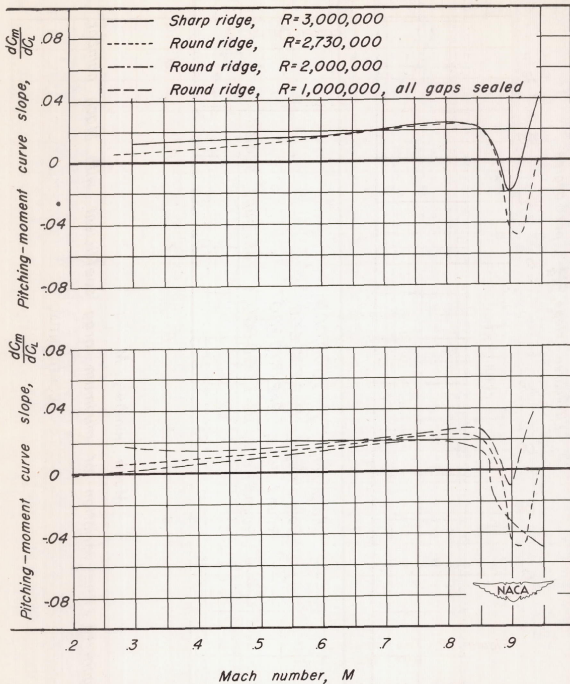
Figure 13.-The variation of pitching-moment-curve slope at zero lift with Mach number.
