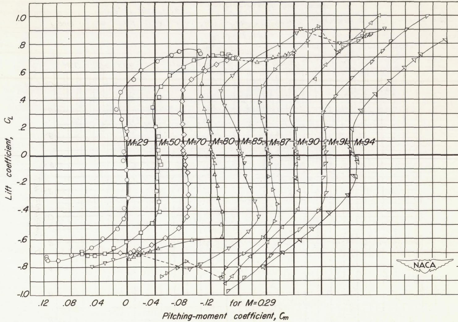
(b) C_m vs C_L Figure 11.-Continued.
