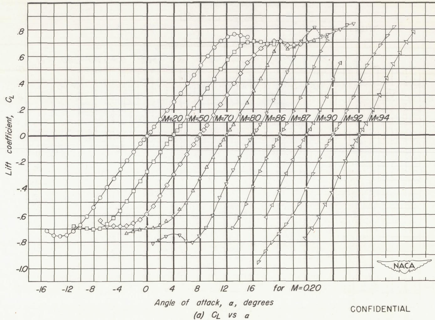
Figure 10.-The effect of Mach number on the aerodynamic characteristics of the wing with the round ridge profile. R , 2,000,000.
