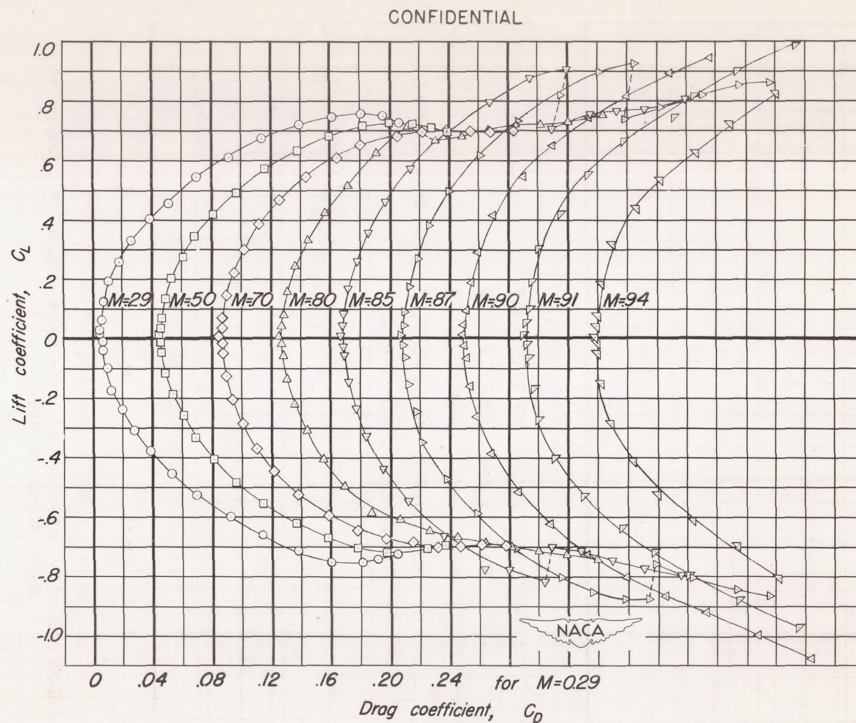
(c) C_D vs C_L Figure 11.-Concluded.
