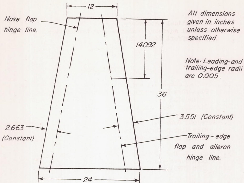
Wing plan form
