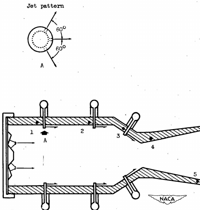
Figure 13. - Diagrammatic sketch of rocket engine cooled by individual jets. Wall thermocouples were located at five positions shown.
