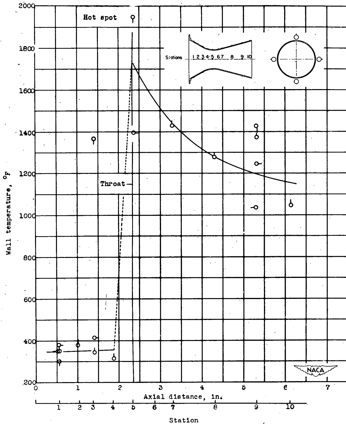
Figure 9. - Concluded. Effect of water from porous ring at flow of 3.5 percent of propellant flow on wall temperatures of thin-wall stainless-steel nozzle.
