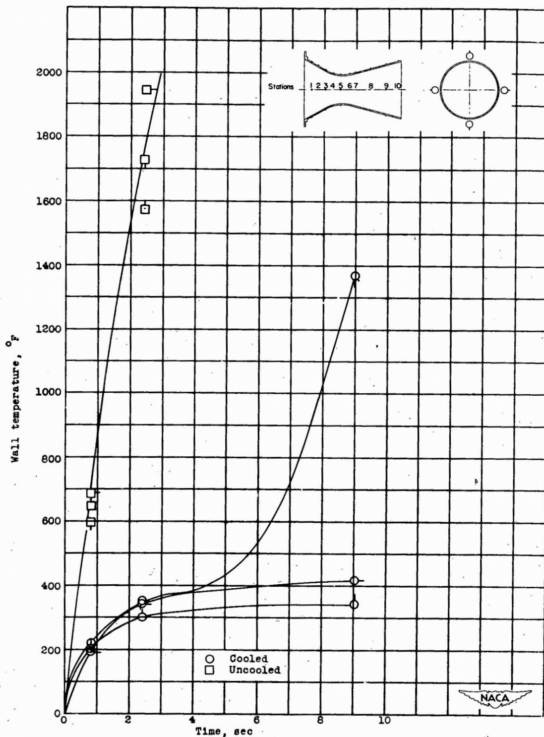
(b) Station 3 (convergent section ).
