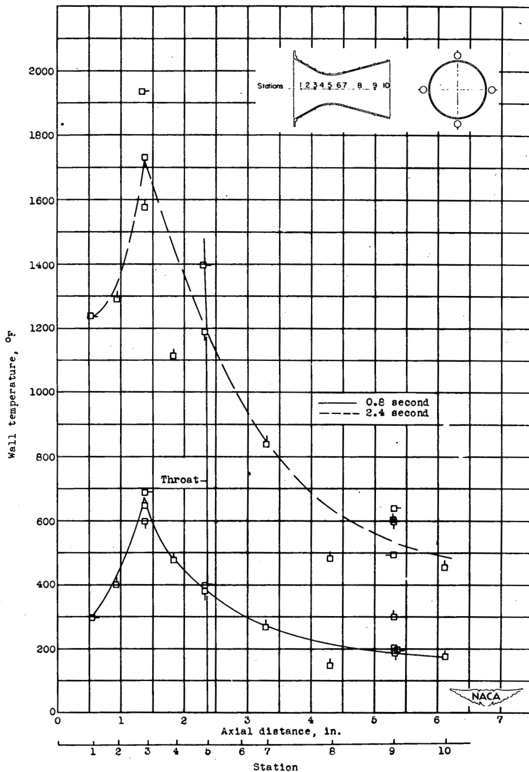
Figure 8. - Wall temperatures for uncooled thin-wall stainless-steel nozzle after 0.8 and 2.4 seconds.
