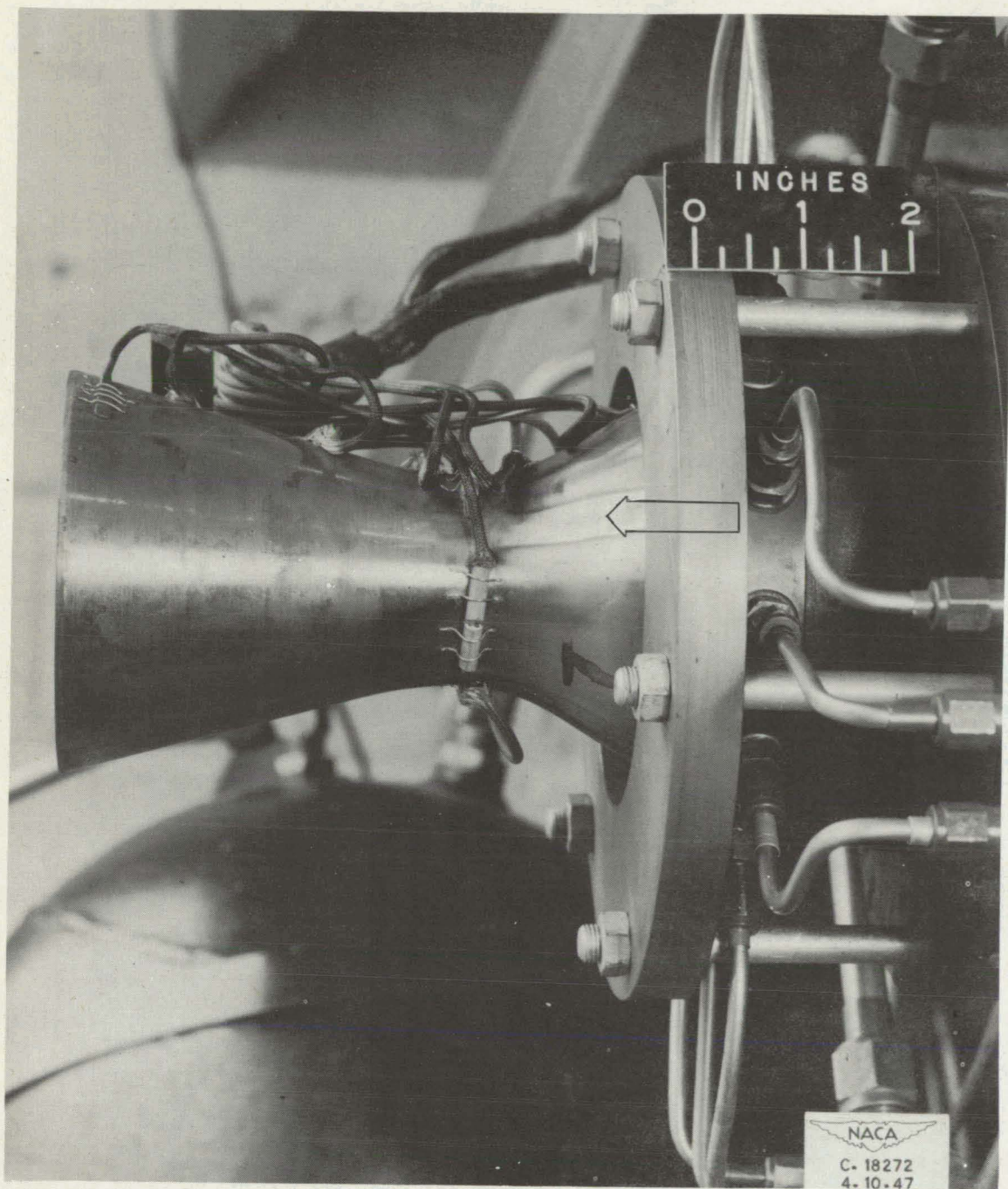
Figure 12. - Thin-wall stainless-steel nozzle after run with jet cooling along inner surface. Note heat patterns on convergent section.
