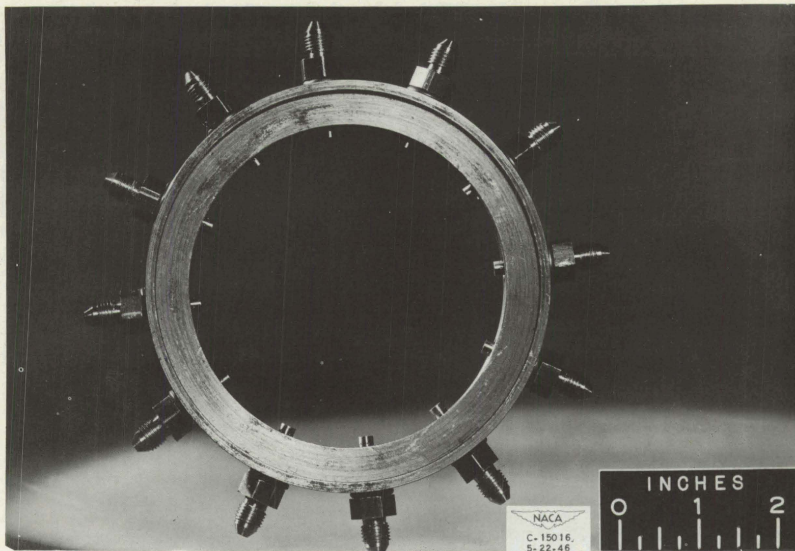
Figure 5. - Ring with twelve coolant injectors each with three directed jets.
