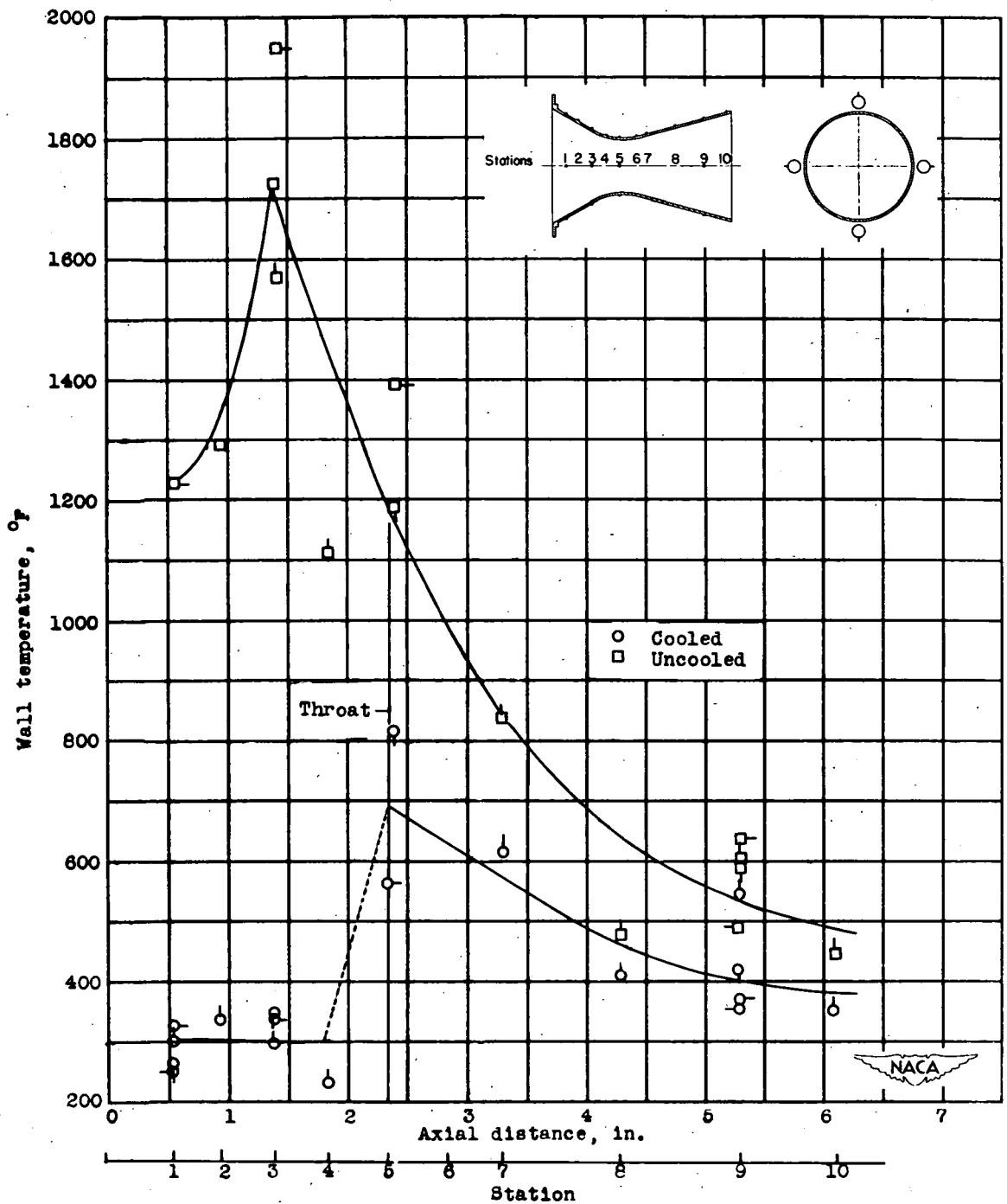
Figure 9. - Continued. Effect of water from porous ring at flow of 3.5 percent of propellant flow on wall temperatures of thin-wall stainless-steel nozzle.
