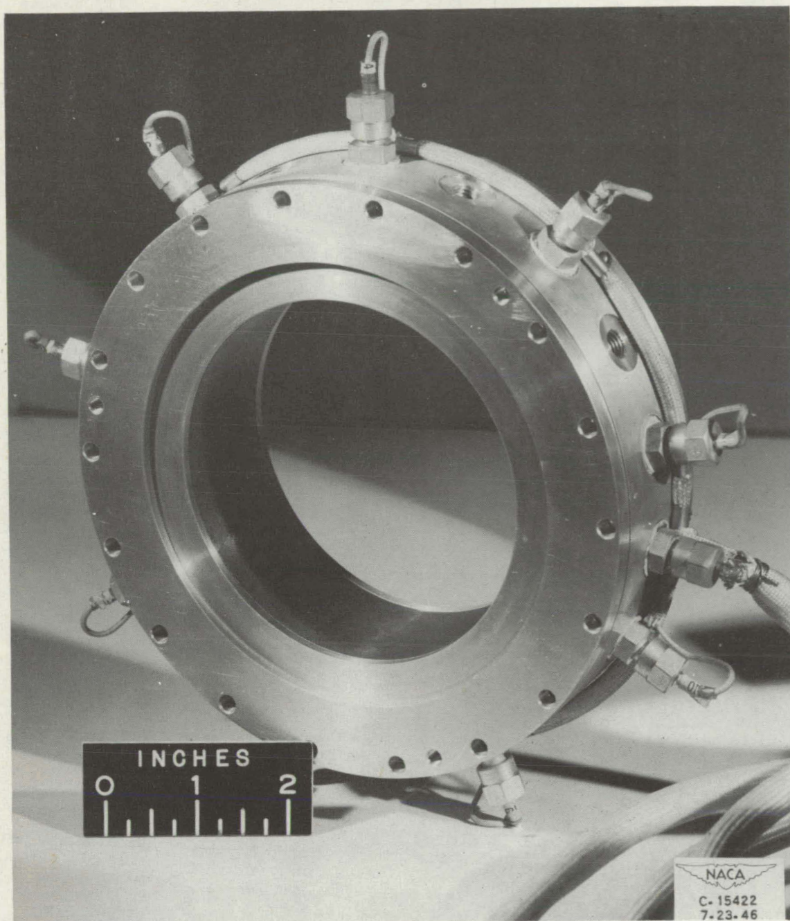
Figure 6. - Porous-metal ring and holder with thermocouples installed.
