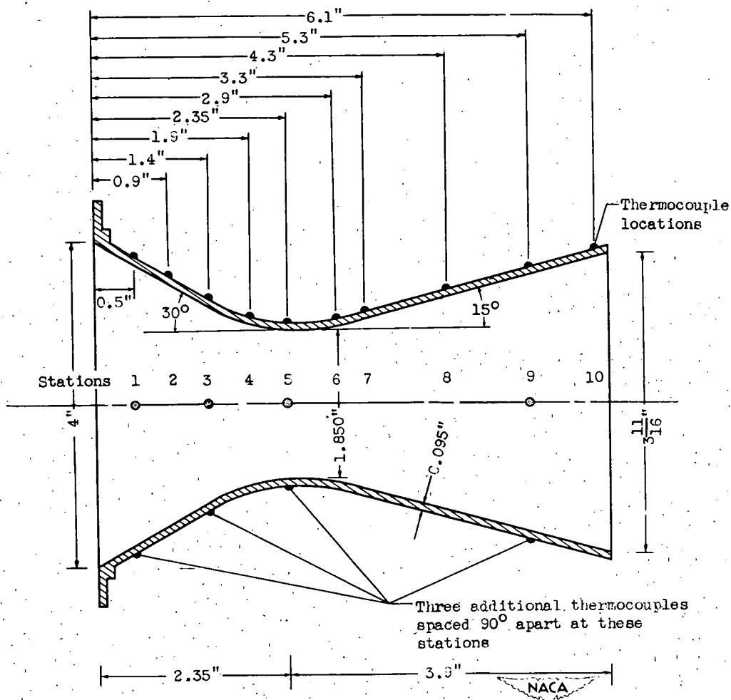
Figure 3. - Thin-wall stainless-steel nozzle showing location of ten thermocouples in straight line along nozzle contour and three additional circumferential thermocouples at each of stations 1, 3, 5, and 9.
