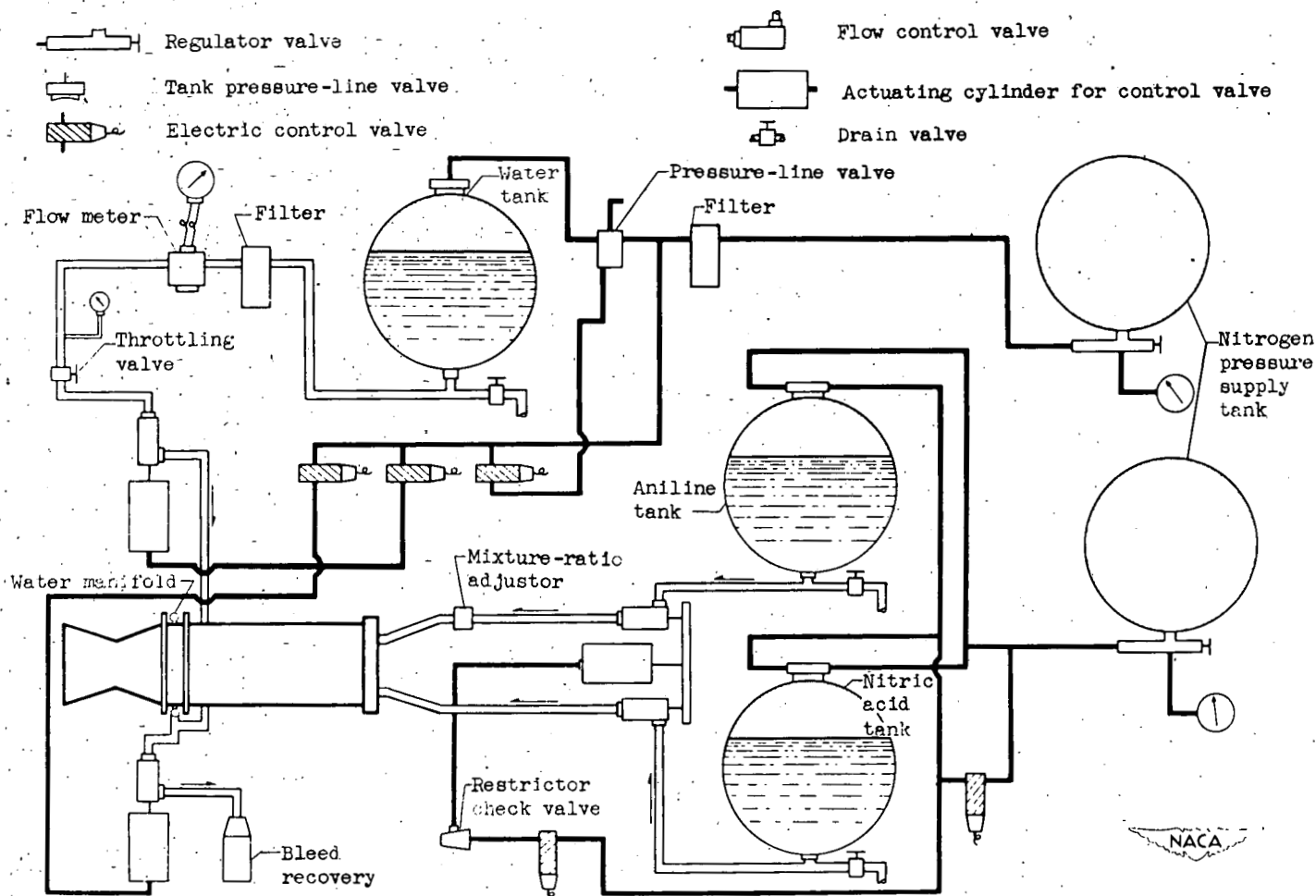
Figure 1. - Flow diagram of experimental 1000-pound thrust rocket engine using red fuming nitric acid and aniline as propellants and water as an internal coolant.
