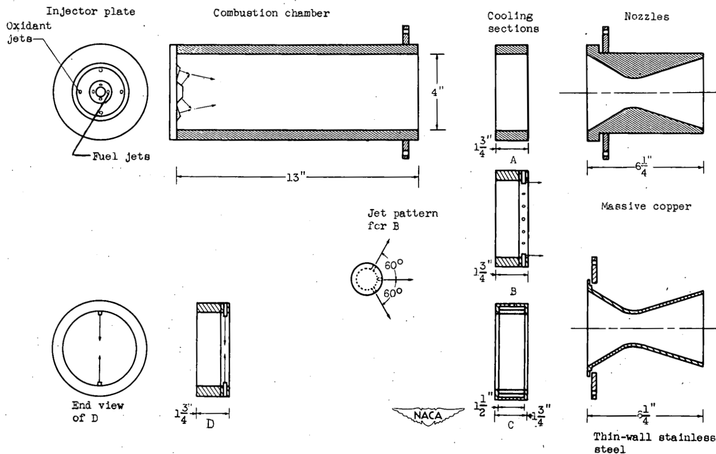
Figure 2. - Diagrammatic sketches of parts of rocket engine used in different combinations for nozzle-cooling experiments.
