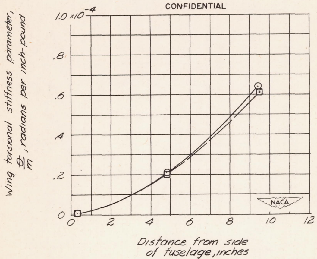
Figure 3.- Stiffness characteristics of two typical wings of the present tests.
