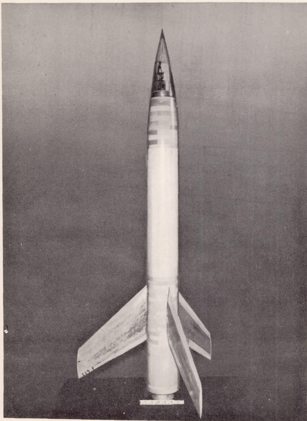
Figure 2.- Photograph of test vehicle.
