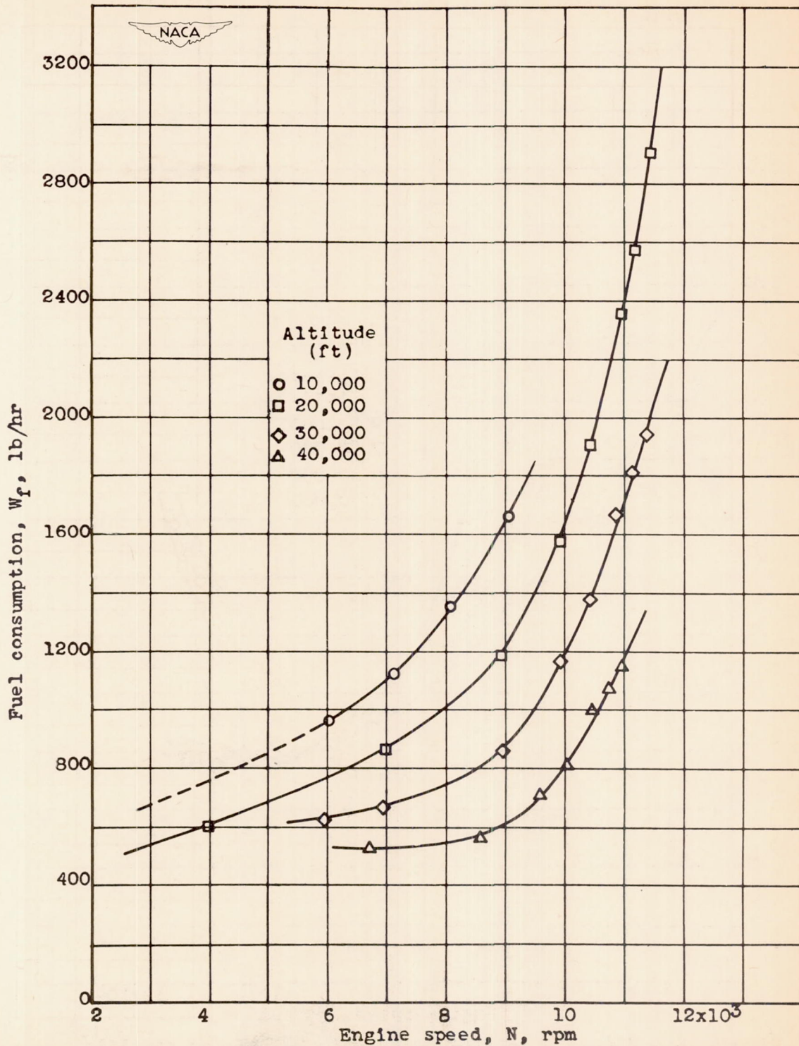
Figure 16.- Effect of engine speed and altitude on fuel consumption at ram pressure ratio of approximately 1.2.
