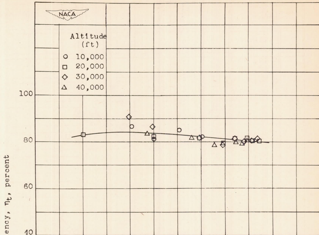
(a) Effect of altitude at ram pressure ratio of approximately 1.2.
