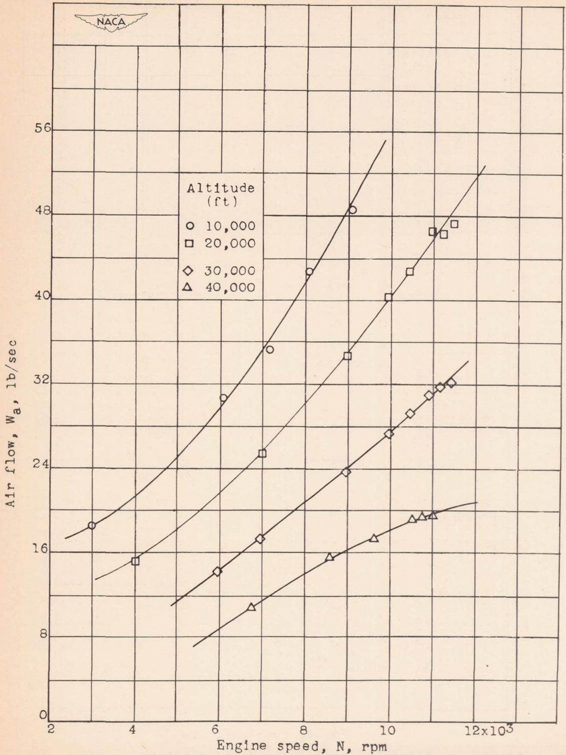
Figure 9.- Effect of engine speed and altitude on air flow at ram pressure ratio of approximately 1.2.
