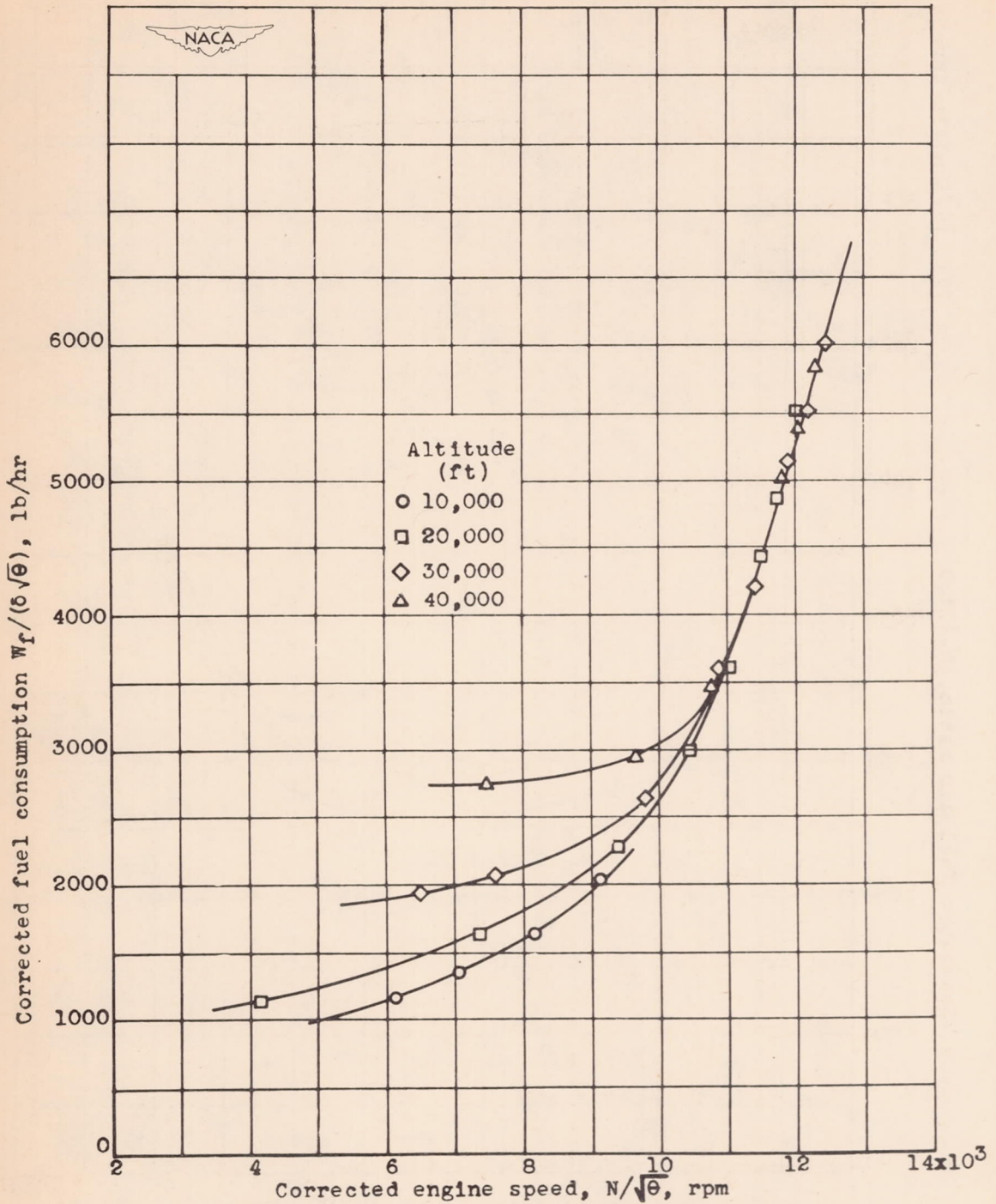
Figure 39.- Effect of corrected engine speed and altitude on corrected fuel consumption at ram pressure ratio of approximately 1.2. Engine speed and fuel consumption corrected to NACA standard atmospheric conditions at sea level.
