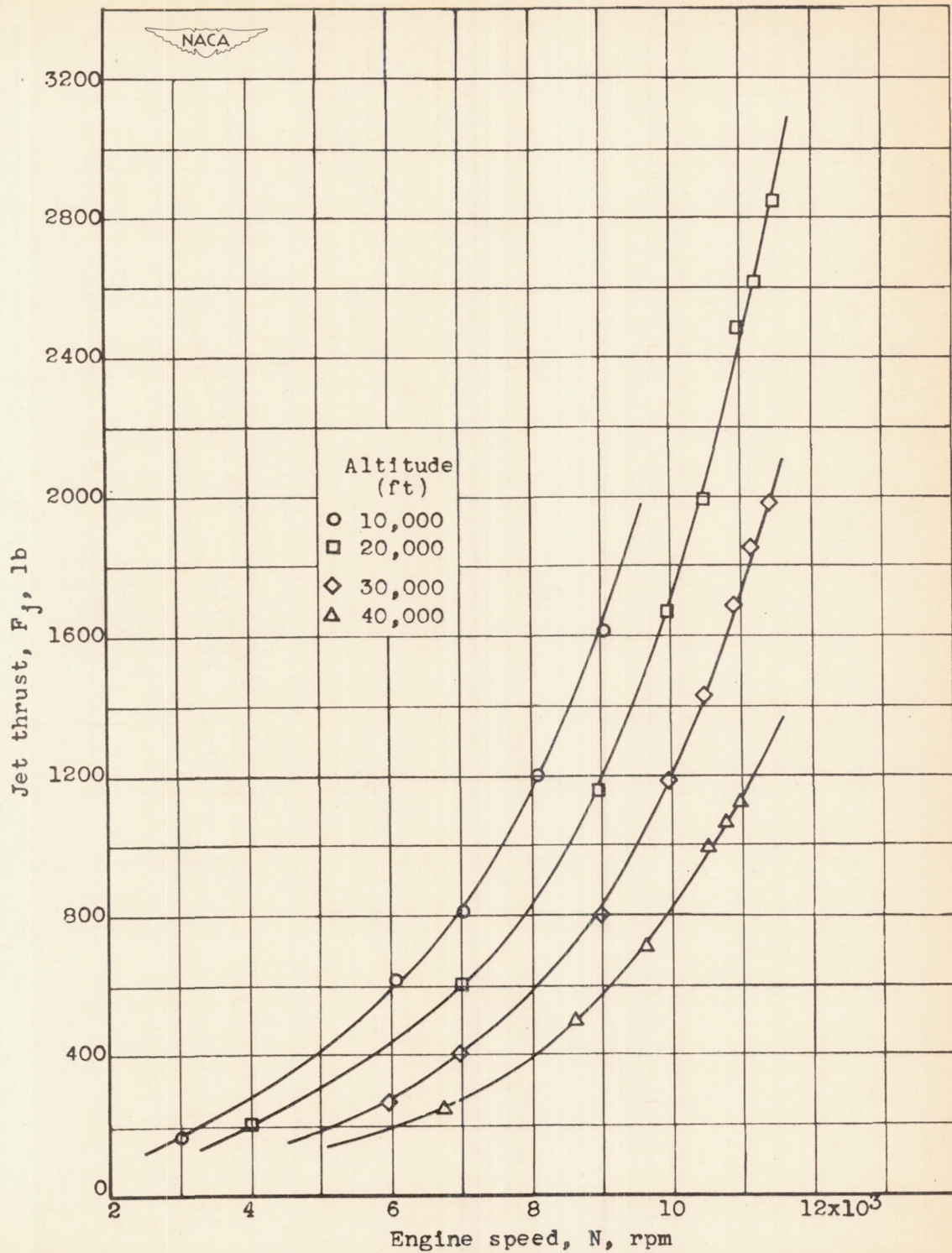
Figure 10.- Effect of engine speed and altitude on jet thrust at ram pressure ratio of approximately 1.2.
