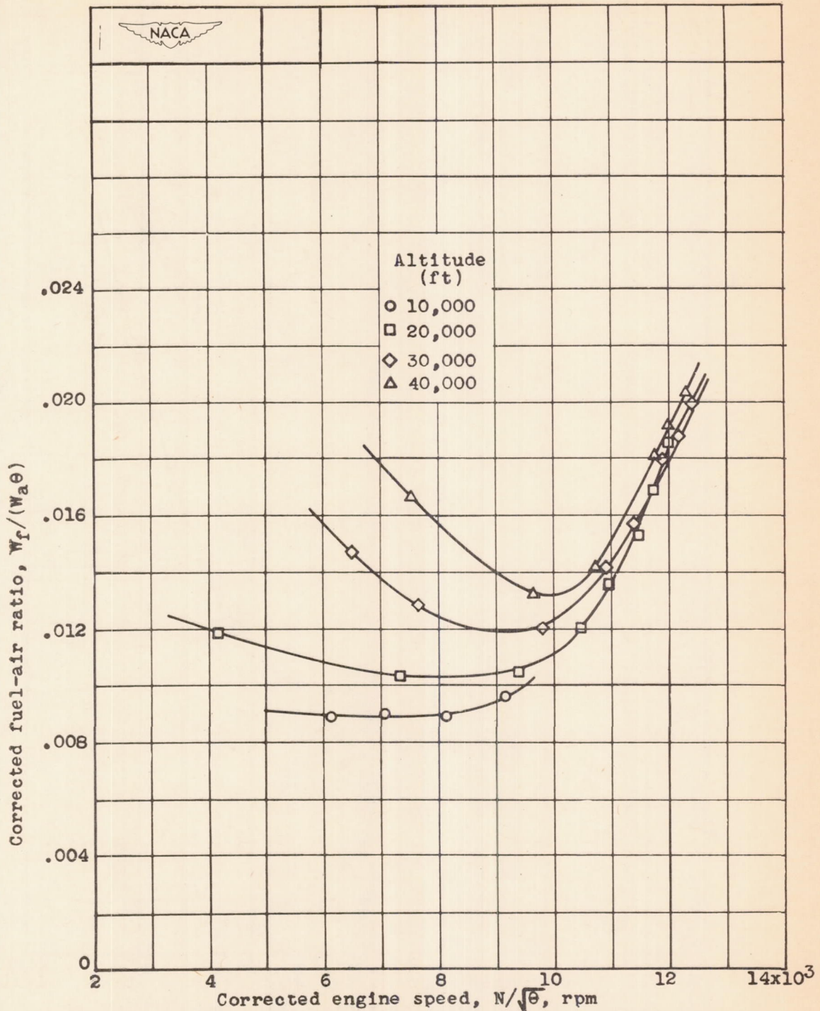
Figure 40.- Effect of corrected engine speed and altitude on corrected fuel-air ratio at ram pressure ratio of approximately 1.2. Engine speed and fuel-air ratio corrected to NACA standard atmospheric conditions at sea level.
