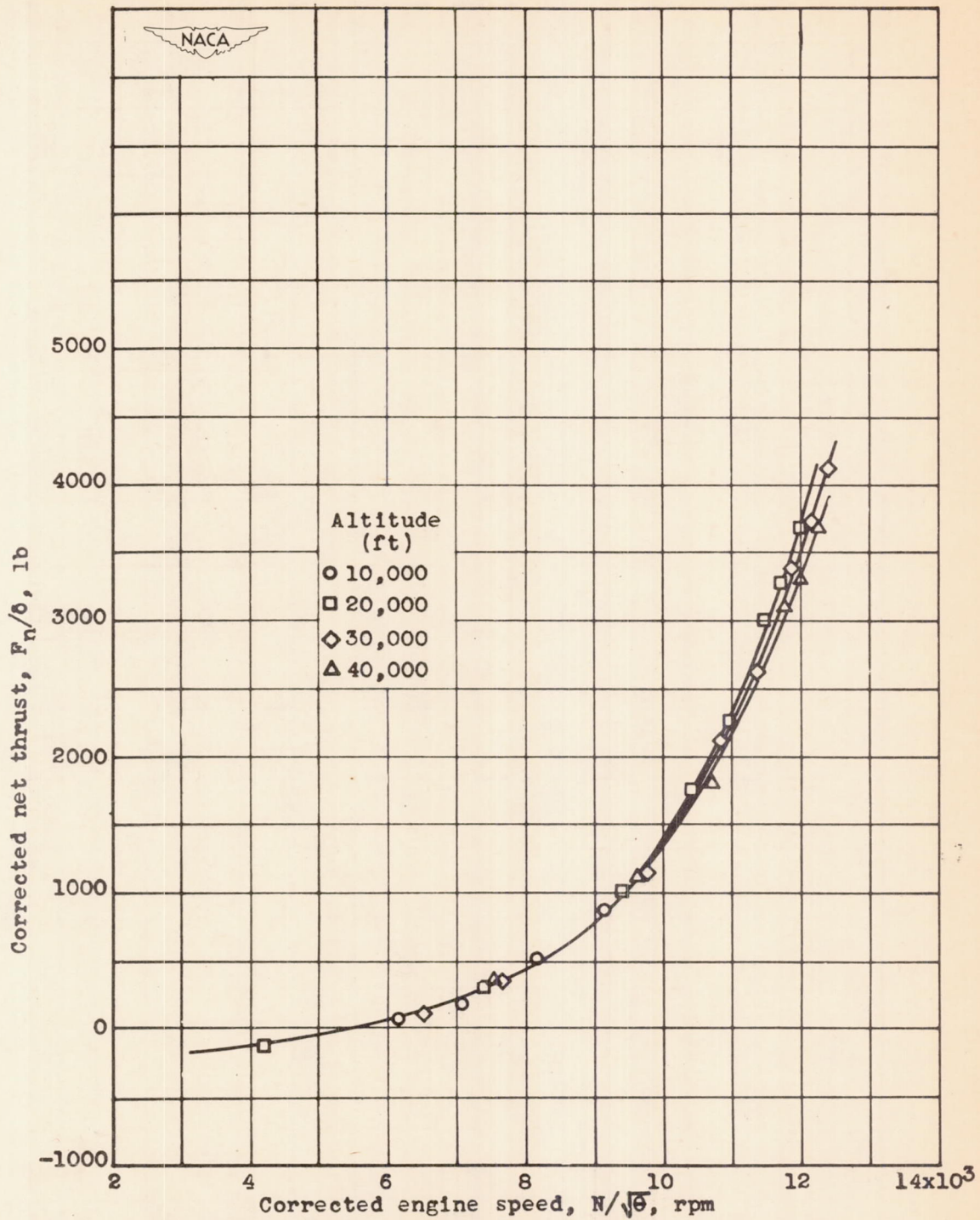
Figure 34.- Effect of corrected engine speed and altitude on corrected net thrust at ram pressure ratio of approximately 1.2. Engine speed and net thrust corrected to NACA standard atmospheric conditions at sea level.
