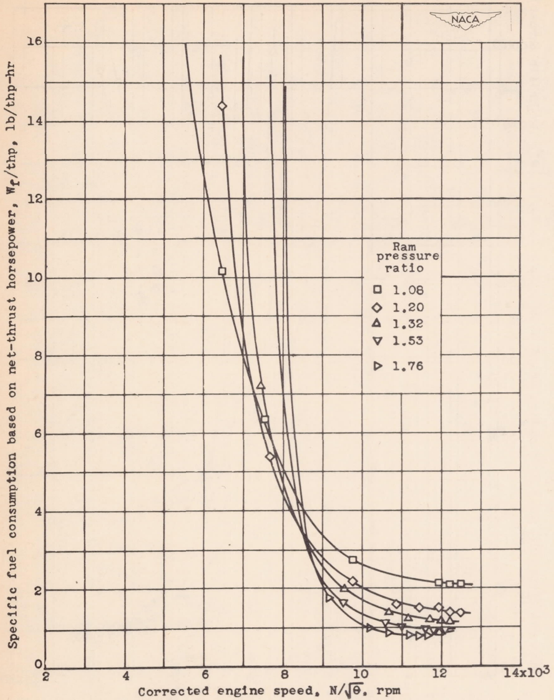
Figure 45.- Effect of corrected engine speed and ram pressure ratio on specific fuel consumption based on net-thrust horsepower at altitude of 30,000 feet. Engine speed corrected to NACA standard atmospheric conditions at sea level.
