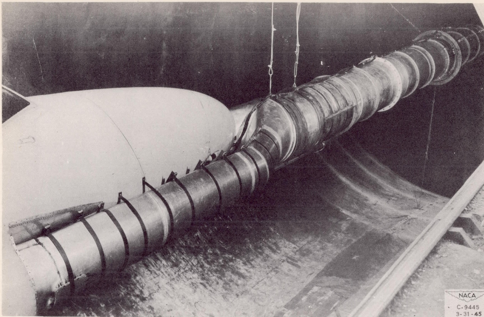
Figure 4. - Y-shaped ram pipe attached to nose of airplane.
