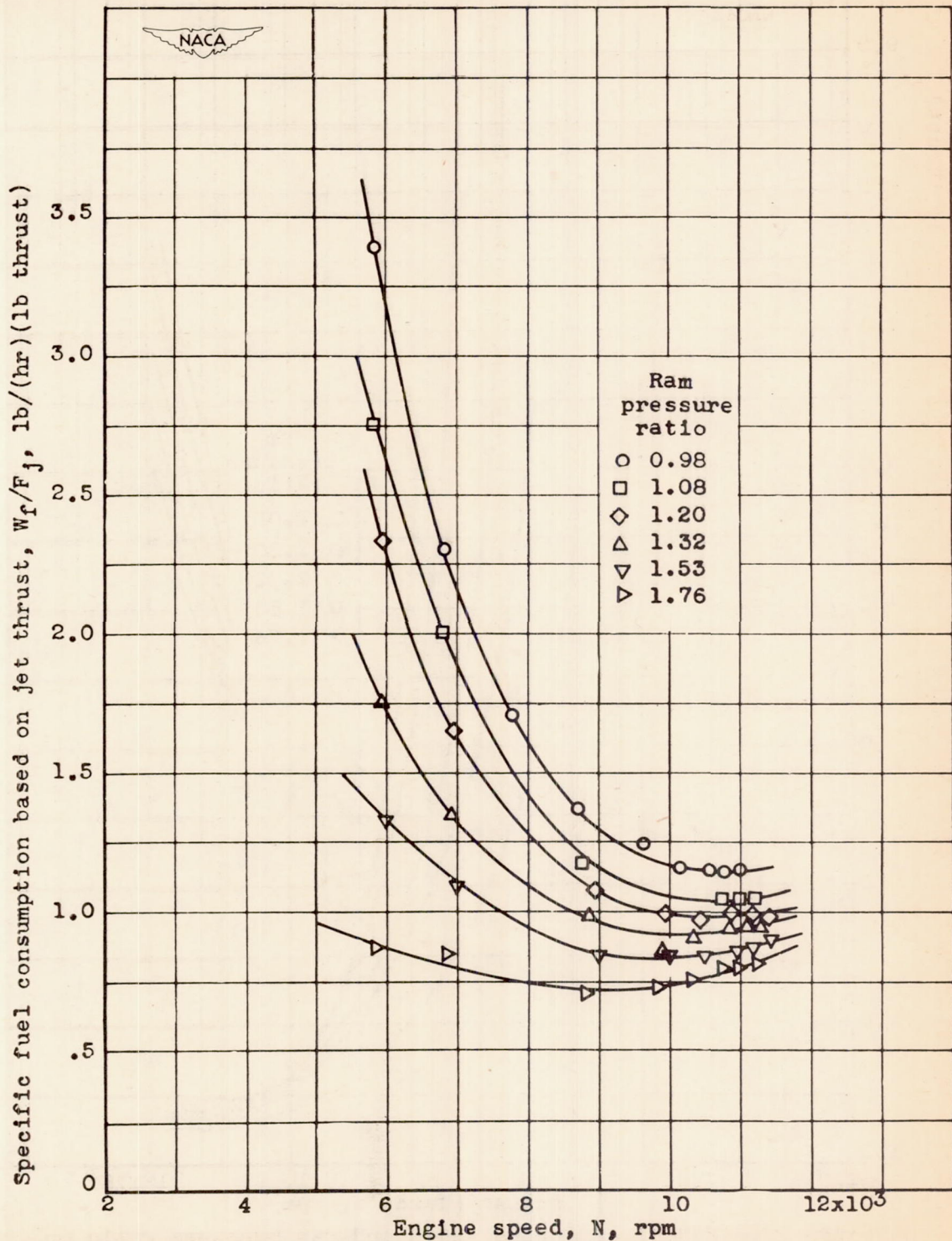
Figure 24.- Effect of engine speed and ram pressure ratio on specific fuel consumption based on jet thrust at altitude of 30,000 feet.
