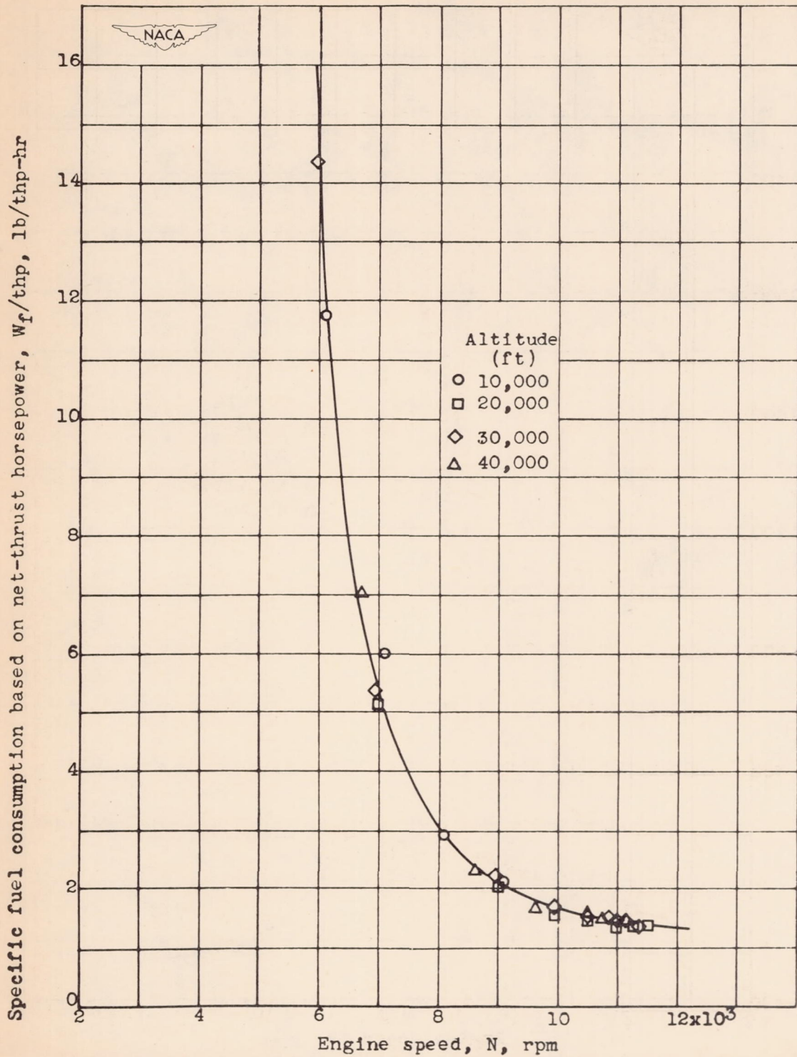
Figure 13.- Effect of engine speed and altitude on specific fuel consumption based on net-thrust horsepower at ram pressure ratio of approximately 1.2.
