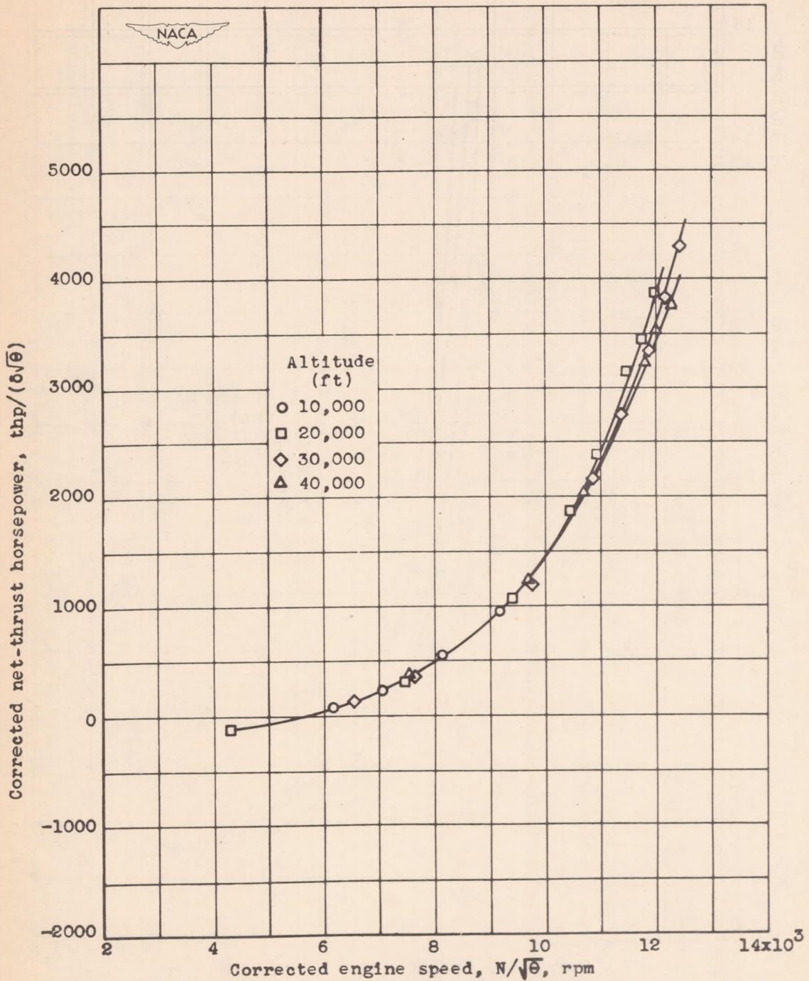
Figure 35.- Effect of corrected engine speed and altitude on corrected net-thrust horsepower at ram pressure ratio of approximately 1.2. Engine speed and net-thrust horsepower corrected to NACA standard atmospheric conditions at sea level.
