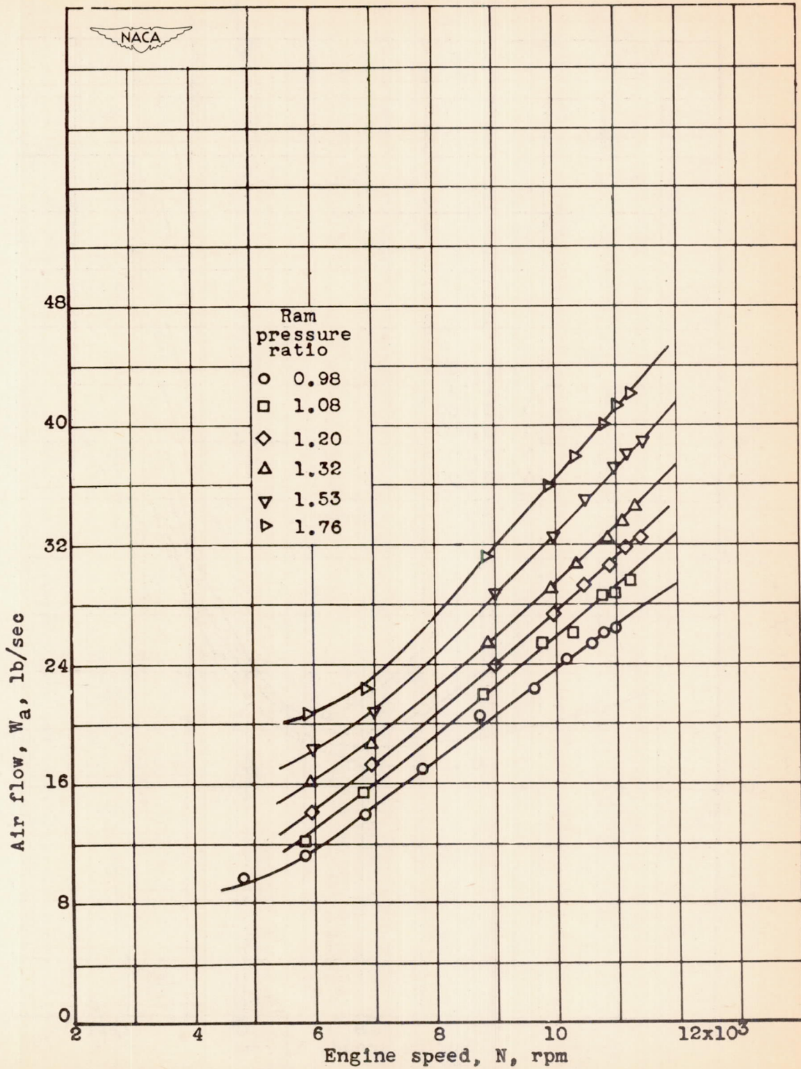
Figure 18.- Effect of engine speed and ram pressure ratio on air flow at altitude of 30,000 feet.
