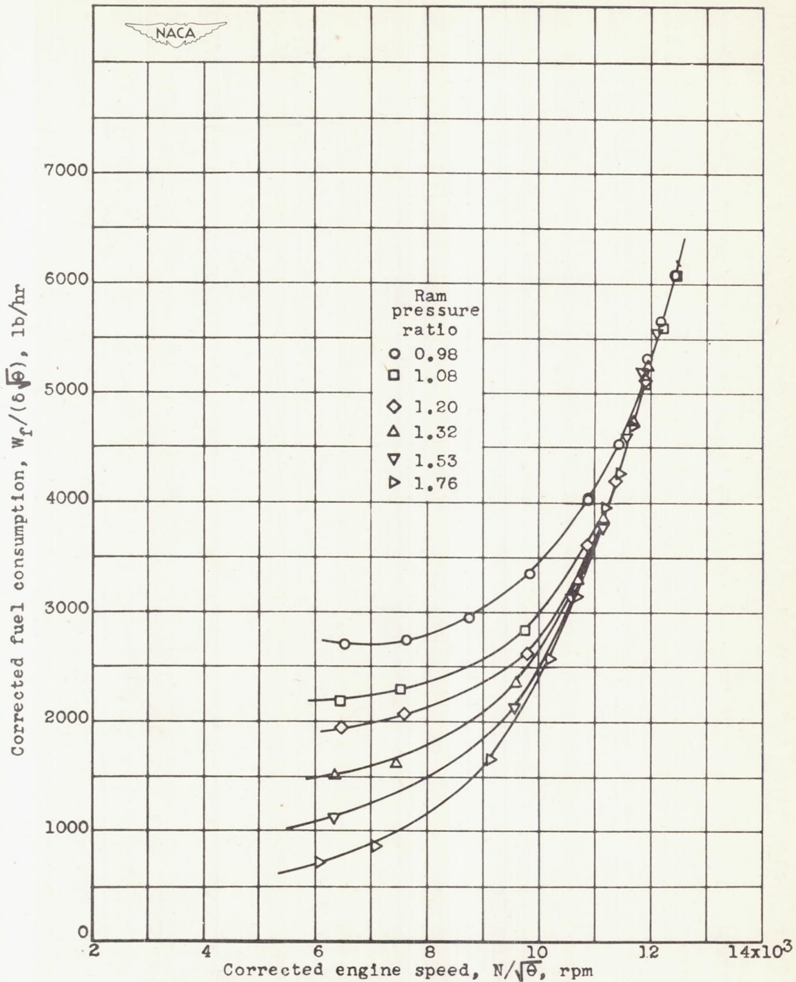
Figure 48.- Effect of corrected engine speed and ram pressure ratio on corrected fuel consumption at altitude of 30,000 feet. Engine speed and fuel consumption corrected to NACA standard atmospheric conditions at sea level.
