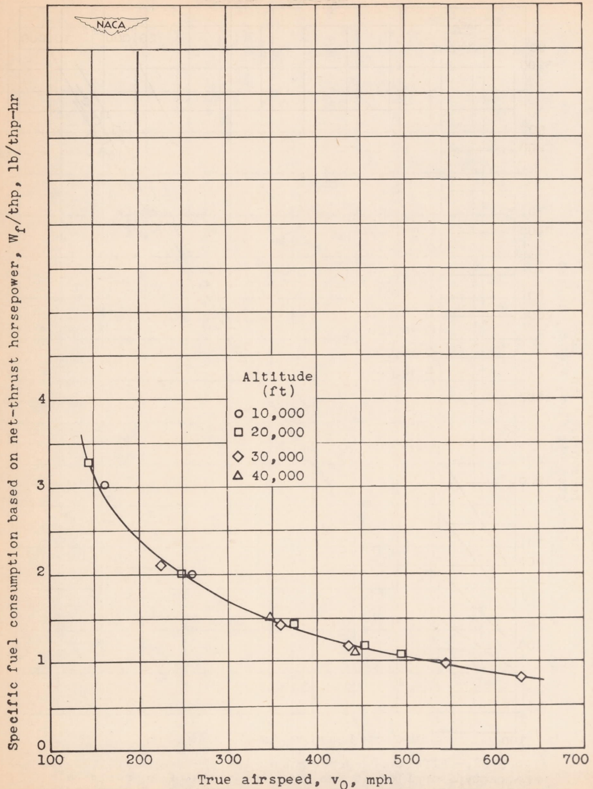
Figure 31.- Effect of true airspeed and altitude on specific fuel consumption based on net-thrust horsepower at engine speed of 11,500 rpm.
