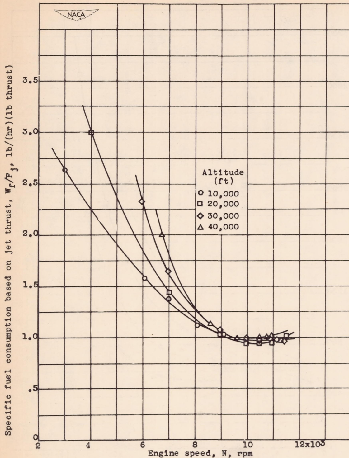
Figure 15.- Effect of engine speed and altitude on specific fuel consumption based on jet thrust at ram pressure ratio of approximately 1.2.
