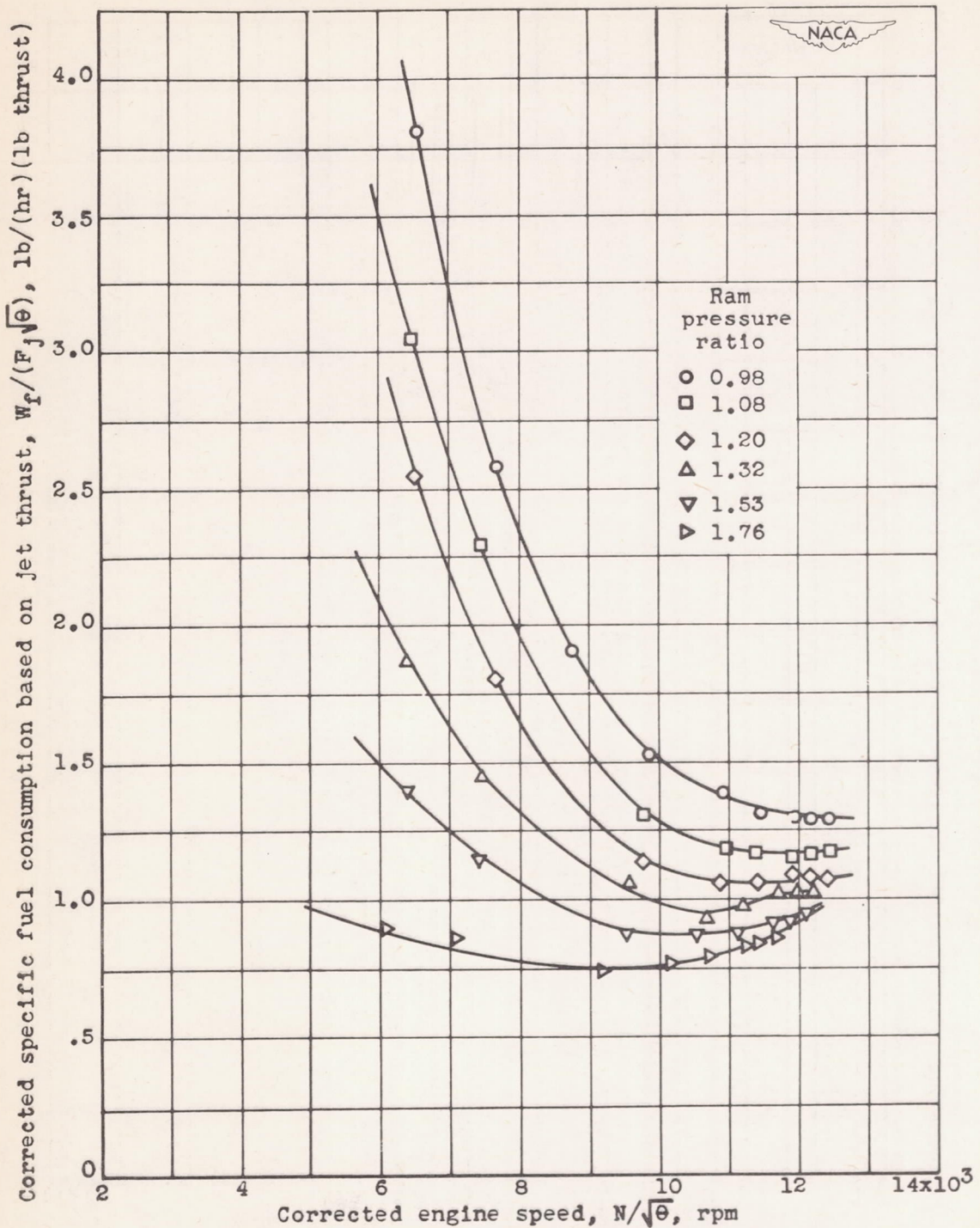
Figure 47.- Effect of corrected engine speed and ram pressure ratio on corrected specific fuel consumption based on jet thrust at altitude of 30,000 feet. Engine speed and specific fuel consumption corrected to NACA standard atmospheric conditions at sea level.
