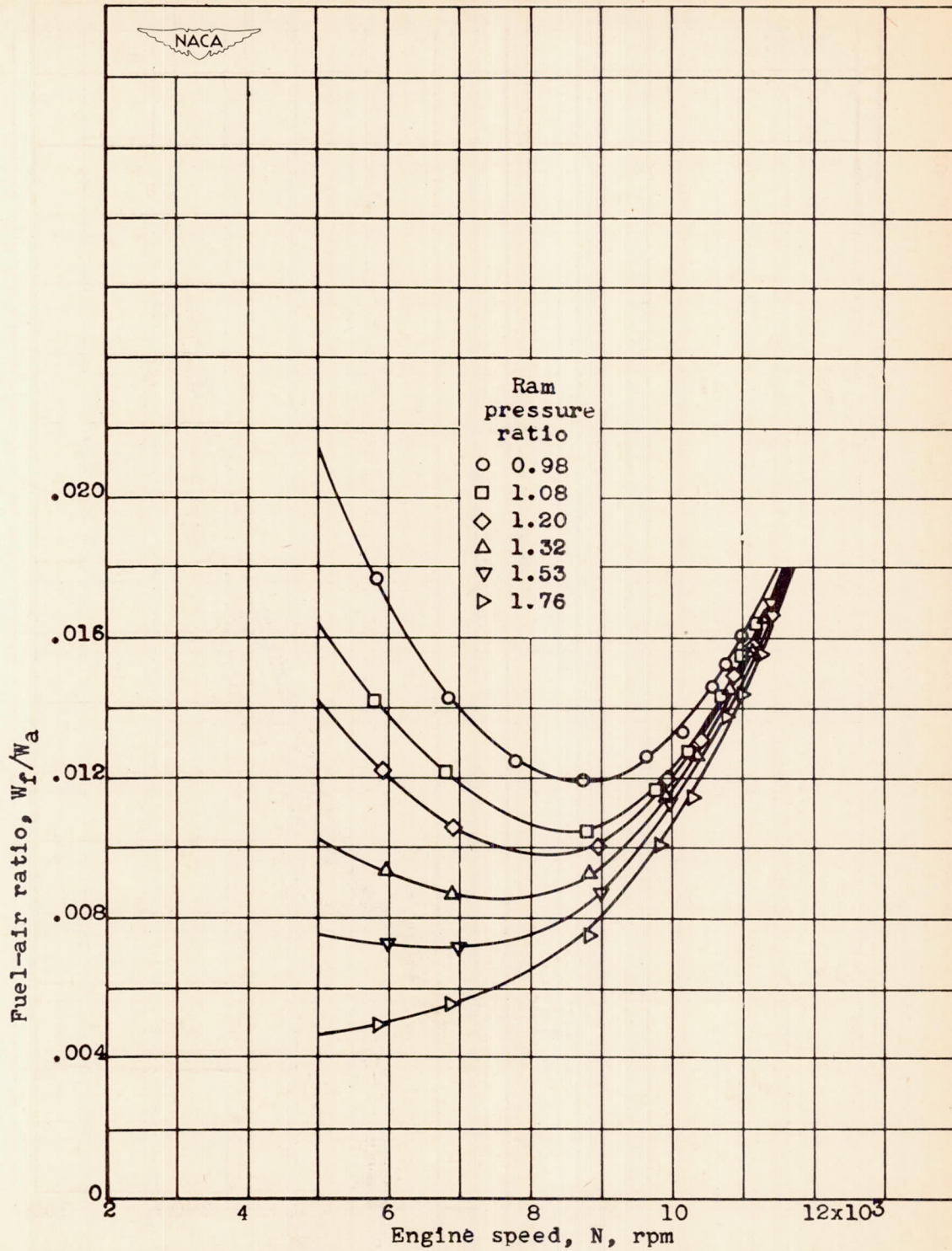
Figure 26.- Effect of engine speed and ram pressure ratio on fuel-air ratio at altitude of 30,000 feet.
