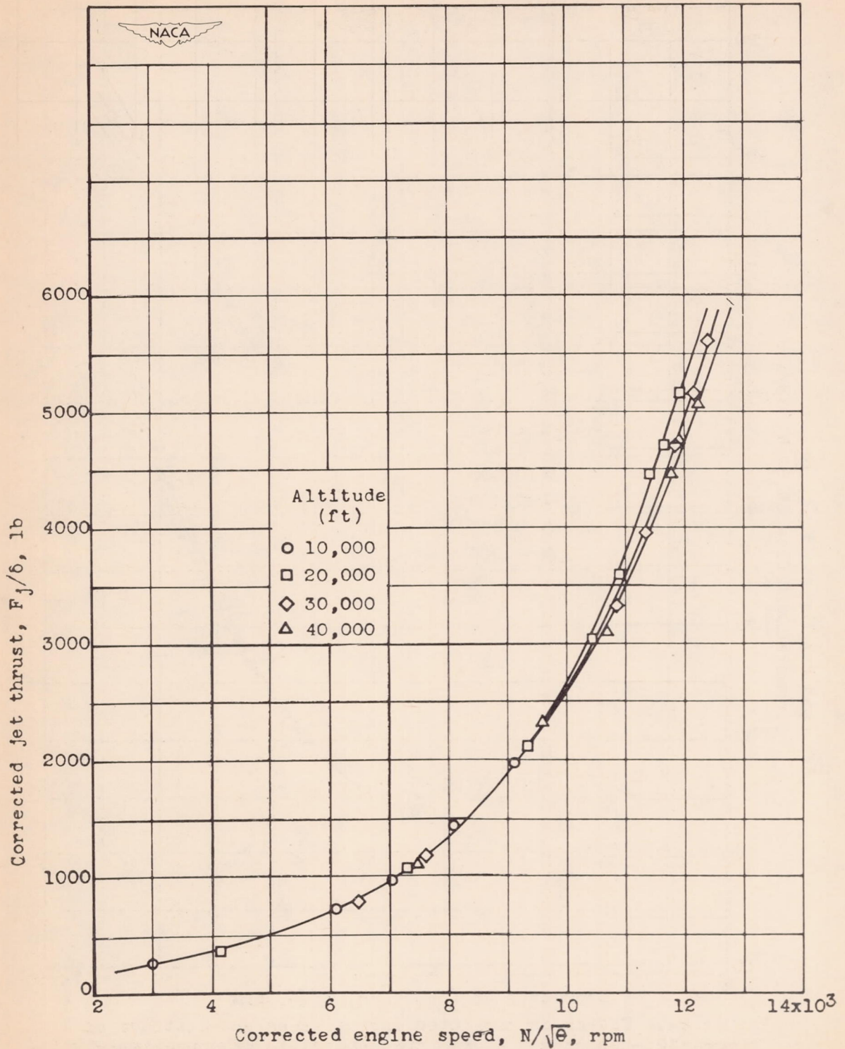
Figure 33.- Effect of corrected engine speed and altitude on corrected jet thrust at ram pressure ratio of approximately 1.2. Engine speed and jet thrust corrected to NACA standard atmospheric conditions at sea level.
