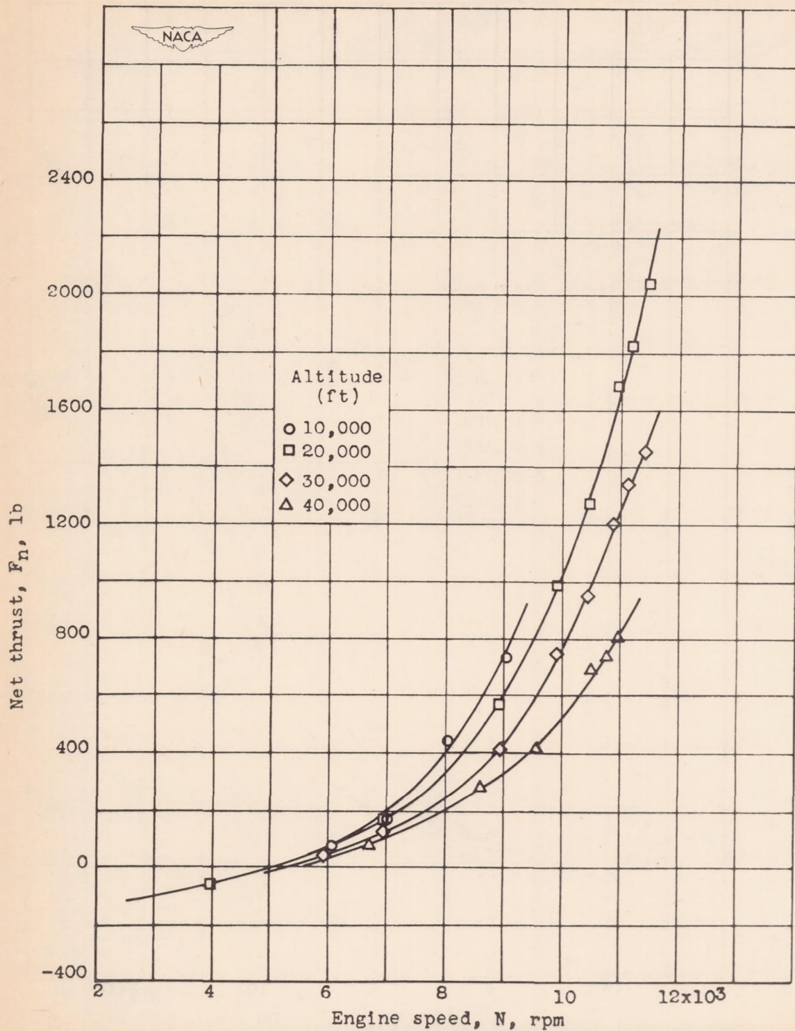
Figure 11.- Effect of engine speed and altitude on net thrust at ram pressure ratio of approximately 1.2.
