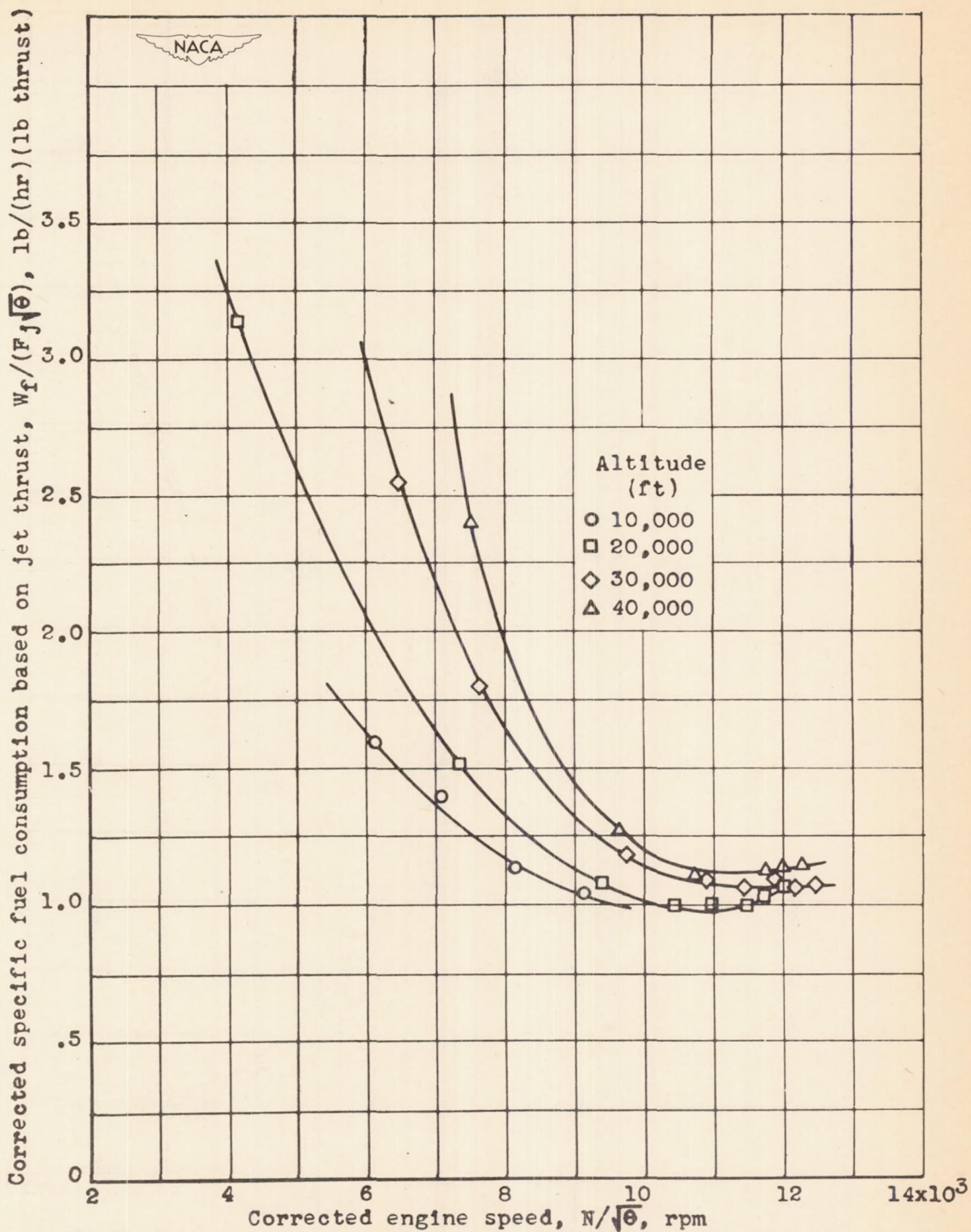
Figure 38.- Effect of corrected engine speed and altitude on corrected specific fuel consumption based on jet thrust at ram pressure ratio of approximately 1.2. Engine speed and specific fuel consumption corrected to NACA standard atmospheric conditions at sea level.
