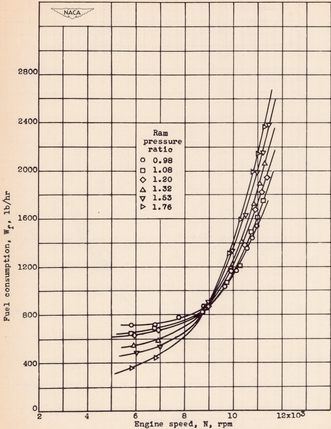
Figure 25.- Effect of engine speed and ram pressure ratio on fuel consumption at altitude of 30,000 feet.
