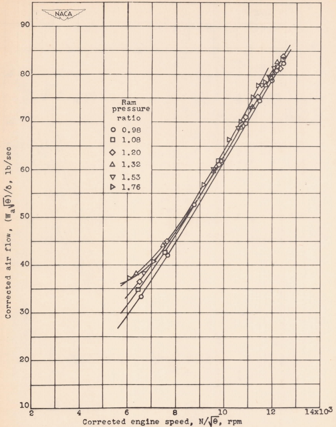
Figure 41.- Effect of corrected engine speed and ram pressure ratio on corrected air flow at altitude of 30,000 feet. Engine speed and air flow corrected to NACA standard atmospheric conditions at sea level.
