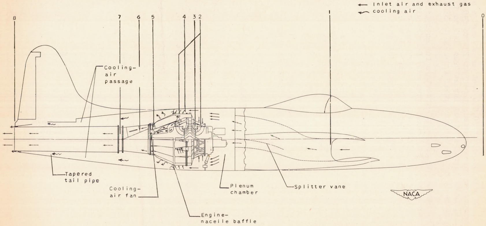
Figure 1. Installation of I-40 jet-propulsion engine.
