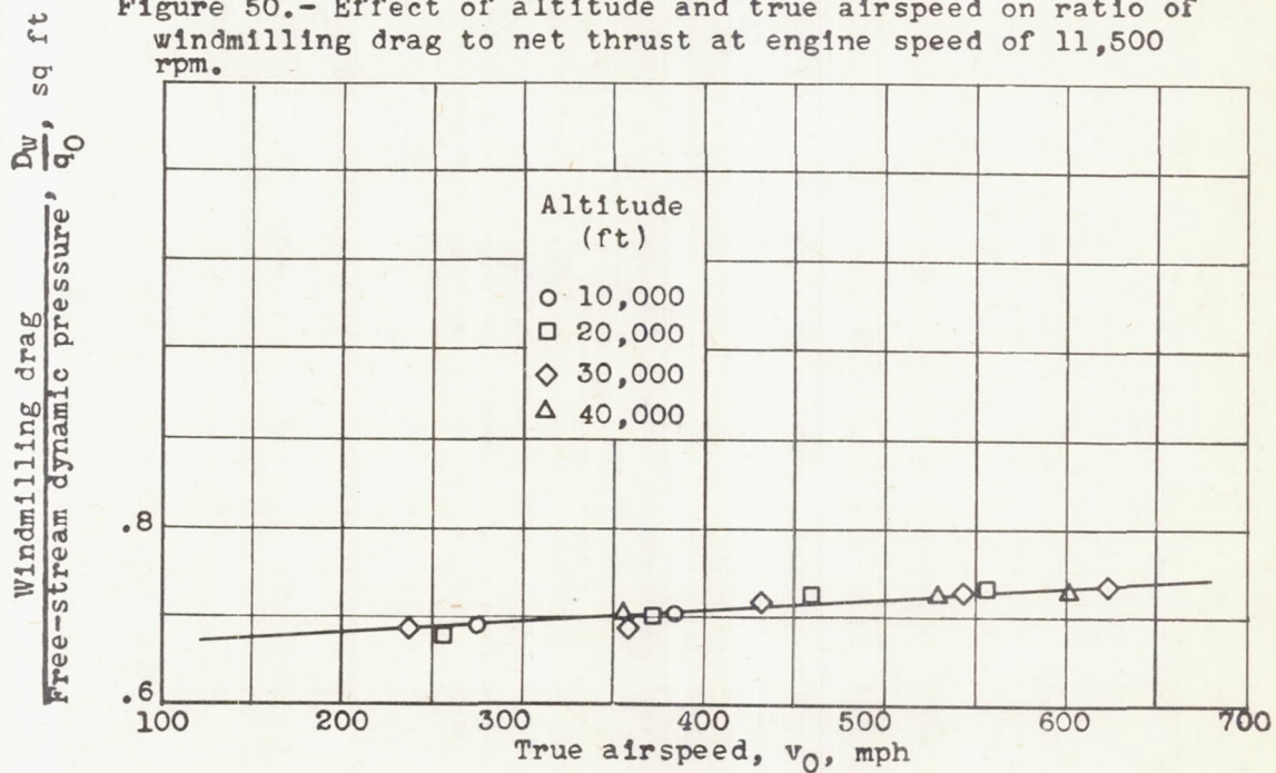
Figure 51.- Effect of pressure altitude and true airspeed on ratio of windmilling drag to free-stream dynamic pressure.
