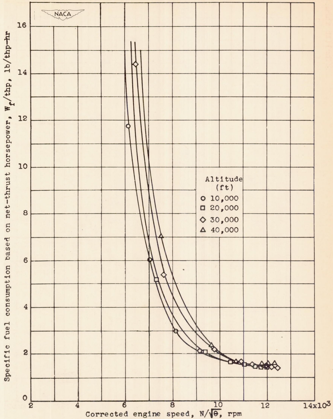
Figure 36.- Effect of corrected engine speed and altitude on specific fuel consumption based on net-thrust horsepower at ram pressure ratio of approximately 1.2. Engine speed corrected to NACA standard atmospheric conditions at sea level.
