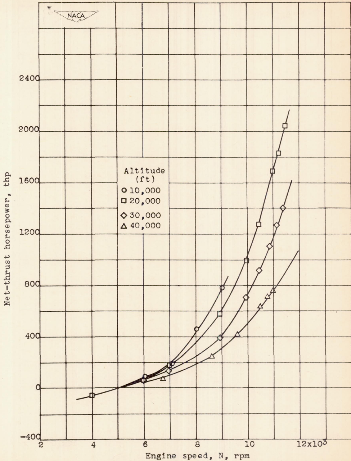
Figure 12.- Effect of engine speed and altitude on net-thrust horsepower at ram pressure ratio of approximately 1.2.
