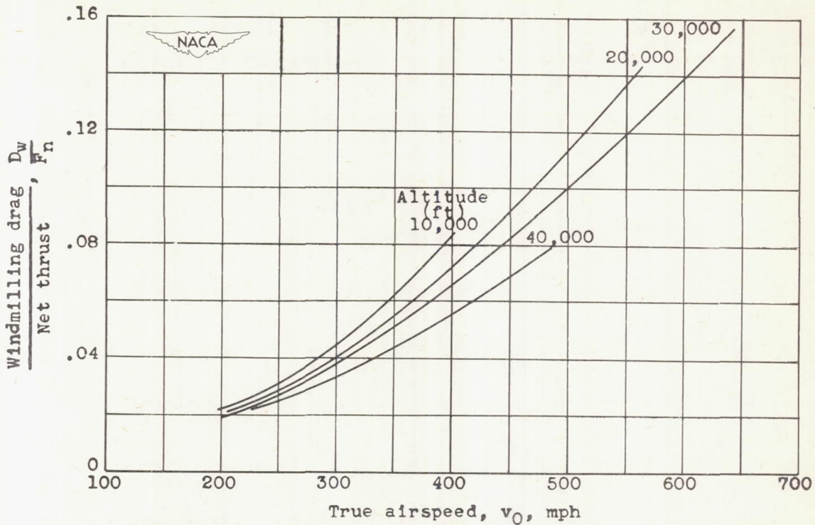
Figure 50.- Effect of altitude and true airspeed on ratio of windmilling drag to net thrust at engine speed of 11,500 rpm.
