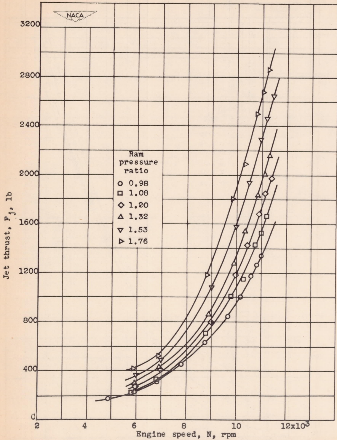
Figure 19.- Effect of engine speed and ram pressure ratio on jet thrust at altitude of 30,000 feet.
