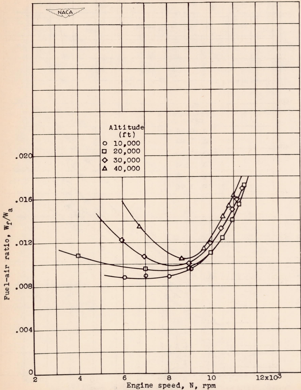
Figure 17.- Effect of engine speed and altitude on fuel-air ratio at ram pressure ratio of approximately 1.2.
