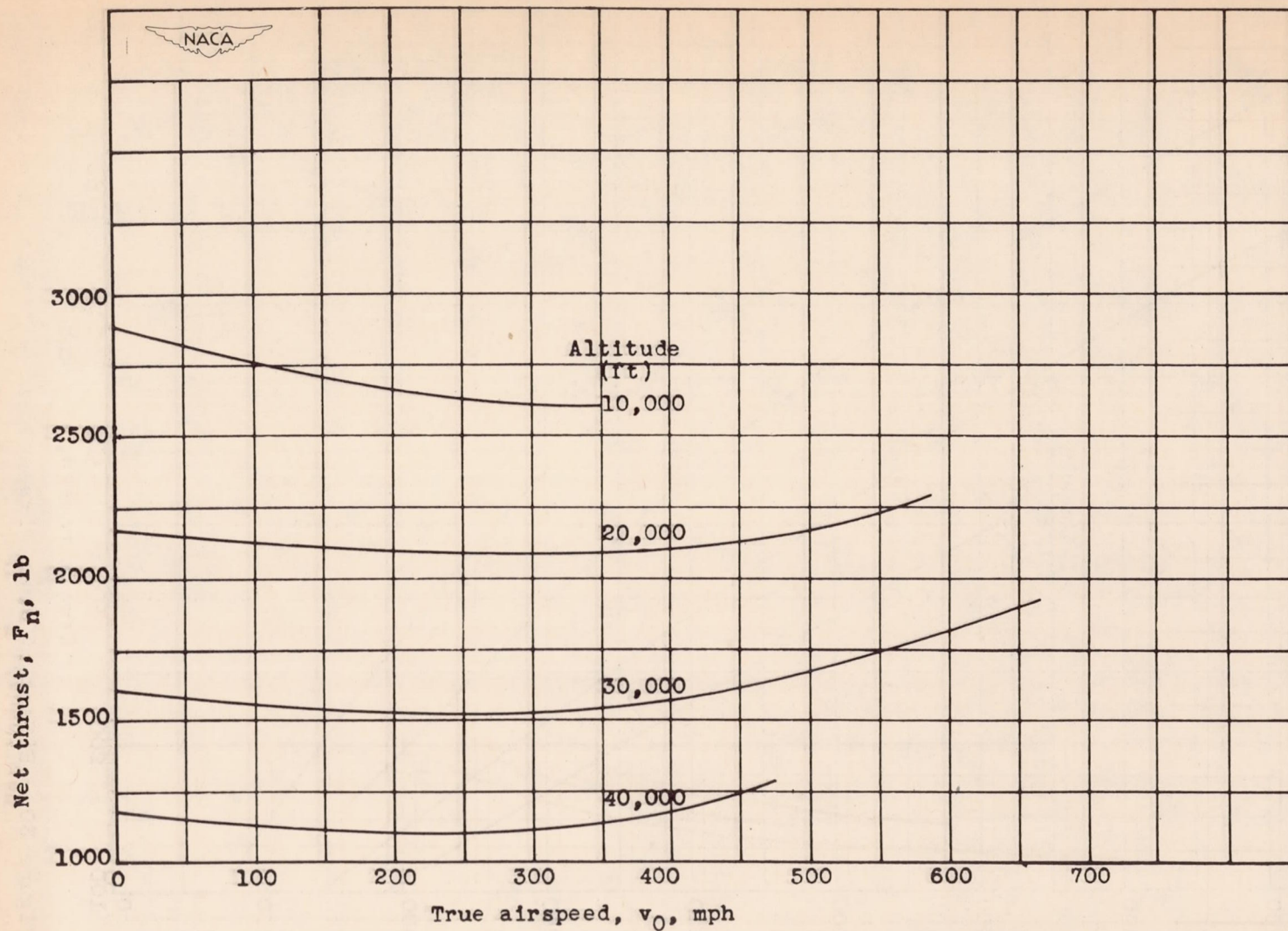
Figure 29.- Effect of true airspeed and altitude on net thrust at engine speed of 11,500 rpm.
