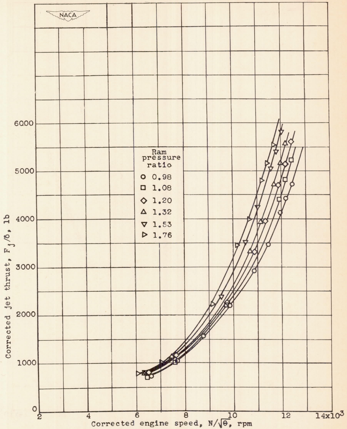
Figure 42.- Effect of corrected engine speed and ram pressure ratio on corrected jet thrust at altitude of 30,000 feet. Engine speed and jet thrust corrected to NACA standard atmospheric conditions at sea level.
