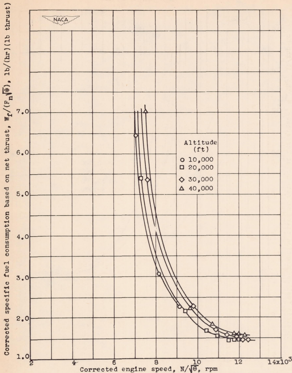
Figure 37.- Effect of corrected engine speed and altitude on corrected specific fuel consumption based on net thrust at ram pressure ratio of approximately 1.2. Engine speed and specific fuel consumption corrected to NACA standard atmospheric conditions at sea level.
