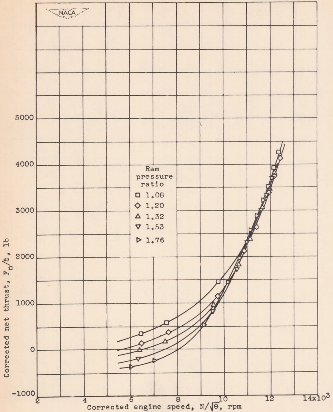
Figure 43.- Effect of corrected engine speed and ram pressure ratio on corrected net thrust at altitude of 30,000 feet. Engine speed and net thrust corrected to NACA standard atmospheric conditions at sea level.
