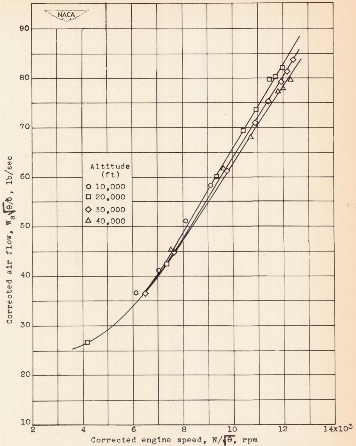
Figure 32.- Effect of corrected engine speed and altitude on corrected air flow at ram pressure ratio of approximately 1.2. Air flow and engine speed corrected to NACA standard atmospheric conditions at sea level.
