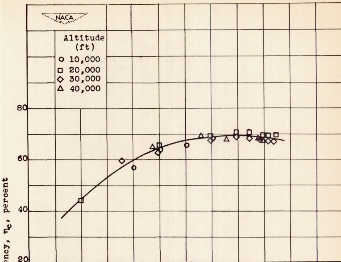
(a) Effect of altitude at ram-pressure ratio of approximately 1.2.
