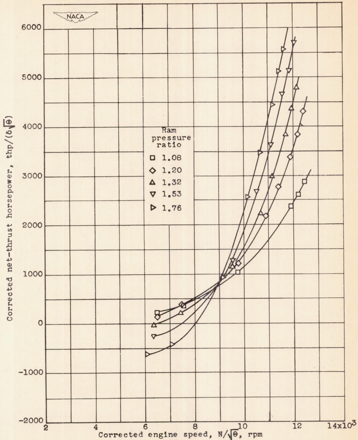
Figure 44.- Effect of corrected engine speed and ram pressure ratio on corrected net-thrust horsepower. Engine speed and net-thrust horsepower corrected to NACA standard atmospheric conditions at sea level.
