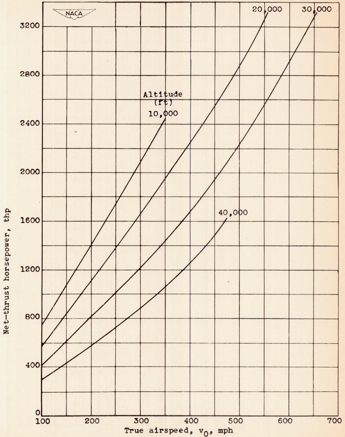
Figure 30.- Effect of true airspeed and altitude on net-thrust horsepower at engine speed of 11,500 rpm.
