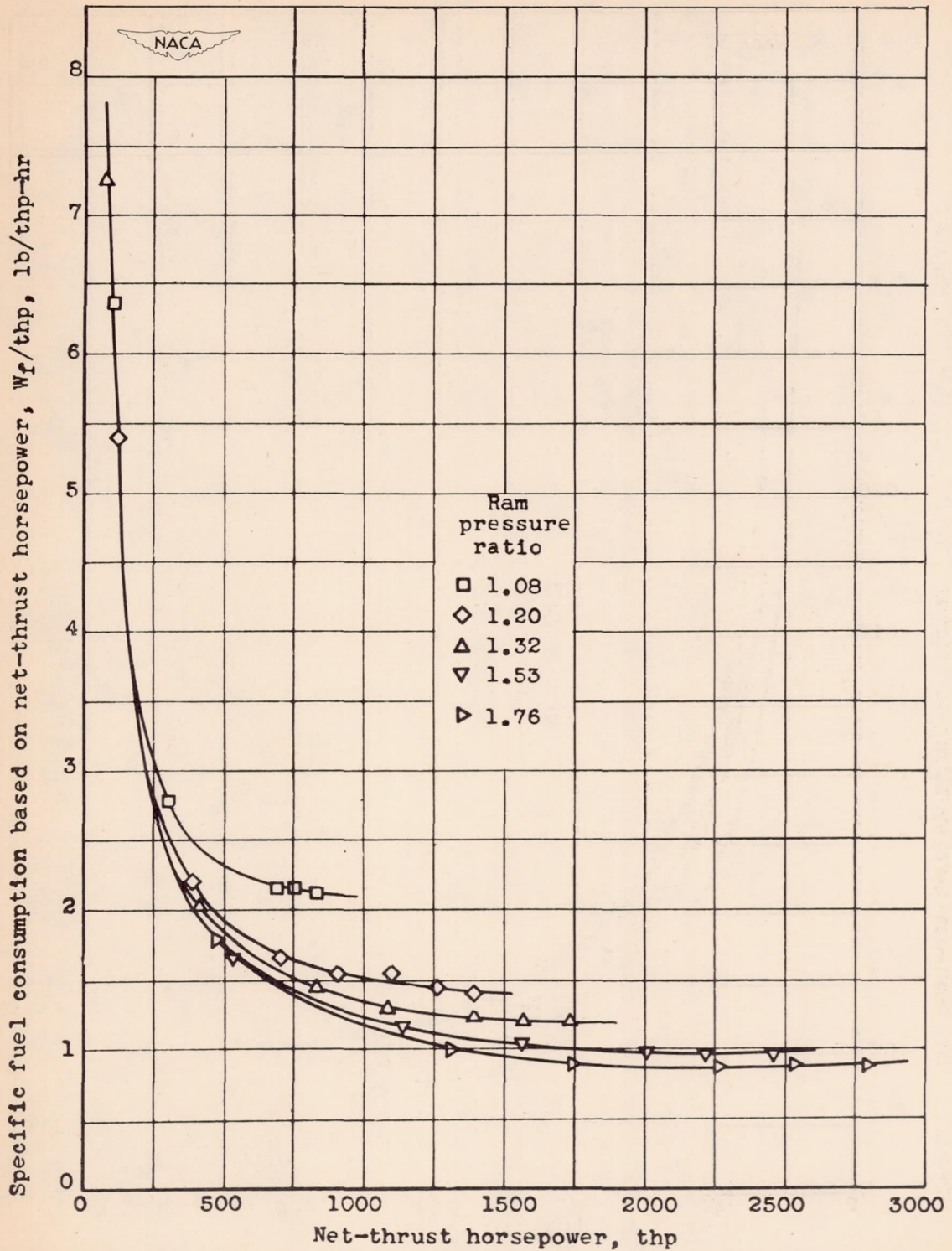
Figure 27.- Variation of specific fuel consumption based on net-thrust horsepower with ram pressure ratio and net-thrust horsepower at altitude of 30,000 feet.
