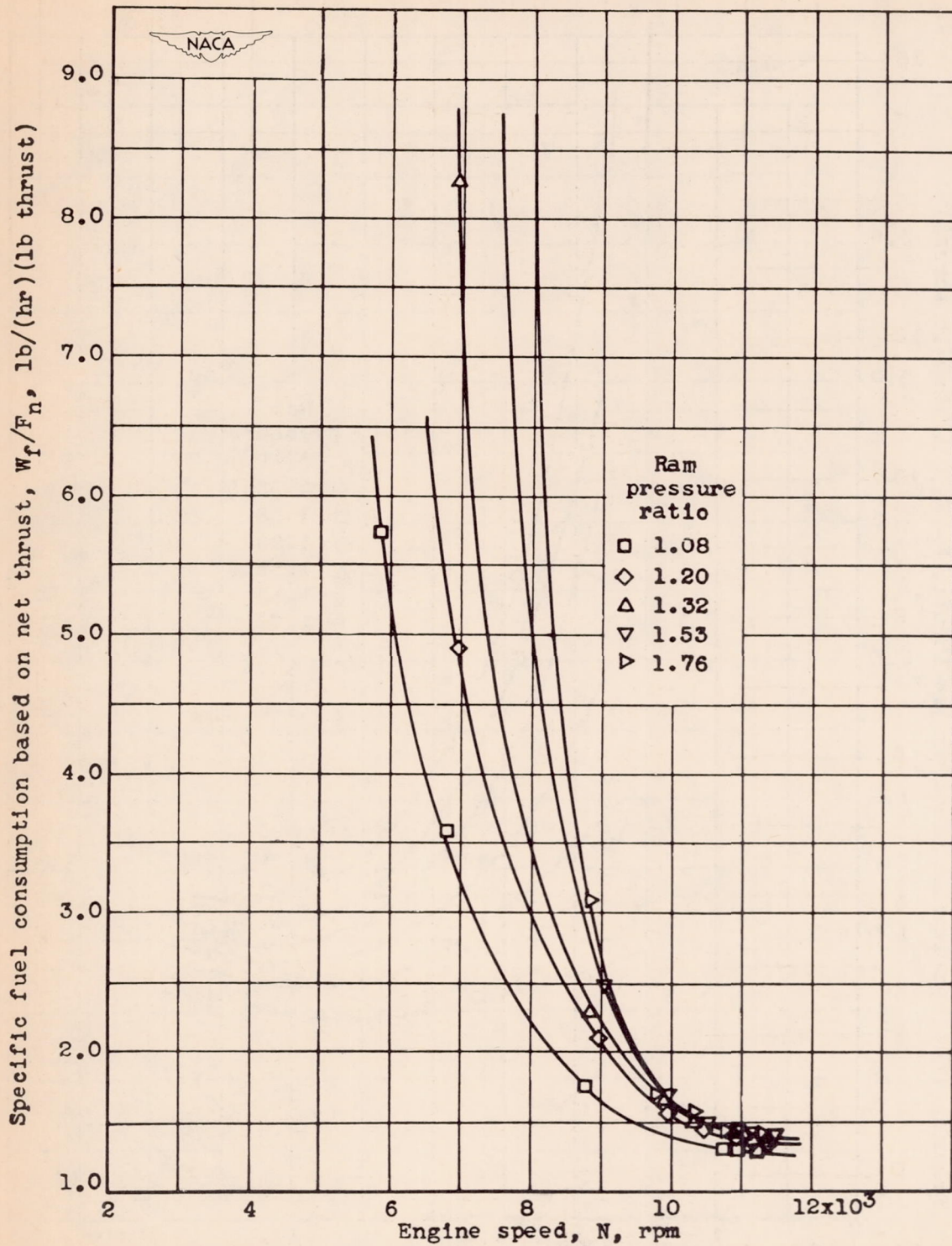
Figure 23.- Effect of engine speed and ram pressure ratio on specific fuel consumption based on net thrust at altitude of 30,000 feet.
