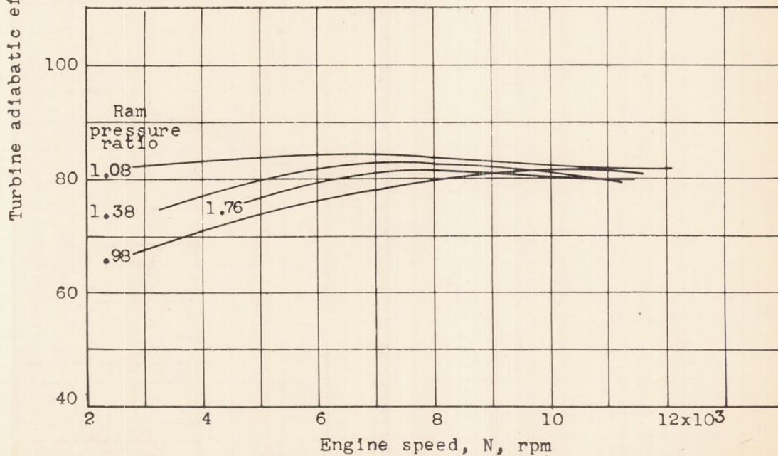
(b) Effect of ram pressure ratio at altitudes from 10,000 to 40,000 feet.
