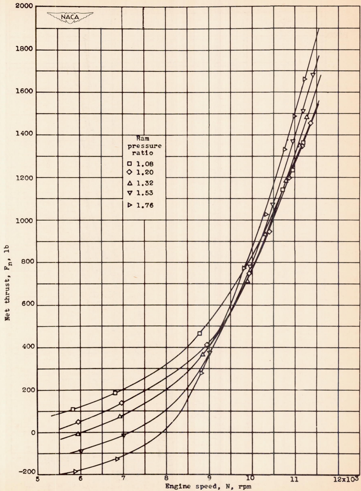
Figure 20.- Effect of engine speed and ram pressure ratio on net thrust at altitude of 30,000 feet.
