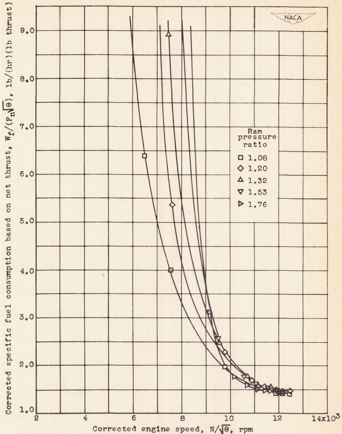
Figure 46.- Effect of corrected engine speed and ram pressure ratio on corrected specific fuel consumption based on net thrust at altitude of 30,000 feet. Engine speed and specific fuel consumption corrected to NACA standard atmospheric conditions at sea level.
