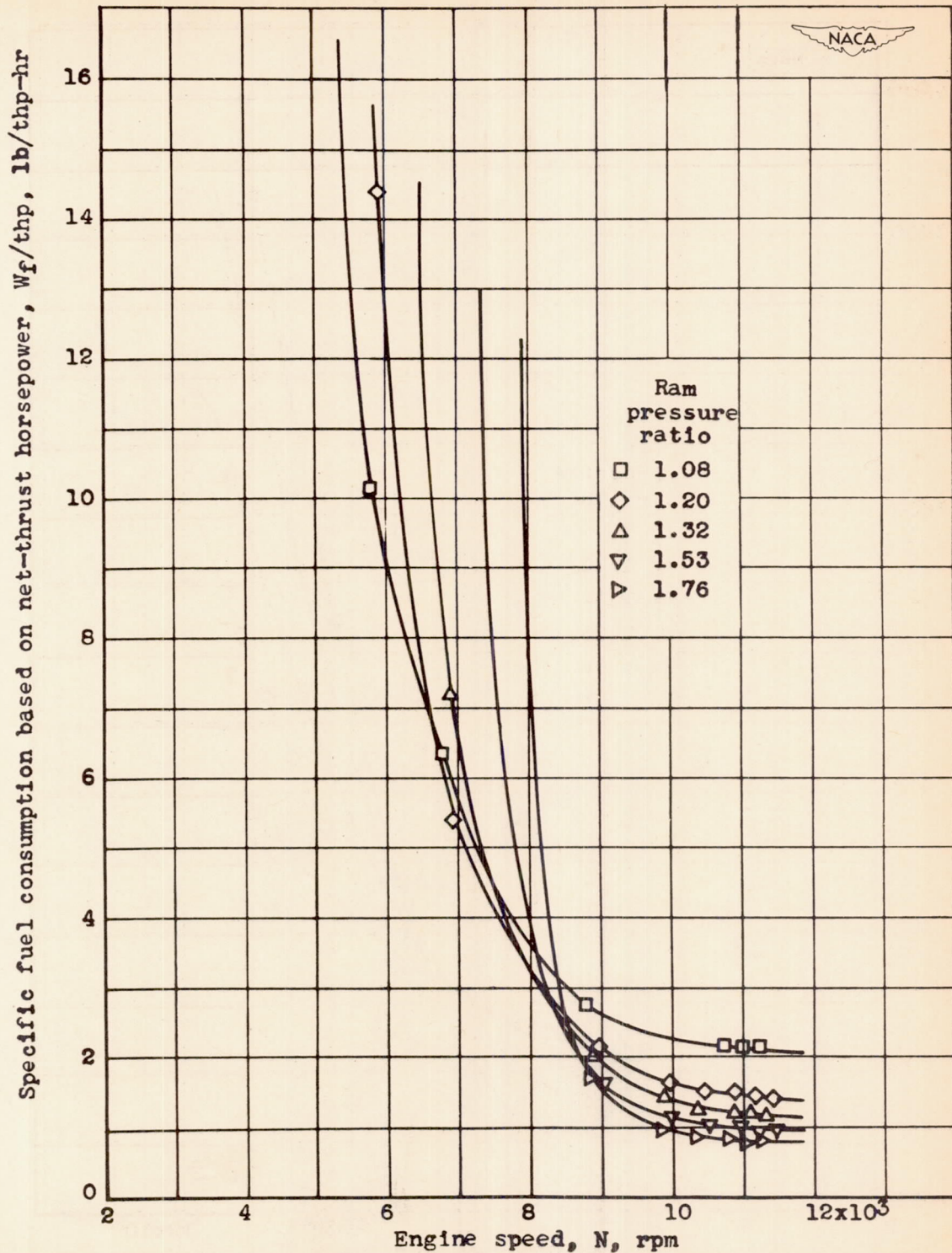
Figure 22.- Effect of engine speed and ram pressure ratio on specific fuel consumption based on net-thrust horsepower at altitude of 30,000 feet.
