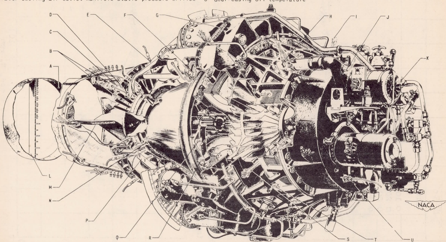
Figure 5. - Drawing of I-40 jet-propulsion engine showing location of instrumentation. (Slant type indicates instrumentation used to obtain data presented in this report.)
