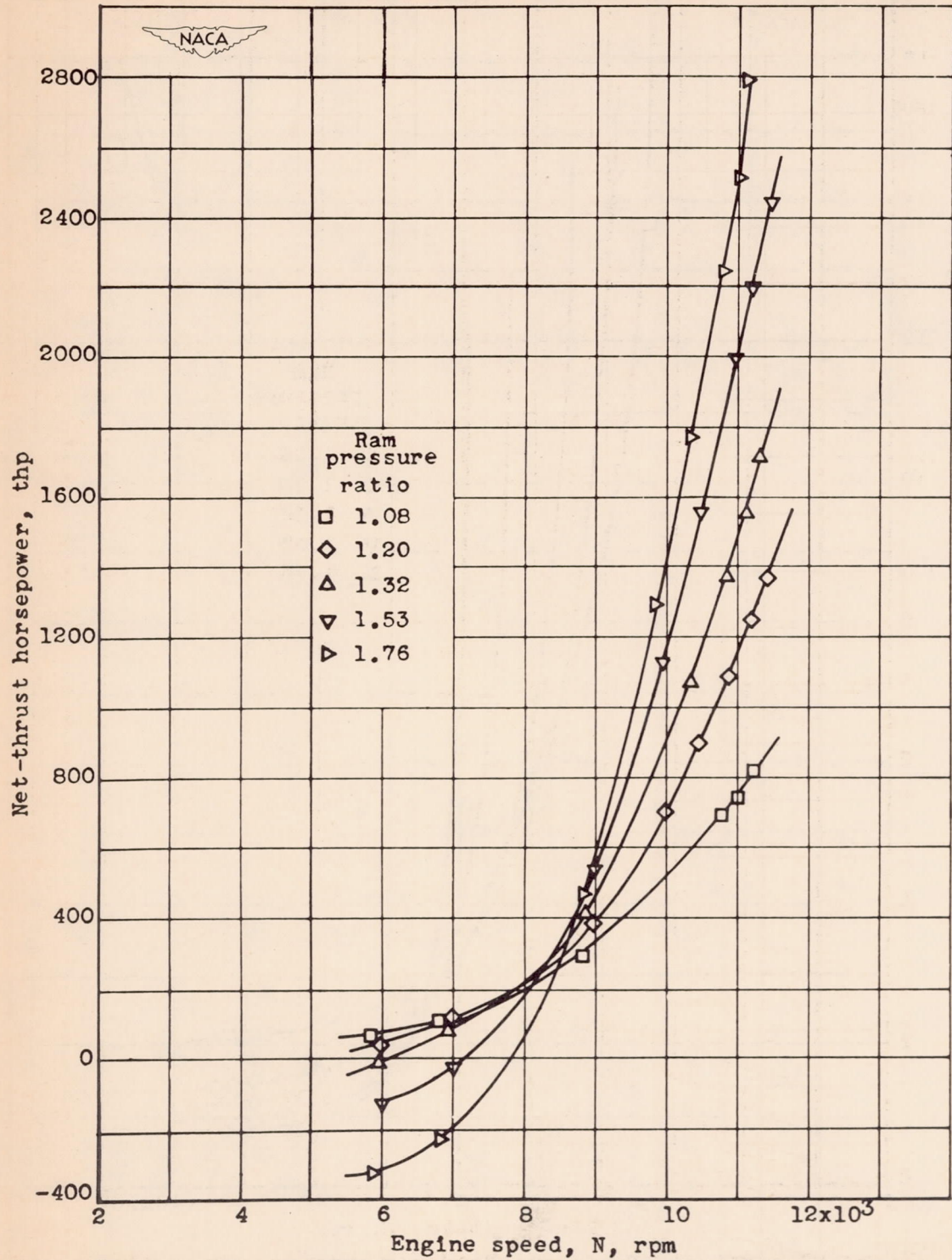
Figure 21.- Effect of engine speed and ram pressure ratio on net-thrust horsepower at altitude of 30,000 feet.
