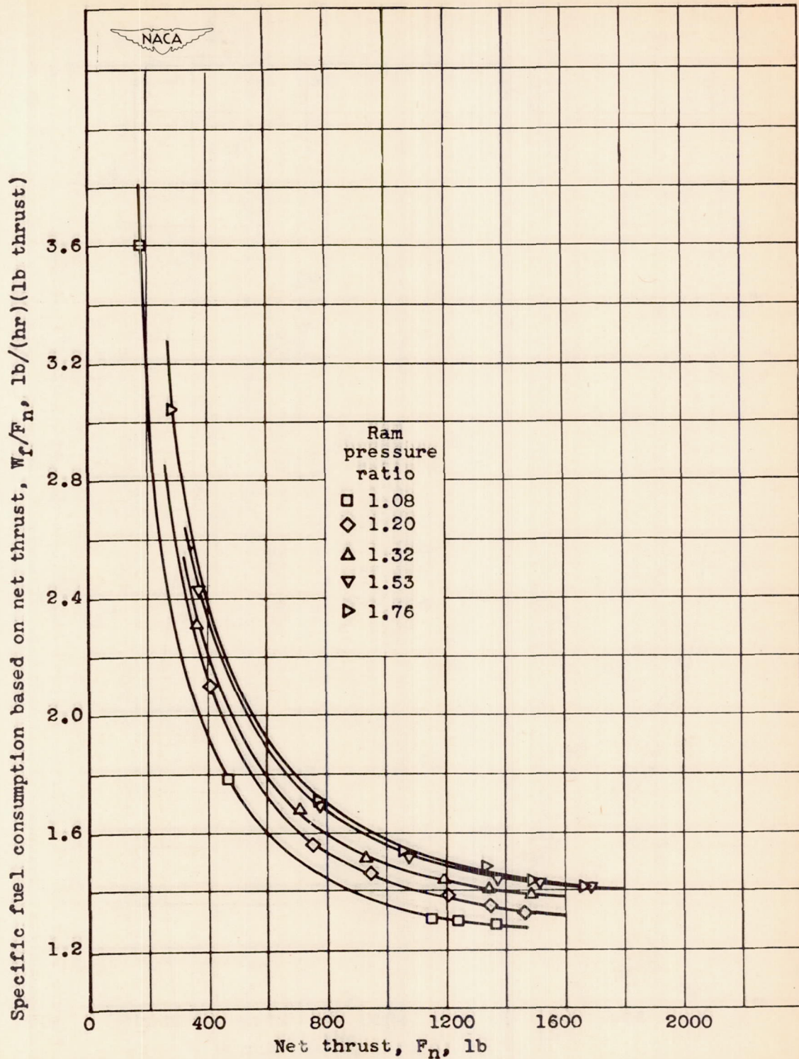
Figure 28.- Variation of specific fuel consumption based on net thrust with ram pressure ratio and net thrust at altitude of 30,000 feet.
