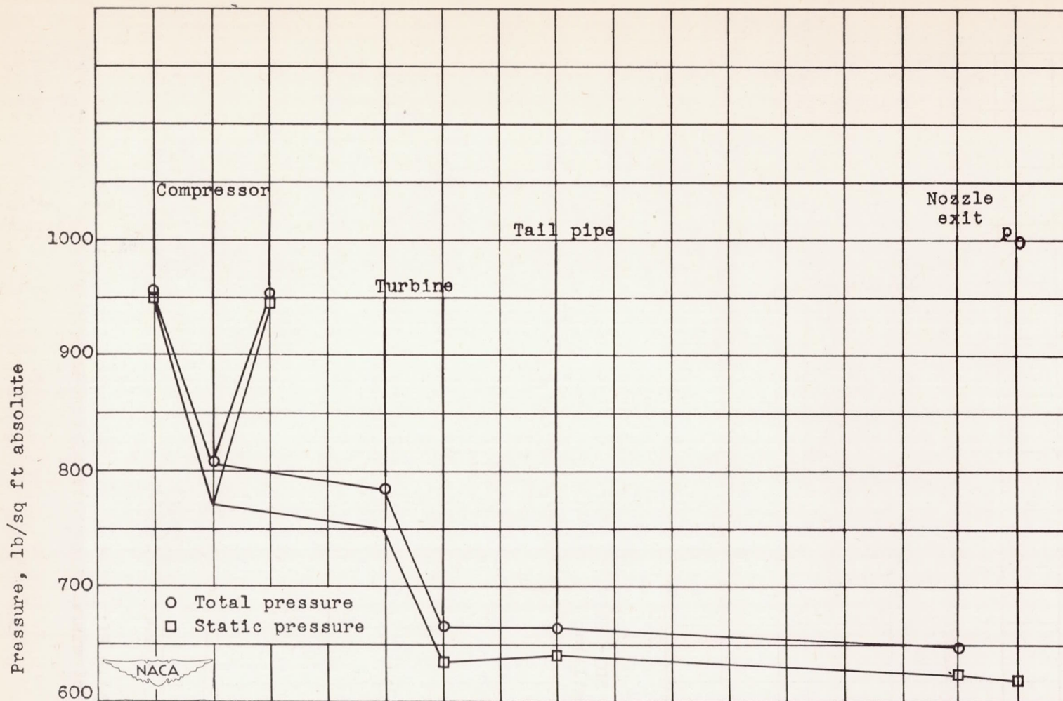
Figure 52.- Windmilling pressure survey of I-40 jet-propulsion engine. Pressure altitude, 30,000 feet; true airspeed, 543 miles per hour; ram pressure ratio, 1.53.
