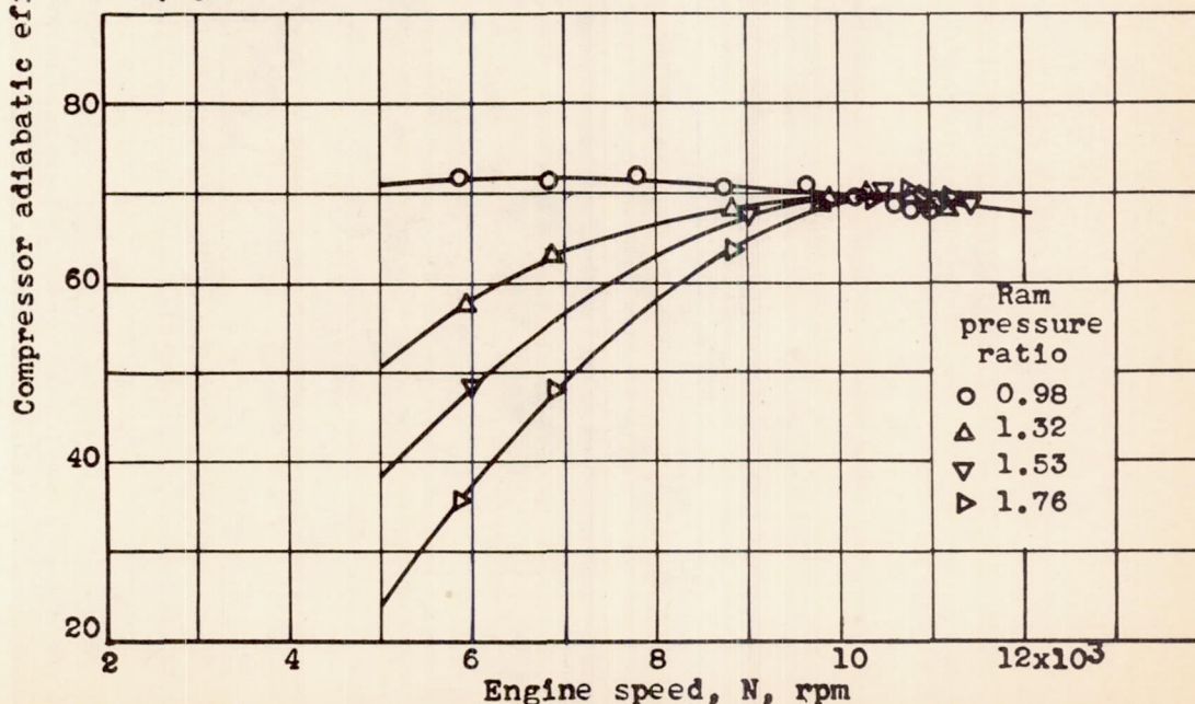
(b) Effect of ram pressure ratio at altitude of 30,000 feet.
