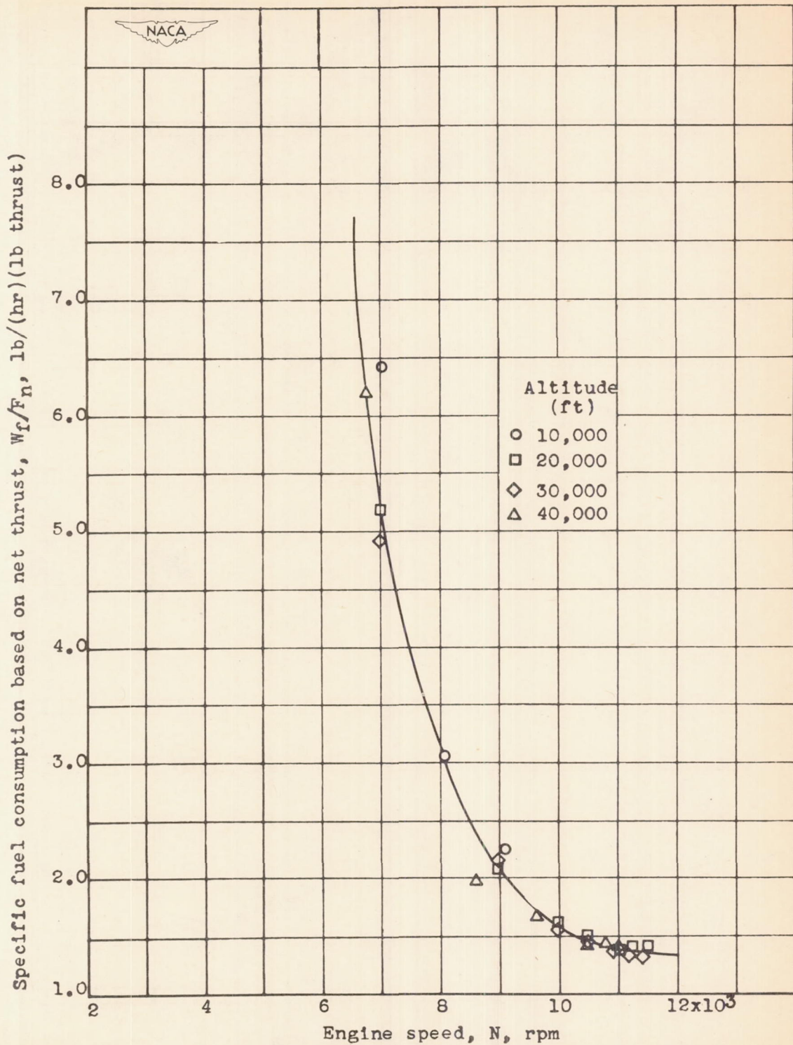
Figure 14.- Effect of engine speed and altitude on specific fuel consumption based on net thrust at ram pressure ratio of approximately 1.2.
