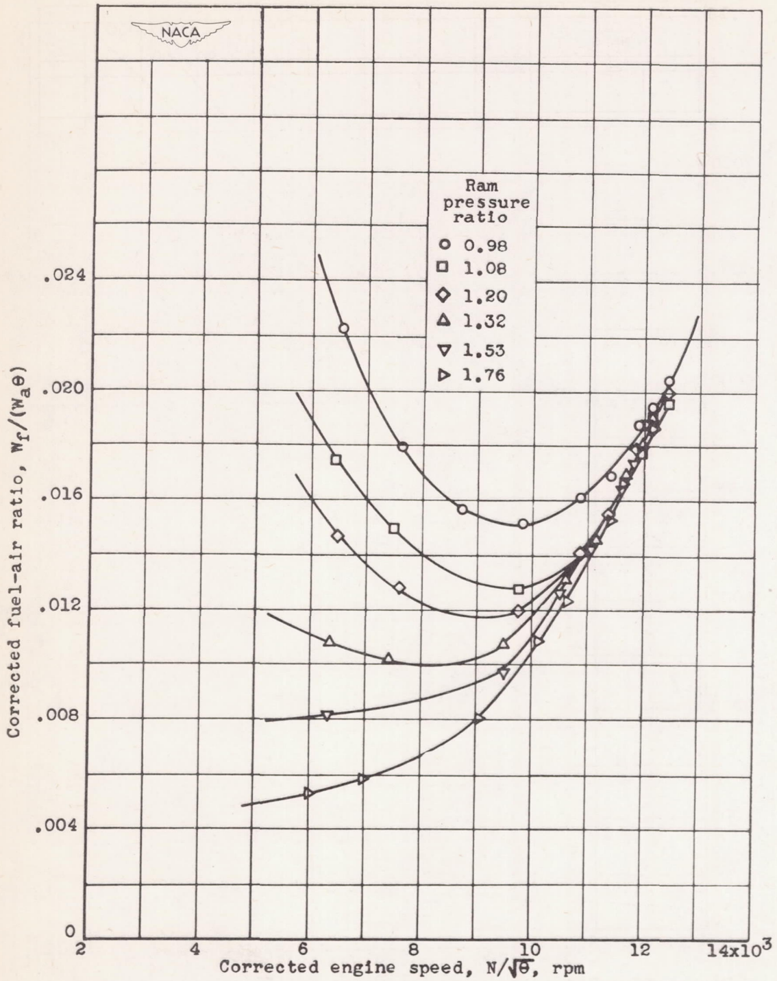
Figure 49.- Effect of corrected engine speed, and ram pressure ratio on corrected fuel-air ratio at altitude of 30,000 feet. Engine speed and fuel-air ratio corrected to NACA standard atmospheric conditions at sea level.
