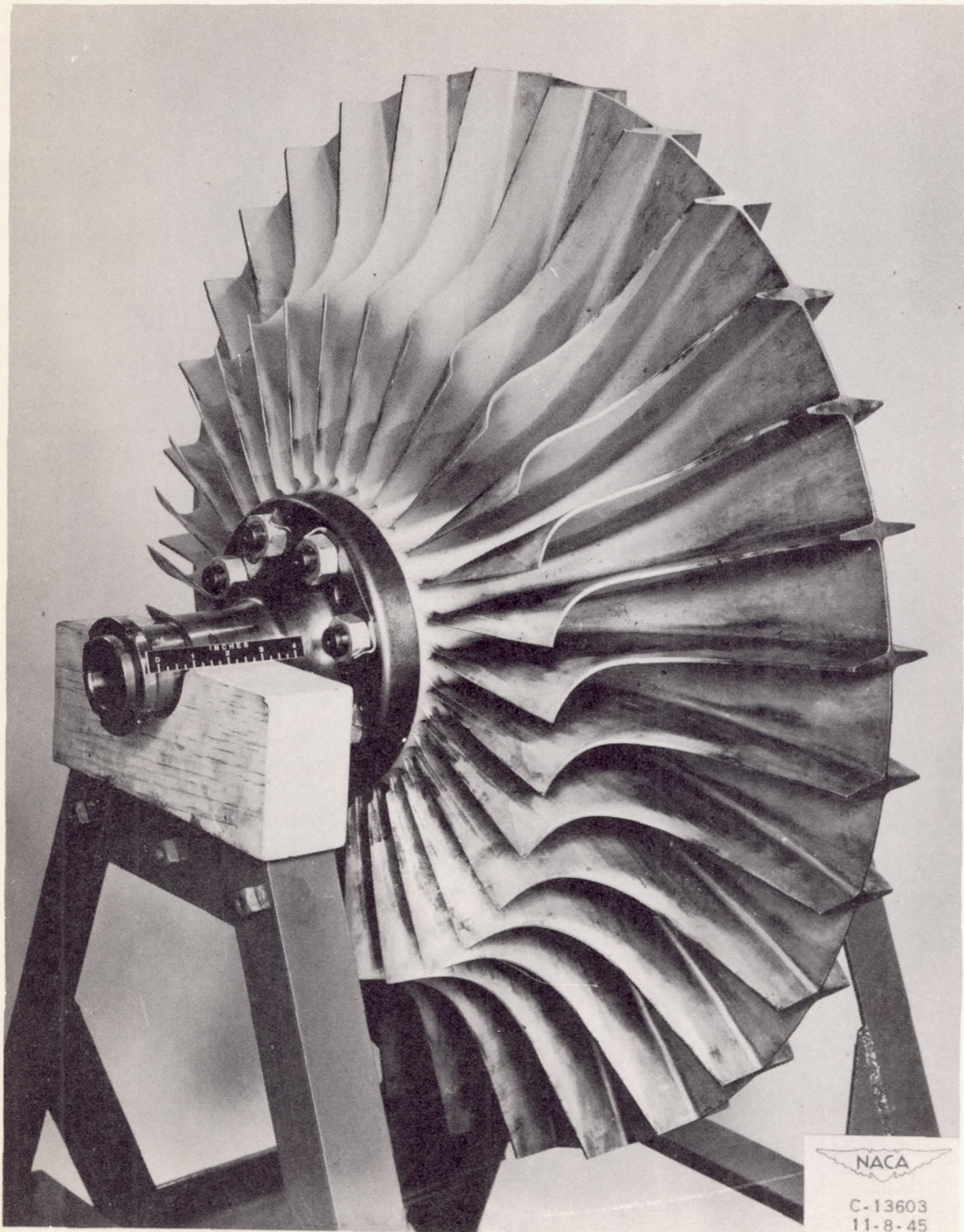
Figure 1. - Centrifugal-compressor impeller of I-40 jet-propulsion engine.
