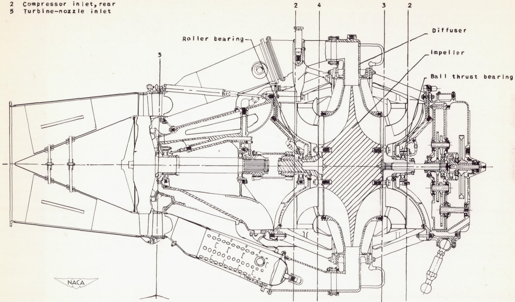
Figure 2. - Cross section of I-40 jet-propulsion engine.
