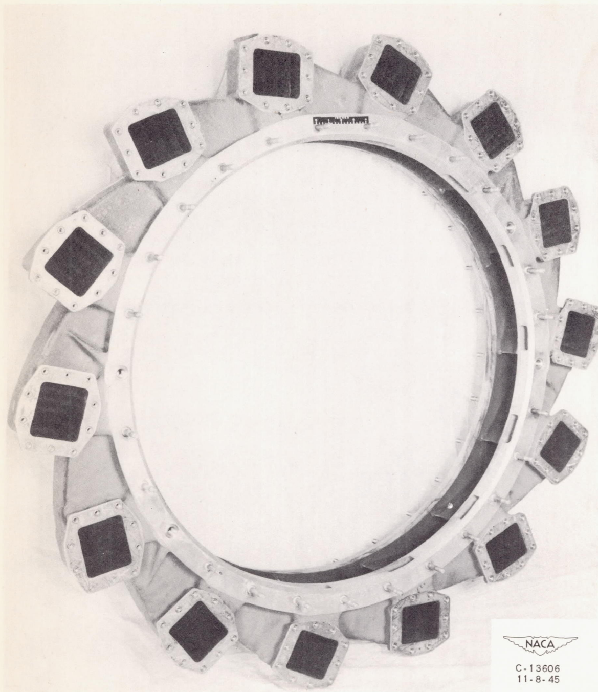
Figure 3. - Diffuser of I-40 jet-propulsion engine showing vanes around periphery and turning vanes in diffuser elbows.
