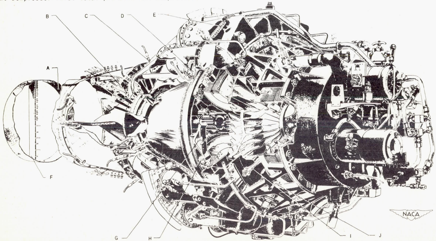
Figure 5. - Drawing of I-40 turbojet engine showing location of instrumentation.
