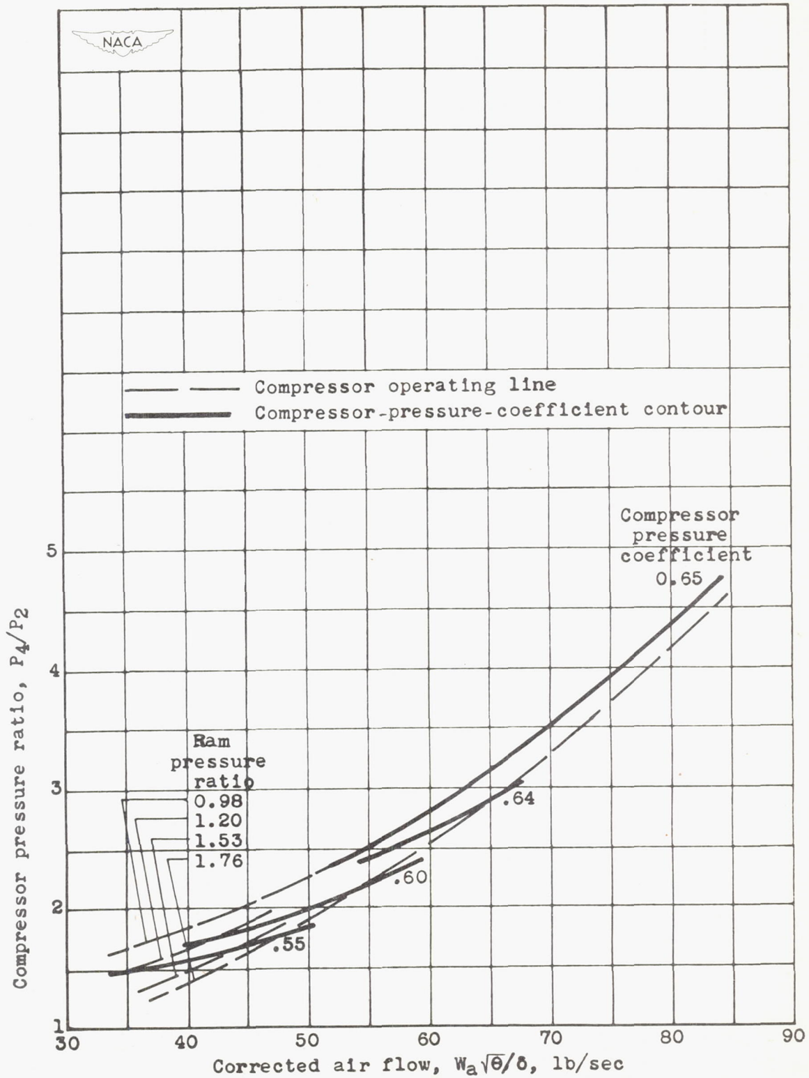
Figure 11.- Pressure coefficient contours at simulated altitude of 30,000 feet.
