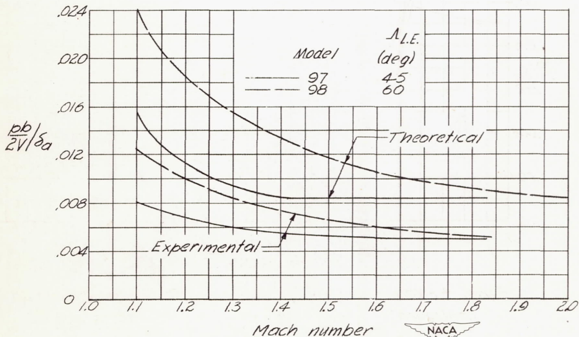
(b) Constant-chord ailerons. The experimental values are averages of 97e and 98a etc, respectively. Figure 5.- Comparison of experimental and theoretical results.
