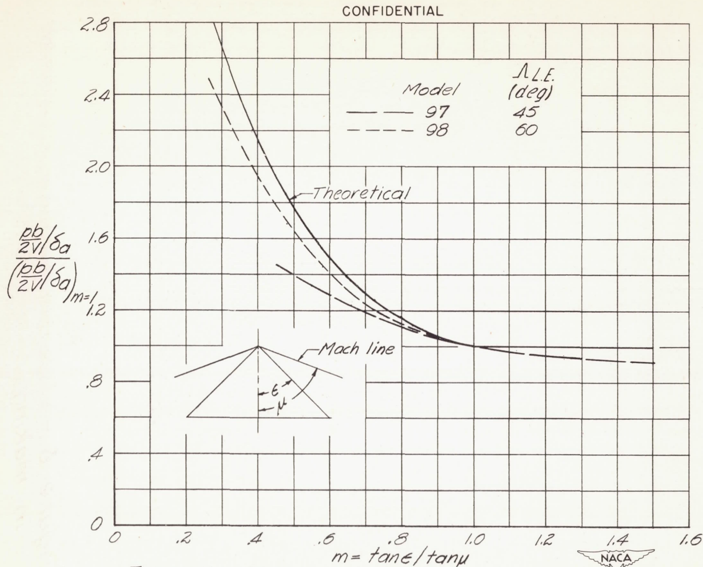
Figure 7.- Comparison of theoretical and experimental results. Constant-chord ailerons on delta wings.
