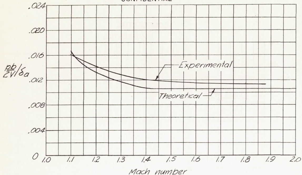
(a) Delta ailerons ; \Lambda_{LE} = 45^\circ ; model 84.
