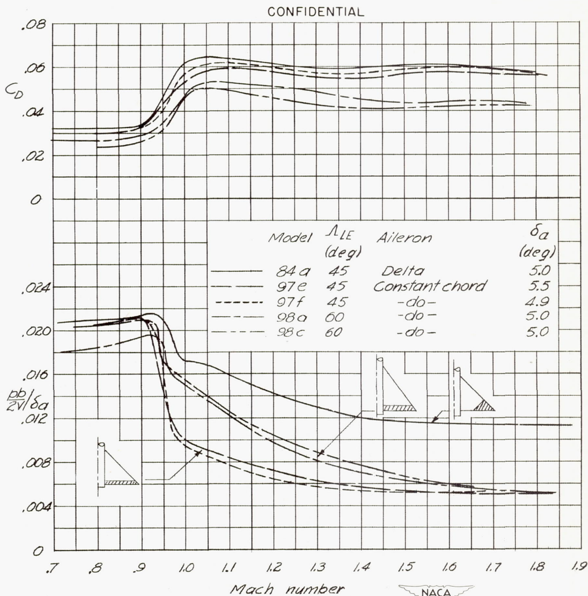
Figure 4.- Variation of \frac{p_b}{2V/s_a} and C_D with Mach number for configurations of present tests.
