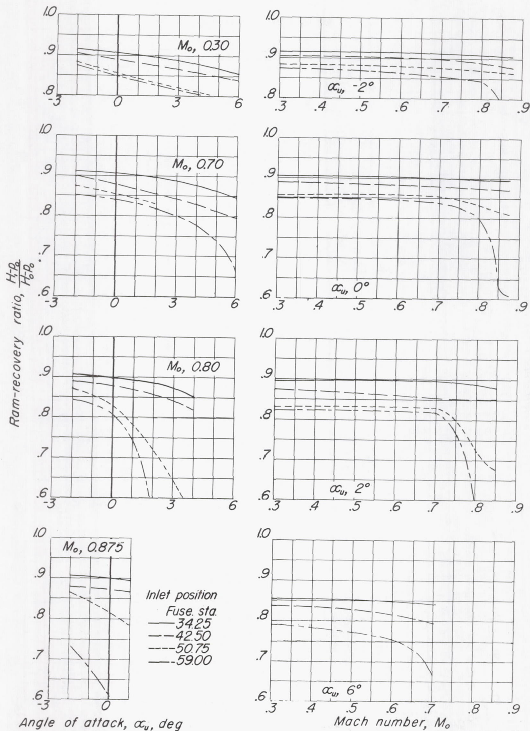
(a) m_1/m_o, 0.60 Figure 8 — Effect of inlet location on ram-recovery ratio. No deflectors on ramp; natural boundary layer.
