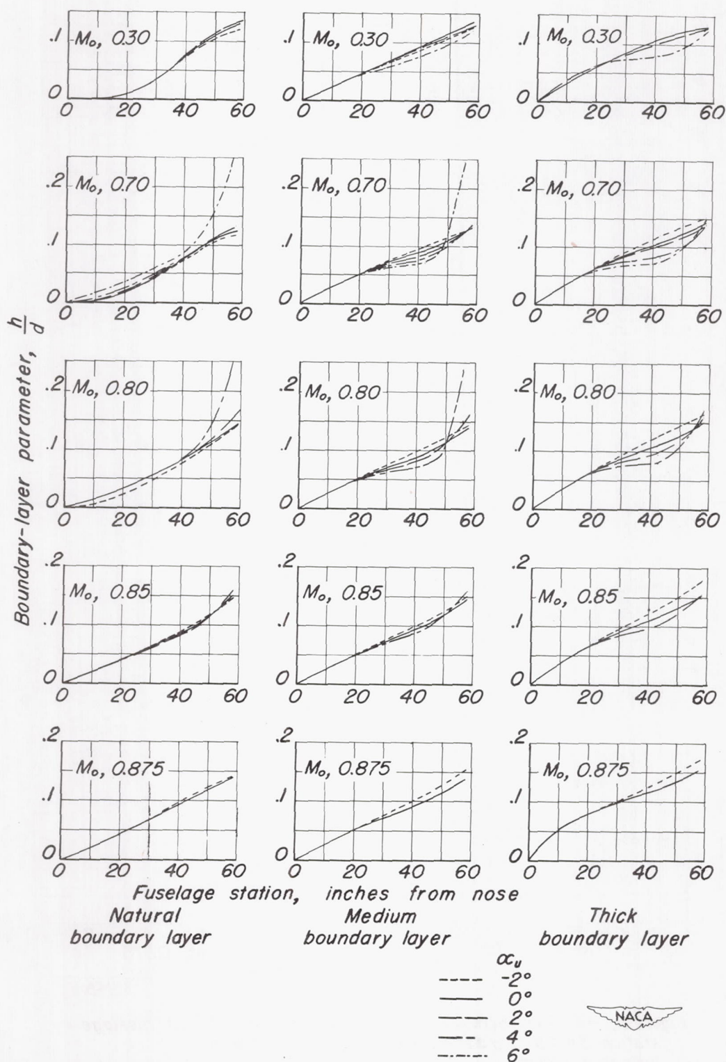
Figure 6. — Boundary-layer parameter.
