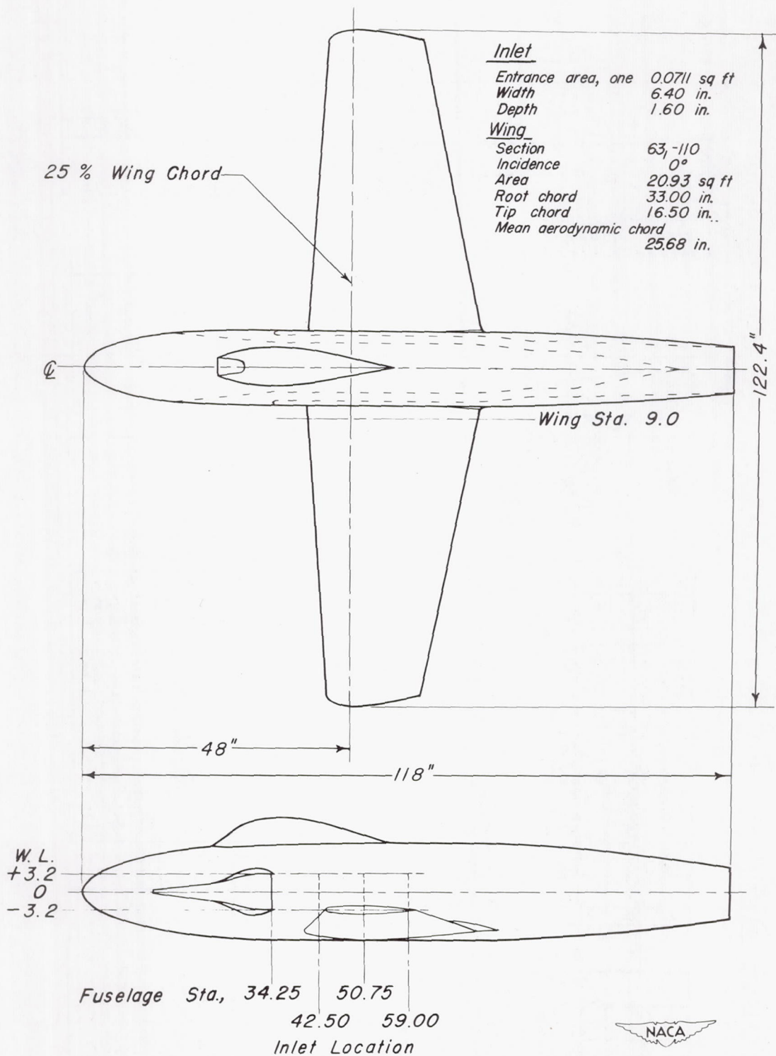
Figure 2. — Submerged-inlet model.
