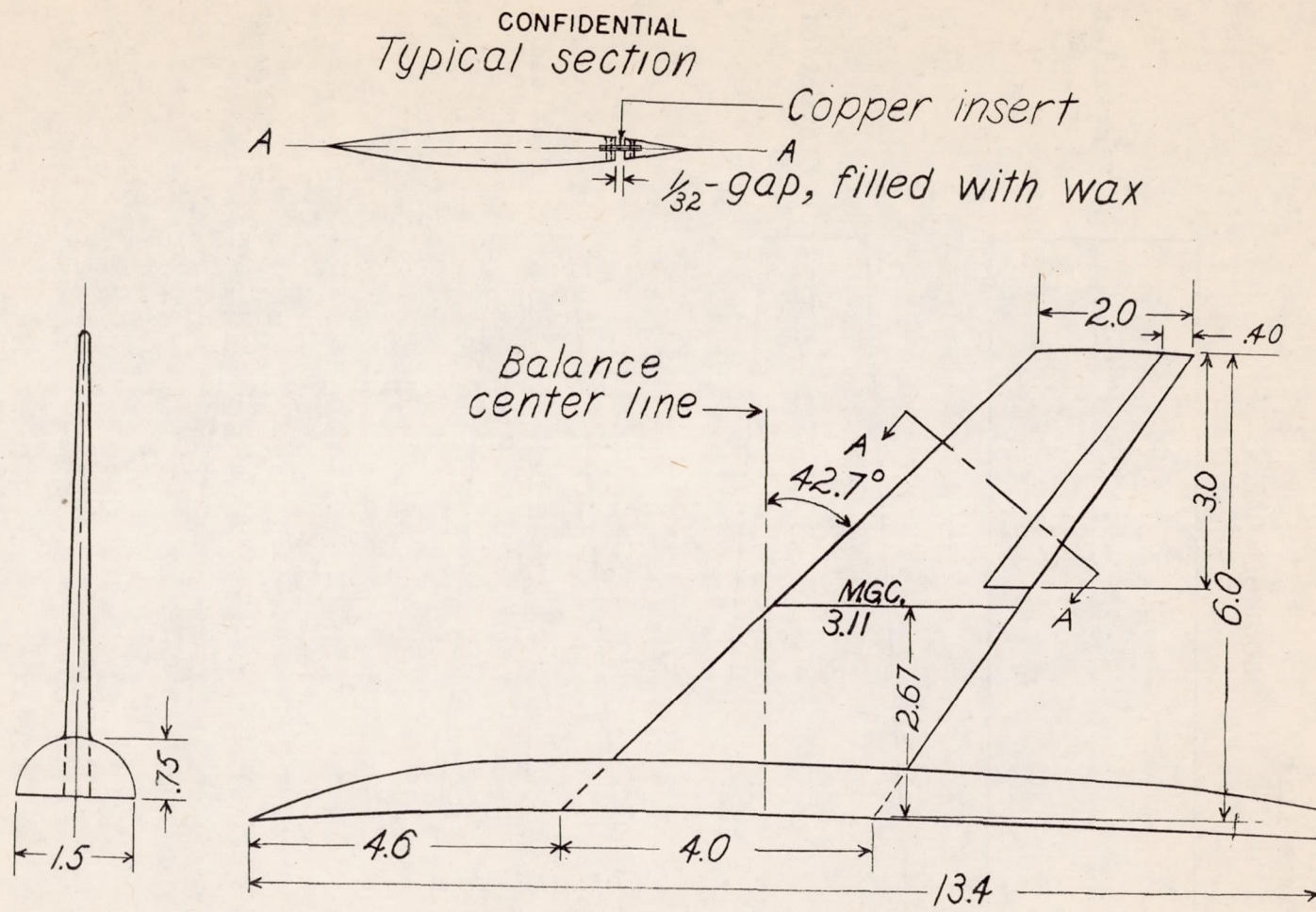
Figure 1.- Drawing of the 42.7° sweptback wing and fuselage combination. All dimensions in inches.
