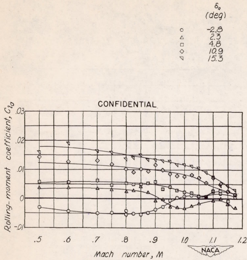
Figure 15.- Variation of rolling-moment coefficient with Mach number for a 0.20-chord circular-arc aileron. t = 0 ; \alpha = 0^\circ ; data from transonic bump.
