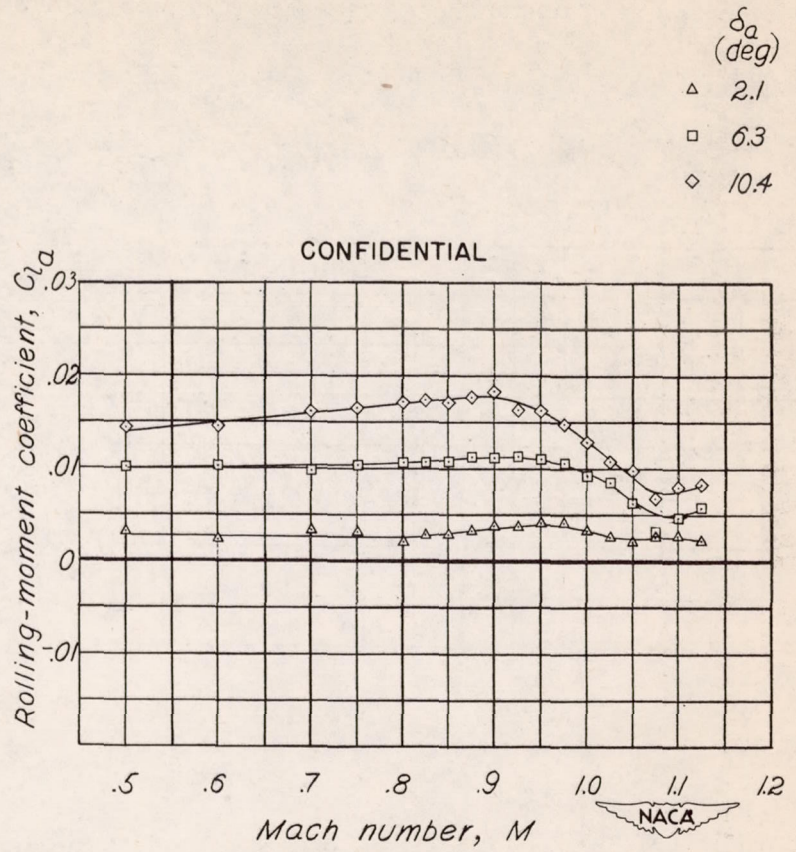
Figure 16.- Variation of rolling-moment coefficient with Mach number for a 0.20-chord flat-sided aileron. t = 1.00 ; \alpha = 0^\circ ; data from transonic bump.
