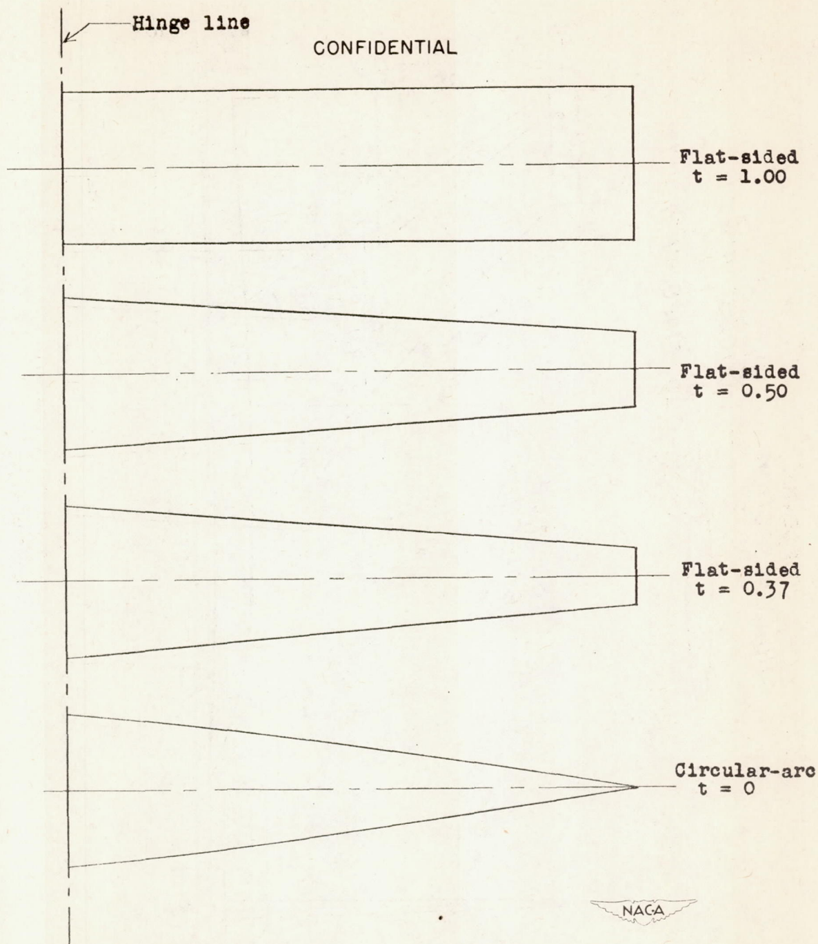
Figure 2.- Section profiles of the 0.20c aileron tested.
