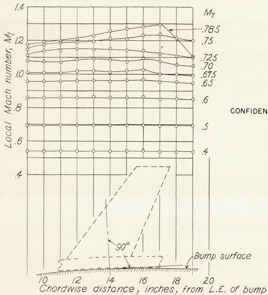
Figure 5.- Spanwise and chordwise distribution of Mach number over transonic bump. Model off.
